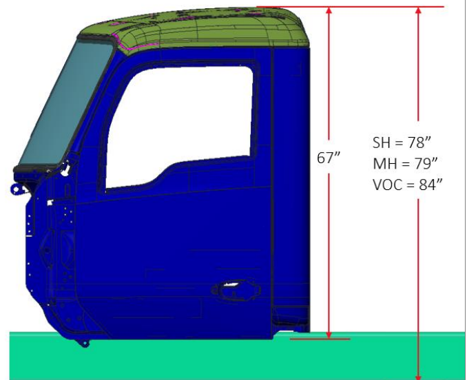
Figure 12 Low Roof and Raised Roof Cab Height 2.1m Medium Duty
