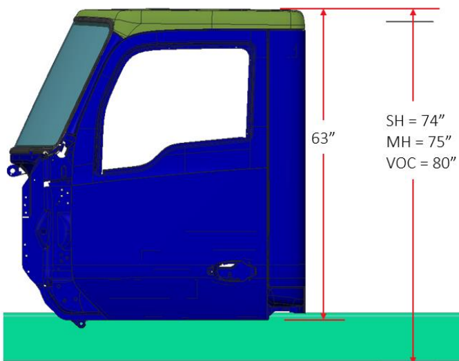
Figure 12 Low Roof and Raised Roof Cab Height 2.1m Medium Duty
