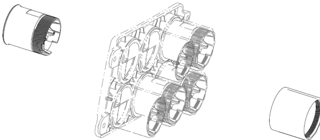
FIGURE 8-33. Gauge Installation
