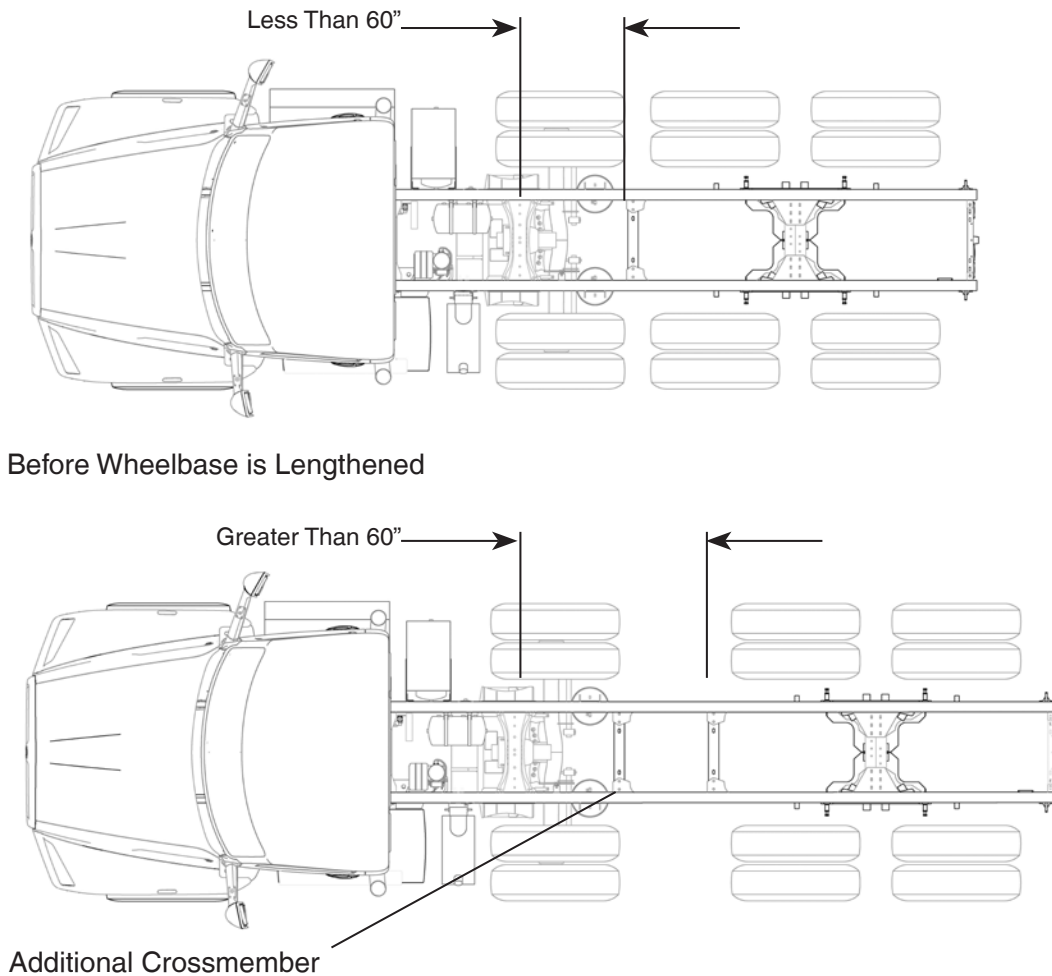
FIGURE 7-4. Crossmember Added When Distance Exceeds 60 Inches (1524 mm)
