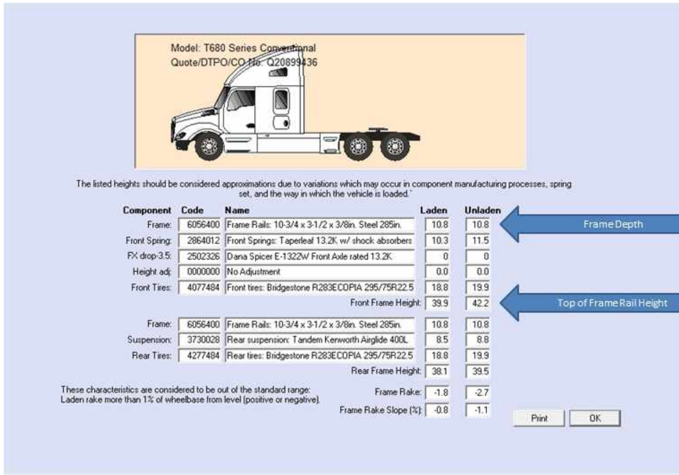
FIGURE 4-58. Dimension A = Top of Rail Frame Height from Prospector – Frame Depth.
