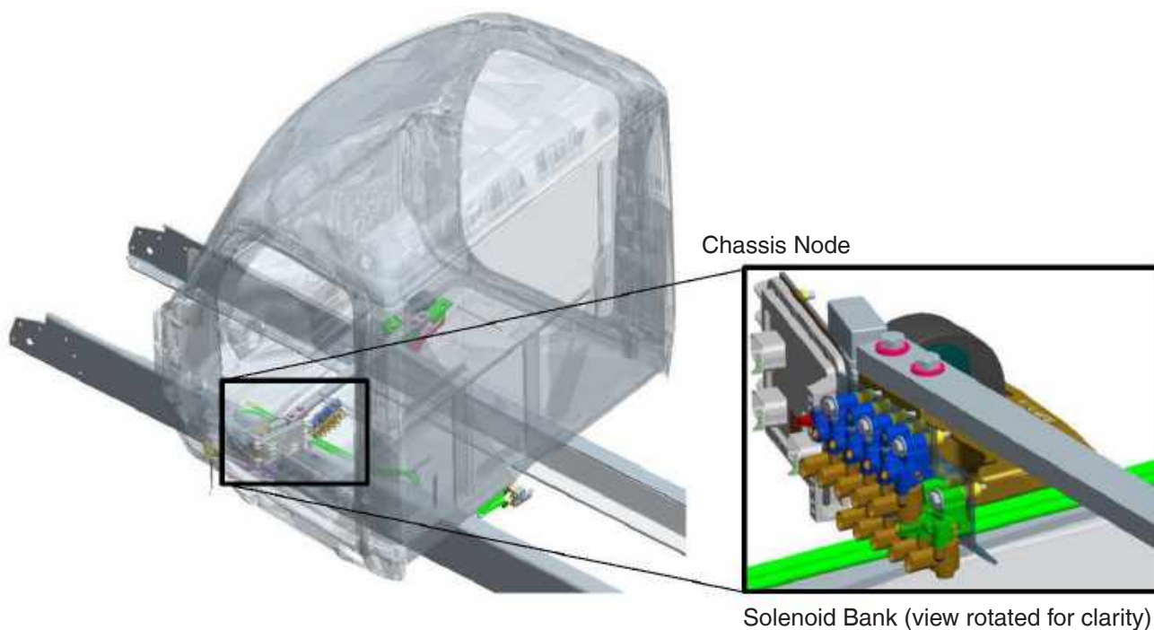
FIGURE 8-8. Air Solenoid Bank and Chassis Node
