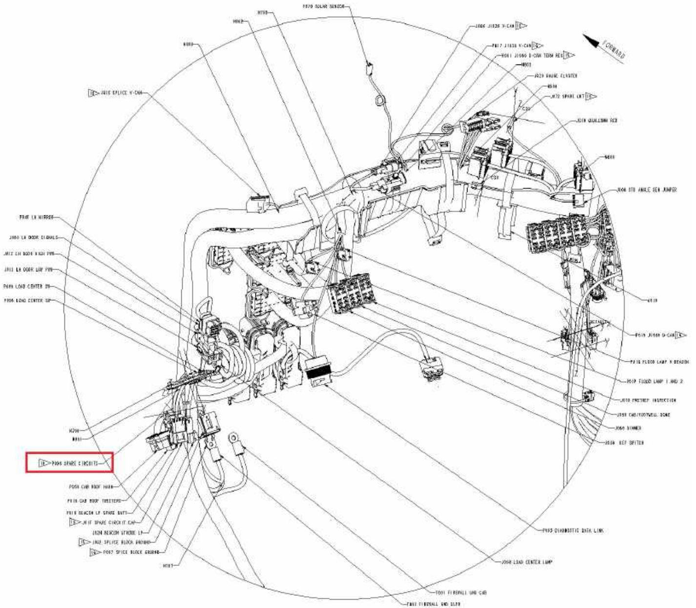
FIGURE 8-4. Spare circuit location under-dash (P096)
