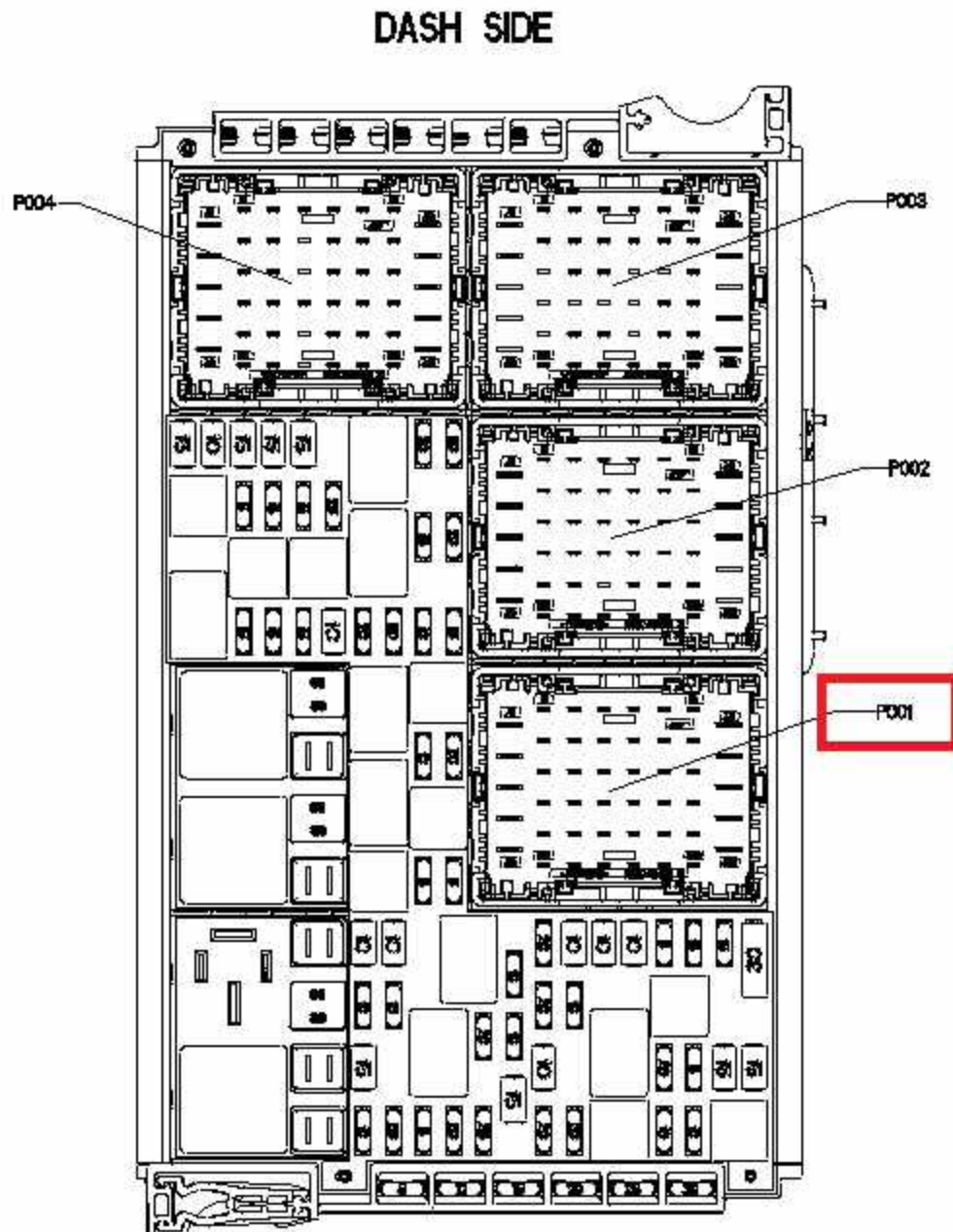
FIGURE 8-5. Spare circuit location on Power Distribution Center (Dash-Side, P001)
