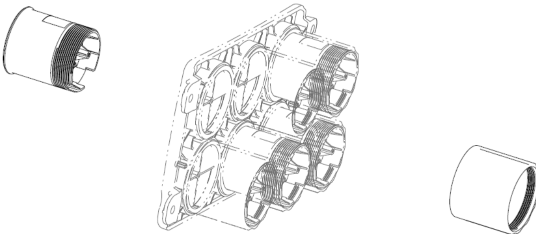
FIGURE 8-33. Gauge Installation
