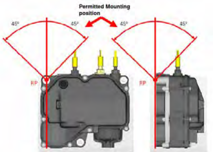
FIGURE 5-8: Supply Module Allowed Clocking Angles
