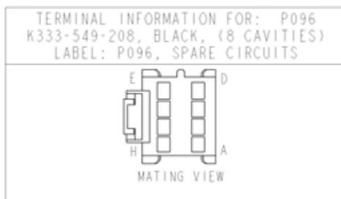
FIGURE 9-5. Spare circuit connector detail
