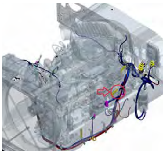
FIGURE 9-34. ISX12 Connection location.
