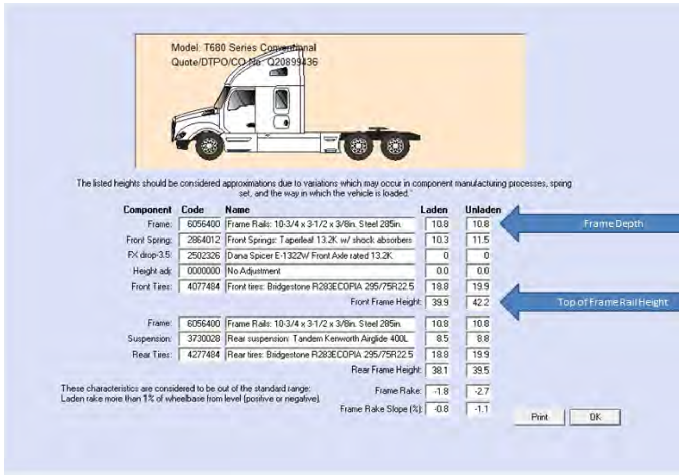
FIGURE 5-58. Dimension A = Top of Rail Frame Height from Prospector – Frame Depth.
