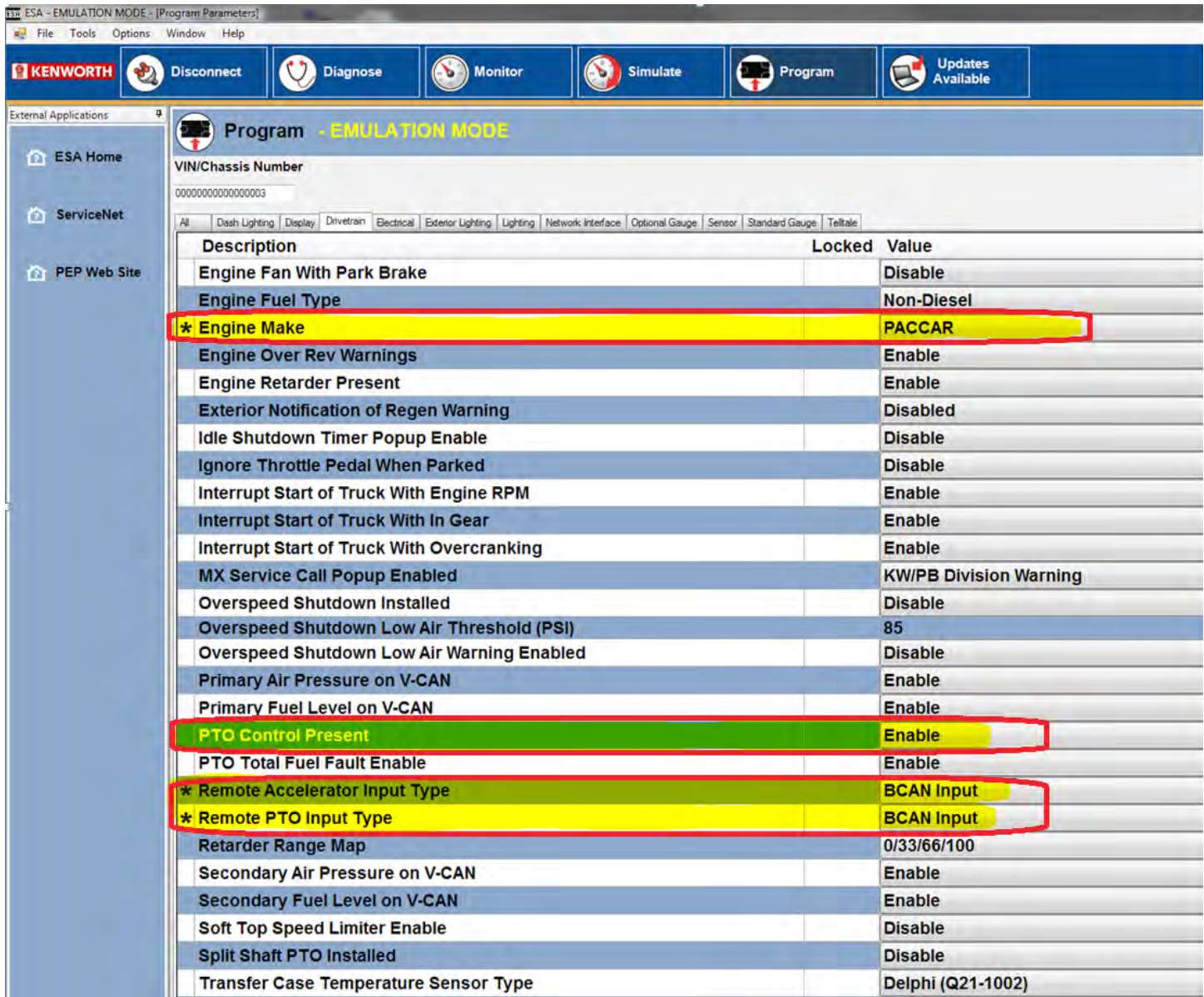
FIGURE 4-29. Remote PTO Control over BCAN with hardwired PTO Engagement Feedback to Engine– ESA Settings T680/T880
