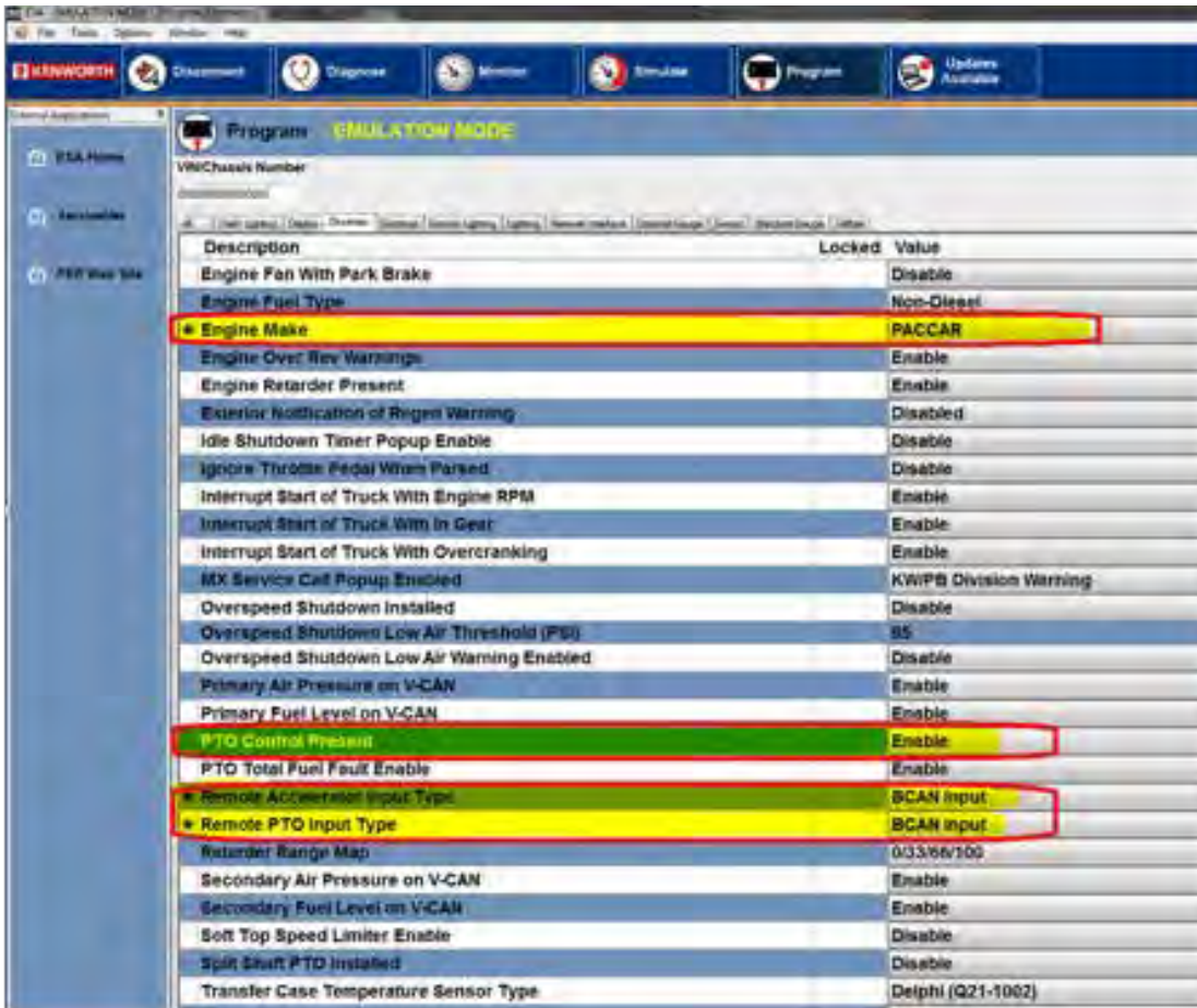
FIGURE 4-32. Remote PTO Control over BCAN with PTO ON/OFF Switch Signal over BCAN – ESA Settings for T680/T880
