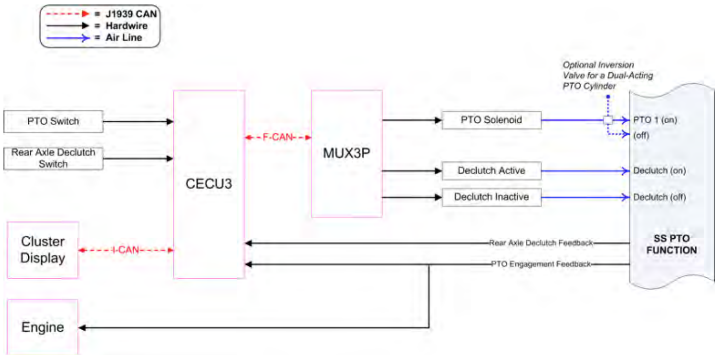
FIGURE 4-20. Split Shaft PTO Example #1
