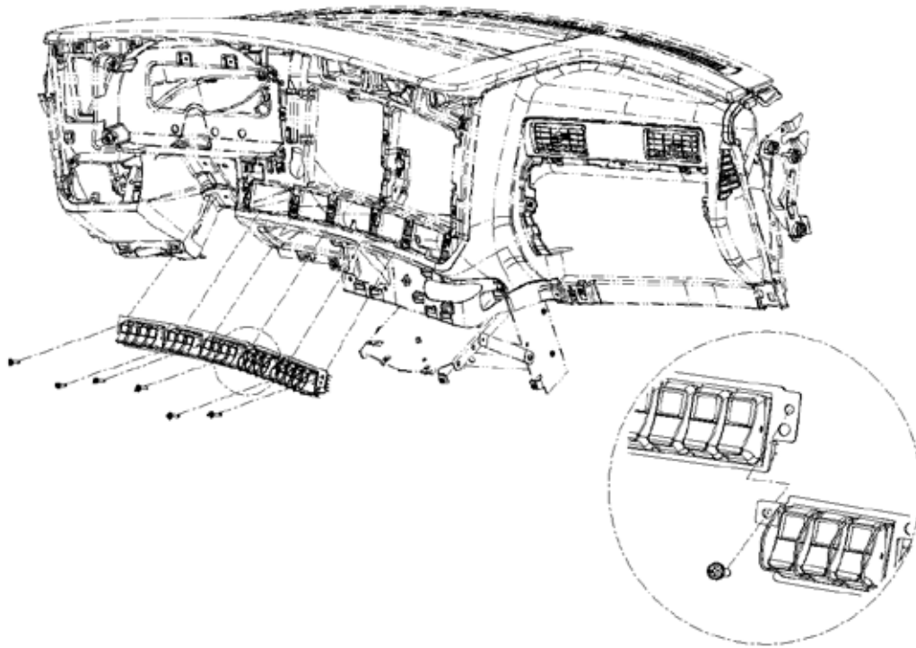
FIGURE 9-44. Switch Installation
