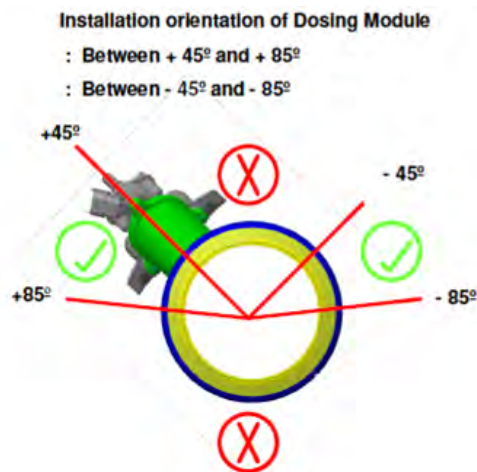
FIGURE 5-3: Orientation of Dosing Module
