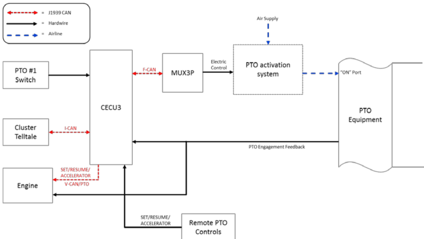
FIGURE 4-25. Hard-Wired Remote PTO Control
