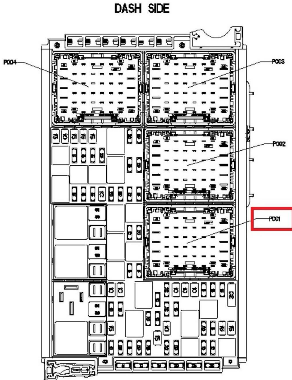
FIGURE 10-36. Spare Circuit Location on PDC (Dash-Side)
