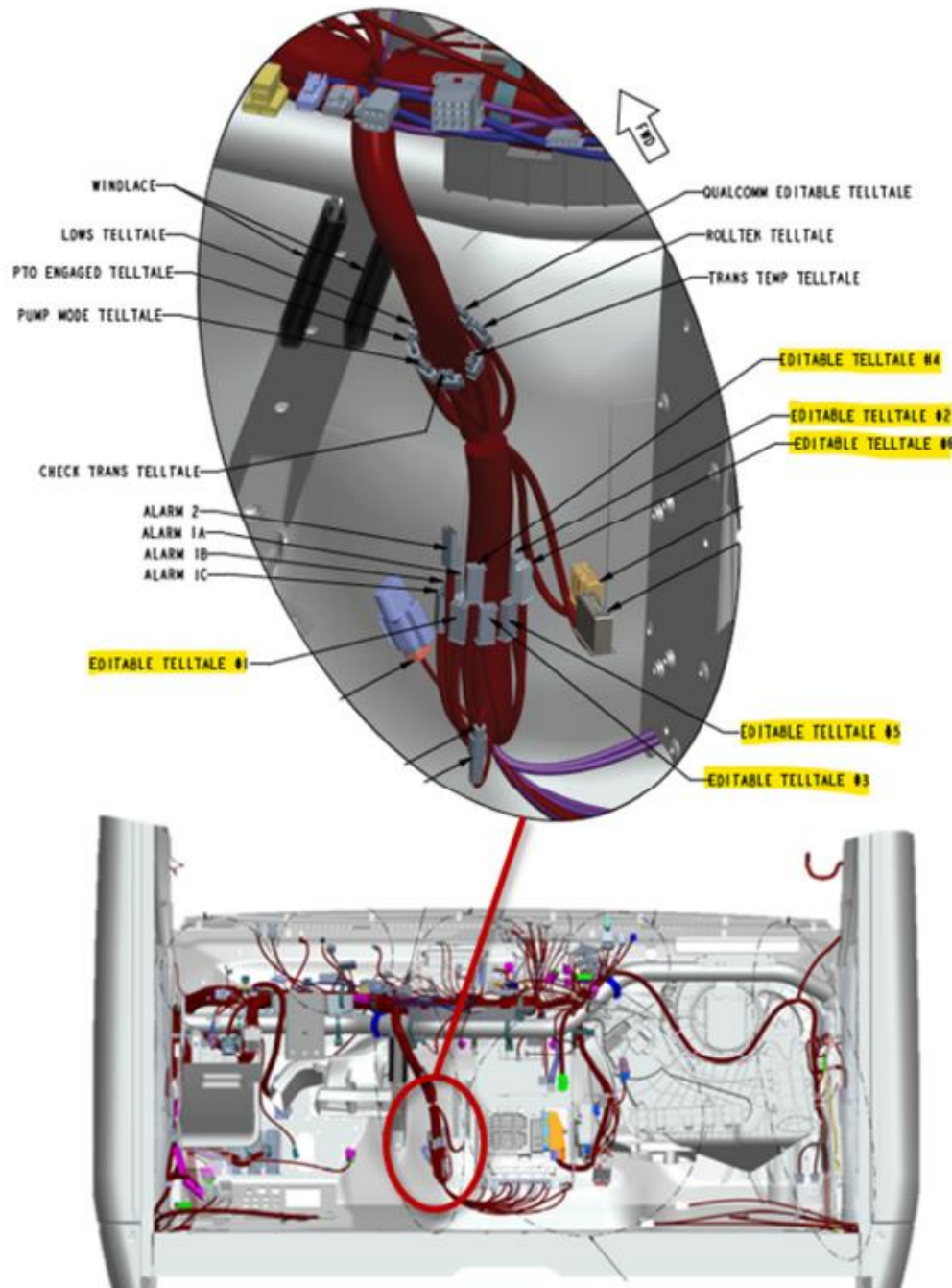
FIGURE 10-43. Telltale Connector Locations
