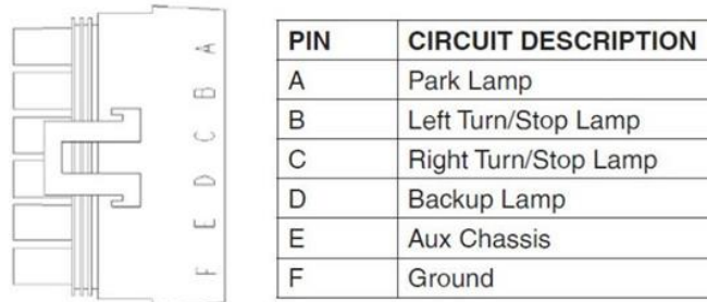
FIGURE 10-39. Mating Connector: Packard PN 12020789
