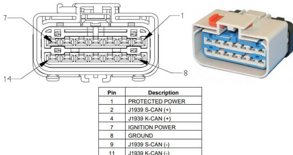
FIGURE 10-5. RP1226 Pinout
