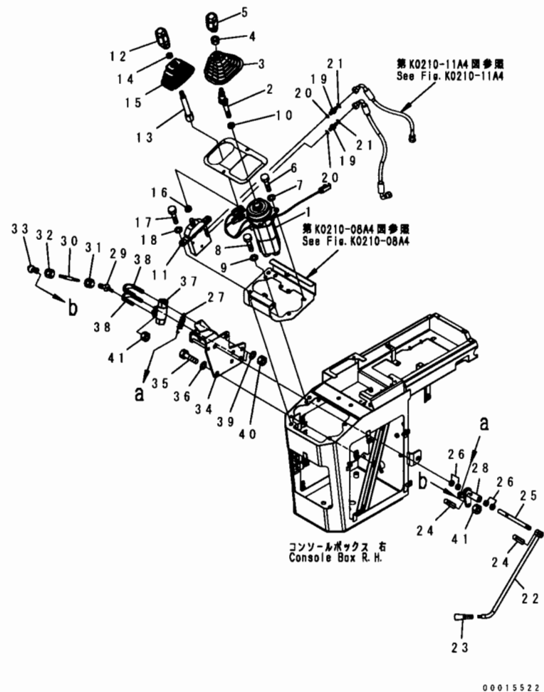
FIG. K0210-10A4 FLOOR (LOADER CONTROL) (1/2) (P.P.C VALVE AND LEVER) (FOR MONO + 1-ATTACHMENT LEVER)
