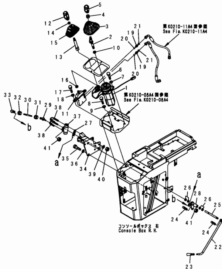
FIG. K0210-10A4 FLOOR (LOADER CONTROL) (1/2) (P.P.C VALVE AND LEVER) (FOR MONO + 1-ATTACHMENT LEVER)
