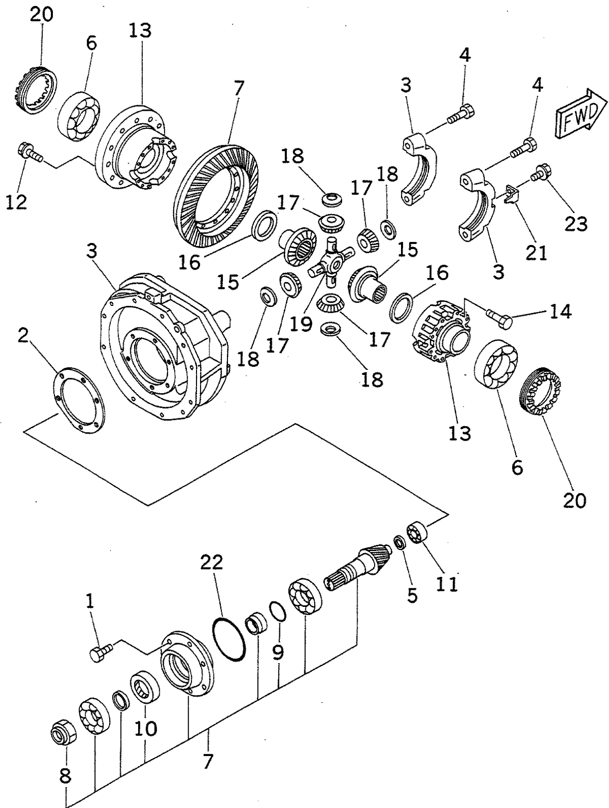
FIG.F4160-28A0 TORQUE FLOW TRANSMISSION (WITH TORQUE CONVERTER) (8/8)
