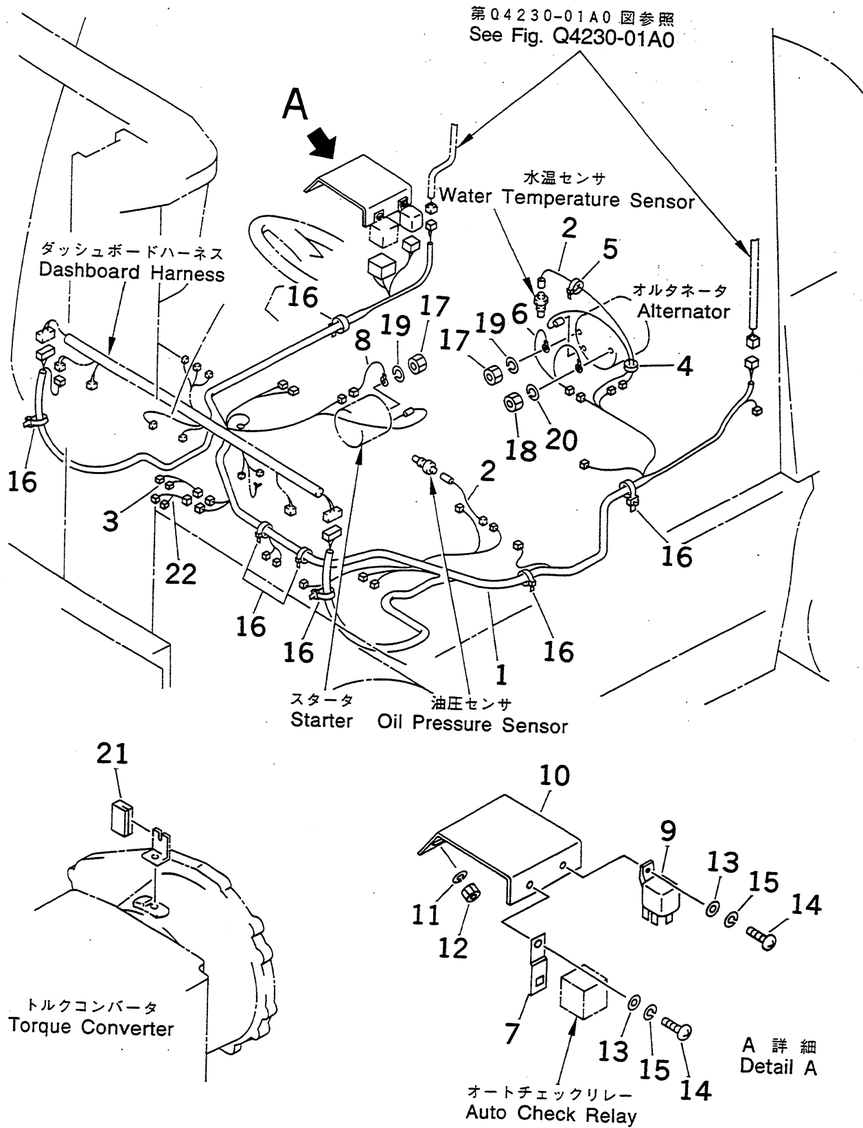
FIG.Q4210-01A0 ELECTRICAL SYSTEM (ENGINE WIRING) (CLUTCH SPEC.)
