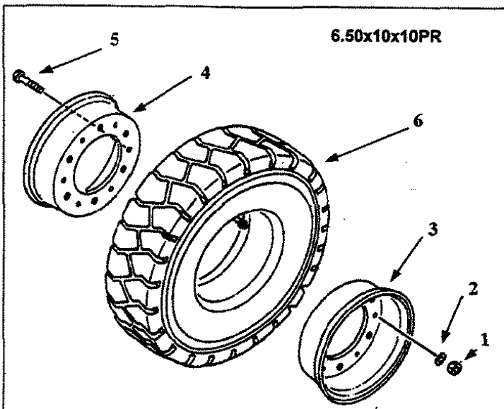
Drive Tire FG15H-16, FG18H-16
