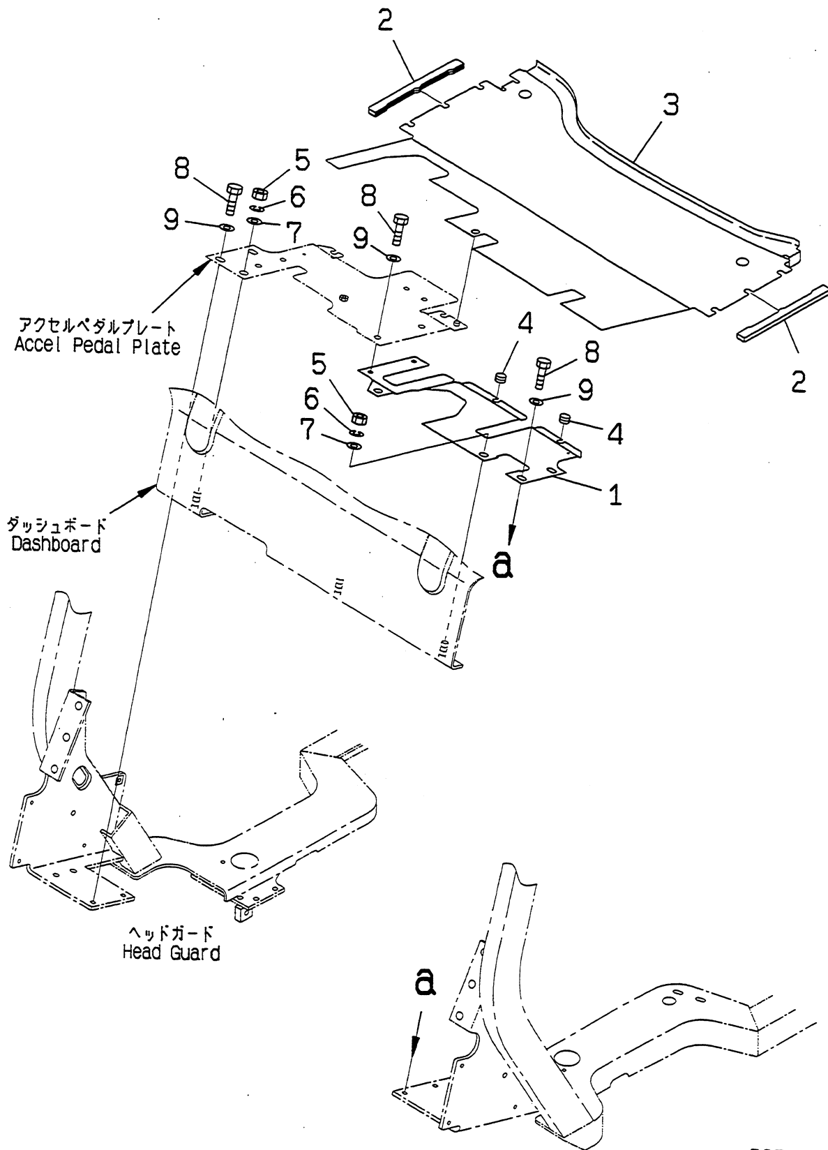
FIG.P4160-01A0 FLOOR PLATE (CLUTCH SPEC.)
