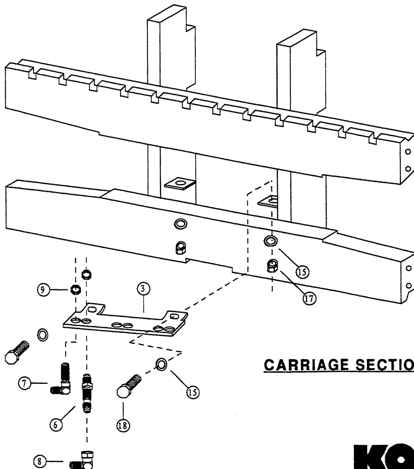
CROSSHEAD SECTION
