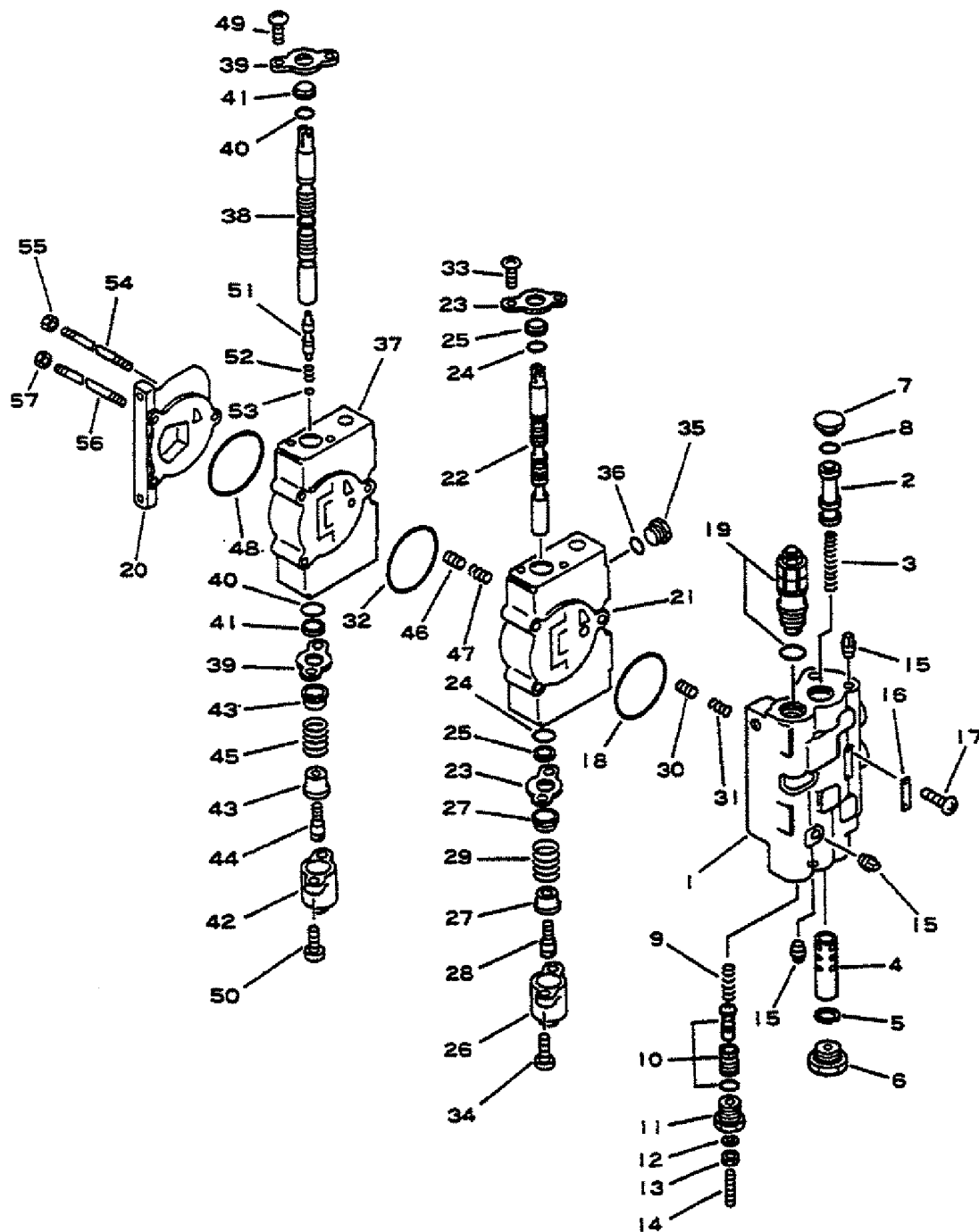
FIG. R4360-01A0 2-SP00L CONTROL VALVE
