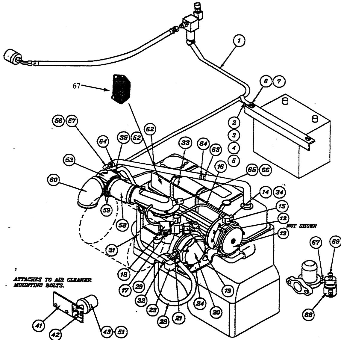
KOMATSU AX SERIES - DUAL FUEL SYSTEM
