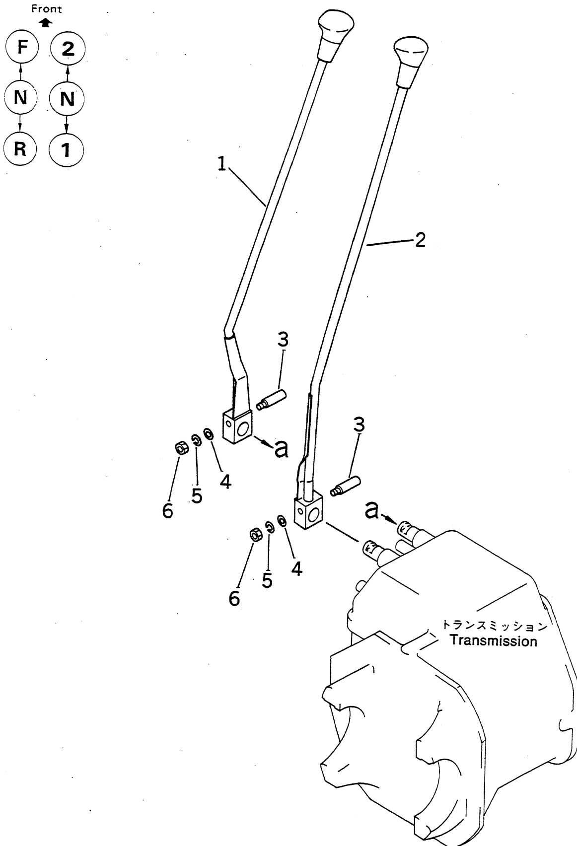
FIG.L4140-01A0 TRANSMISSION SHIFT LEVER (CLUTCH SPEC.)
