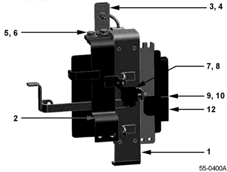
ECM - K21/K25
