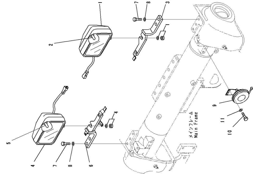
FIG. E0300-001001 Front Working Lamp
