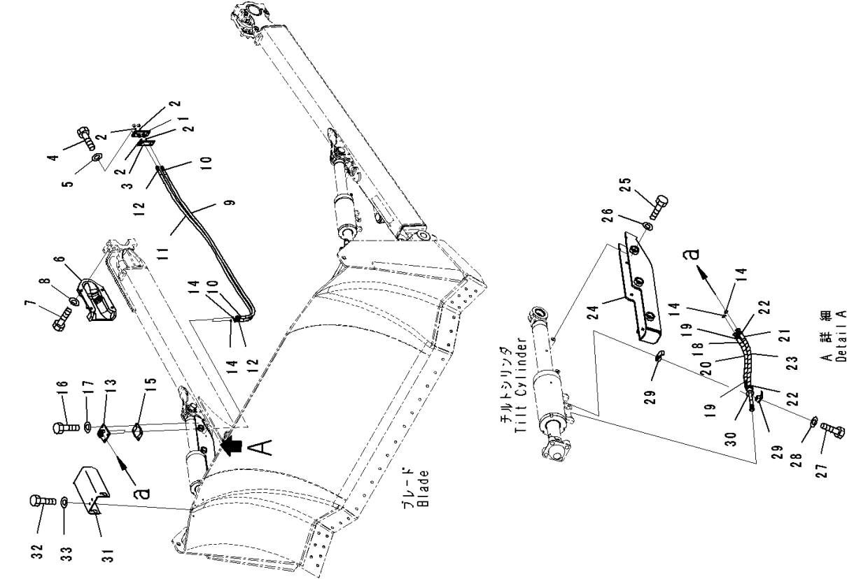
FIG. T2160-001001 Dozer Blade Tilt Cylinder Piping
