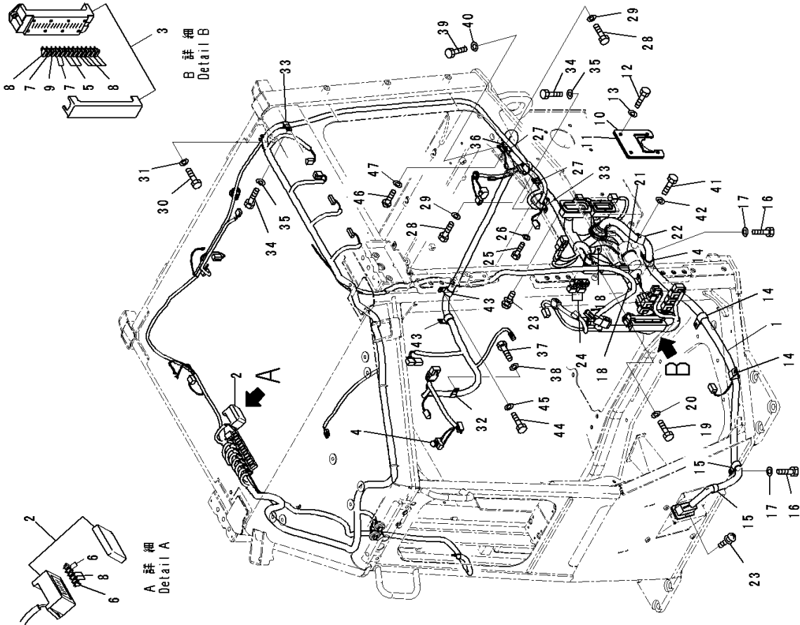
FIG. K0210-012040 ROPS Cab, Floor, Harness (1/3)
