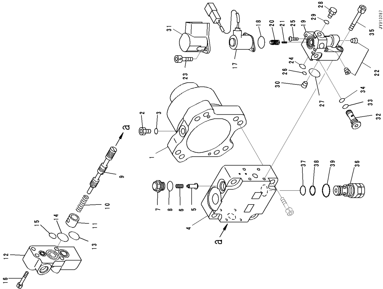
FIG. C0100-001005 Radiator, Cooling Fan Motor (1/2)
