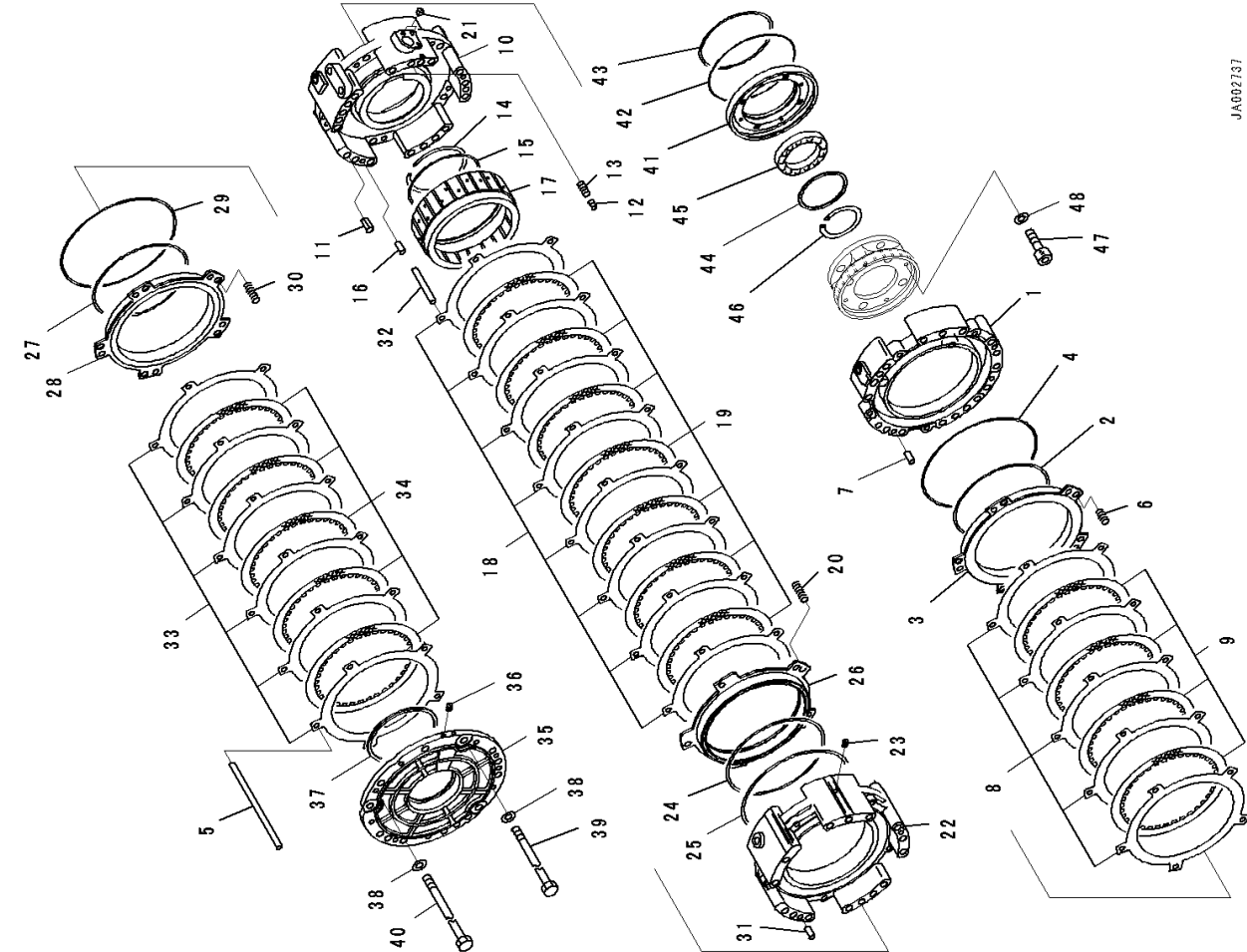
FIG. F2300-001011 Power Train, 2nd, 3rd, Forward and Reverse Housing
