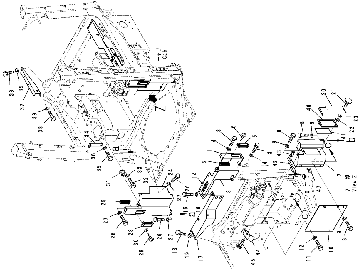
FIG. K0210-007048 ROPS Cab, Floor Cover
