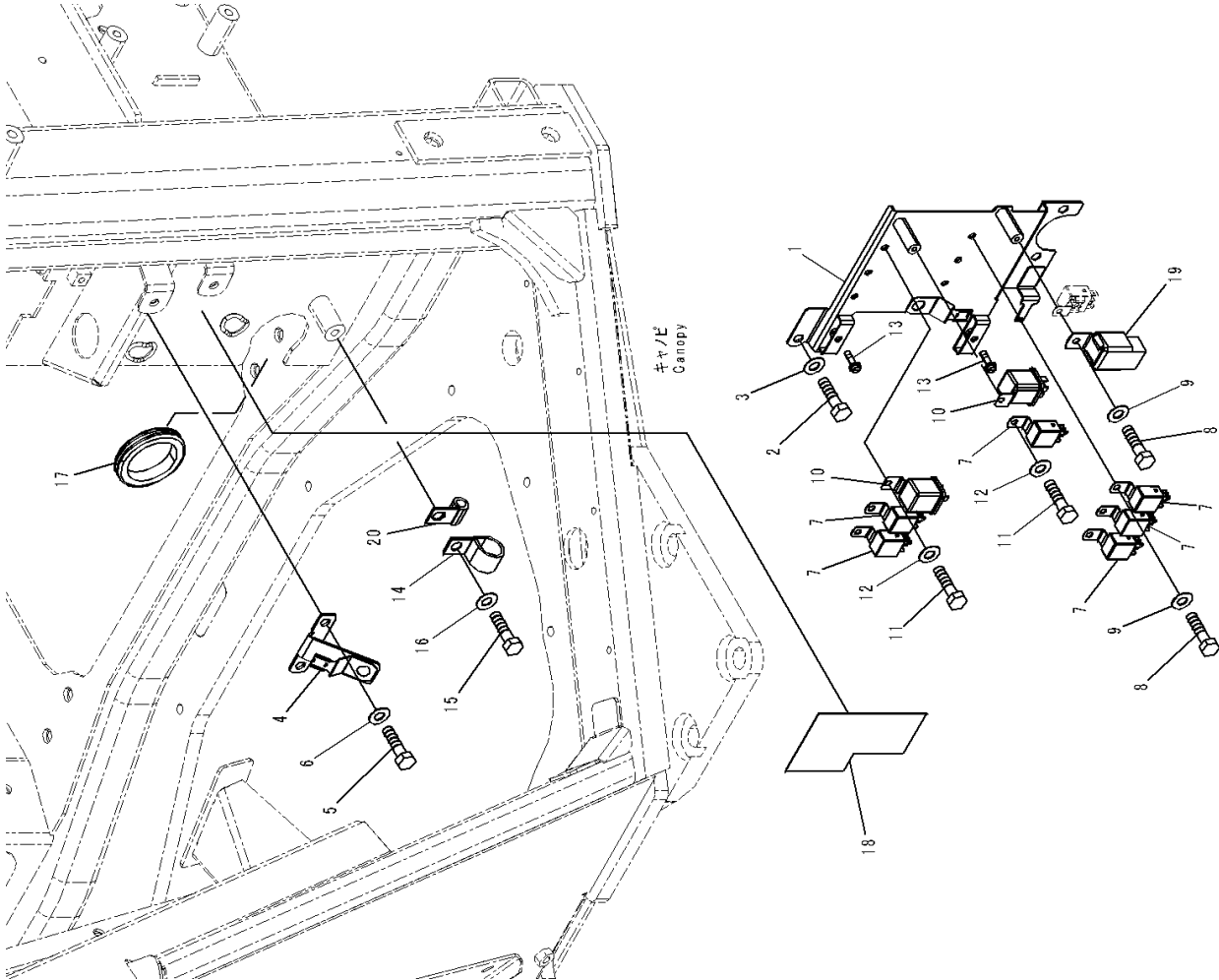
FIG. K0410-002017 ROPS Canopy, Floor, Harness (3/3)
