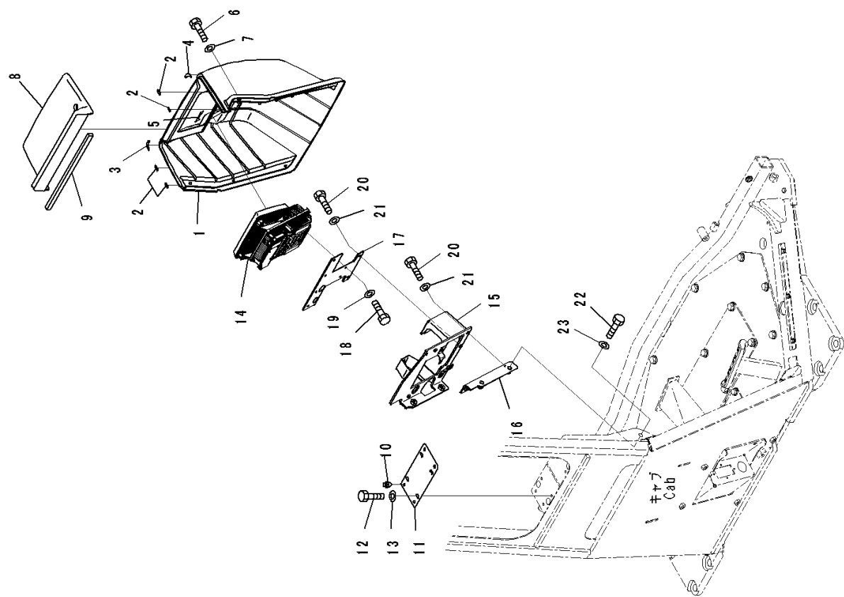
FIG. K0210-007044 ROPS Cab, Dashboard Cover (1/2)
