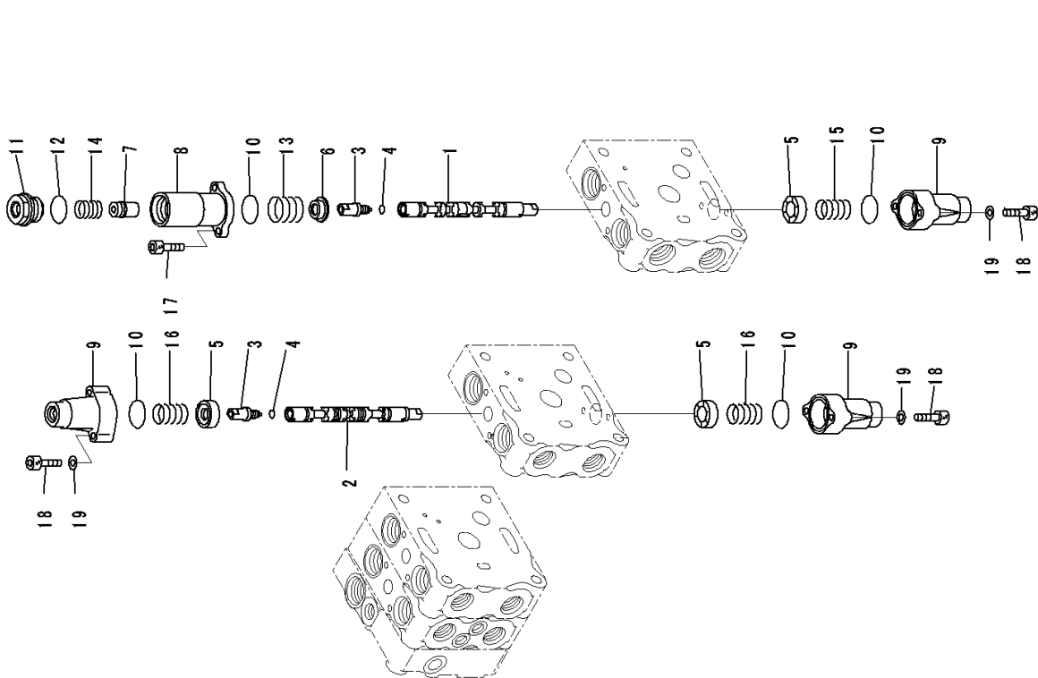
FIG. M2210-005003 Fender Group, Inner Parts (2/12)
