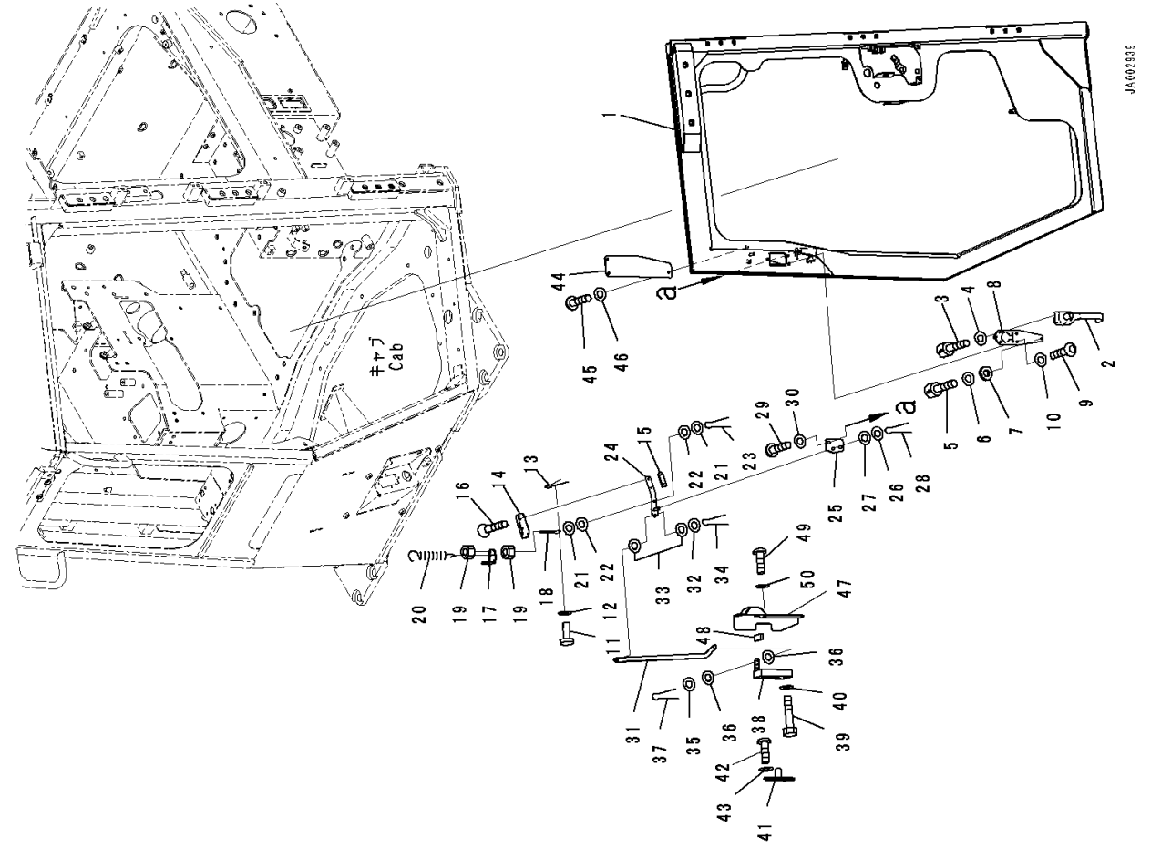
FIG. K0210-002002 ROPS Cab, Door and Latch, LHS
