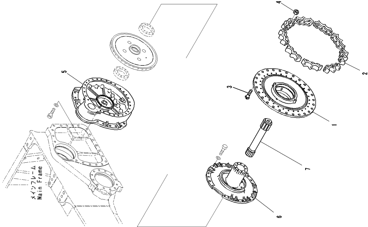
FIG. F2380-003003 Final Drive, Sprocket Hub, LHS
