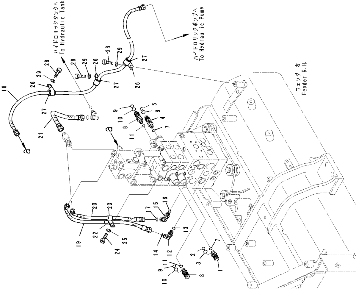
FIG. M2210-001015 Fender Group, For Machine With 3-spool Valve Hydraulics, Control Valve Steering Piping
