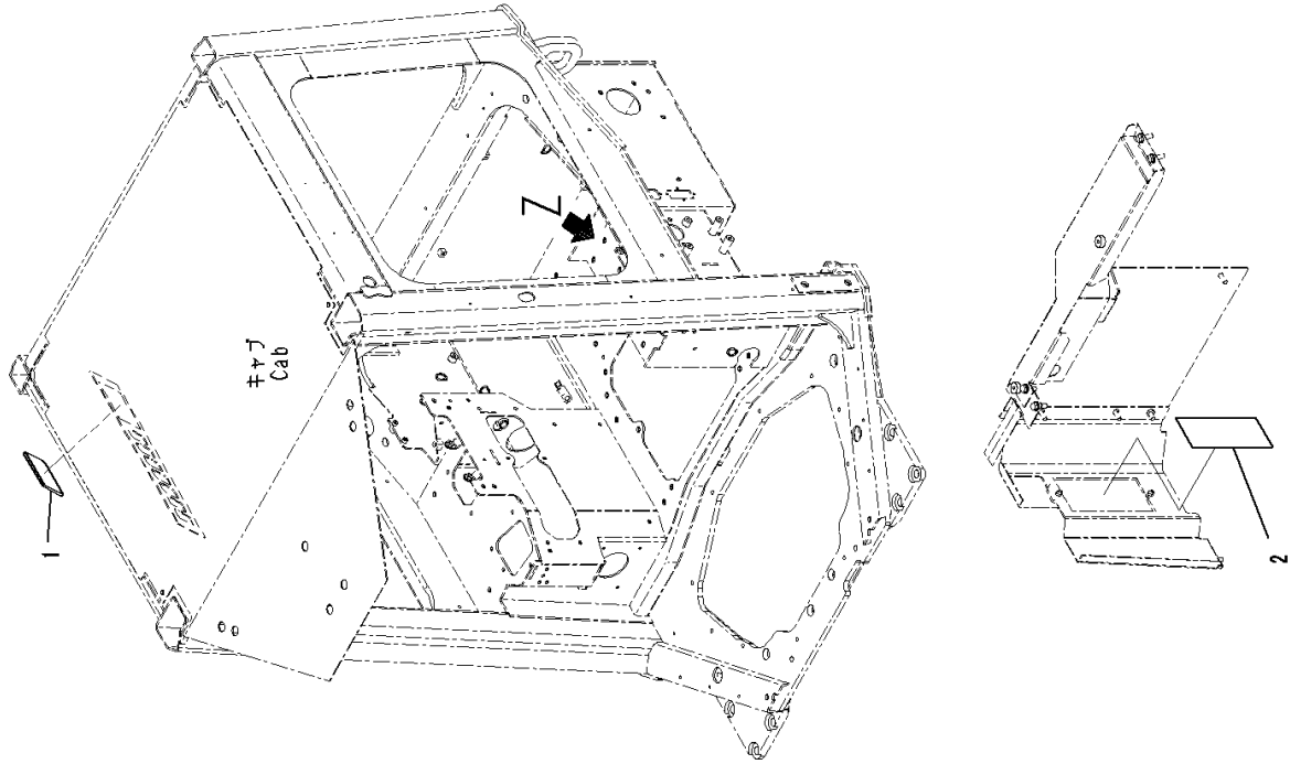
FIG. K0210-002050 ROPS Cab, Decal
