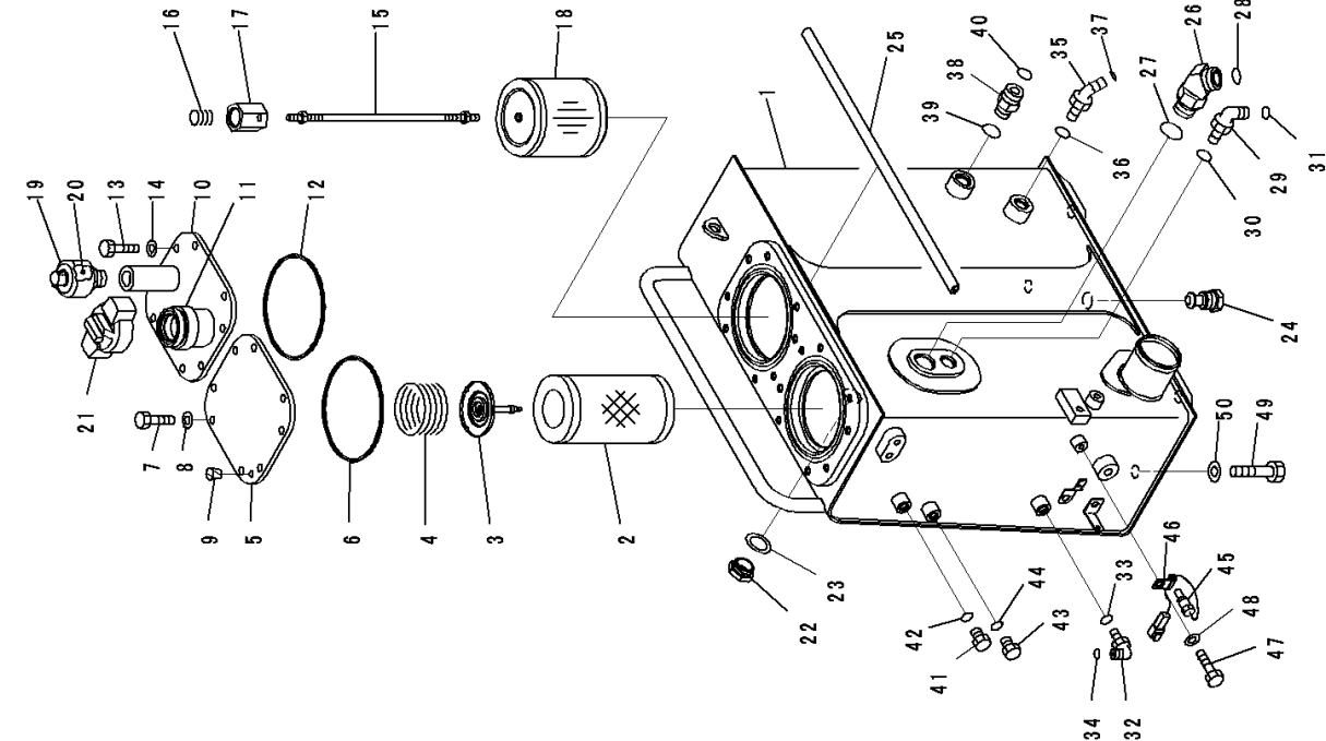
FIG. H0110-001001 Hydraulic Oil Tank
