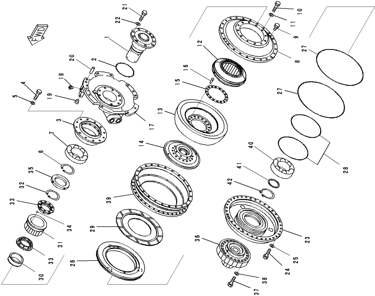
FIG. F2300-001021 Power Train, Pump and Turbine
