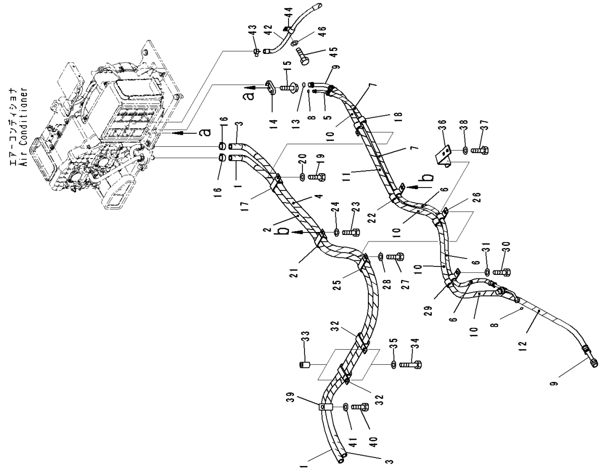
FIG. K0210-007027 ROPS Cab, Air Conditioner Piping
