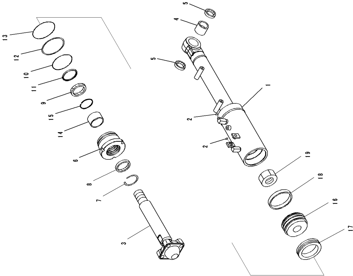
FIG. T2150-001001 Dozer Blade Tilt Cylinder, Inner Parts
