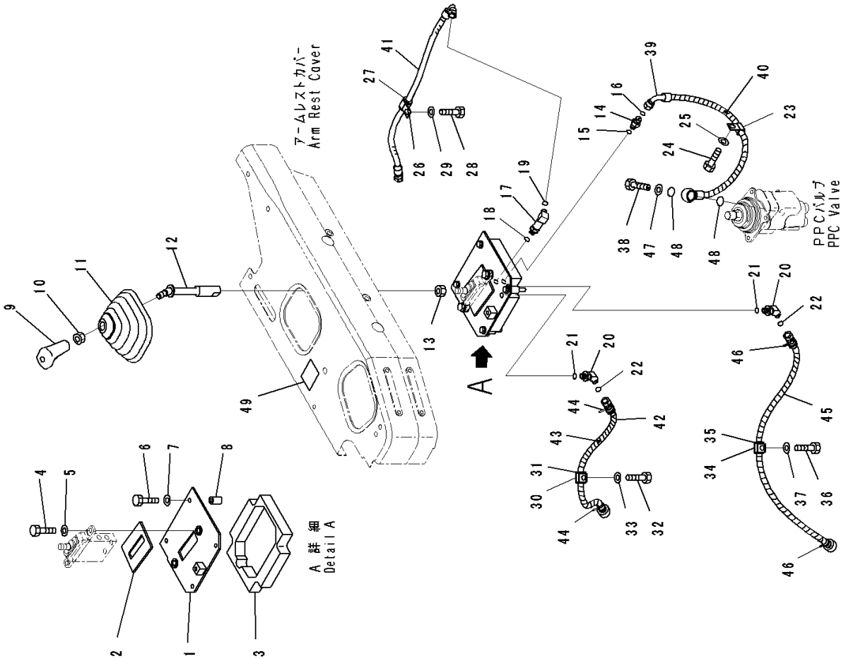
Dozer Control, With Power Angle Power Tilt Dozer, For Machine With Rear Actuator, ROPS Canopy, Attachment Lever
