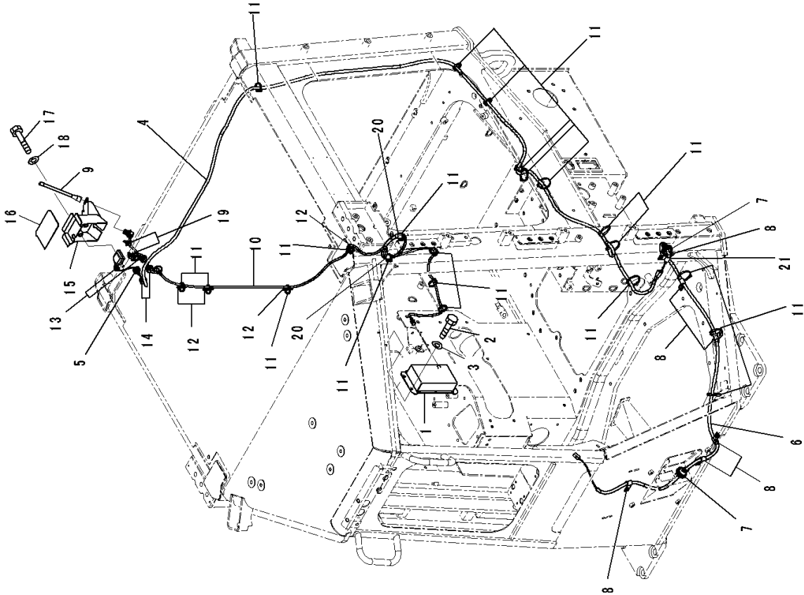
FIG. K0210-002049 ROPS Cab, KOMTRAX Controller
