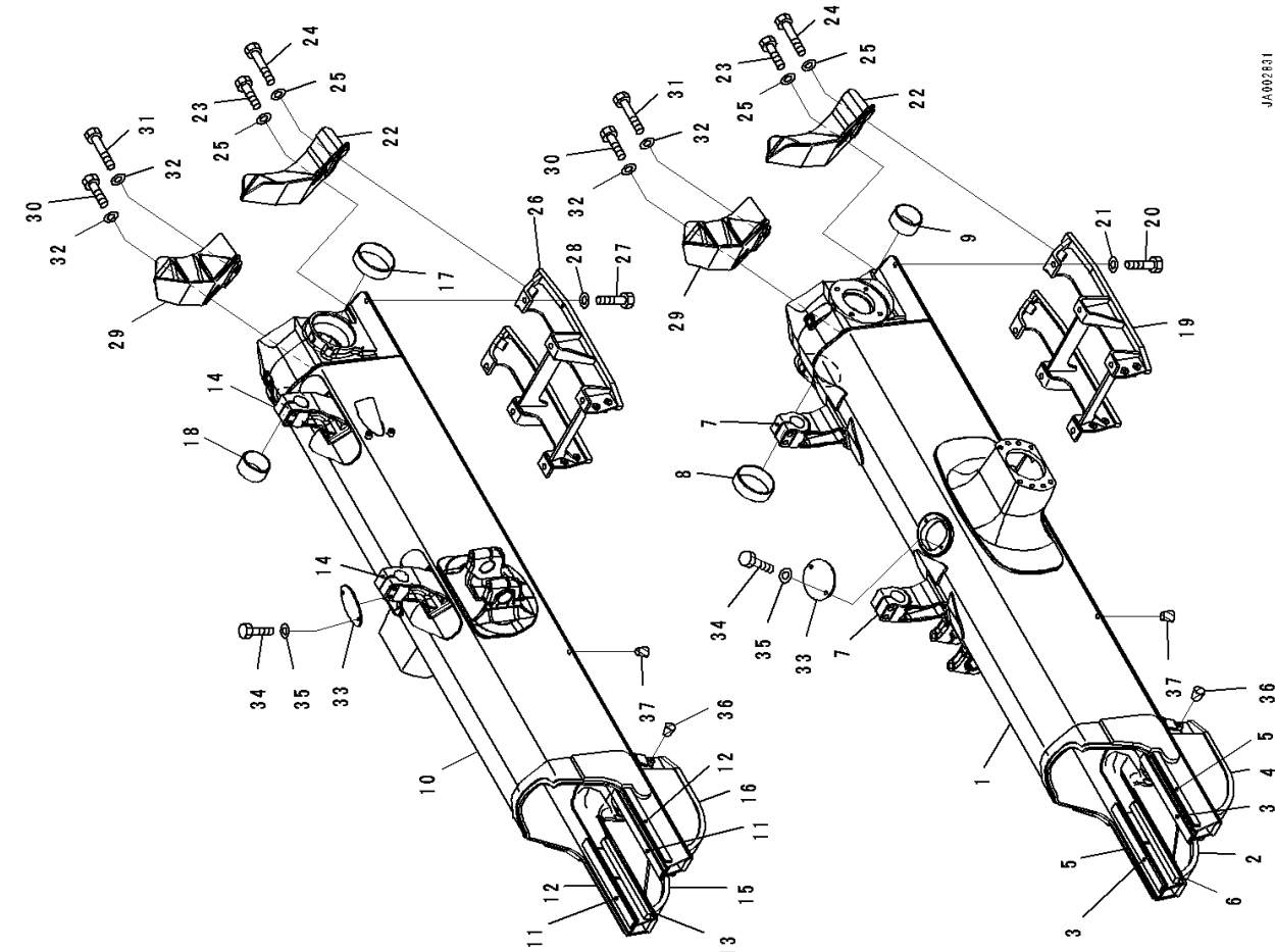
FIG. R2100-001001 Track Frame
