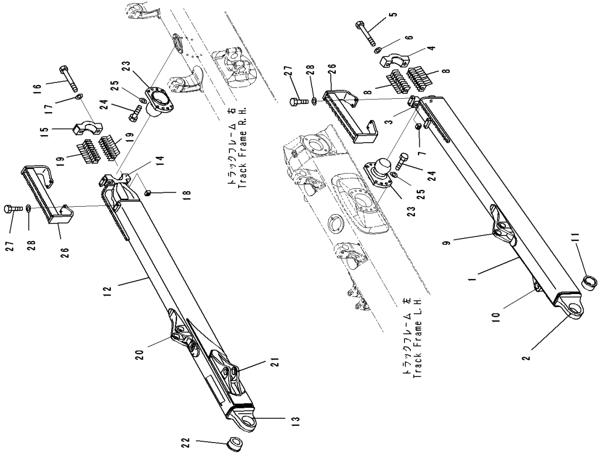
FIG. T21110-001001 Dozer Frame
