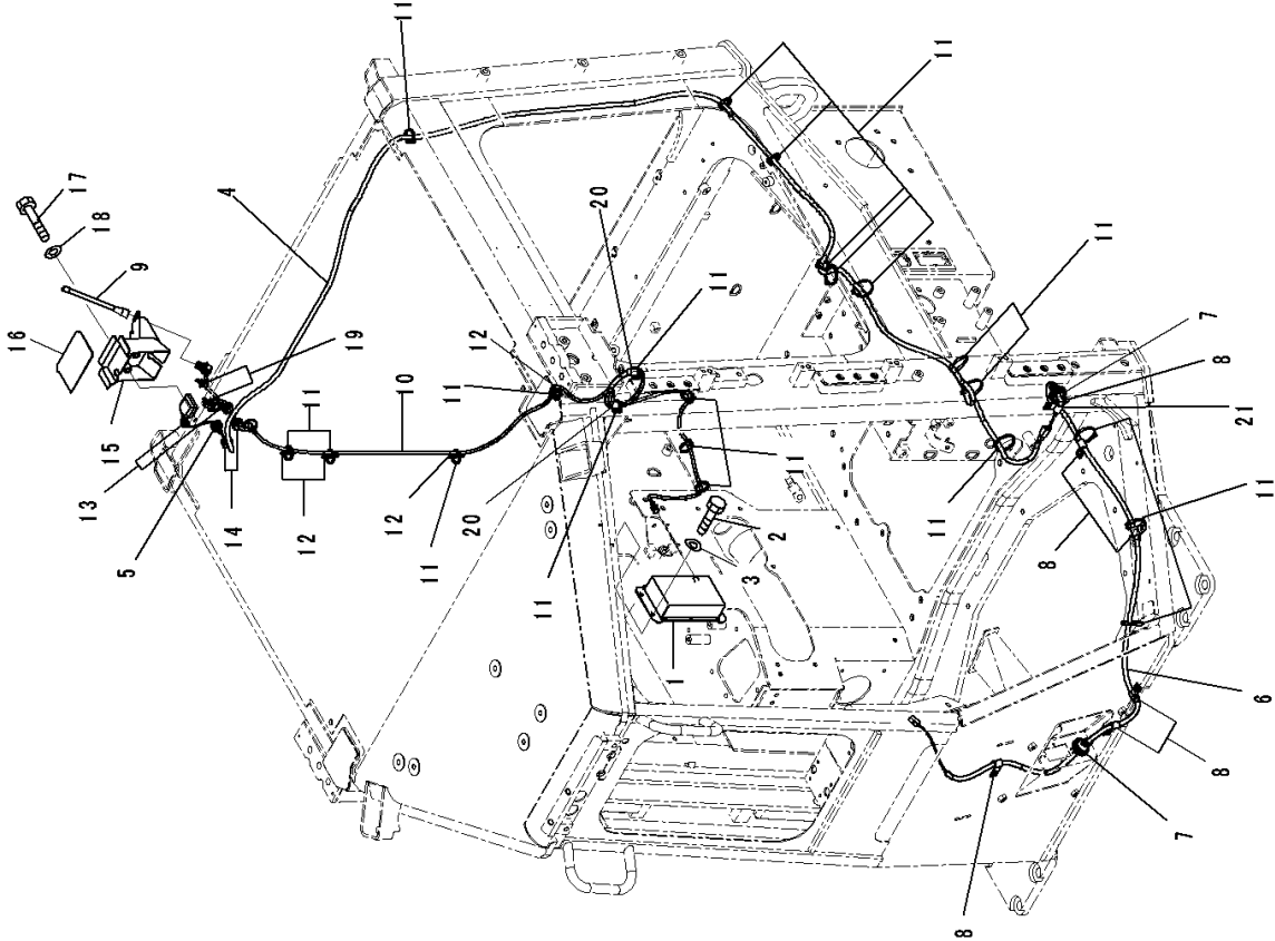
FIG. K0210-007049 ROPS Cab, KOMTRAX Controller
