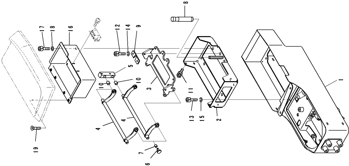
FIG. K0210-007030 ROPS Cab, Console Box
