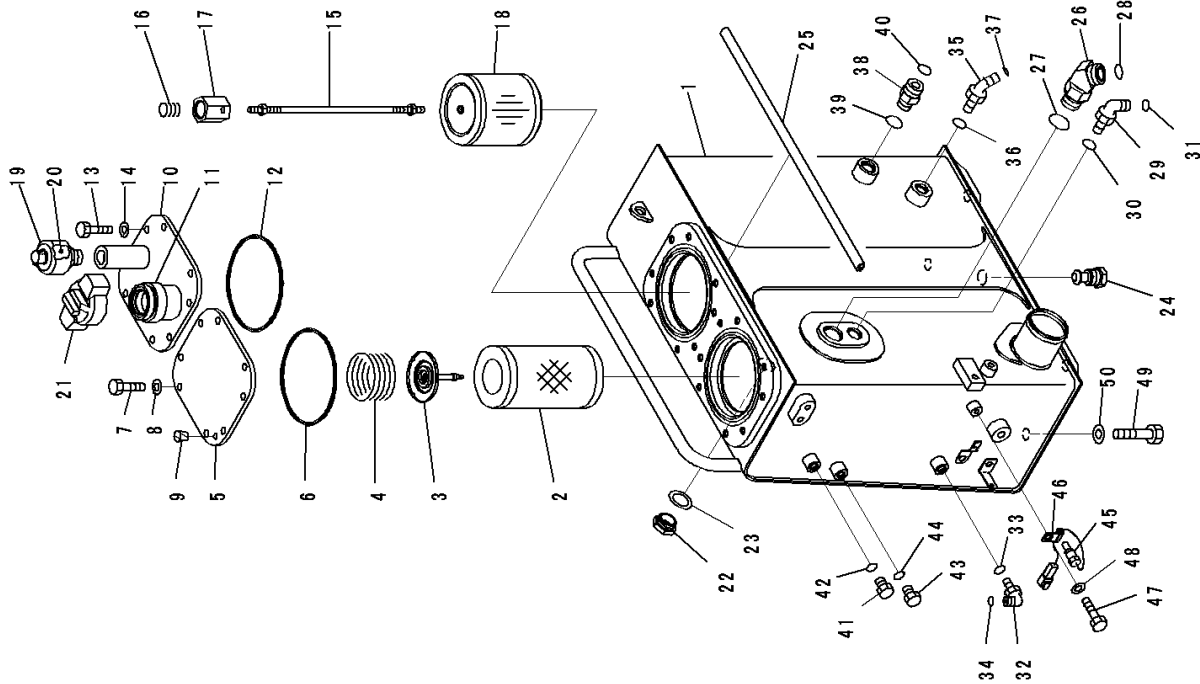
FIG. H0110-001001 Hydraulic Oil Tank
