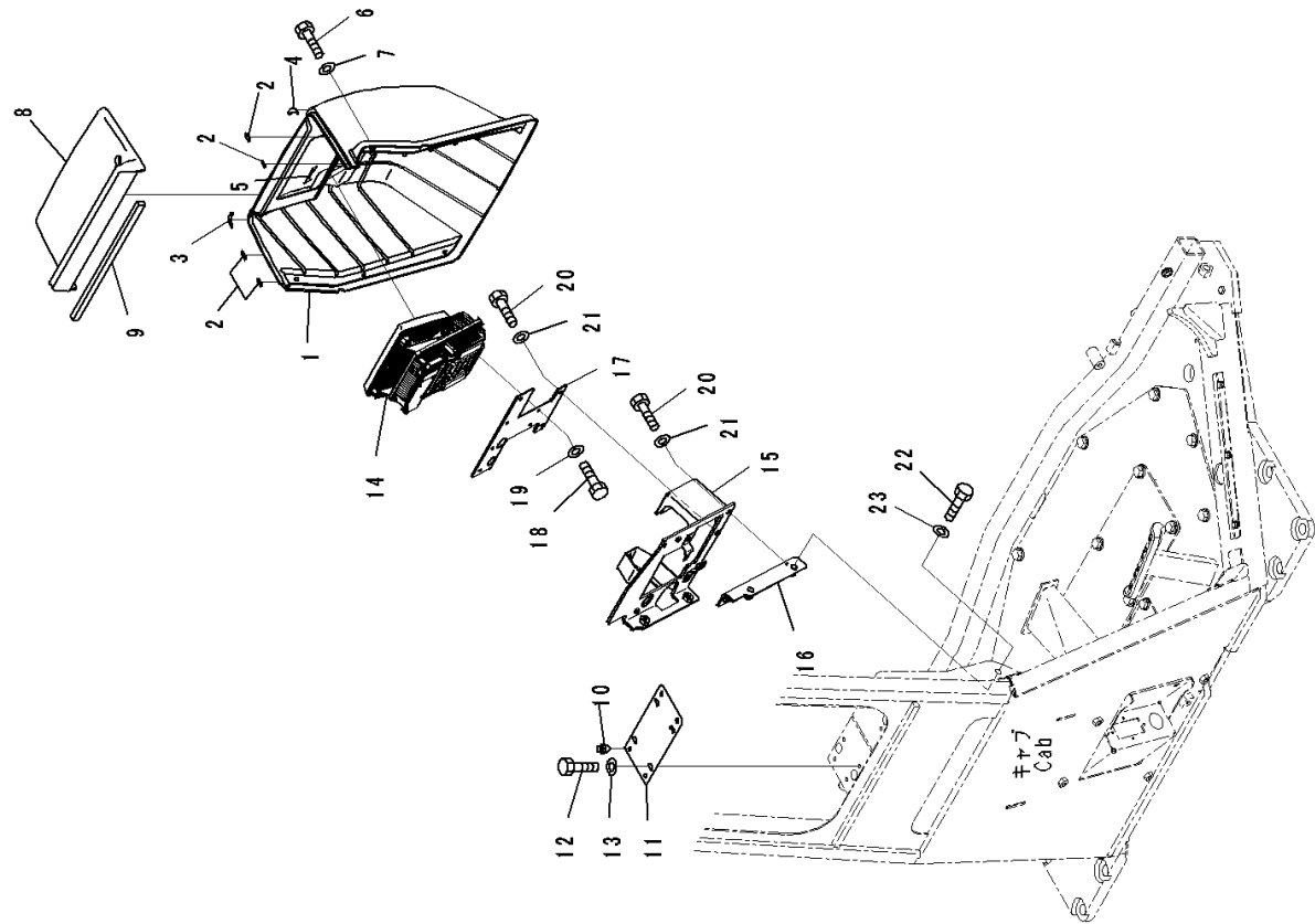
FIG. K0210-012044 ROPS Cab, Dashboard Cover (1/2)
