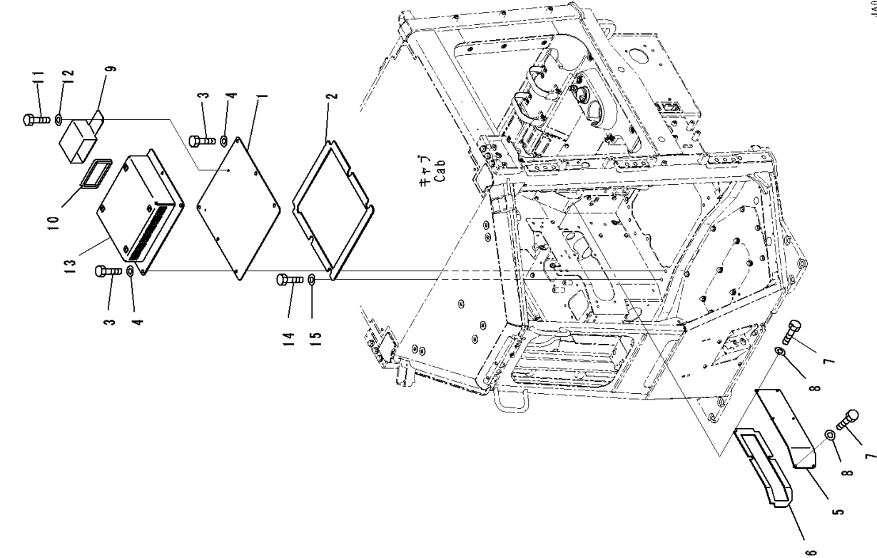
FIG. K2130-002001 Floor Frame Cover
