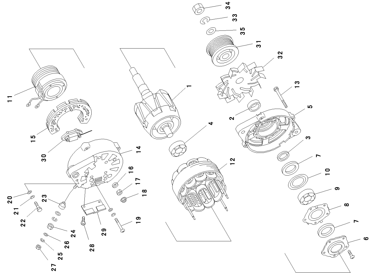
FIG. AEE00-002001 Alternator, 90Amp.
