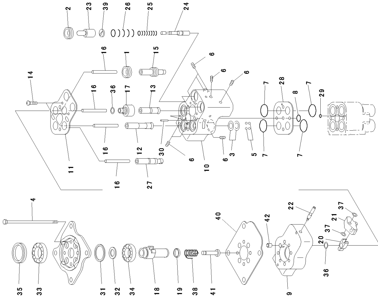
FIG. K2110-005004 Dozer Control, PPC Valve for PAT (2/2)
