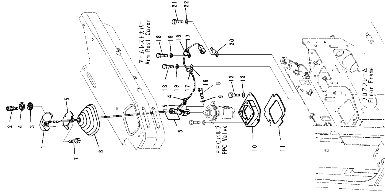
FIG. K2110-004002 Dozer Control, Lever
