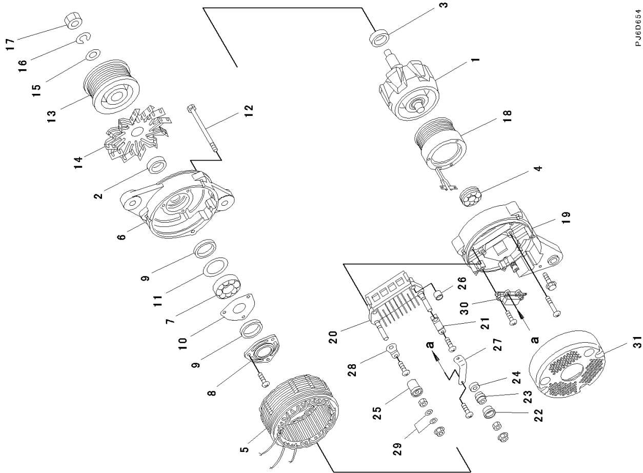
FIG. AEE00-001001 Alternator, 60Amp.
