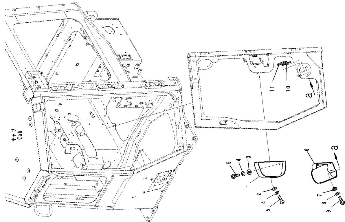
FIG. K0210-002004 ROPS Cab, Door Cover, LHS
