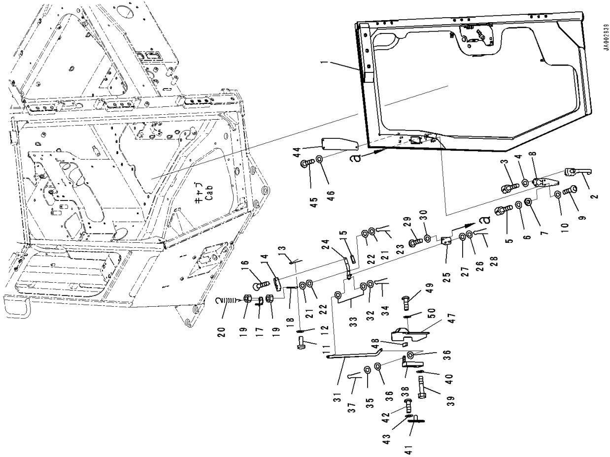
FIG. K0210-007002 ROPS Cab, Door and Latch, LHS
