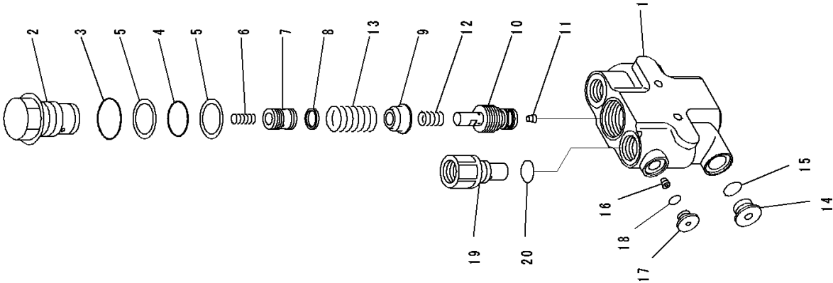
FIG. H2210-003002 Dozer Blade Lift Piping, Valve
