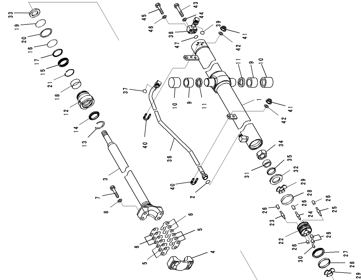
FIG. T2140-001001 Dozer Blade Lift Cylinder, Inner Parts, LHS
