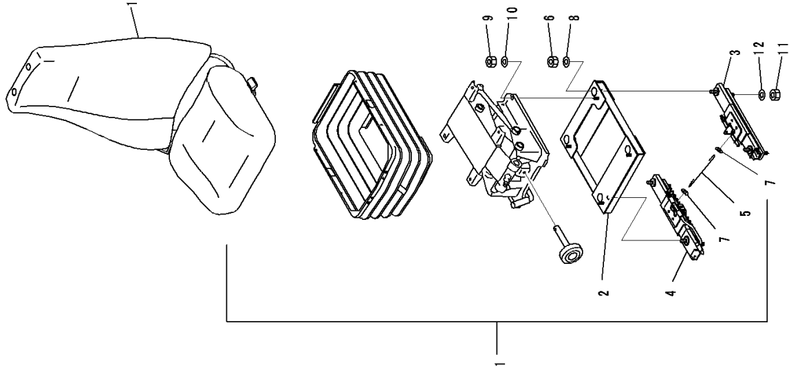
FIG. K0110-010001 Operator's Seat, Suspension Type, Hi-Back Type Operator's Seat, Fabric Type, Turn And Reclining Type
