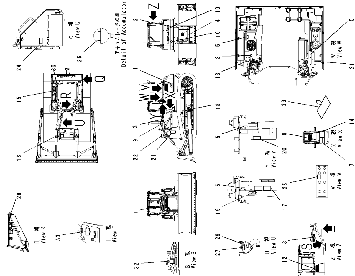
FIG. U0100-012001 Marks And Plates, Germany
