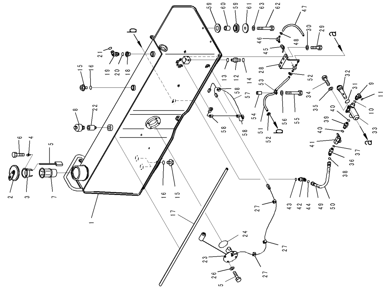
FIG. D0100-002001 Fuel Tank, With Refuel Pump
