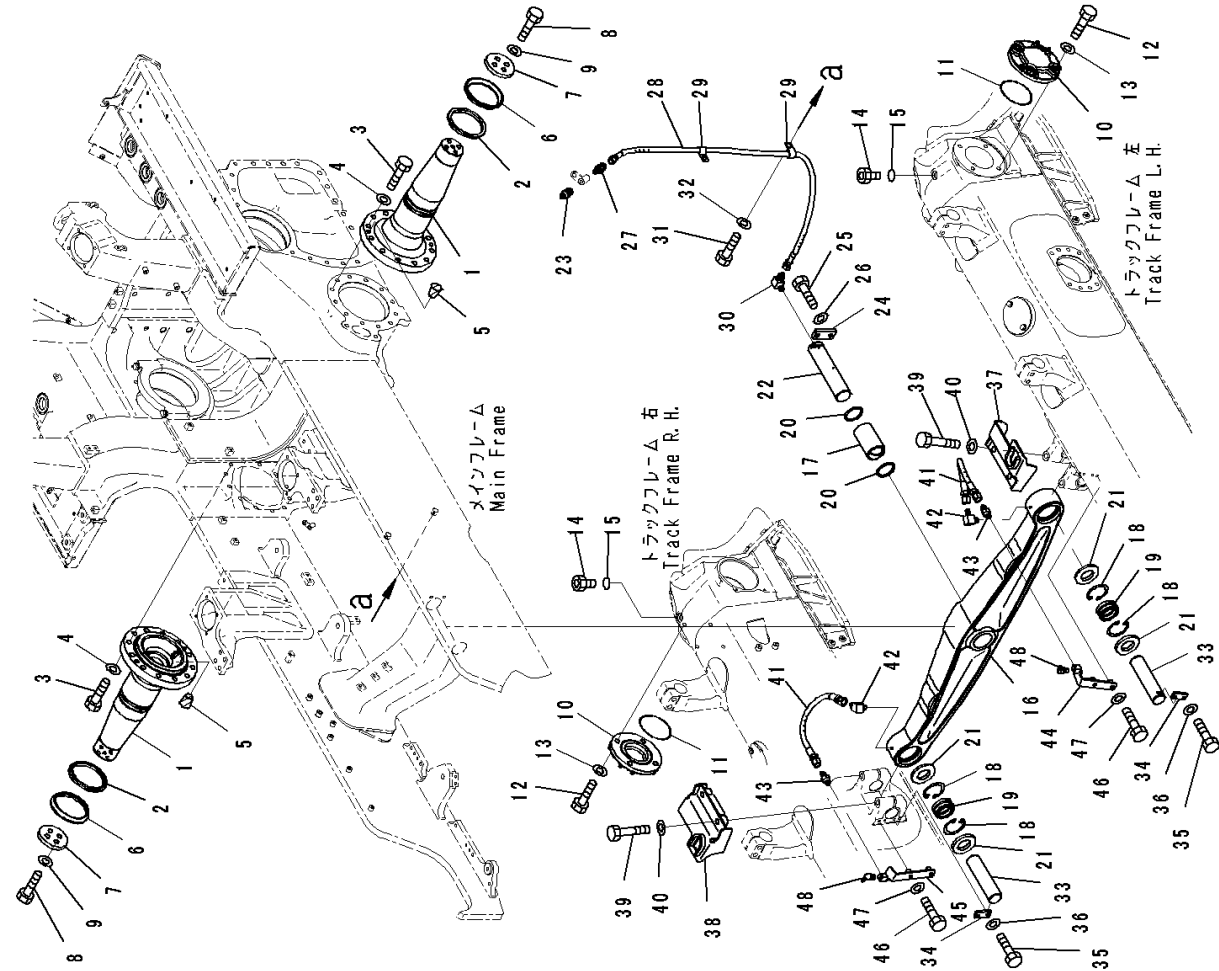
FIG. J2700-002001 Equalizer Bar And Pivot Shaft
