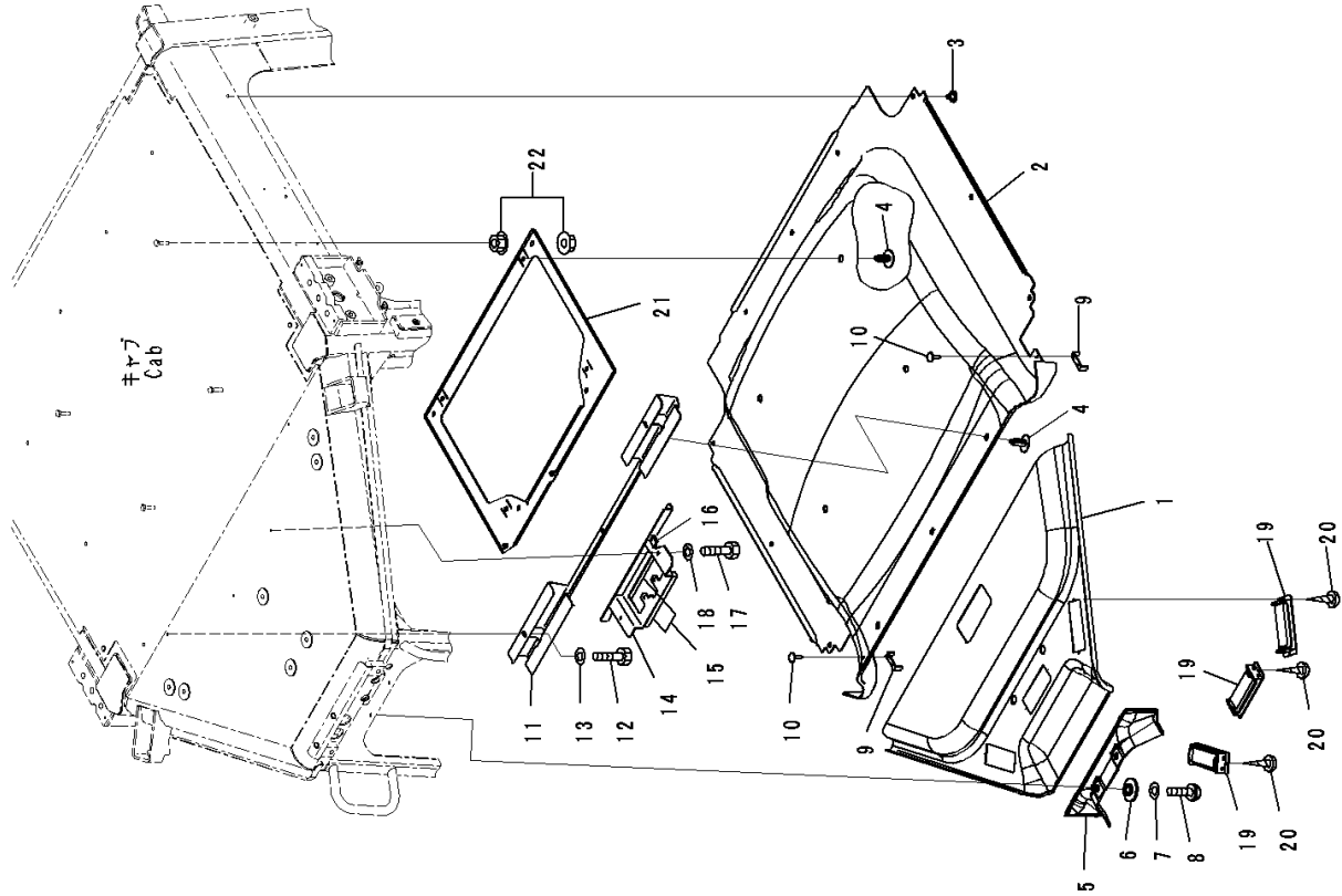
FIG. K0210-007020 ROPS Cab, Roof Cover (1/2)
