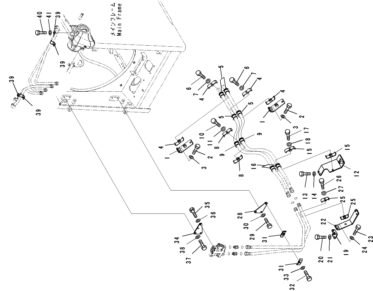
FIG. H2210-003004 Dozer Blade Lift Piping, Clamp
