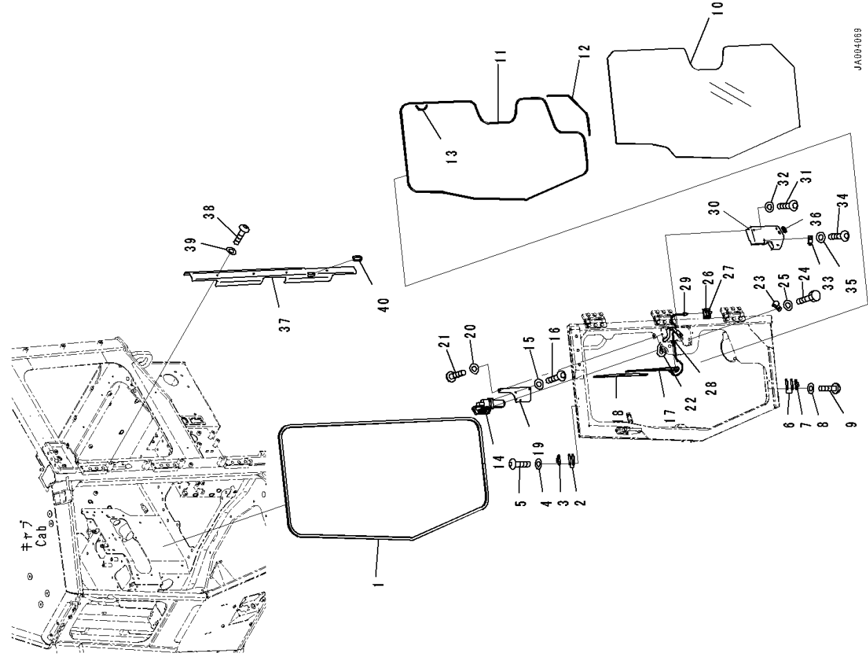
FIG. K0210-002003 ROPS Cab, Door Dumper, Window and Wiper LHS
