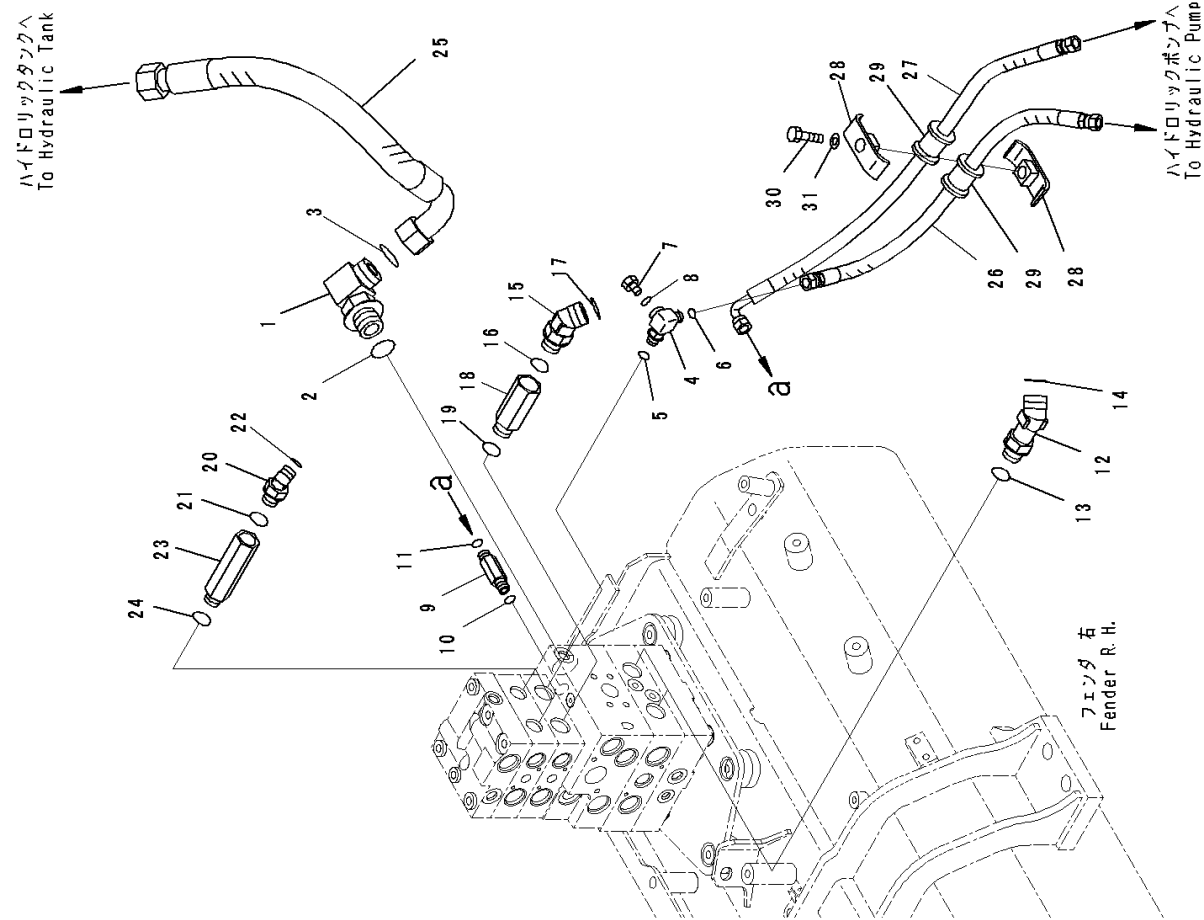
FIG. M2210-001013 Fender Group, For Machine With 3-spool Valve Hydraulics, Hydraulic Piping
