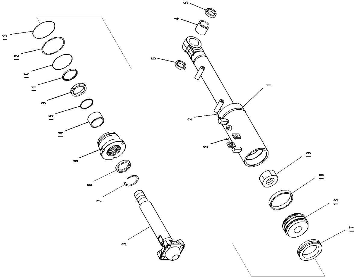
FIG. T2151-001001 Dozer Frame Related Parts, Inner Parts
