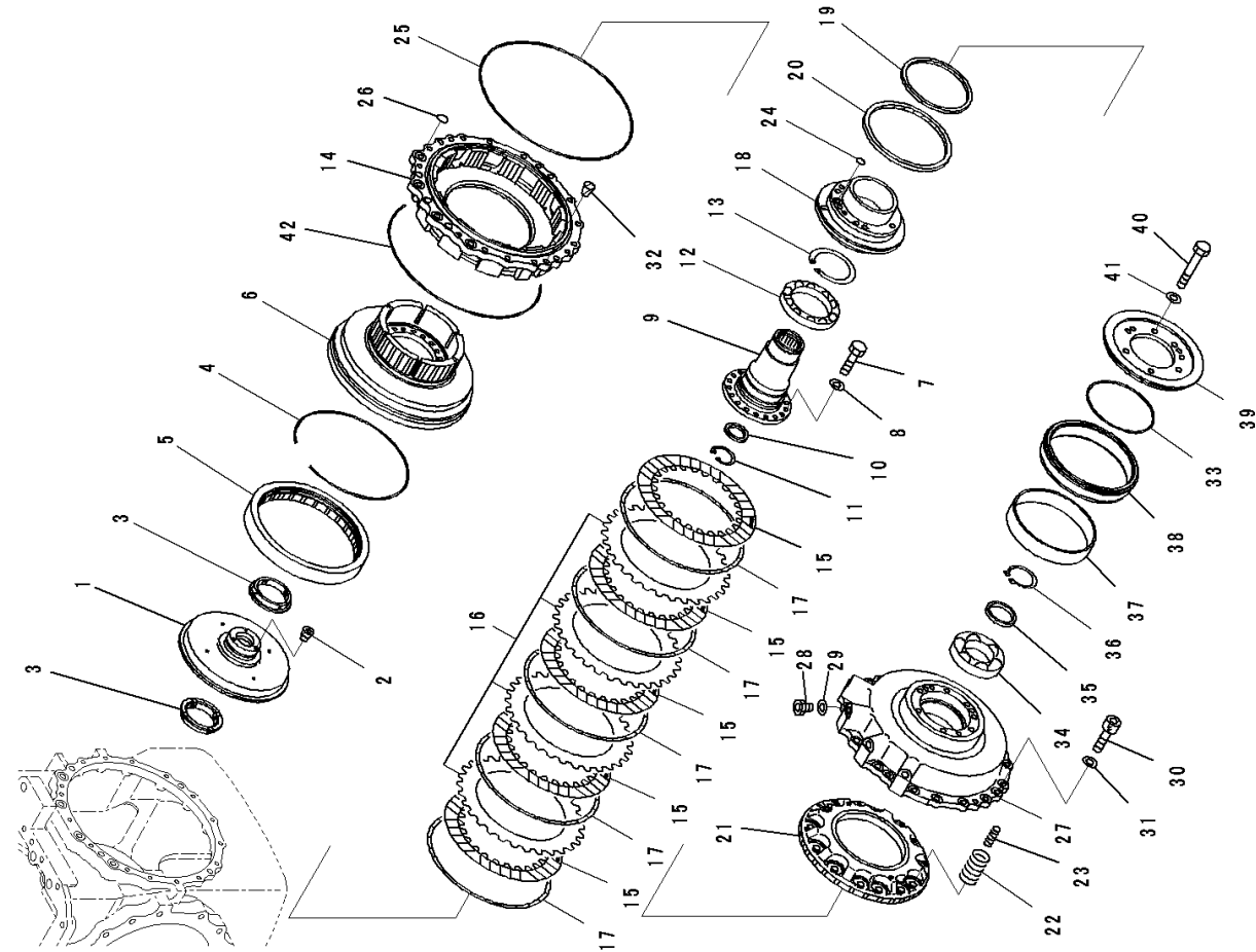
FIG. F2300-001002 Power Train, Brake
