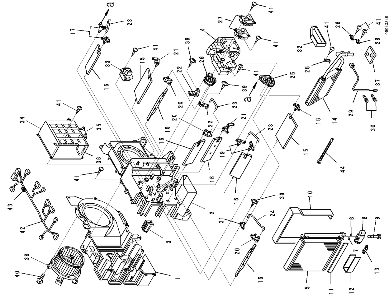
FIG. K0210-007024 ROPS Cab, Air Conditioner Unit
