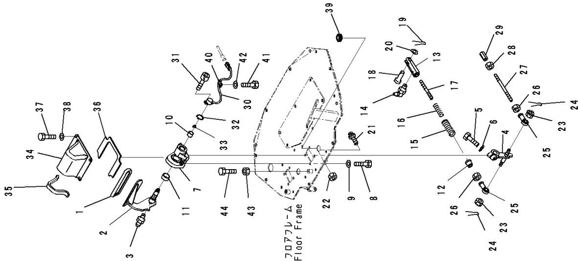
FIG. K0210-002037 ROPS Cab, Brake Pedal
