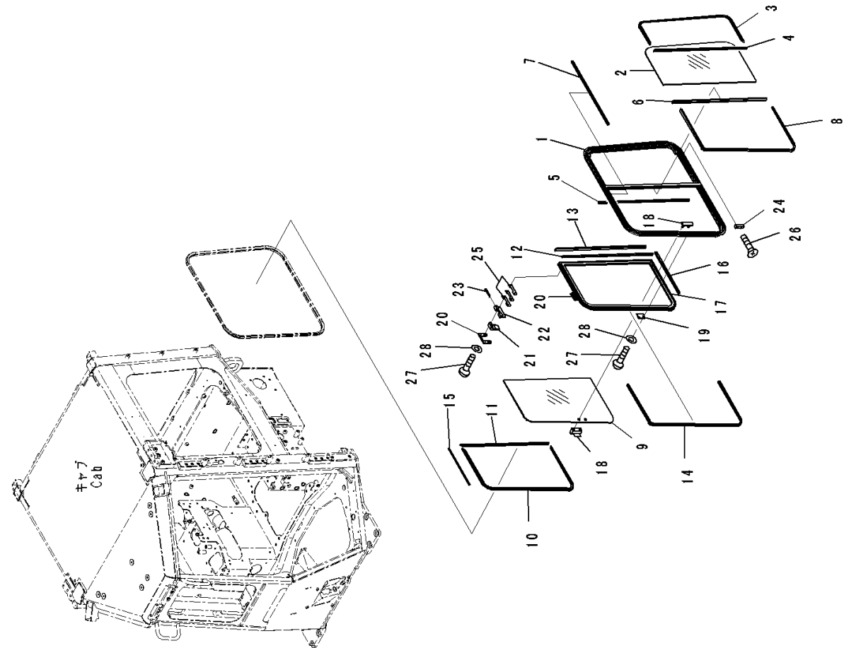
FIG. K0210-002014 ROPS Cab, Sash type Glass Windows, LHS
