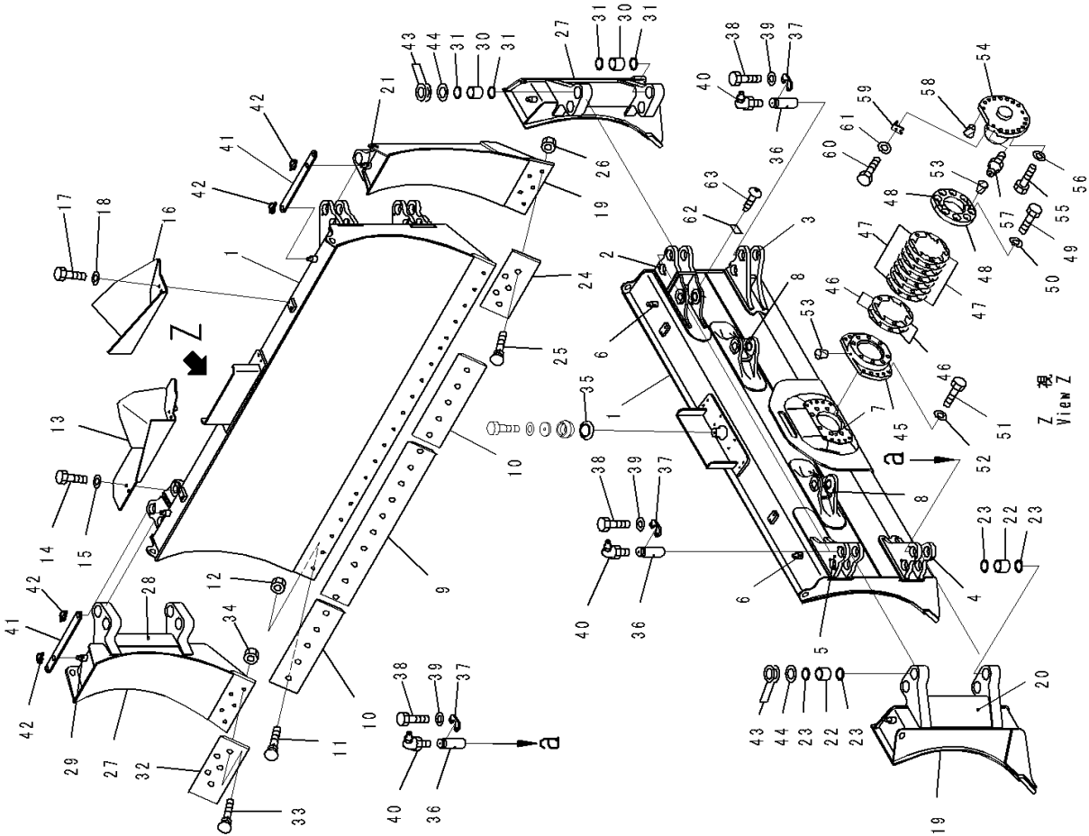
FIG. T2120-003001A Dozer Blade, With 3000mm, Power Angle Power Tilt Blade
