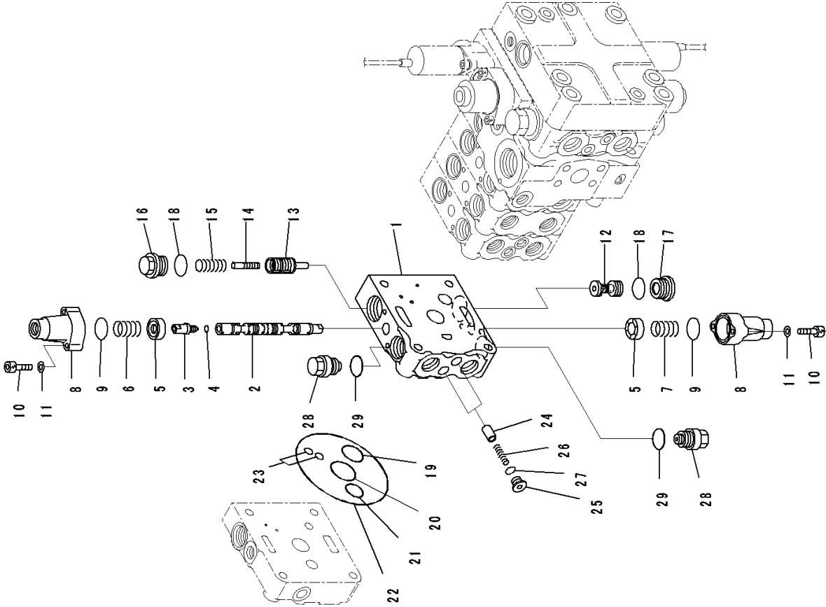
FIG. M2210-003008 Fender Group, Inner Parts (7/12)
