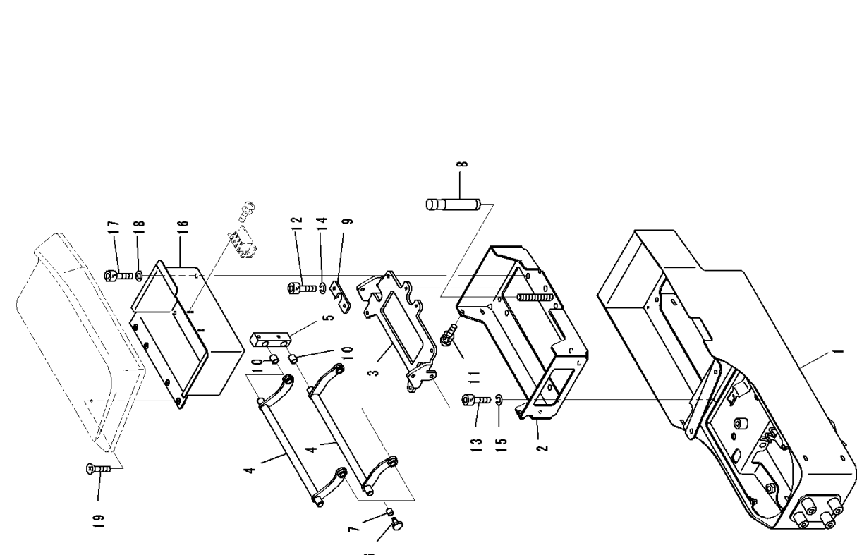
FIG. K0410-002005 ROPS Canopy, Console Box
