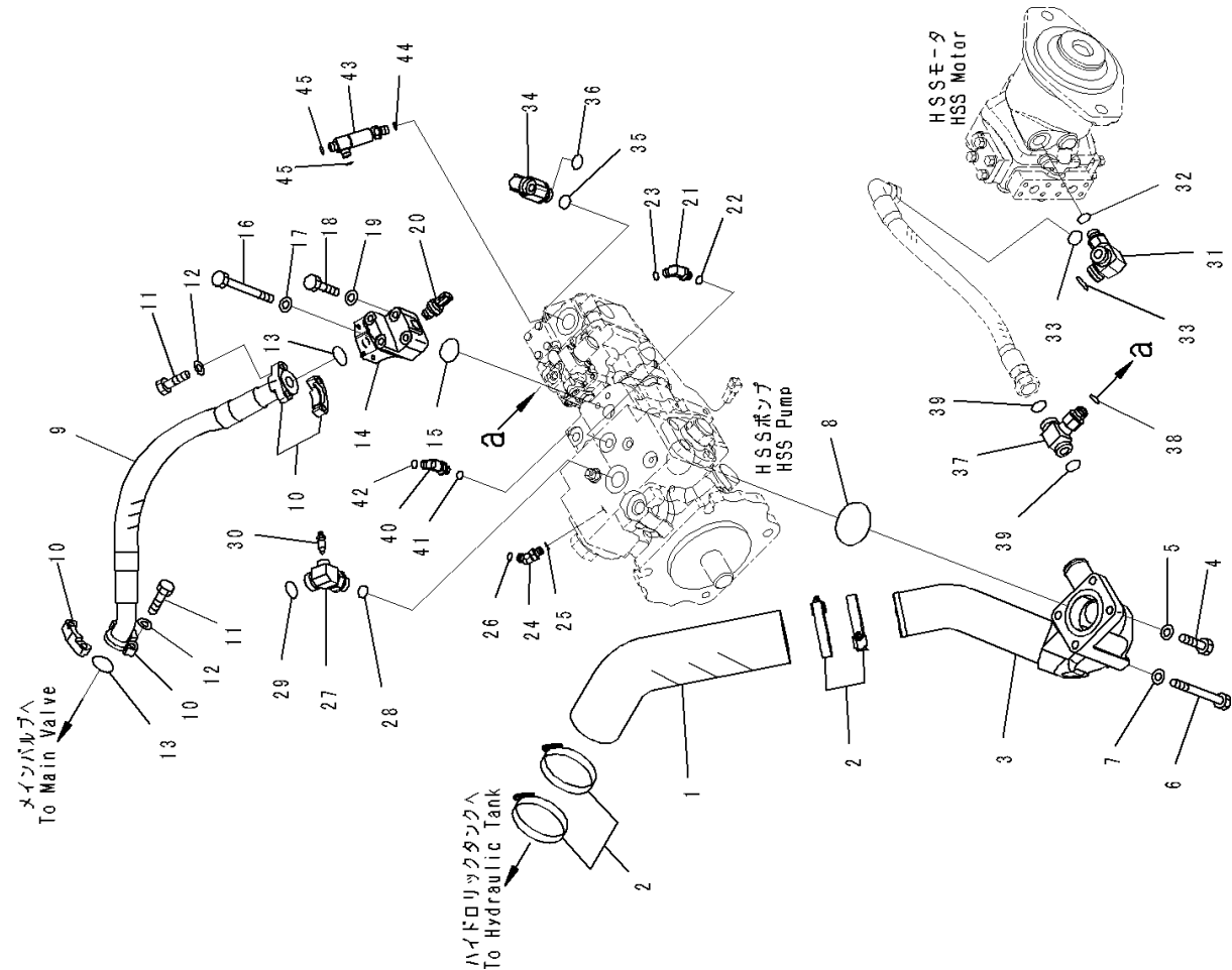
FIG. H0310-001001 Hydraulic Oil Pump Piping, Suction and Delivery Piping
