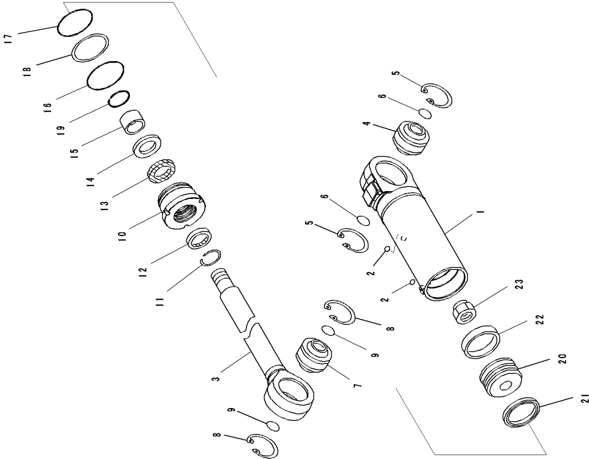
FIG. T2150-002001 Dozer Blade Tilt Cylinder, With Power Angle Power Tilt Dozer, Inner Parts
