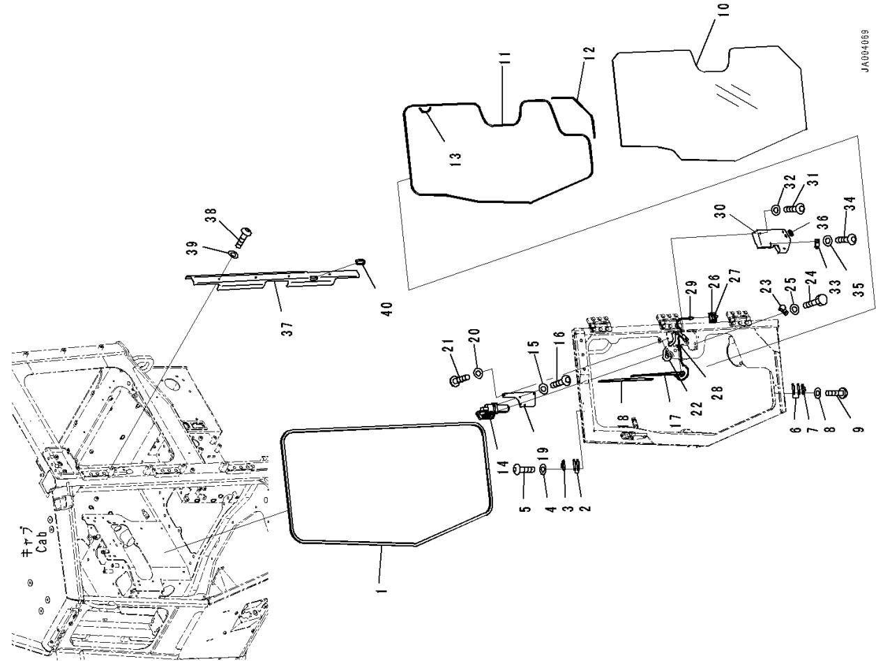
FIG. K0210-007003 ROPS Cab, Door Dumper, Window and Wiper LHS
