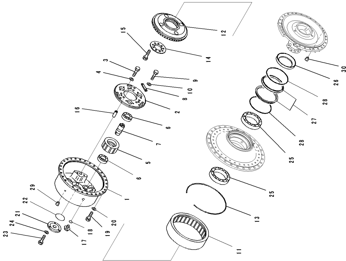
FIG. F2380-001005 Final Drive, Carrier, RHS
