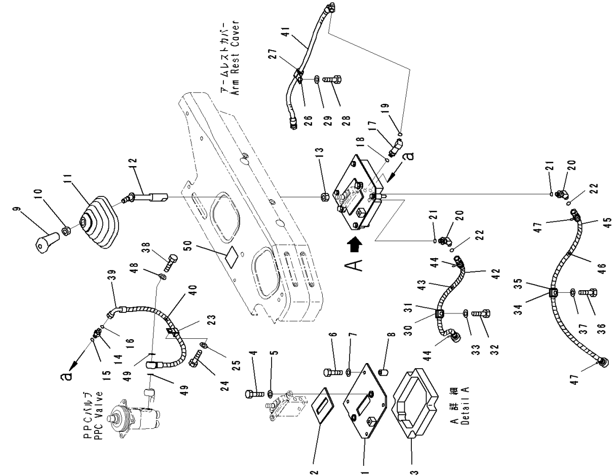
FIG. K2110-002006 Dozer Control, Attachment Lever
