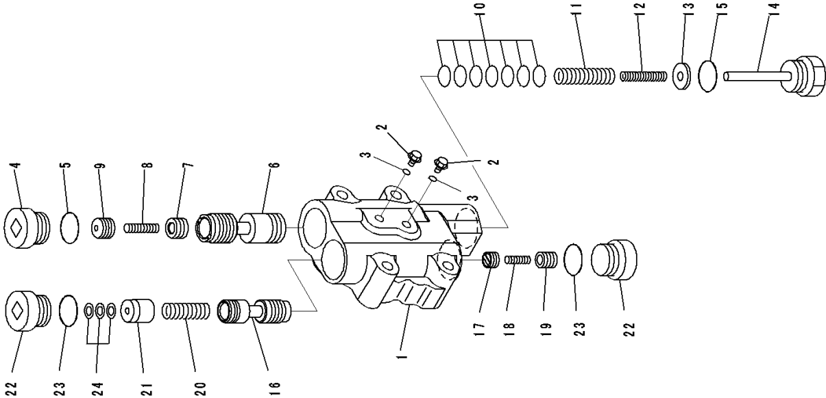
FIG. F2300-001018 Power Train, Relief Valve
