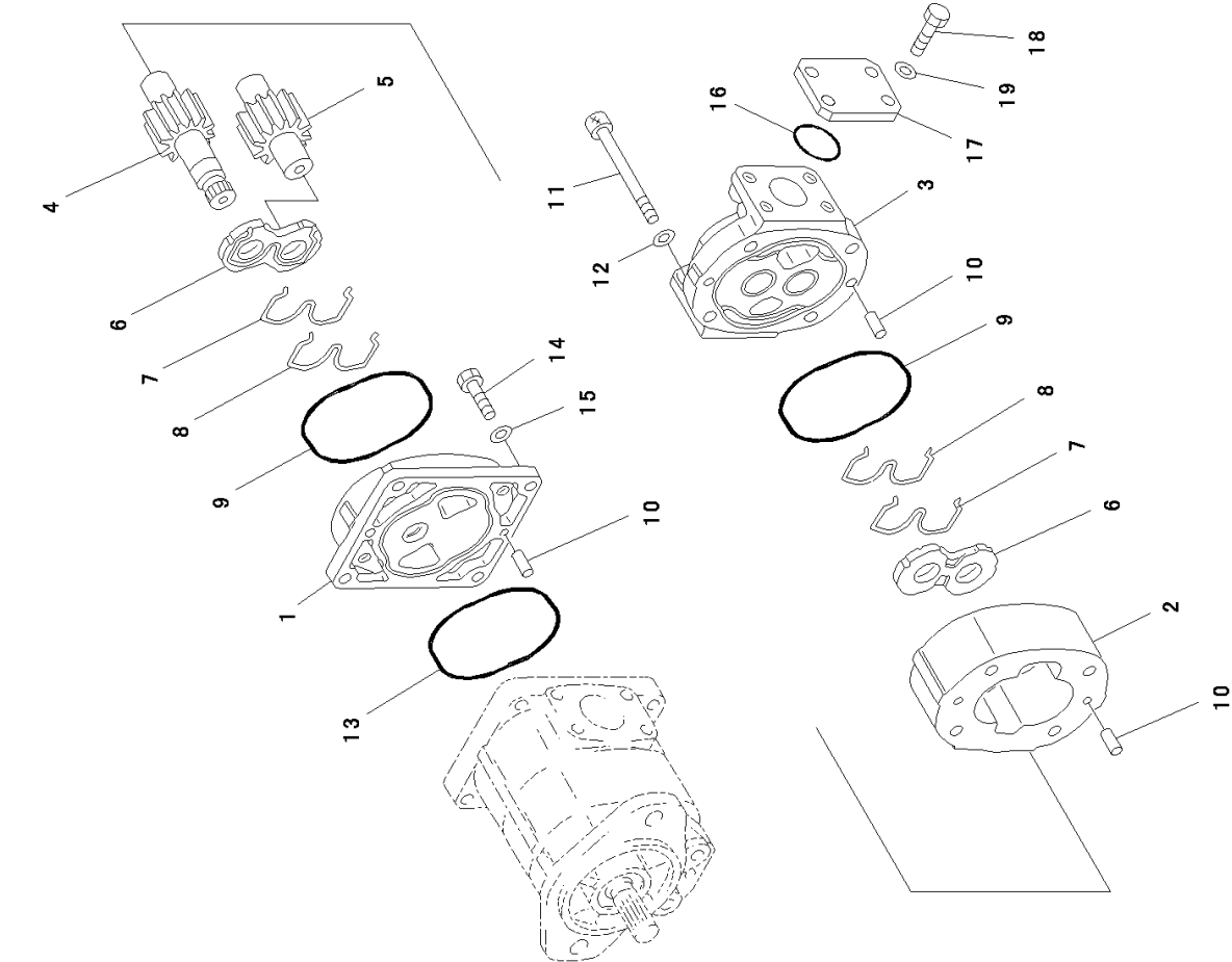
FIG. F2300-001028 Power Train, Gear Pump, SAL (2) 45+ 45 (2/2)
