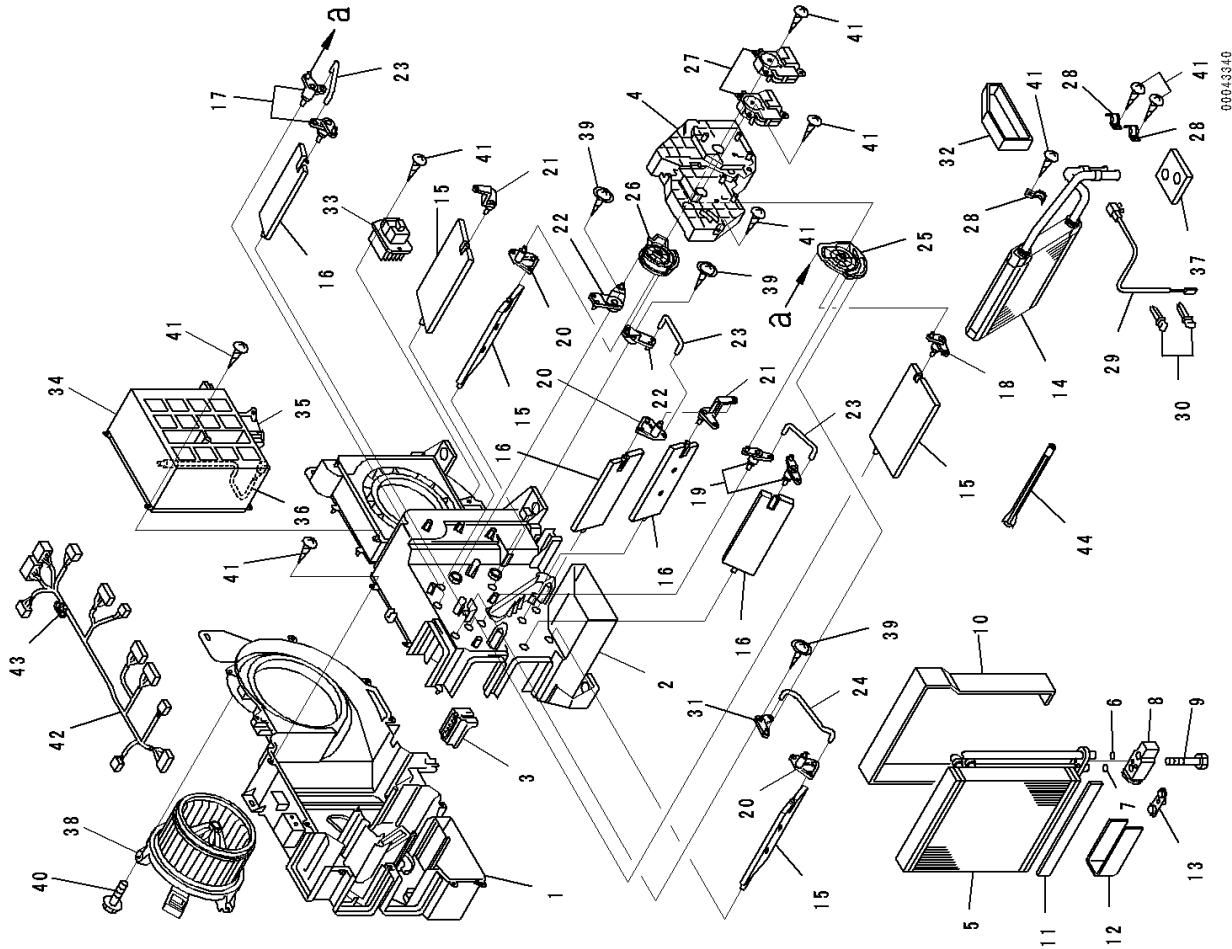
FIG. K0210-002024 ROPS Cab, Air Conditioner Unit
