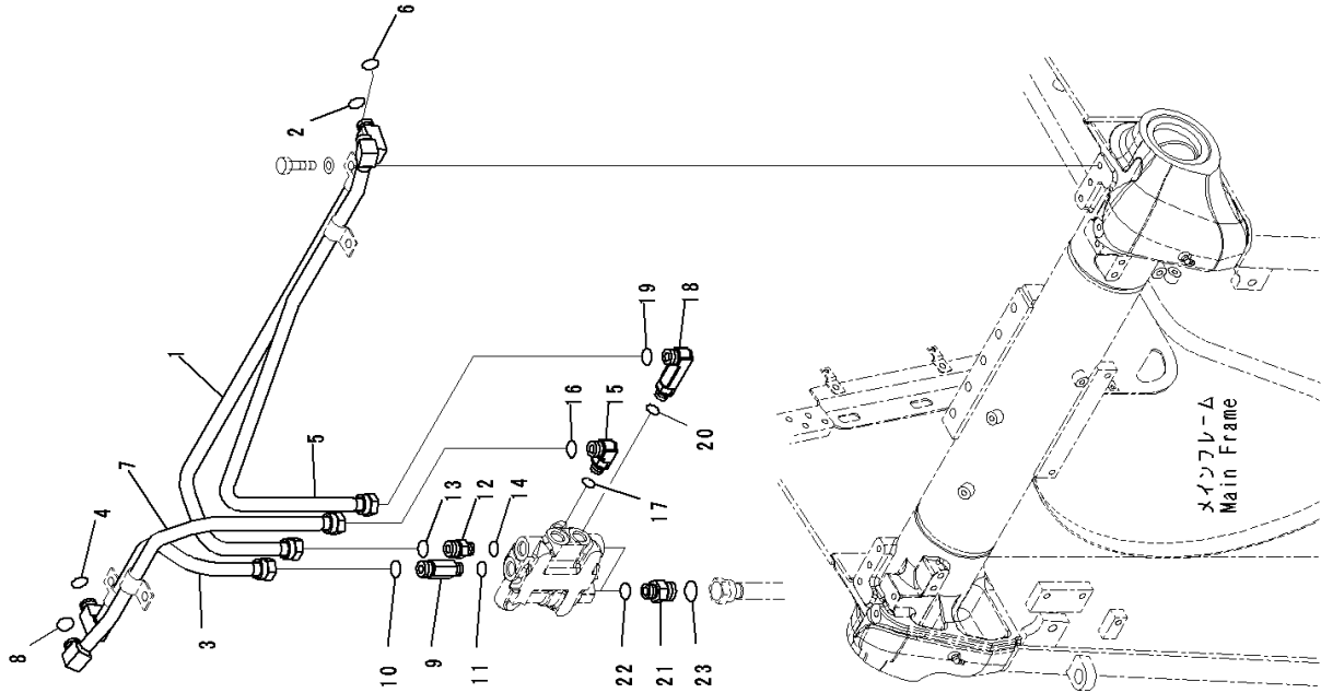
FIG. H2210-003003 Dozer Blade Lift Piping, Piping (2/2)
