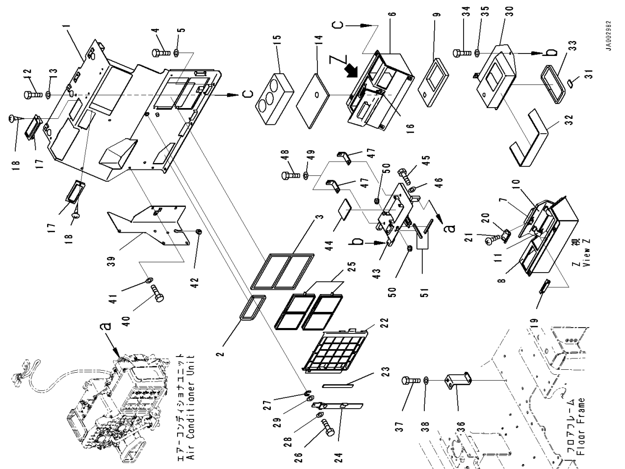
FIG. K0210-012029 ROPS Cab, Air Conditioner Duct (3/3)
