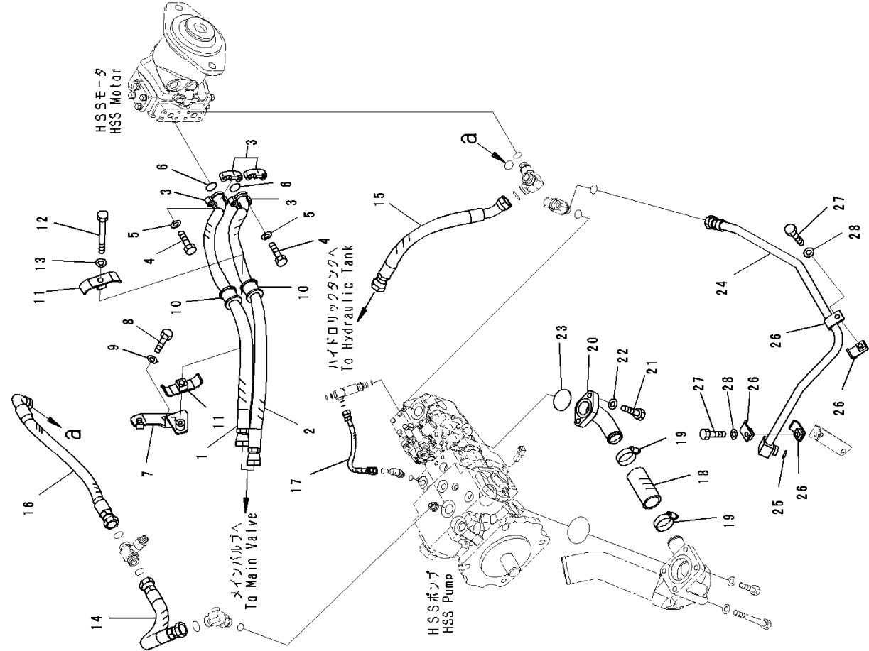
FIG. H0310-001002 Hydraulic Oil Pump Piping, HSS Motor Piping
