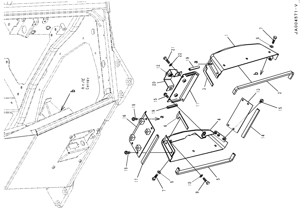
FIG. K0410-002018 ROPS Canopy, Dashboard Cover
