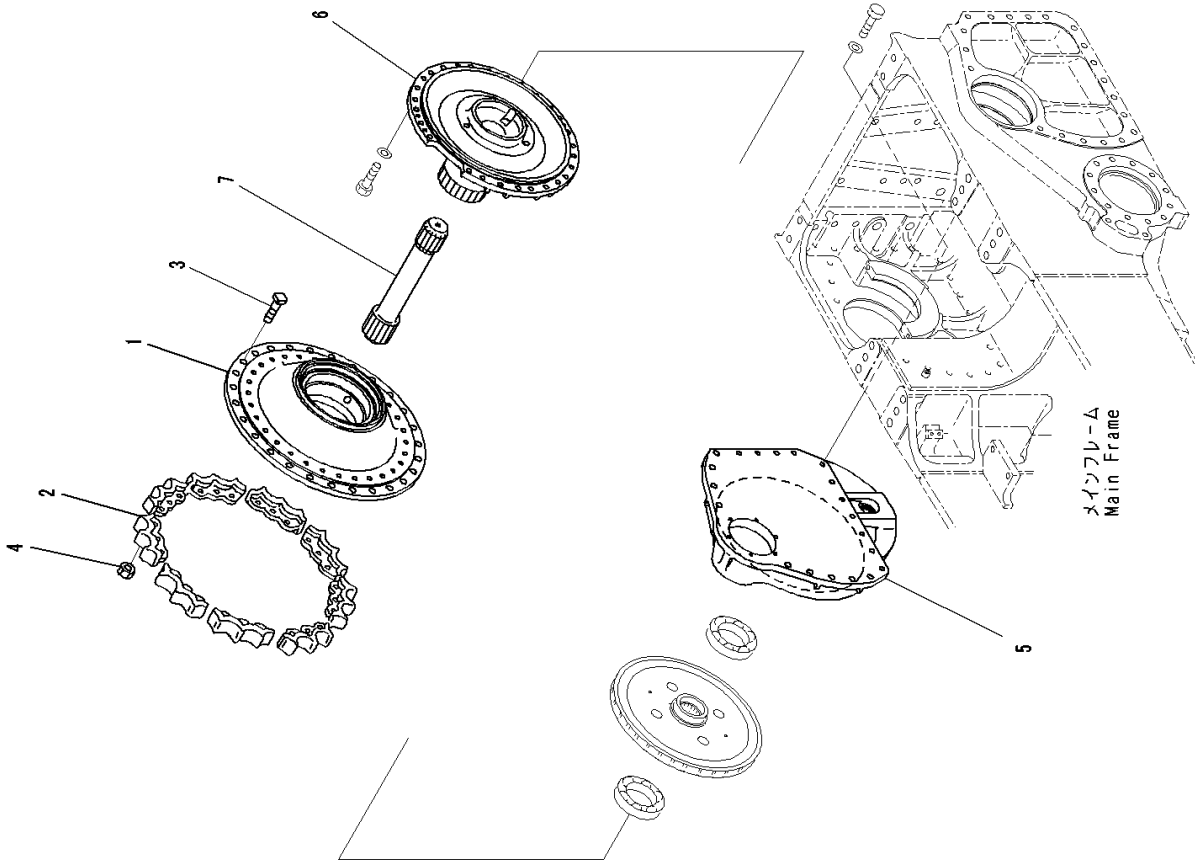
FIG. F2380-003006 Final Drive, Sprocket Hub, RHS
