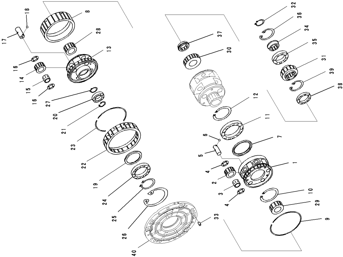
FIG. F2300-001012 Power Train, Transmission Carrier (1/2)
