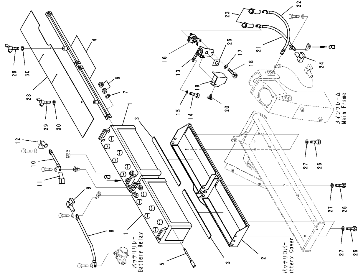
FIG. E0100-006001 Battery, With Refuel Pump, For Large Capacity Battery
