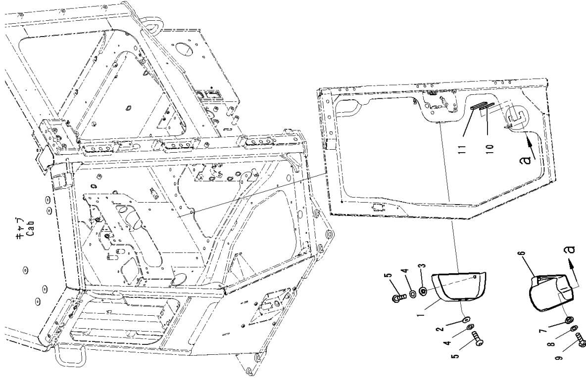
FIG. K0210-007004 ROPS Cab, Door Cover, LHS
