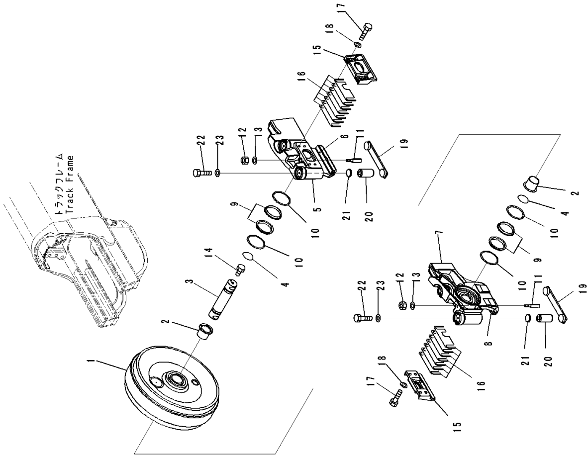
FIG. R0110-001001 Front Idler
