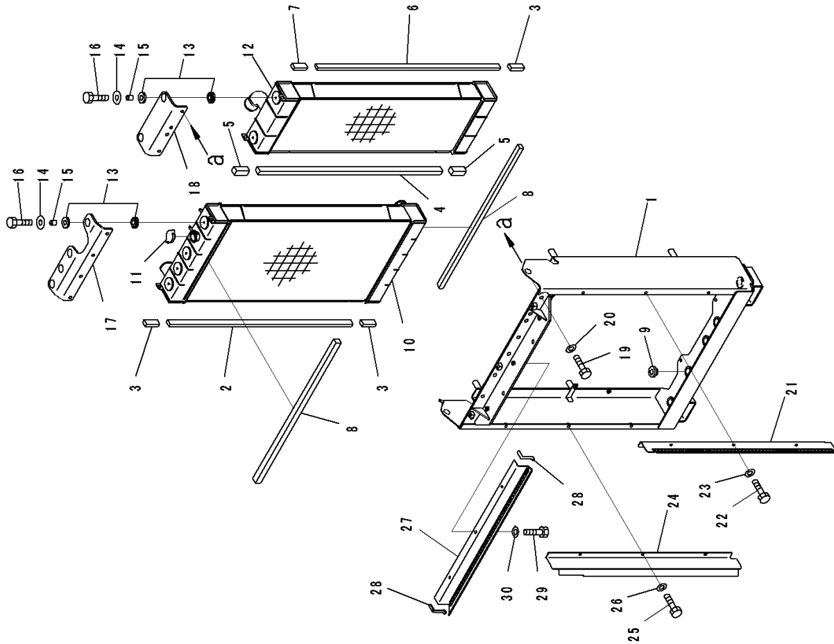
FIG. C0100-001001 Radiator, Radiator Core and Aftercooler
