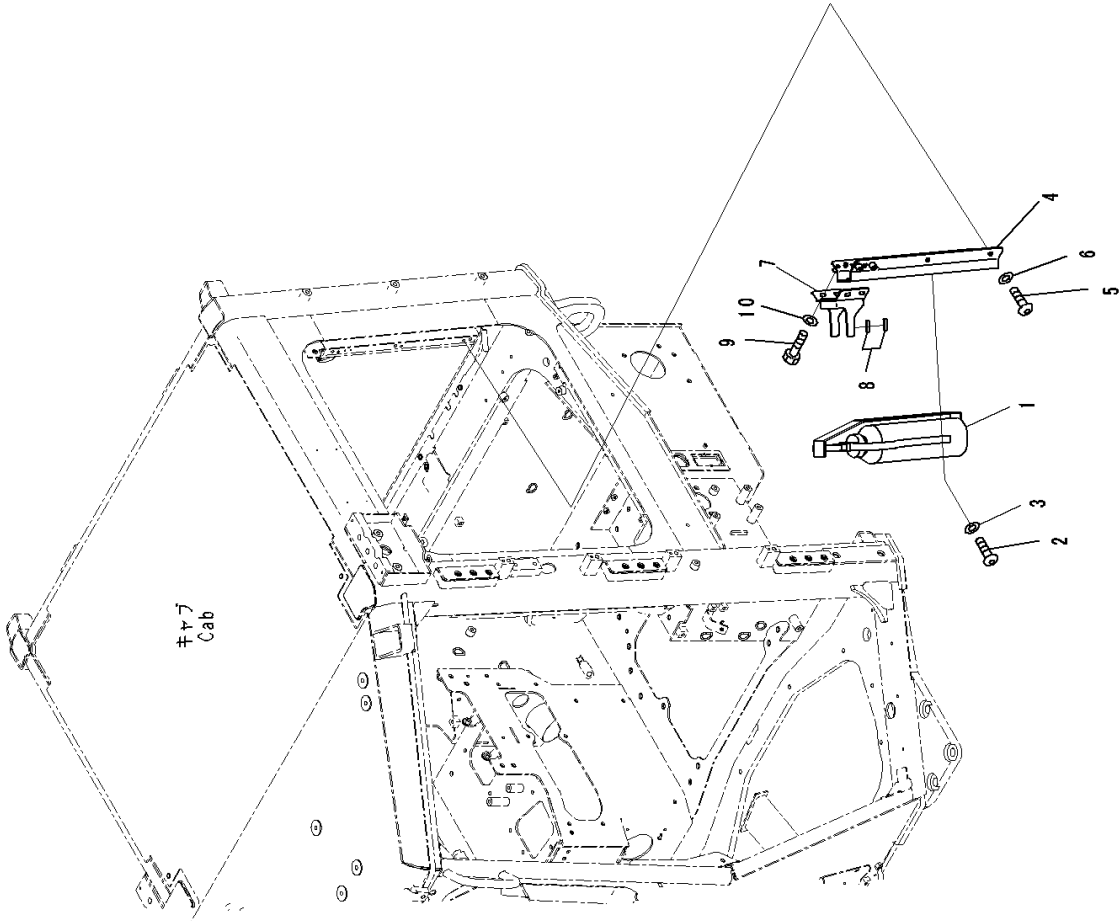
FIG. K0830-001001 Fire Extinguisher, English
