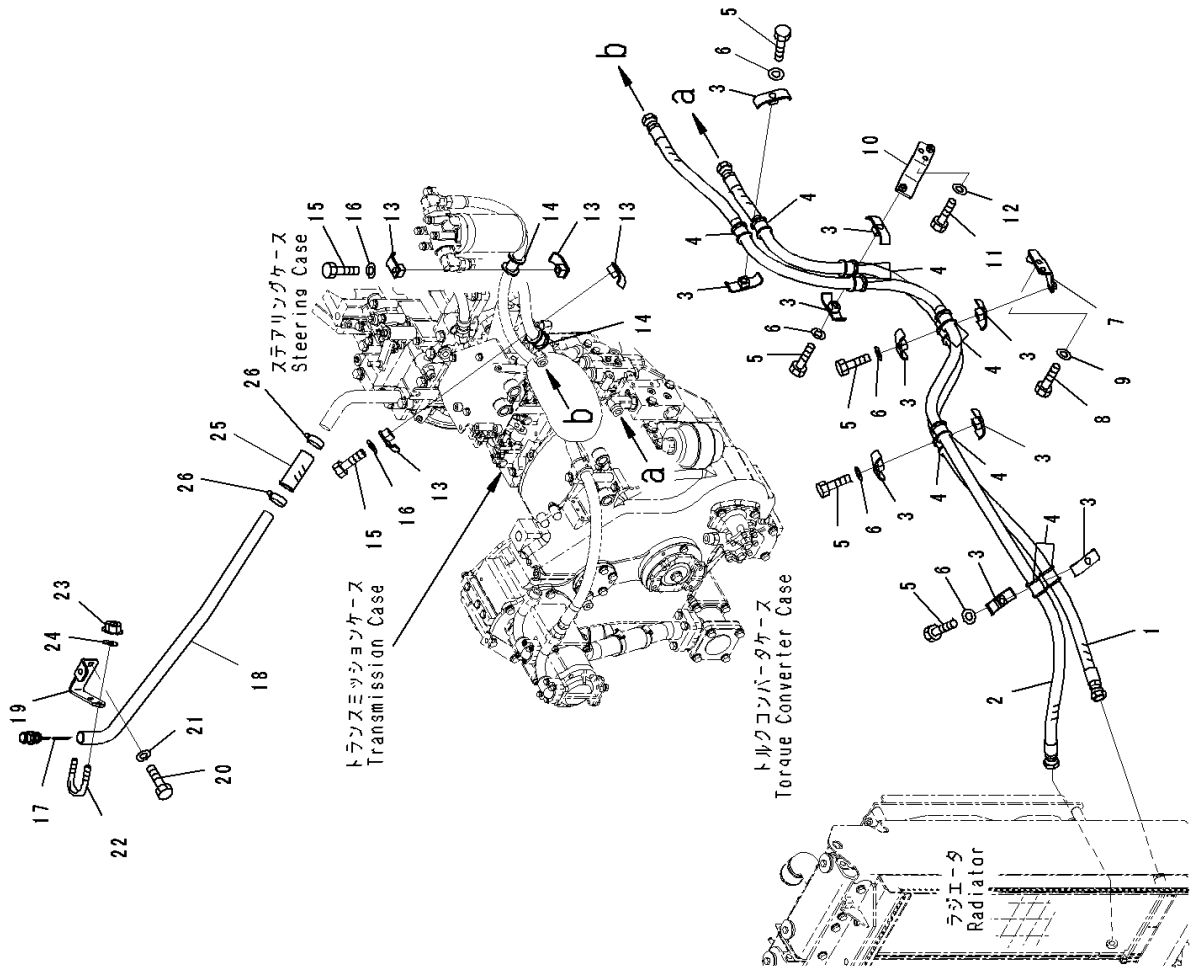
FIG. F2730-001001 Power Train Piping, Piping
