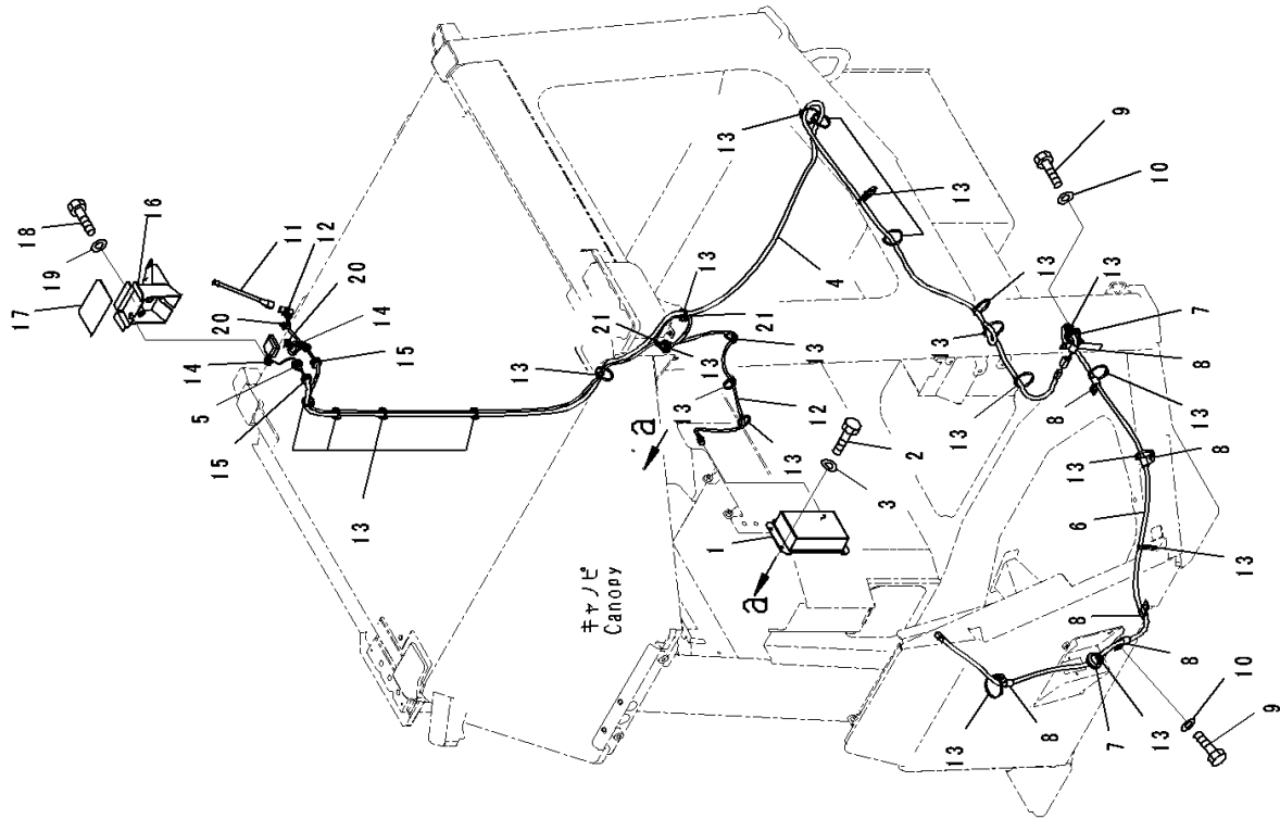
FIG. K0410-002023 ROPS Canopy, KOMTRAX Controller
