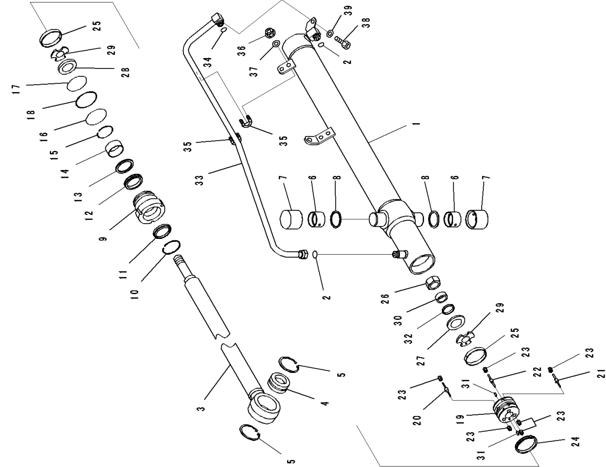
FIG. T2140-002001 Dozer Blade Lift Cylinder, With Power Angle Power Tilt Dozer, Inner Parts, LHS
