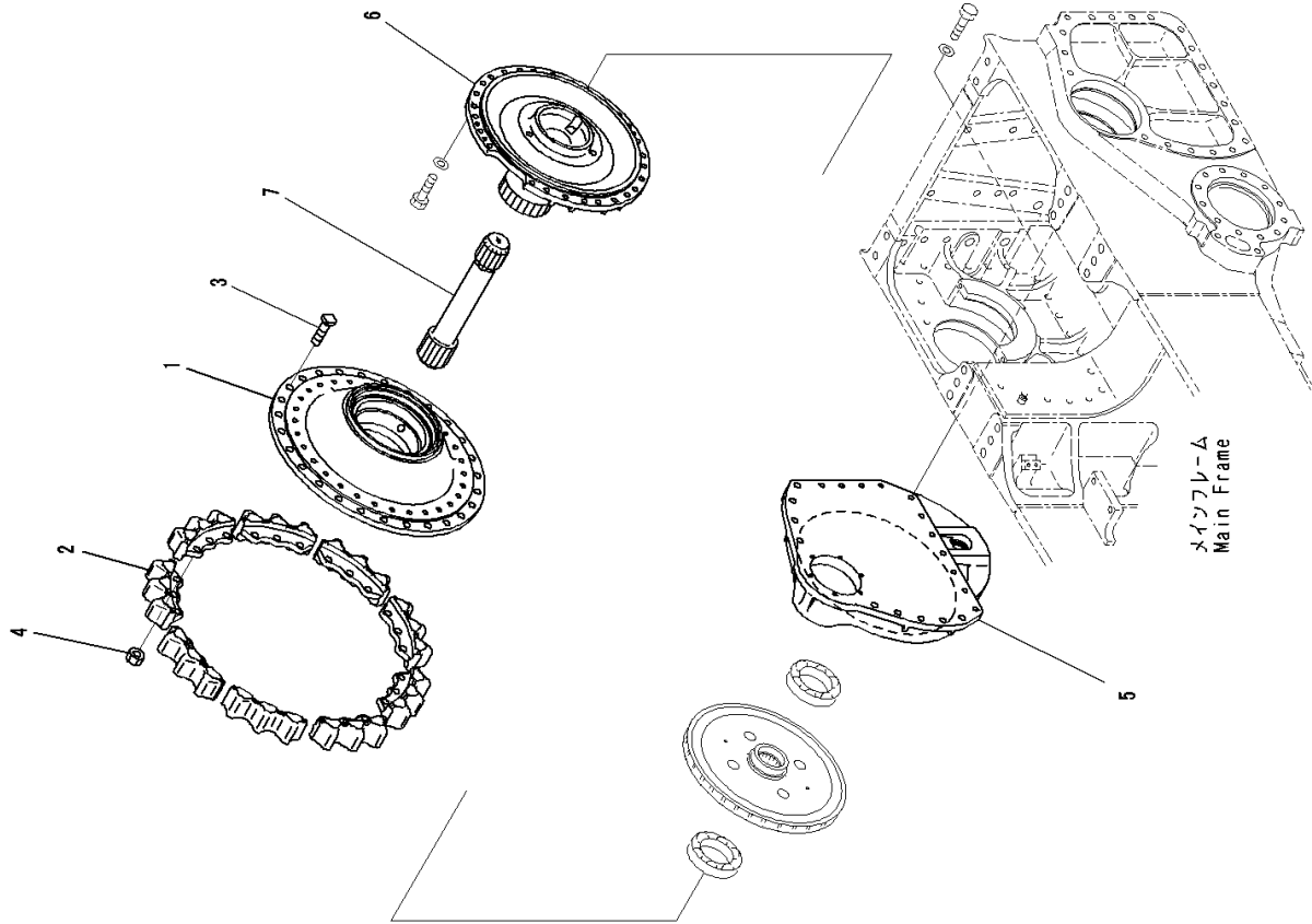
FIG. F2380-001006 Final Drive, Sprocket Hub, RHS
