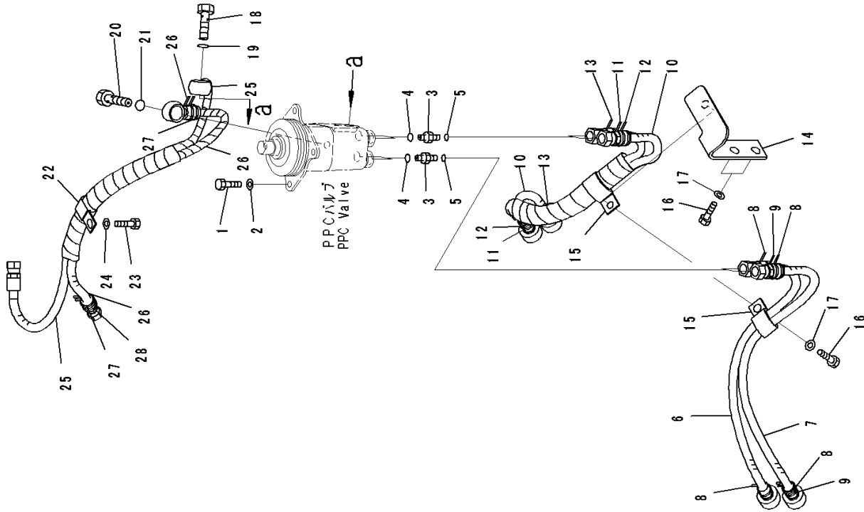
FIG. K2110-001004 Dozer Control, Hose
