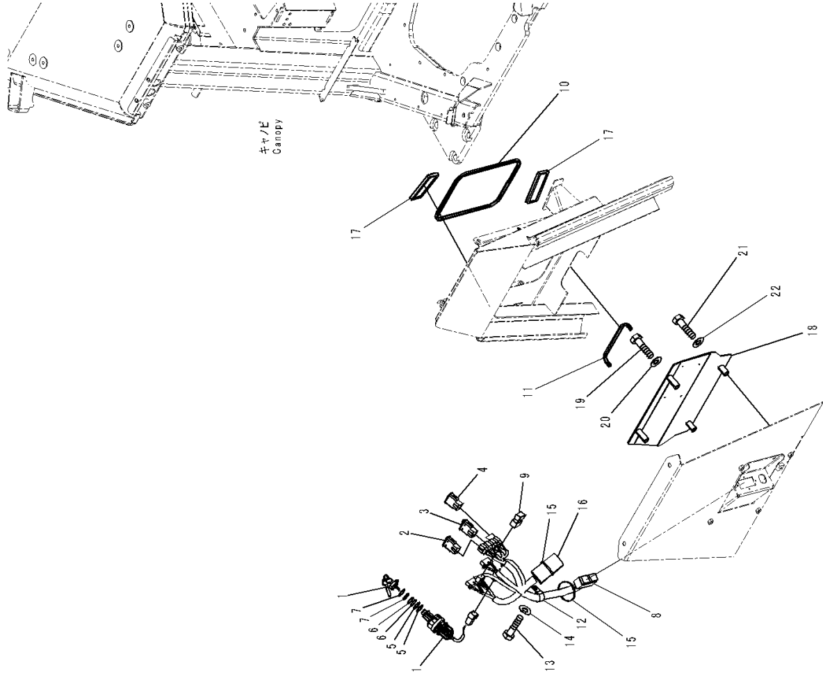
FIG. K0410-002020 ROPS Canopy, Floor, Switch
