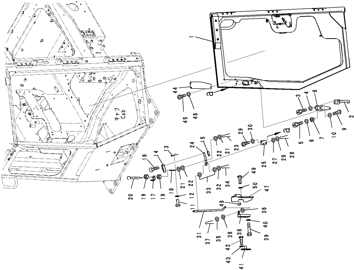
FIG. K0210-002002 ROPS Cab, Door and Latch, LHS
