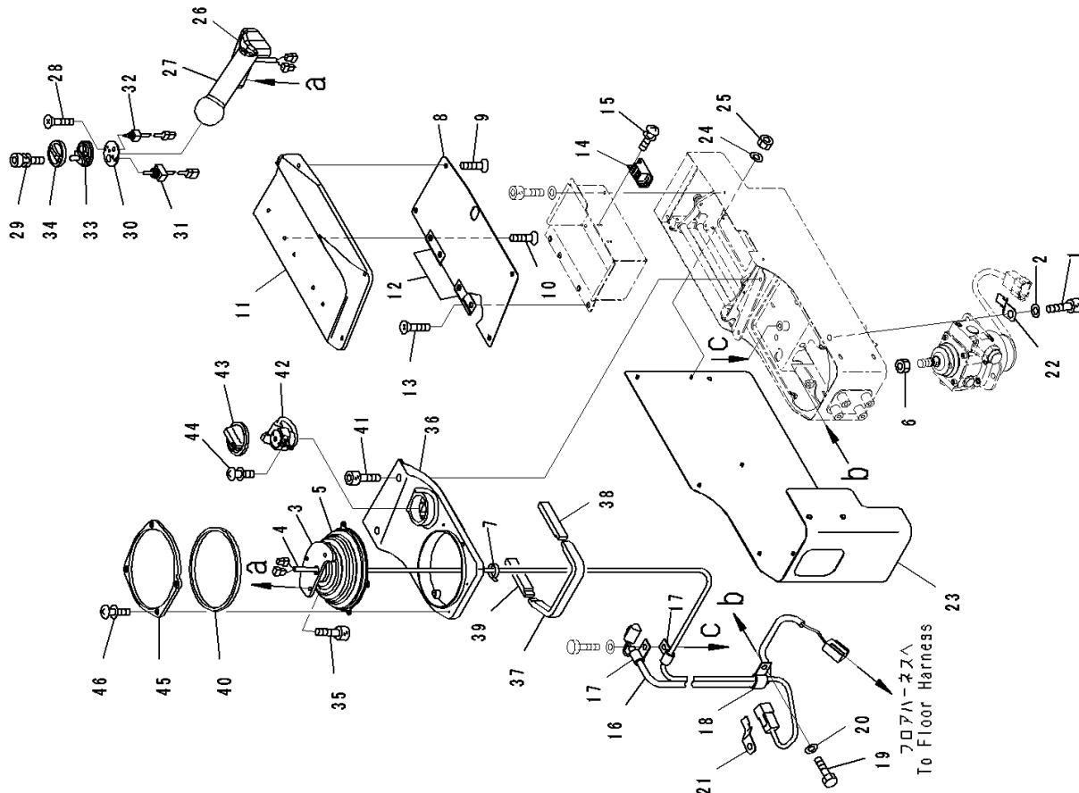
FIG. K0410-002007 ROPS Canopy, Travel Control Lever (2/2)
