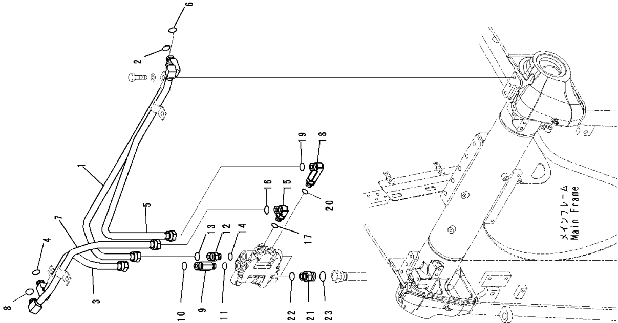
FIG. H2210-001003 Dozer Blade Lift Piping, Piping (2/2)
