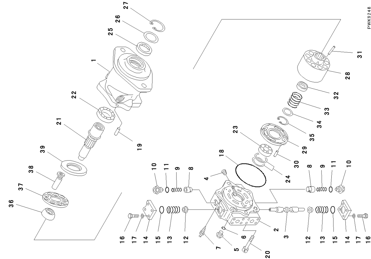
FIG. H0210-001009 Hydraulic Oil Pump and Motor, HSS Motor (1/2)
