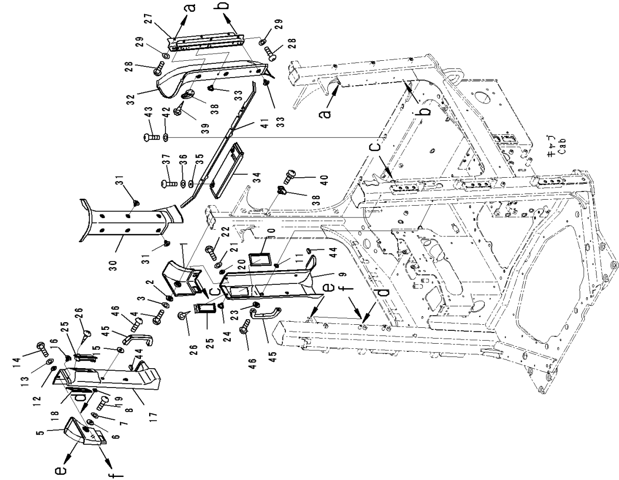
FIG. K0210-007021 ROPS Cab, Roof Cover (2/2)
