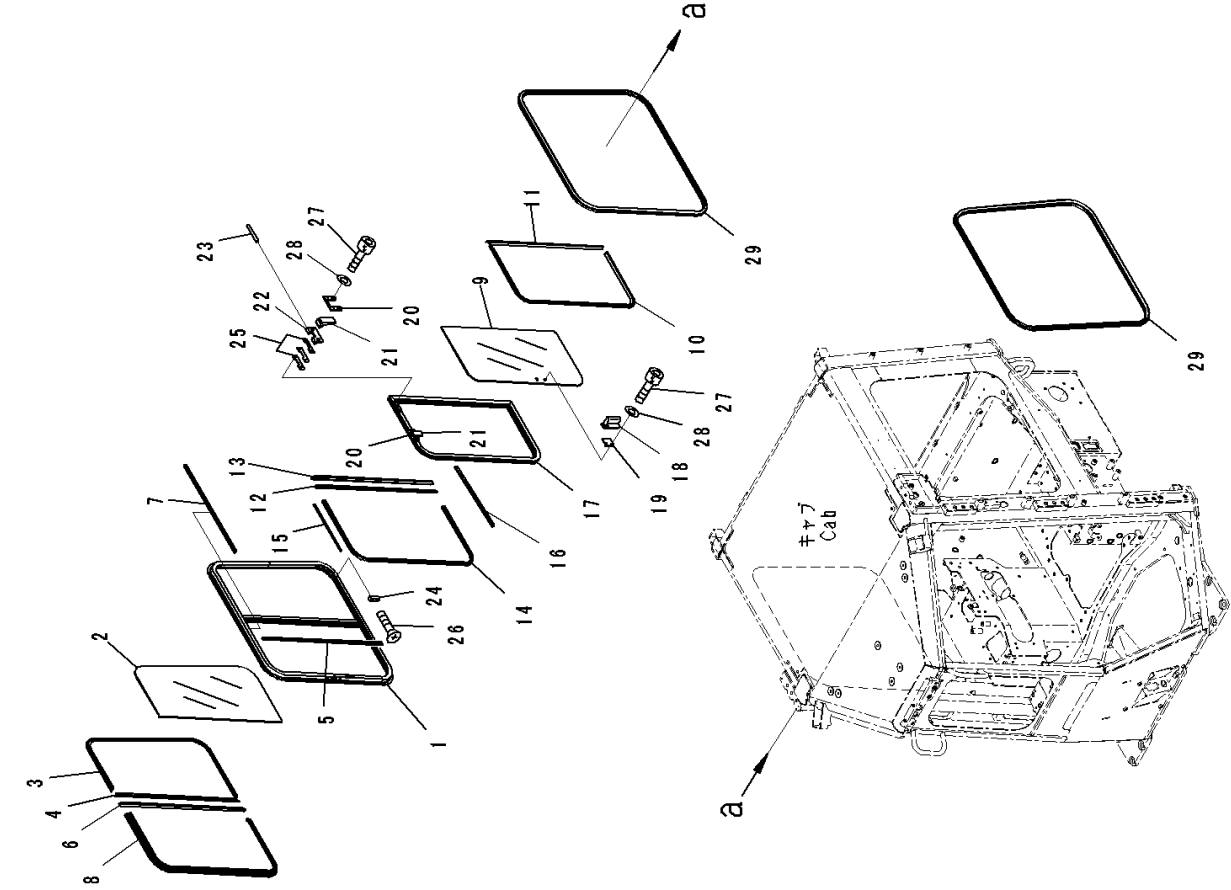
FIG. K0210-007015 ROPS Cab, Sash type Glass Windows, RHS
