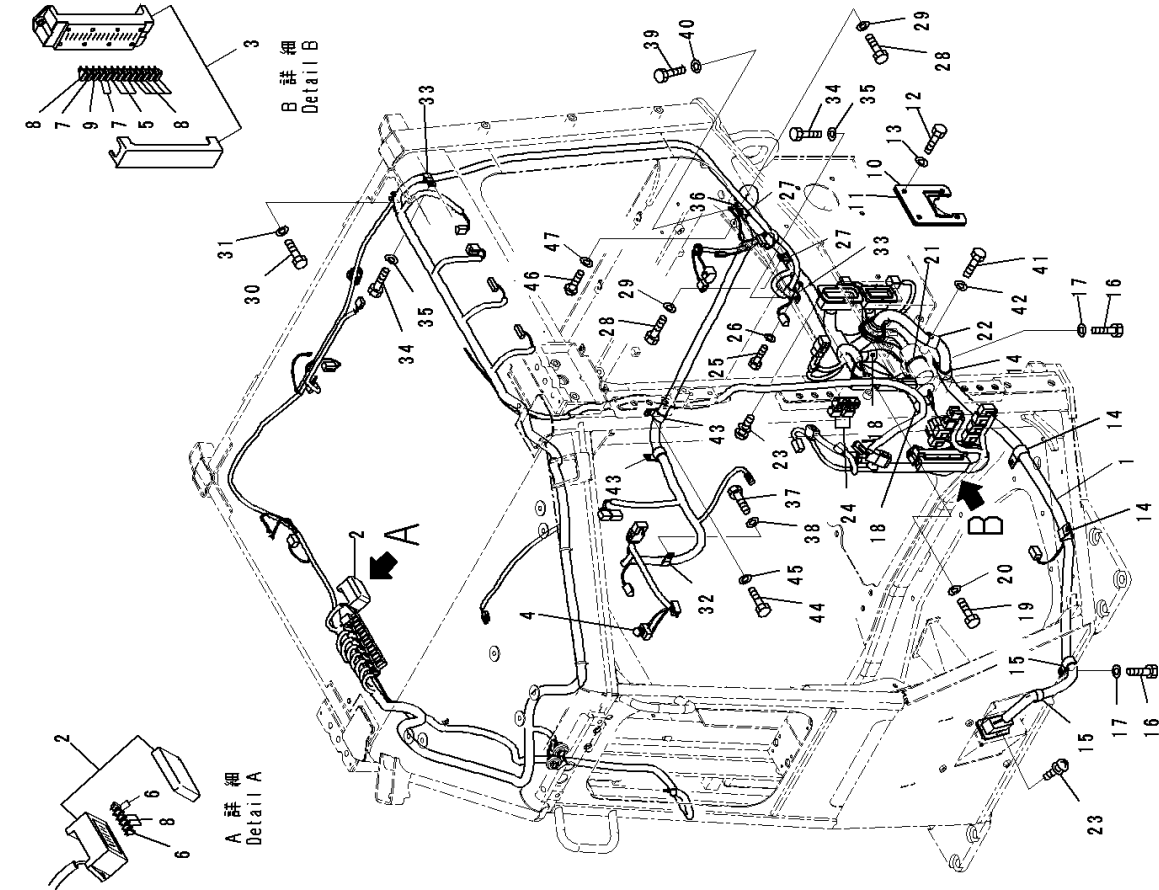
FIG. K0210-012040 ROPS Cab, Floor, Harness (1/3)
