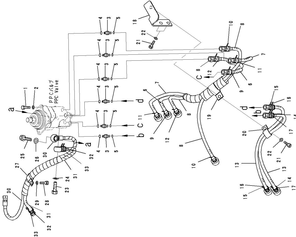
FIG. K2110-012005 Dozer Control, Hose
