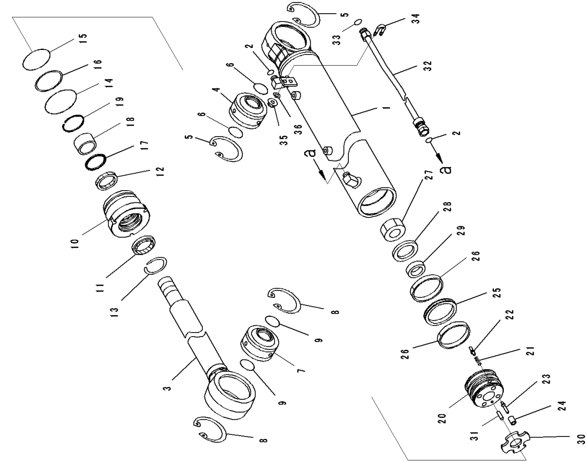
FIG. T2153-001001 Dozer Blade Angle Cylinder, With Power Angle Power Tilt Dozer, Inner Parts
