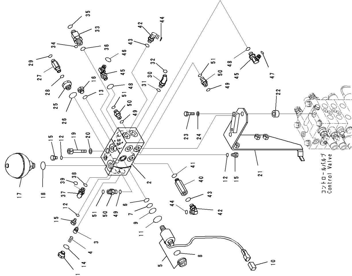
FIG. M2210-005016 Fender Group, PPC Lock Solenoid Valve With Accumulator
