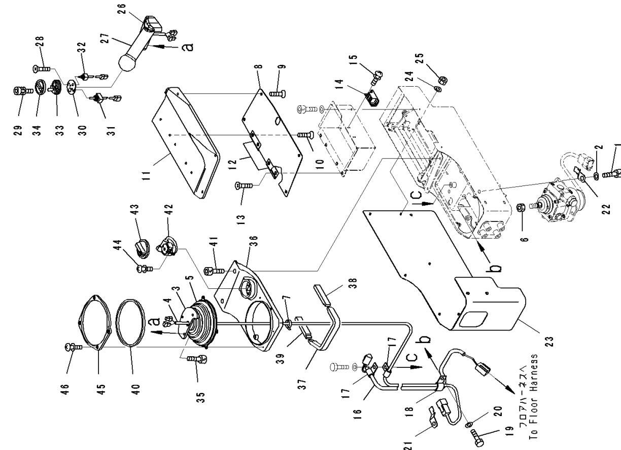
FIG. K0210-002032 ROPS Cab, Travel Control Lever (2/2)
