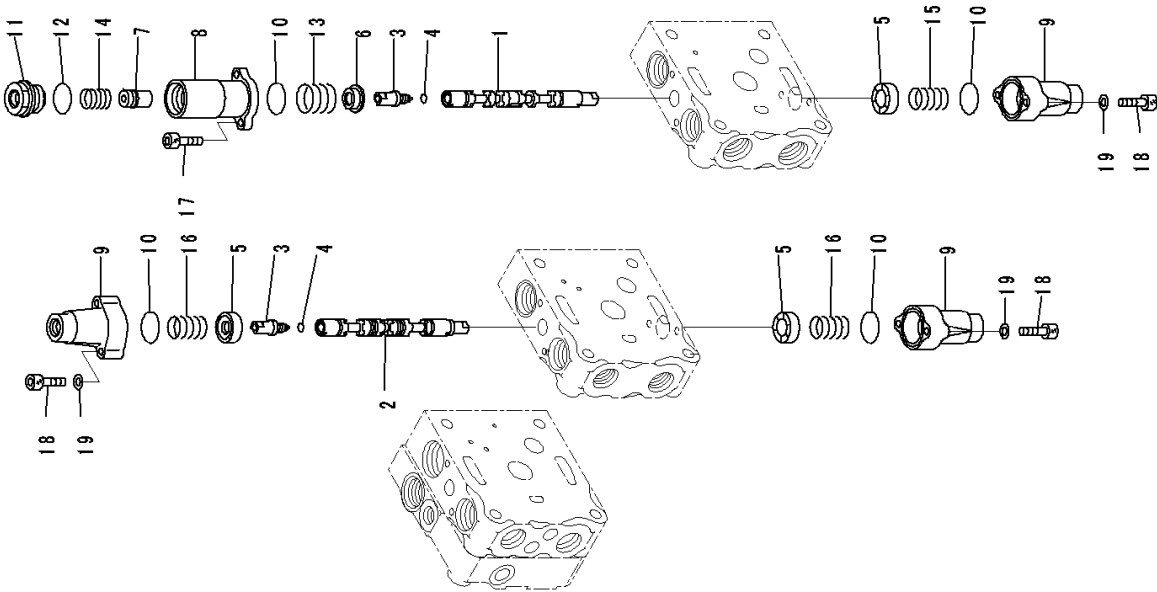
FIG. M2210-002003 Fender Group, For Machine With 4-spool Valve Hydraulics, For Machine With Ripper, Inner Parts (2/11)
