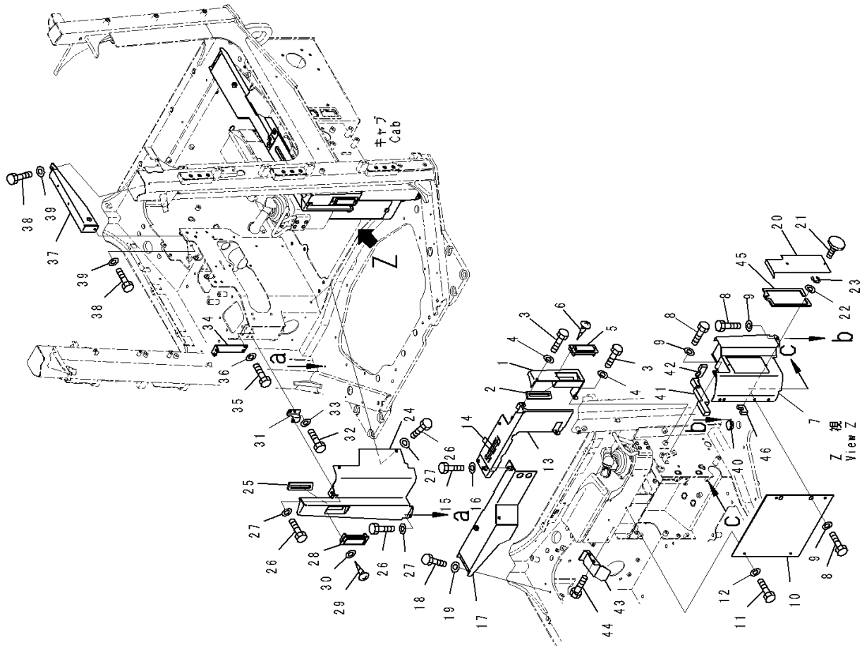
FIG. K0210-012048 ROPS Cab, Floor Cover
