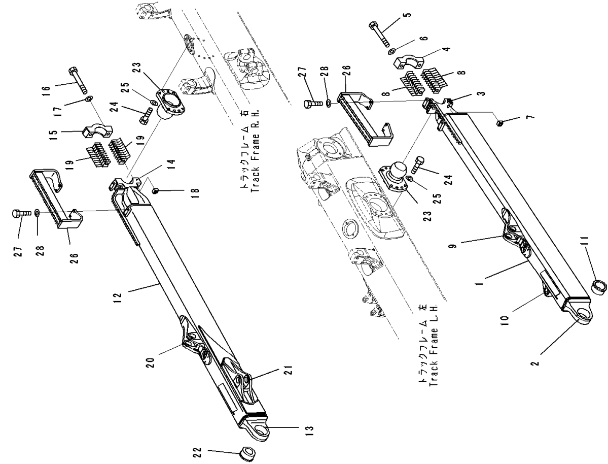
FIG. T21110-003001 Dozer Frame, With Power Tilt Pitch Dozer
