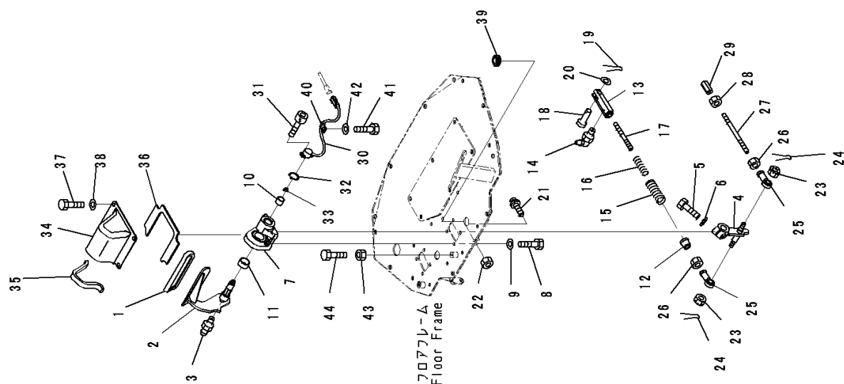
FIG. K0210-007037 ROPS Cab, Brake Pedal
