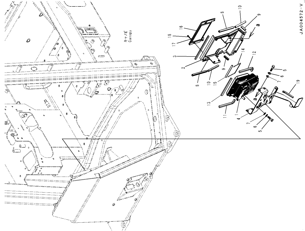
FIG. K0410-002019 ROPS Canopy, Monitor
