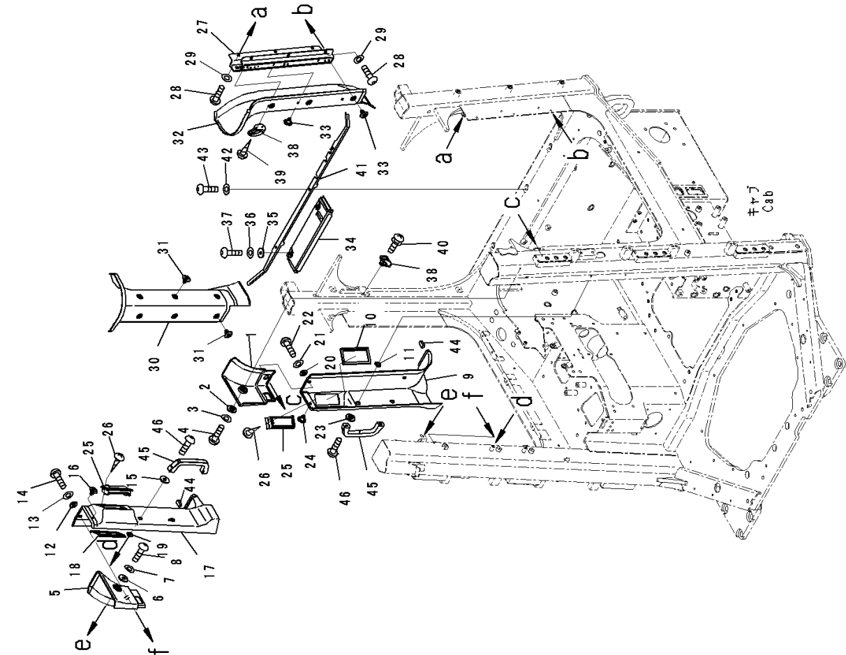
FIG. K0210-002021 ROPS Cab, Roof Cover (2/2)
