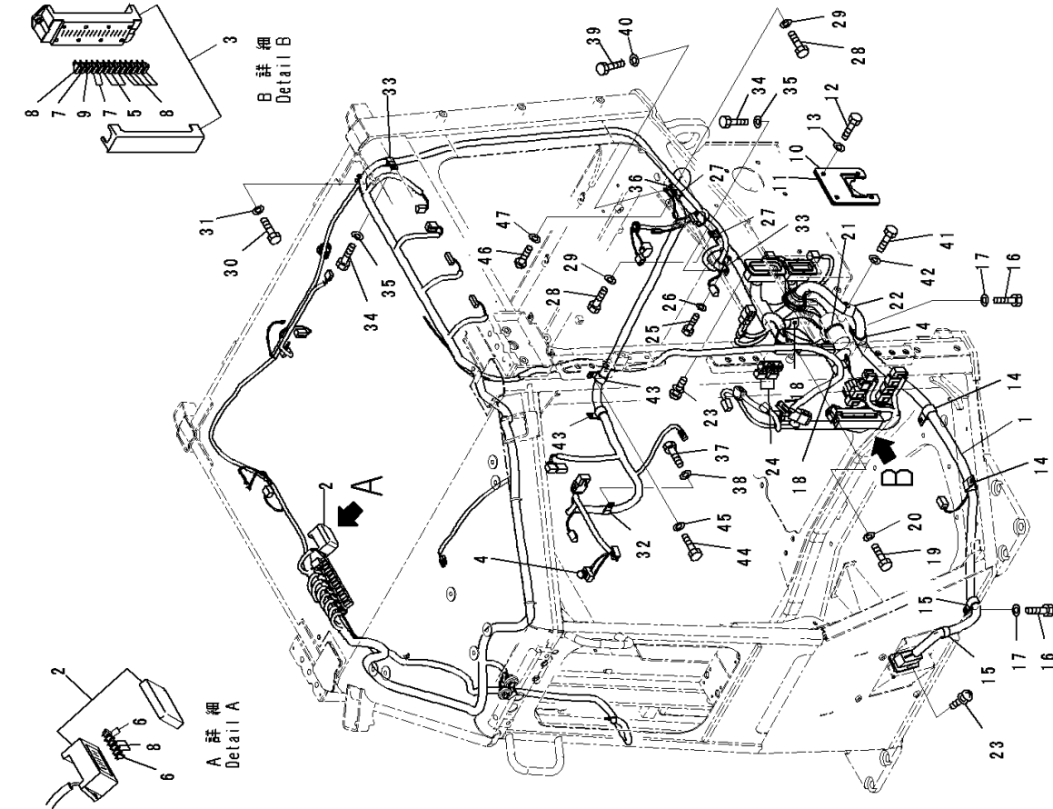
FIG. K0210-002040 ROPS Cab, Floor, Harness (1/3)
