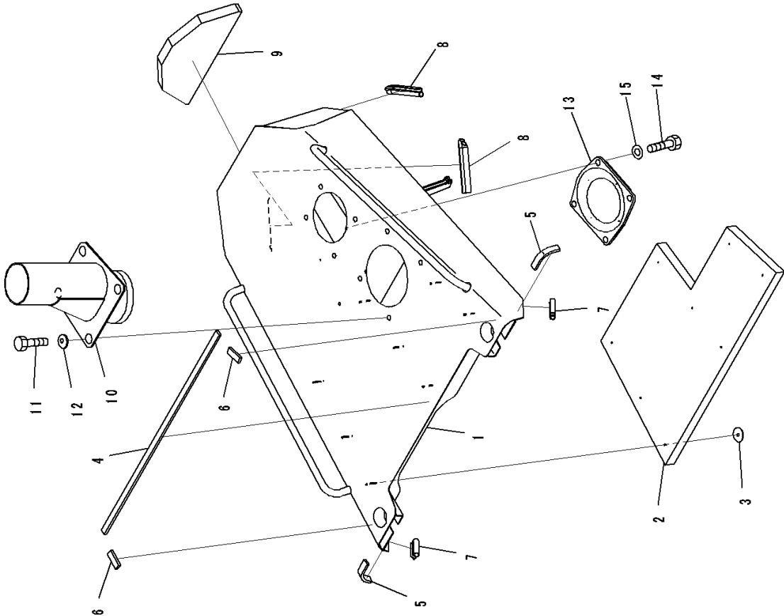
FIG. M2140-002001 Front Guard Group, For Engine Hood And Sides, For EU Noise Reguration, Hood
