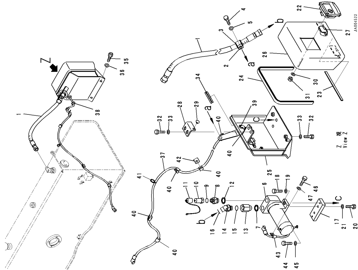
FIG. W1113-001001 Fuel Self Charge Pump
