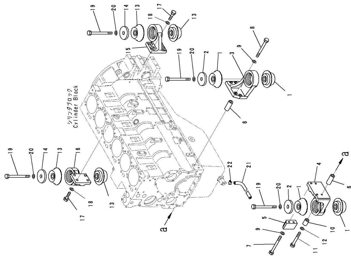
FIG. B0100-001001 Engine Mounts
