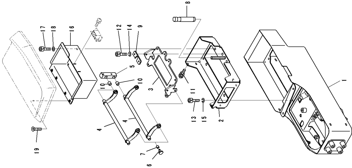
FIG. K0210-002030 ROPS Cab, Console Box
