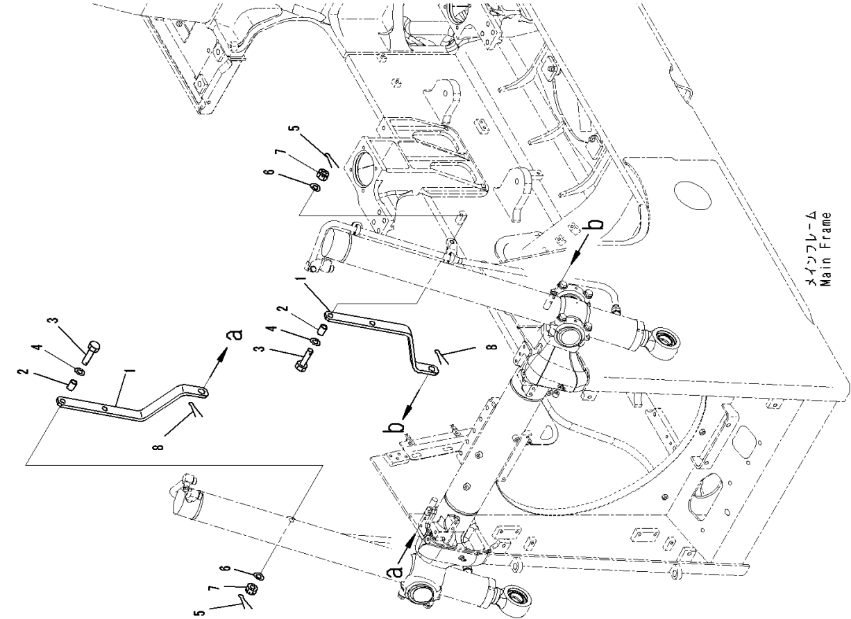
FIG. T2140-001003 Dozer Blade Lift Cylinder
