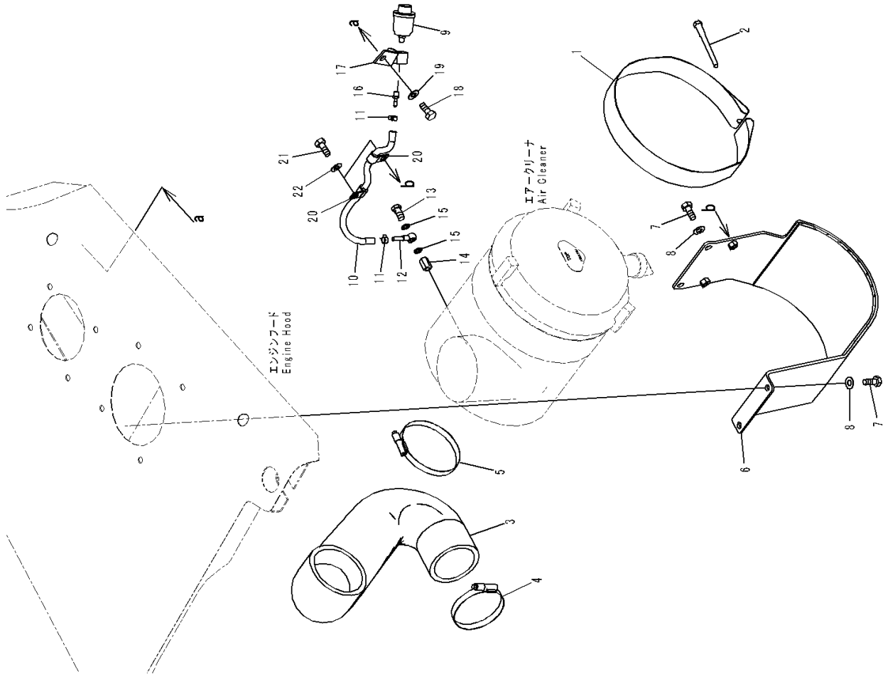
FIG. A1470-501003 Air Cleaner, Mounting
