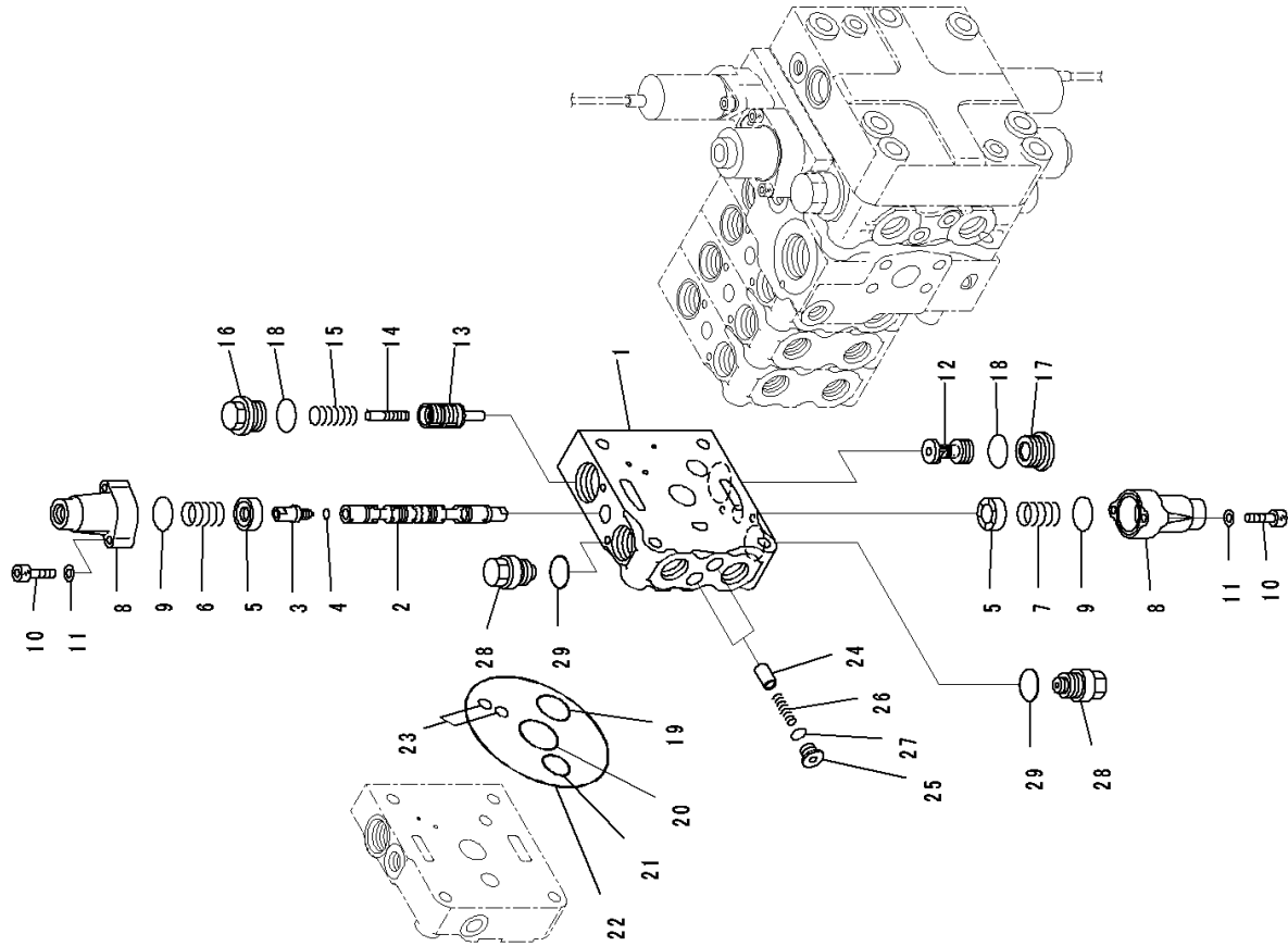
FIG. M2210-005008 Fender Group, Inner Parts (7/12)
