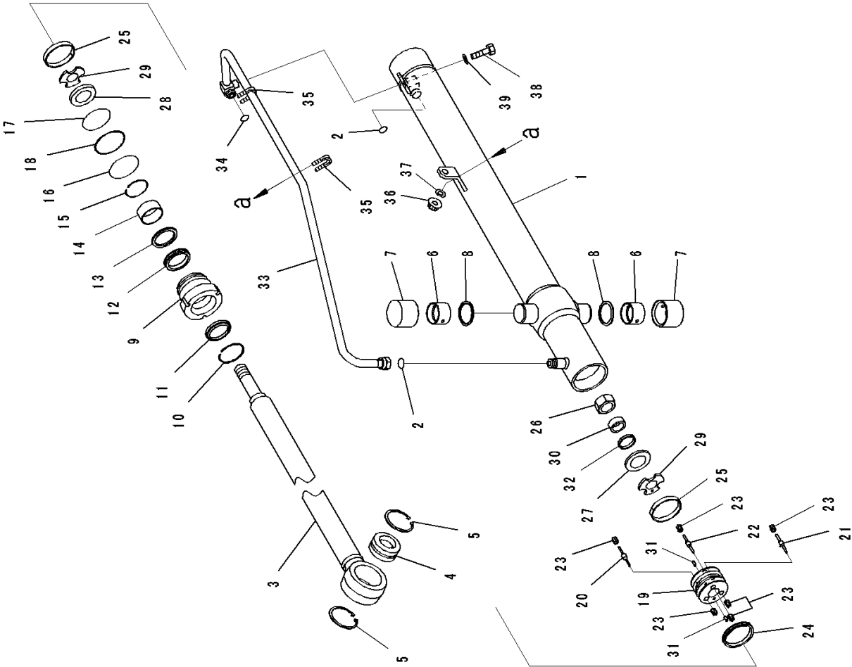
FIG. T2140-002002 Dozer Blade Lift Cylinder, With Power Angle Power Tilt Dozer, Inner Parts, Reduction Gear
