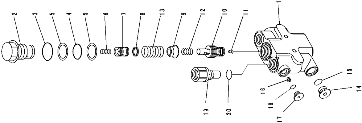
FIG. H2210-001002 Dozer Blade Lift Piping, Valve
