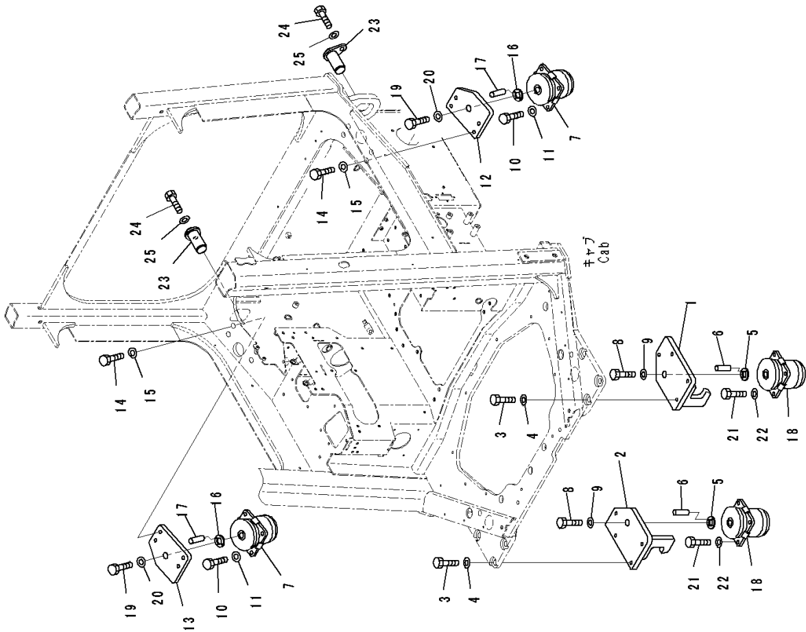
FIG. K2120-001001 Floor Frame Mounts
