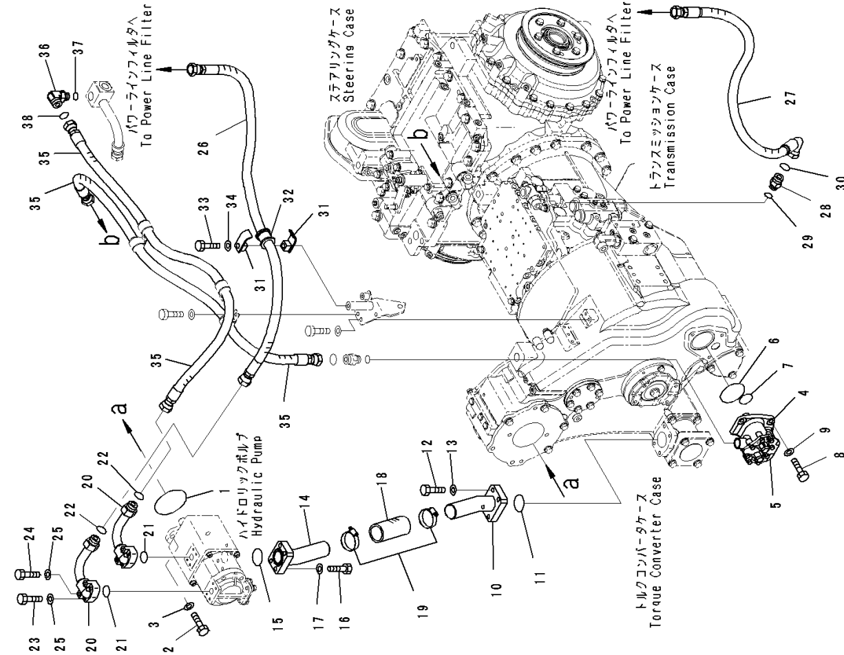
FIG. F2300-001029 Power Train, Power Train to Hydrostatic Tank Piping (1/2)
