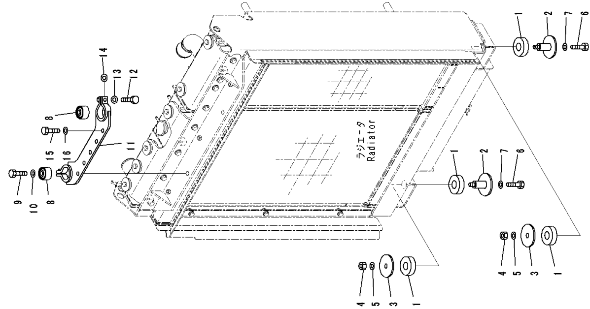
FIG. C0100-001009 Radiator, Mounting
