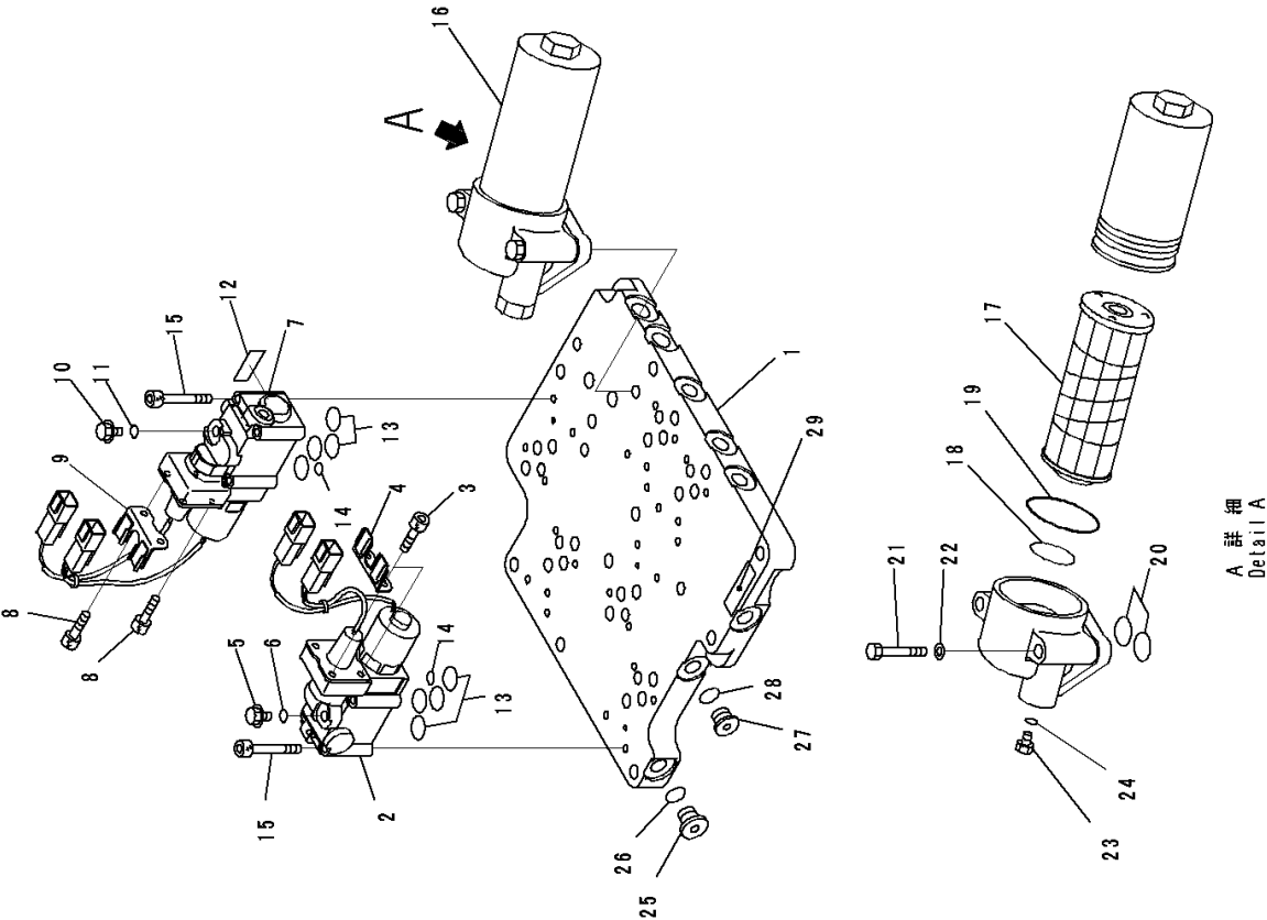
FIG. F2300-001016 Power Train, Transmission E.C.M.V. Valve
