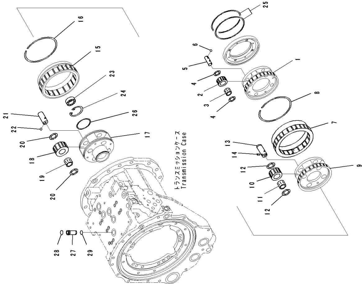
FIG. F2300-001013 Power Train, Transmission Carrier (2/2)
