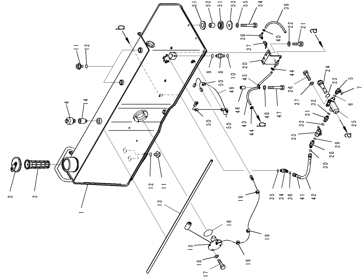
FIG. D0100-001001 Fuel Tank
