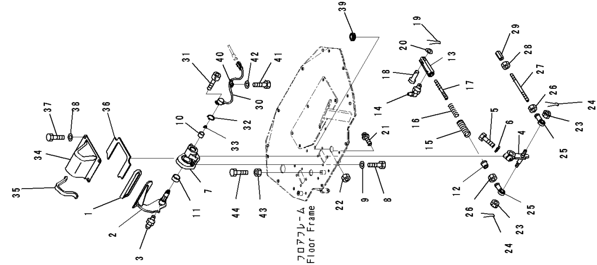
FIG. K0210-007037 ROPS Cab, Brake Pedal
