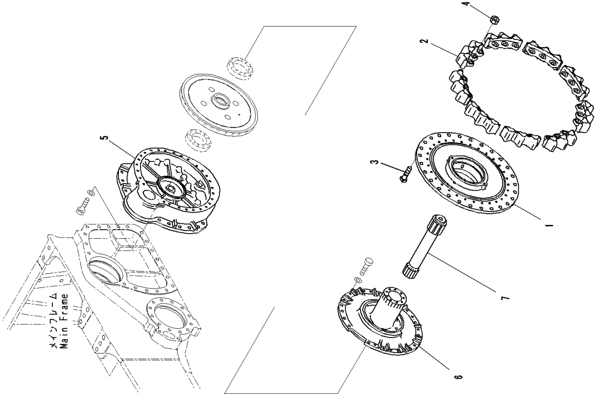
FIG. F2380-001003 Final Drive, Sprocket Hub, LHS
