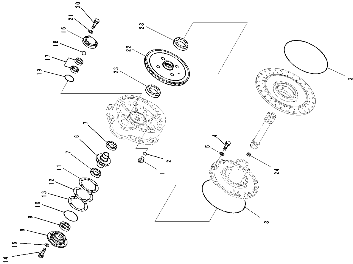
FIG. F2380-001001 Final Drive, Pinion and Gear, LHS
