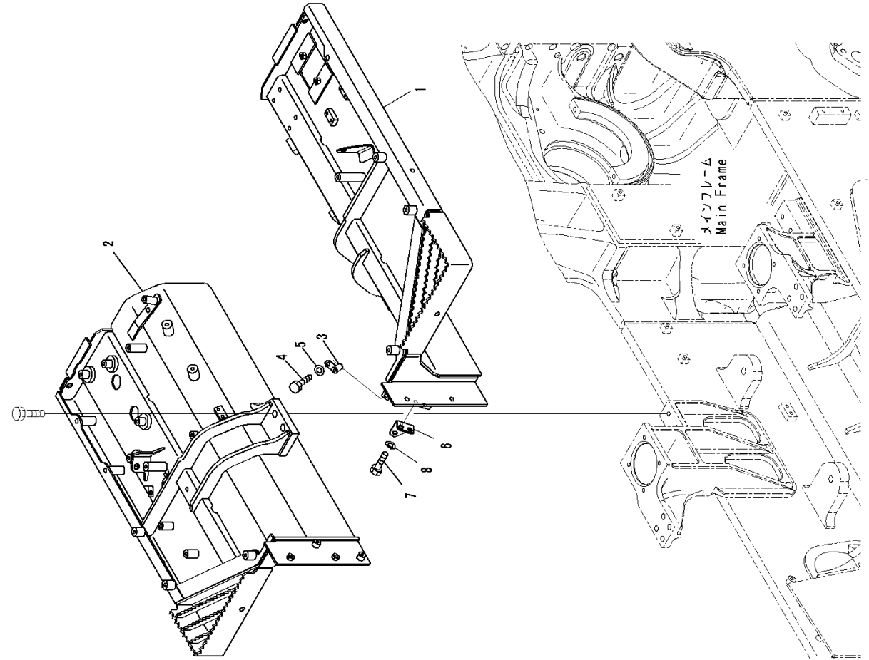
FIG. M2210-001001 Fender Group, Fender
