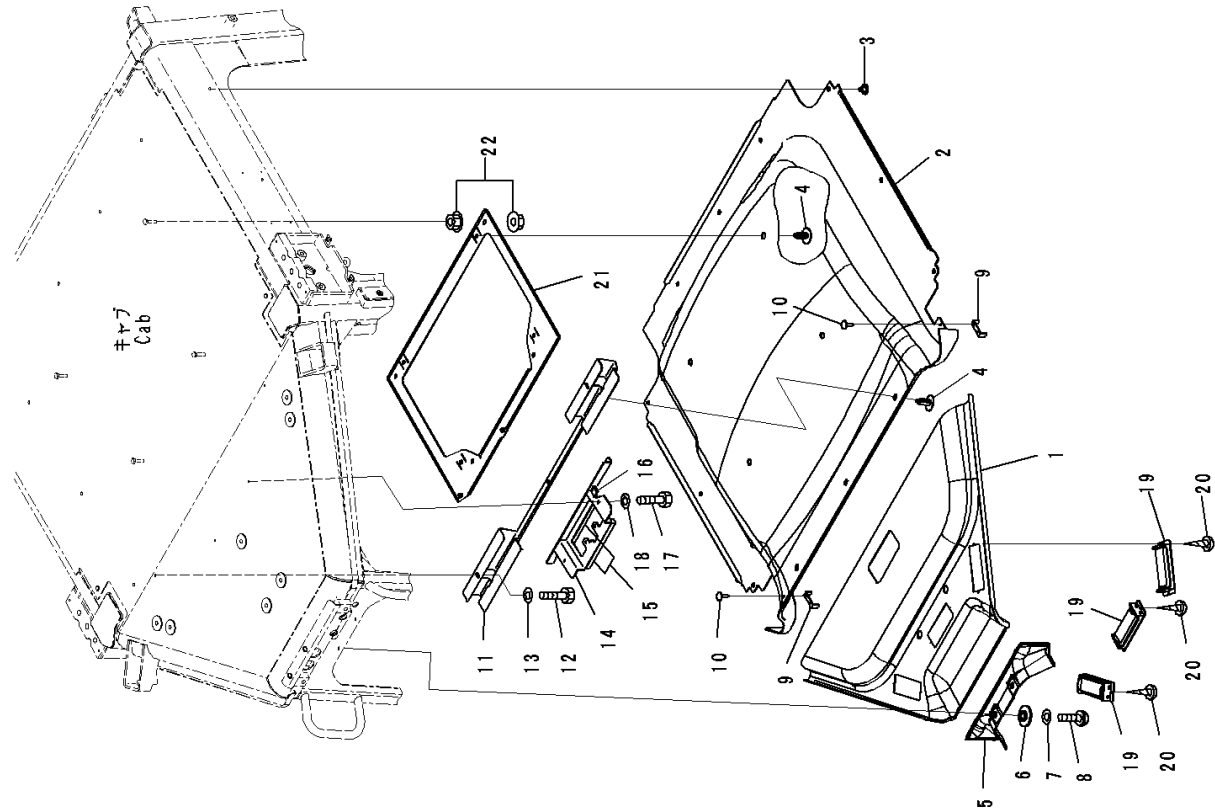
FIG. K0210-002020 ROPS Cab, Roof Cover (1/2)
