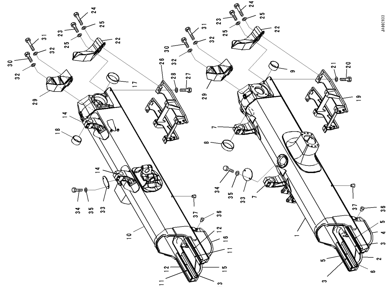
FIG. R2100-003001 Track Frame, Plus Type
