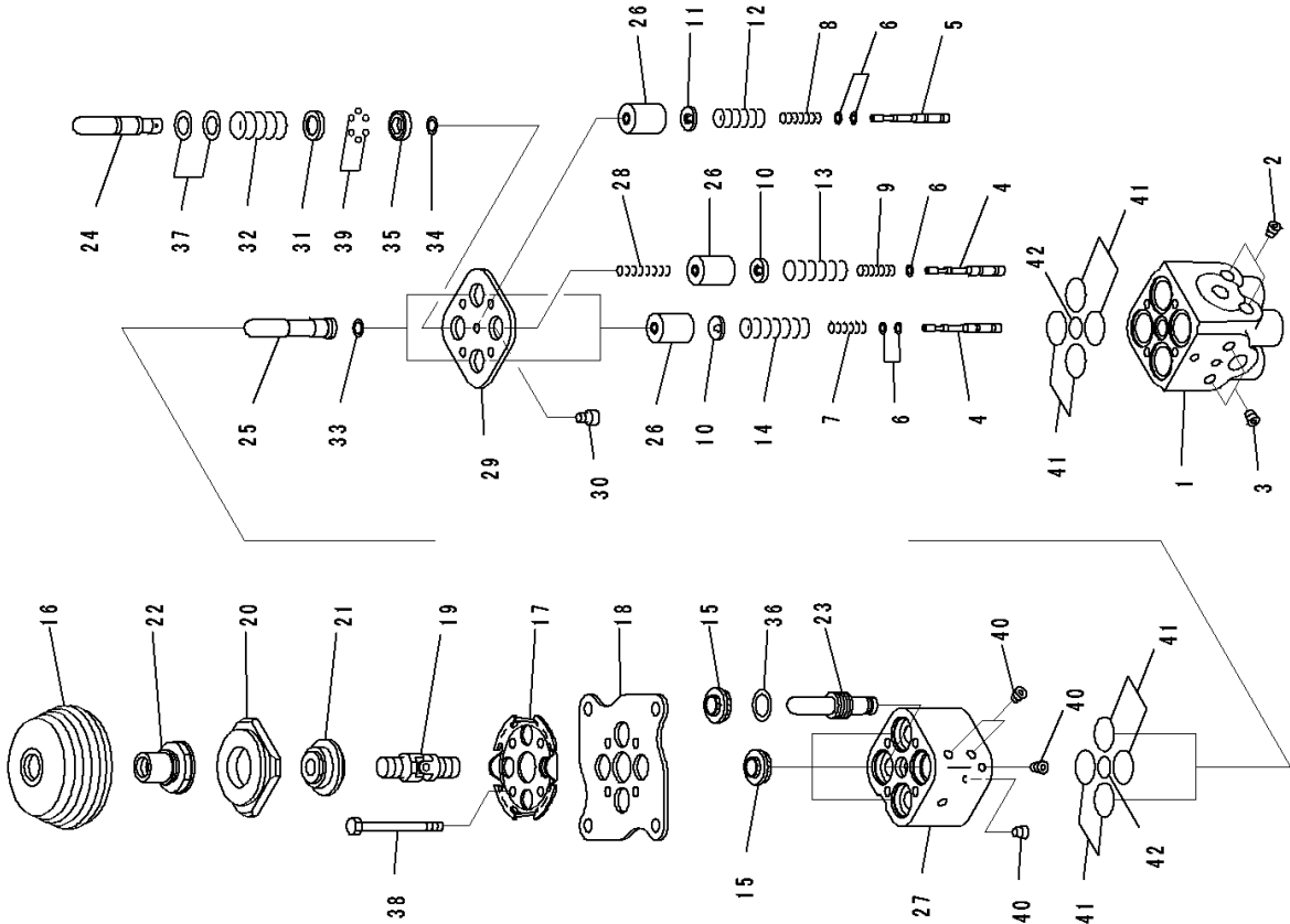
FIG. K2110-001003 Dozer Control, PPC Valve for Blade
