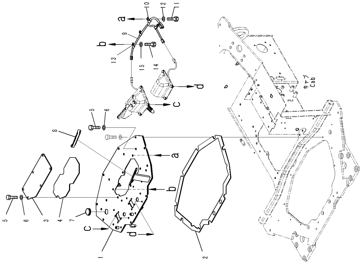
FIG. K0210-002036A ROPS Cab, Floor Frame Inside Cover
