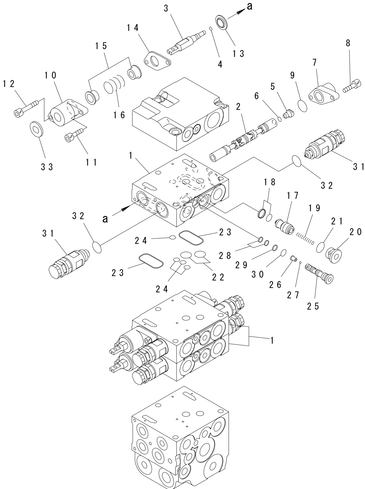
FIG. R4140-85A0 CONTROL VALVE (5-SPOOL) (5/5) (WITH 3,4,5 PORT RELIEF VALVE) (INNER PARTS)
