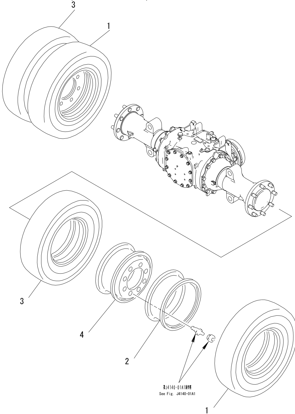
FIG. J4110-21A4 FRONT WHEEL (DOUBLE TIRE) (7.00-15) (ELASTIC CUSHION) (J-LUG) (FOR COMPACT TYPE)
