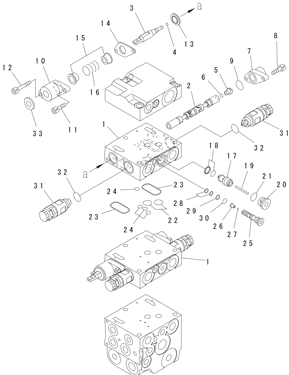
FIG. R4140-75A0 CONTROL VALVE (4-SPOOL) (5/5) (WITH 3,4 PORT RELIEF VALVE) (INNER PARTS)
