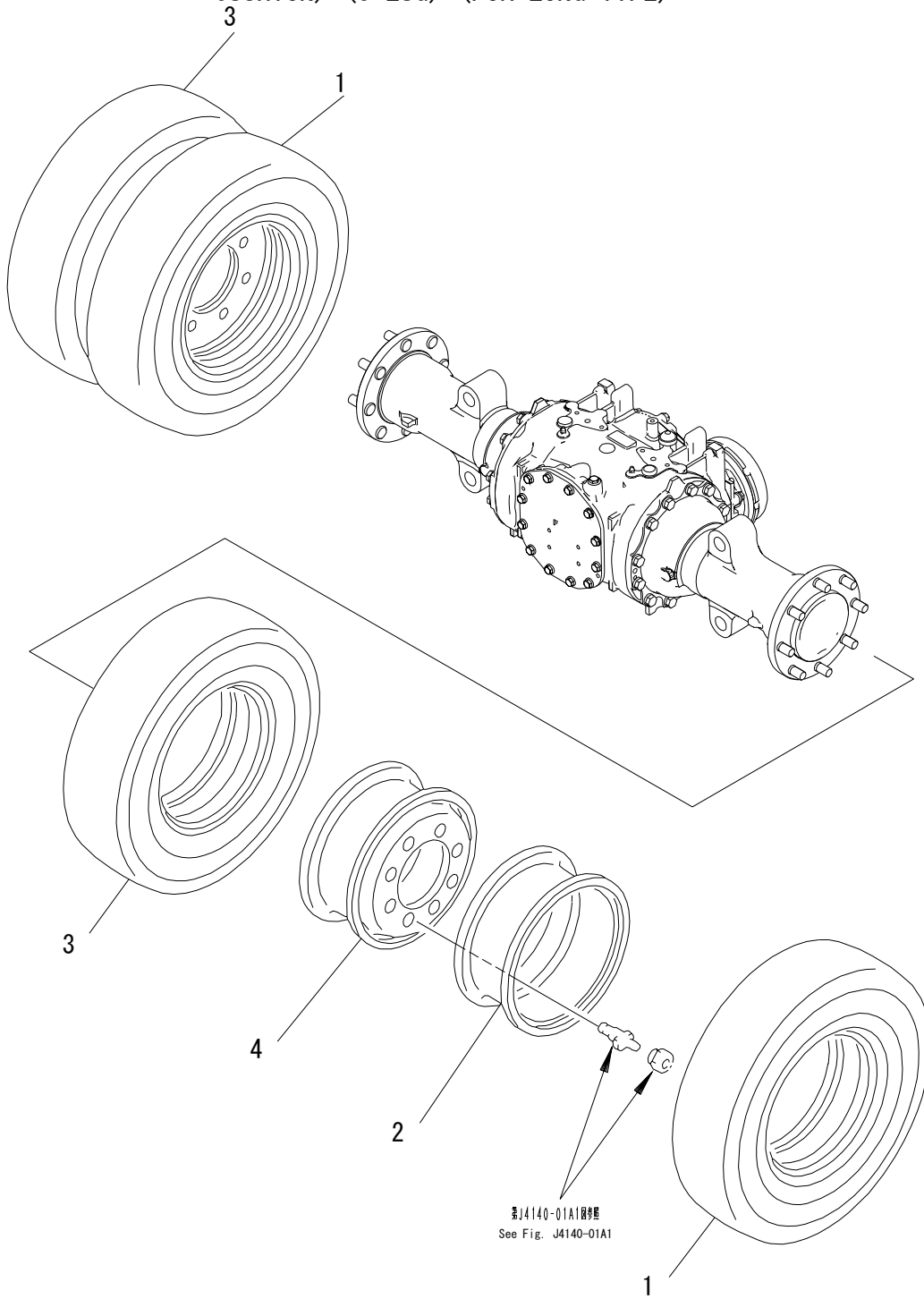
FIG. J4110-21A6 FRONT WHEEL (DOUBLE TIRE) (SINGLE SIZE) (8.25-15) (ELASTIC CUSHION) (J-LUG) (FOR LONG TYPE)
