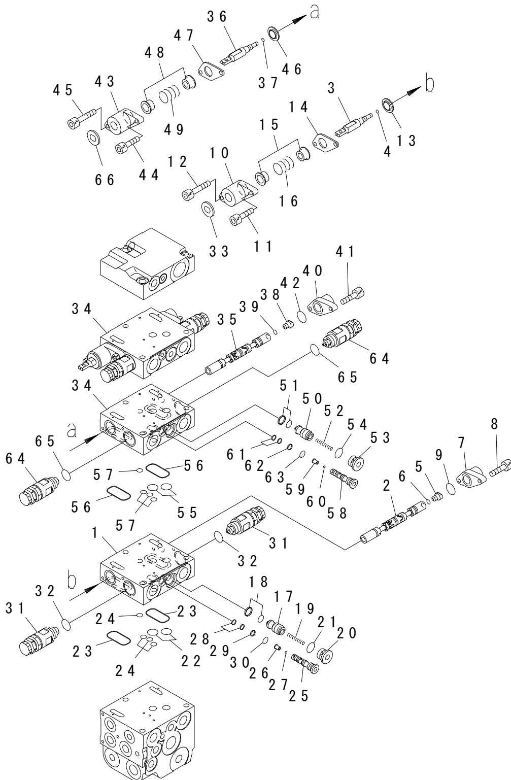
FIG. R4140-85A1 CONTROL VALVE (5-SPOOL) (5/5) (WITH 5 PORT RELIEF VALVE) (INNER PARTS)
