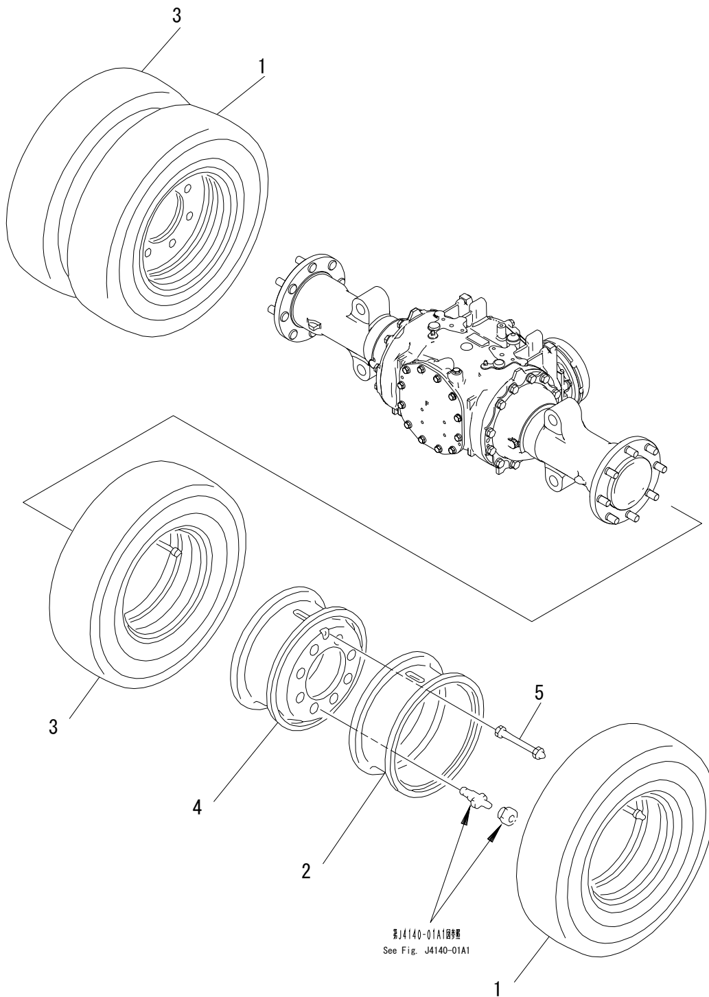
FIG. J4110-21A0 FRONT WHEEL (DOUBLE TIRE) (7.00-15-10PR) (J-LUG) (FOR COMPACT TYPE)
