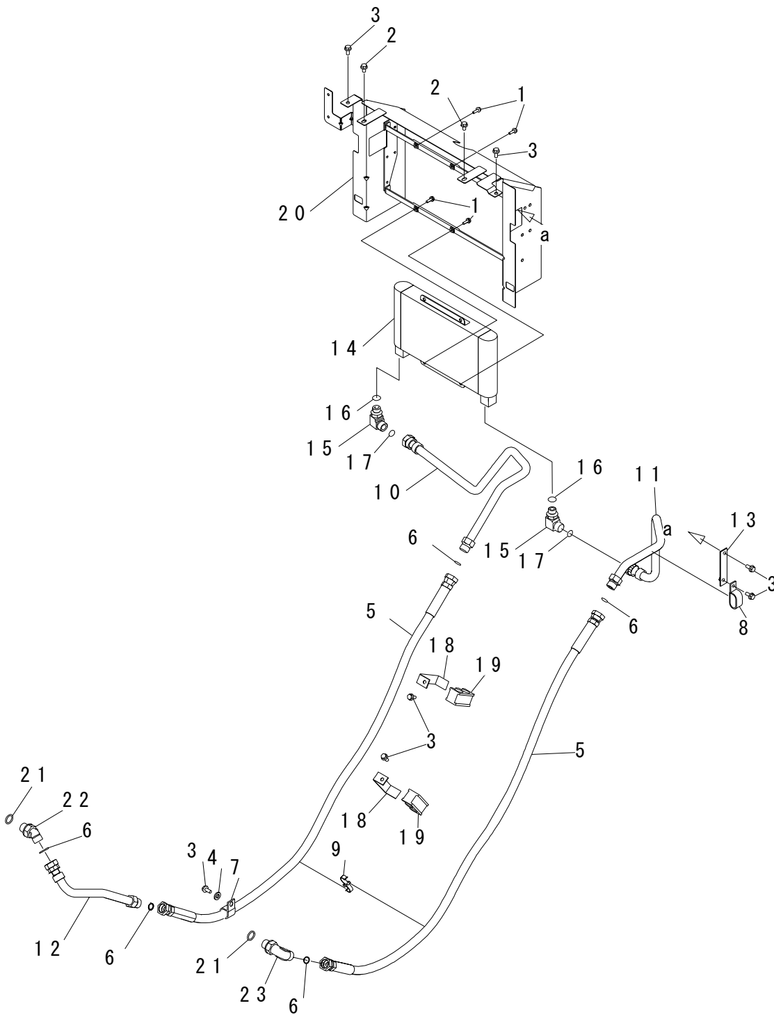
FIG. C4140-01A1 TORQUE CONVERTER COOLER PIPING
