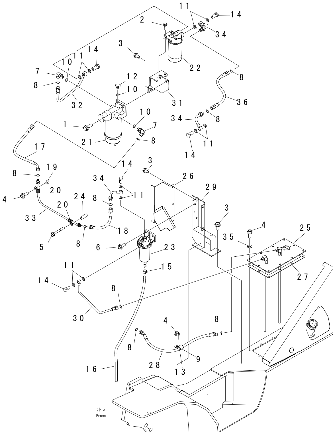
FIG. D4110-11A0 FUEL SYSTEM (ADDITIONAL FUEL FILTER)
