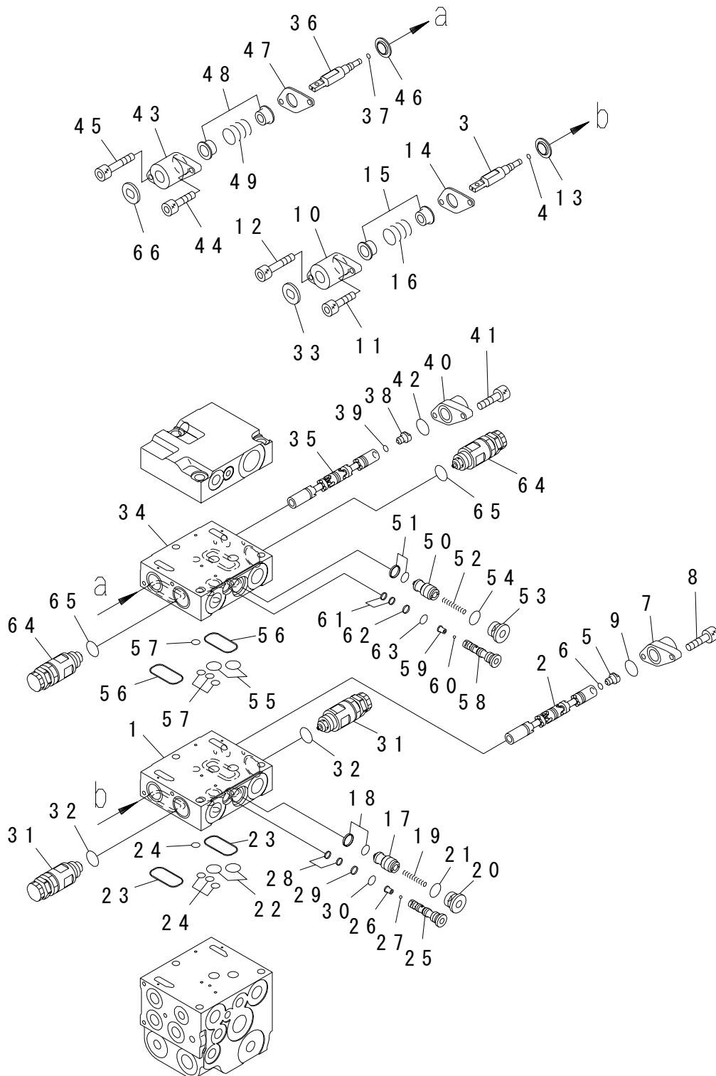
FIG. R4140-75A1 CONTROL VALVE (4-SPOOL) (5/5) (WITH 4 PORT RELIEF VALVE) (INNER PARTS)
