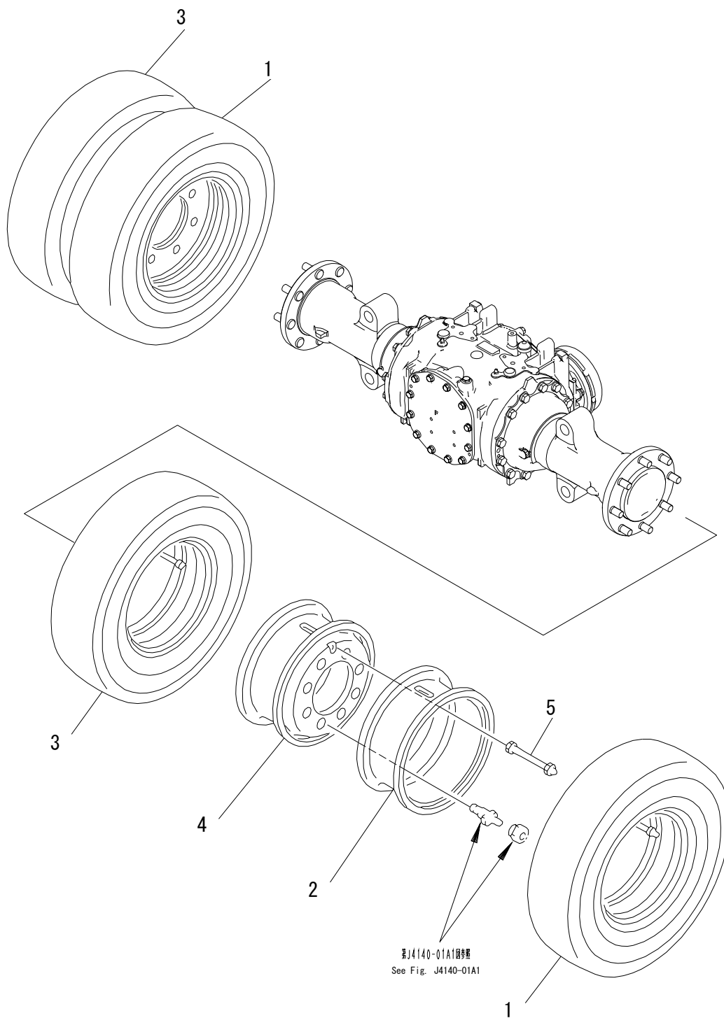
FIG. J4110-21A3 FRONT WHEEL (DOUBLE TIRE) (8.25-15-12PR) (STEEL) (FOR LONG TYPE)
