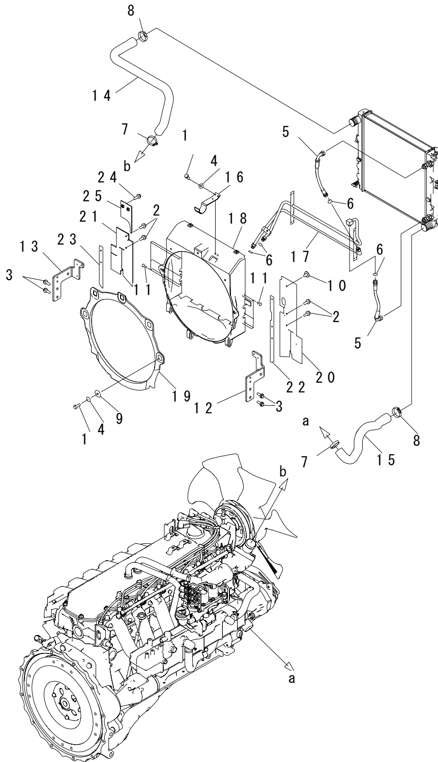
FIG. C4130-01A1 RADIATOR PIPING
