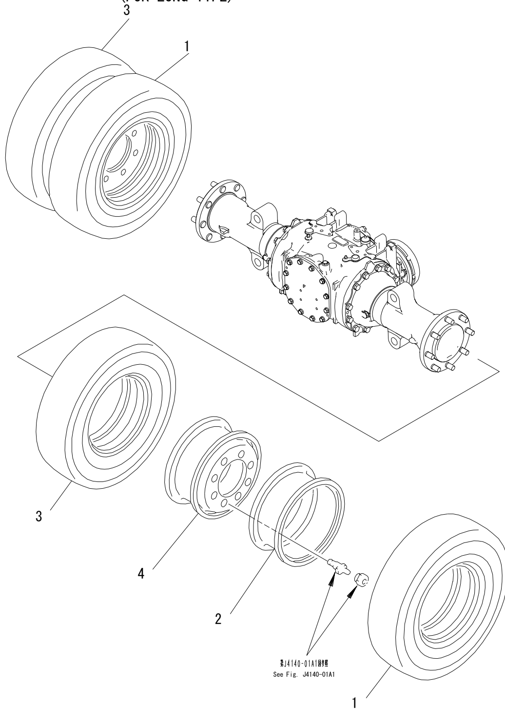
FIG. J4110-21A5 FRONT WHEEL (DOUBLE TIRE) (7.50-16) (ELASTIC CUSHION) (J-LUG)
