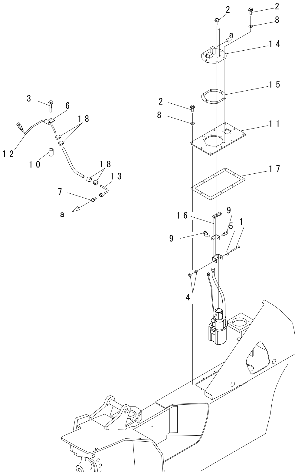
FIG. D4110-01A1 FUEL SYSTEM
