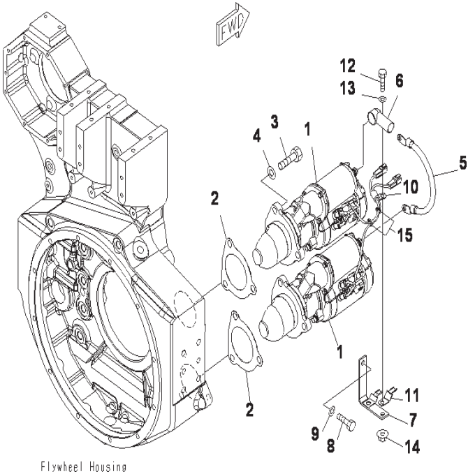
Flywheel Housing
