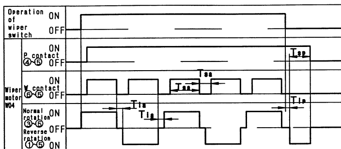
Timing chart (when wiper switch is ON)
