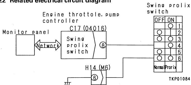
M-22 Related electrical circuit diagram
