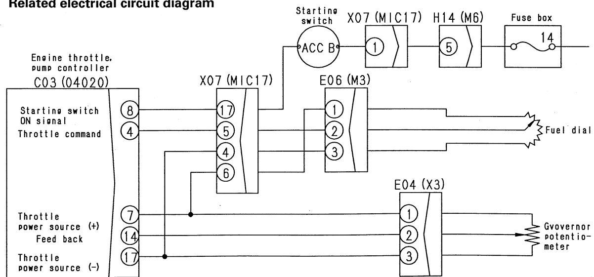
E-10 Related electrical circuit diagram
