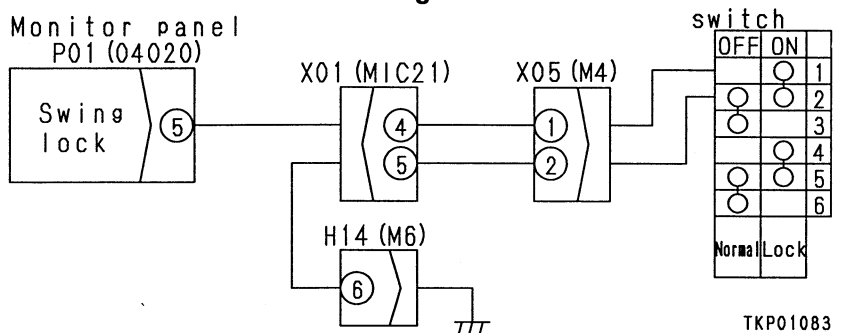
M-21 Related electrical circuit diagram
