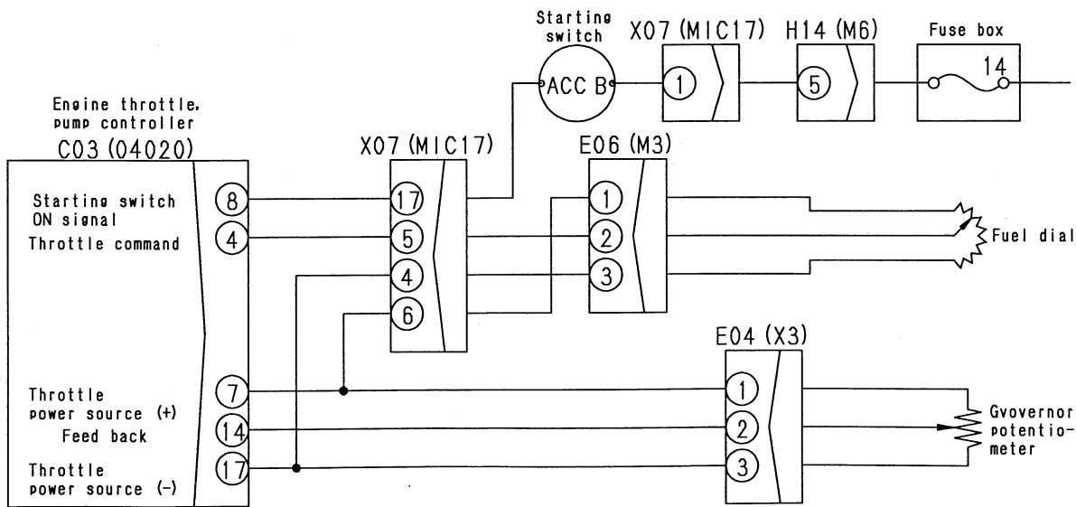
E-9 Related electrical circuit diagram
