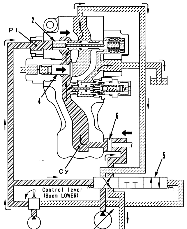
To control valve SWP04675
