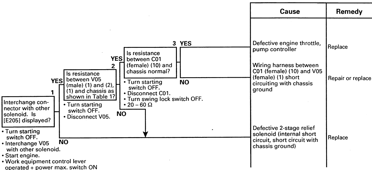
Between V05 (male) (1) and (2) 20 – 60 \Omega Between V05 (male) (1) and chassis Min. 1 M \Omega
