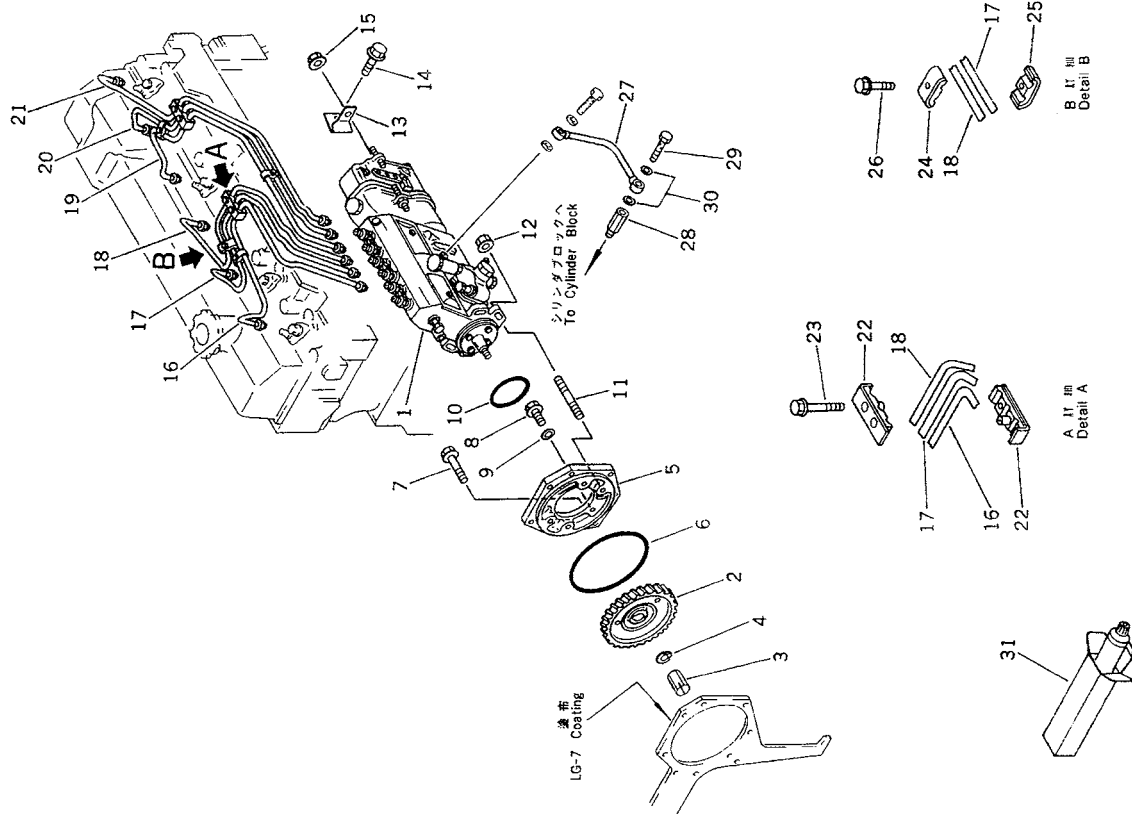
FIG. 0401 FUEL INJECTION PUMP AND PIPING
