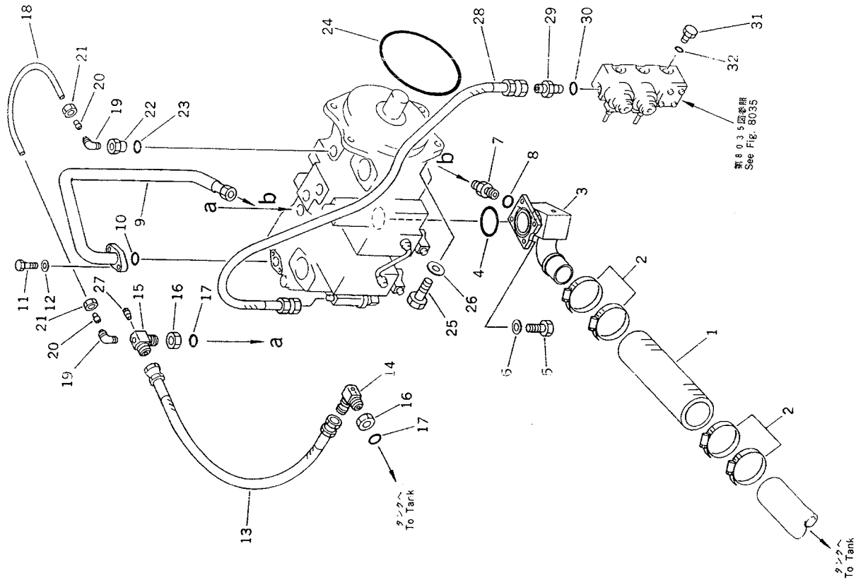
FIG. 8033 HYDRAULIC PIPING (TANK TO PUMP) (TBG SPEC.)
