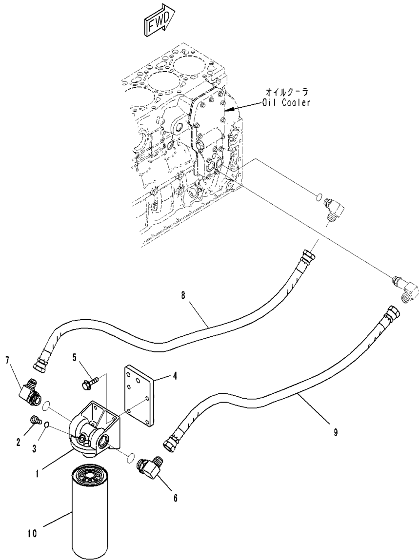
FIG. ALF00-001001 Engine Oil Filter and Piping
