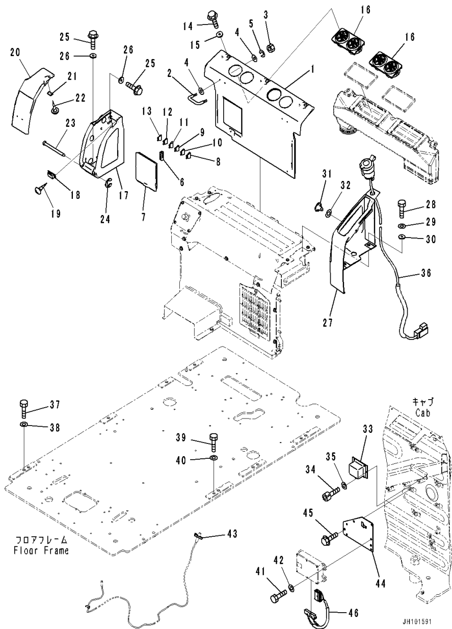
FIG. K1110-001026 Cab (Cab In Parts, Rear Cover, With 12V Converter)
