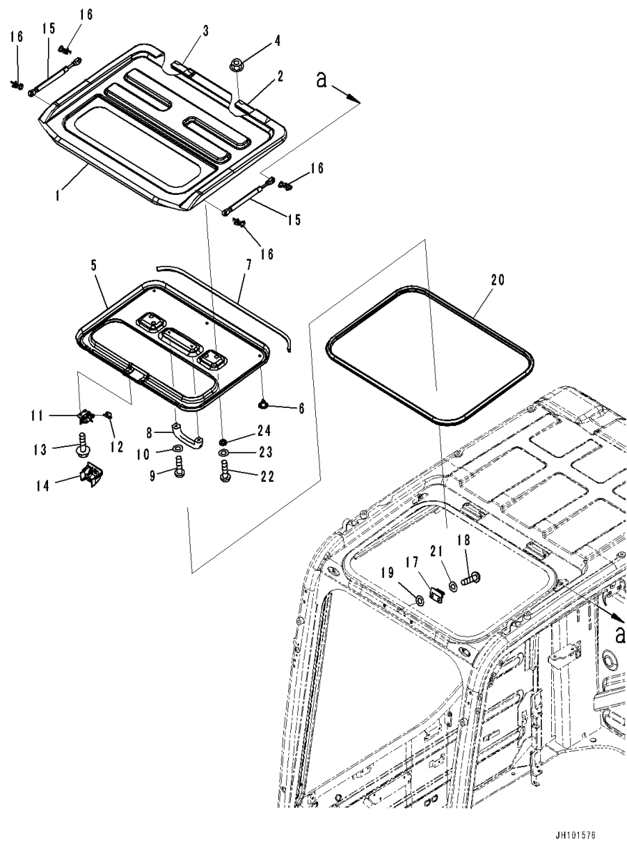
FIG. K1110-001004 Cab (Roof Ventilator)
