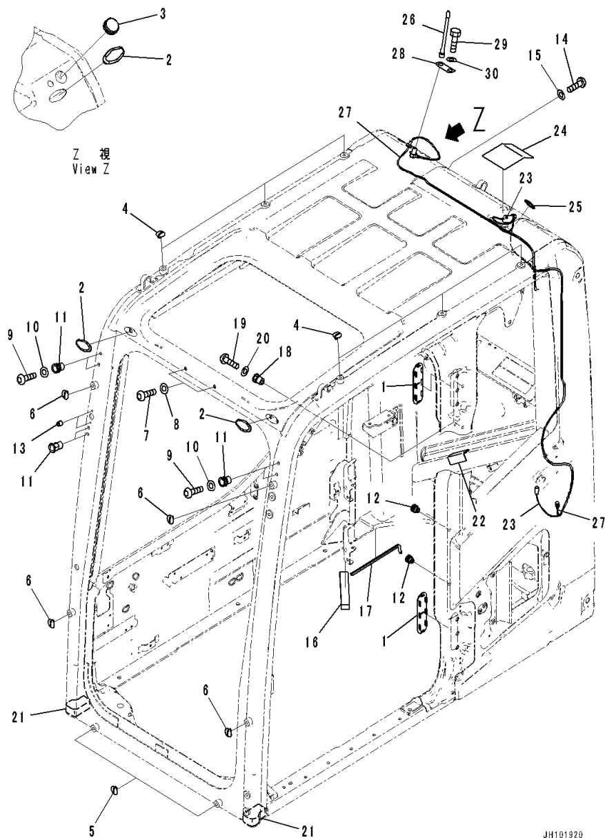
FIG. K1110-002013 Cab (With KOMTRAX) (KOMTRAX Antenna, With KOMTRAX)
