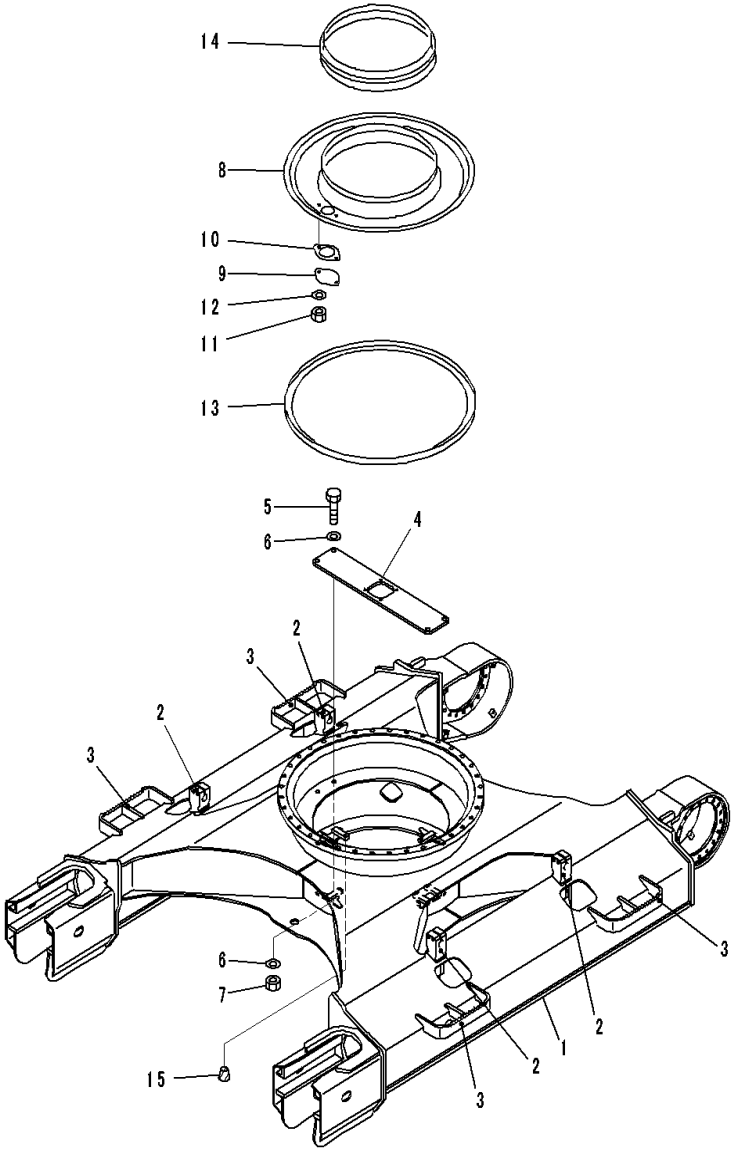
FIG. R1100-003001 Track Frame (Link, 6 Type, For LC)
