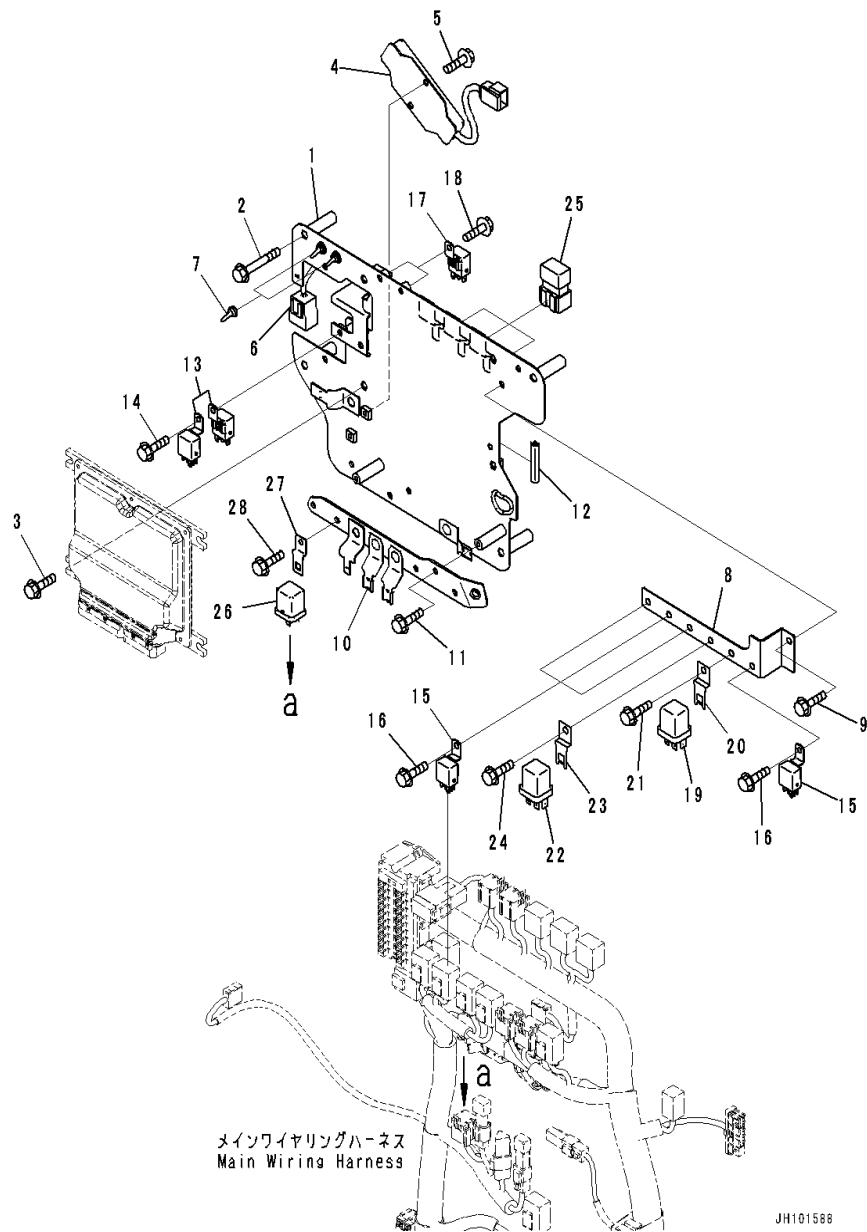
FIG. K1110-001023 Cab (Cab In Parts, Pump Controller and Relay)
