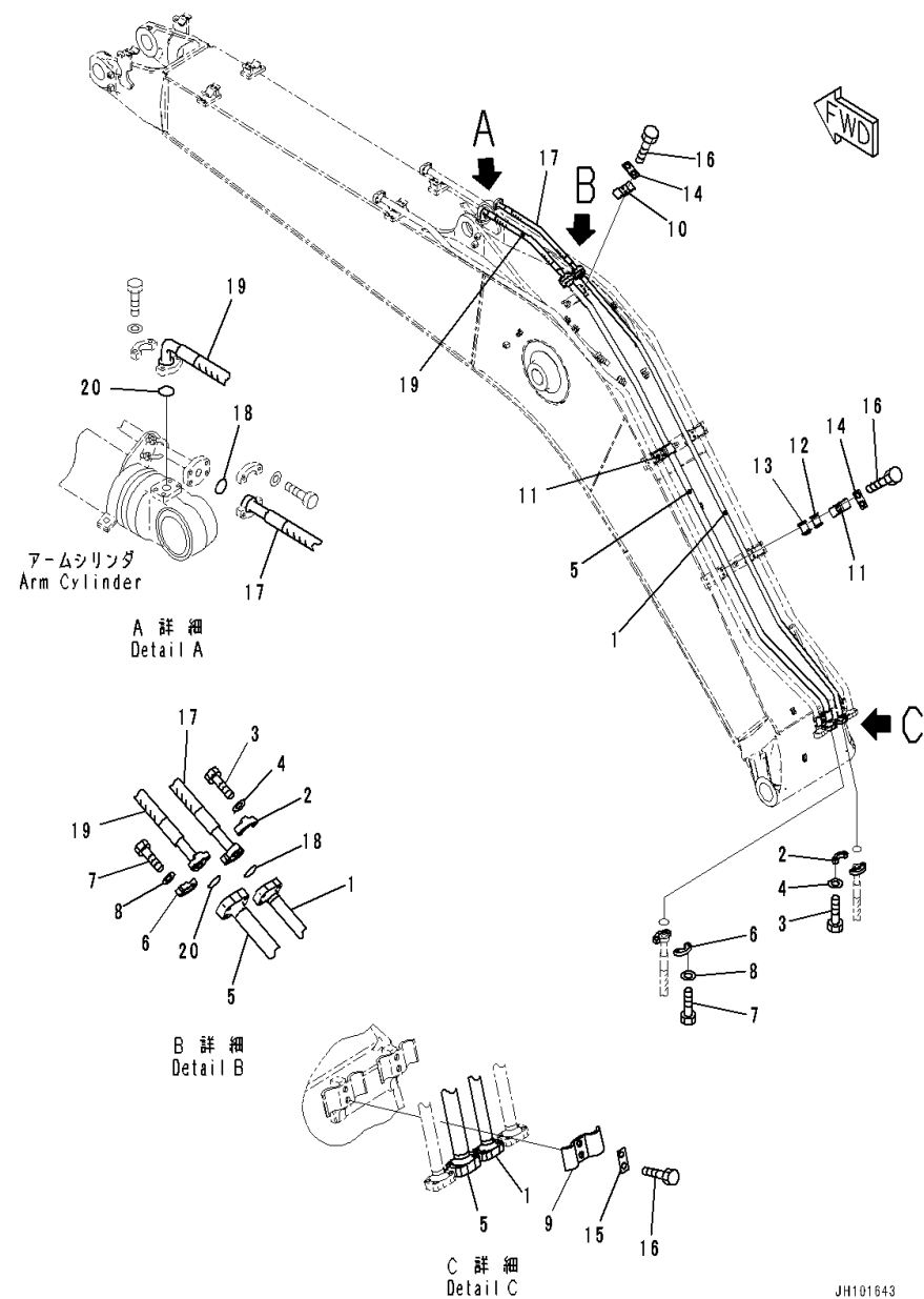
FIG. T1110-002003 Boom (Arm Cylinder Piping)
