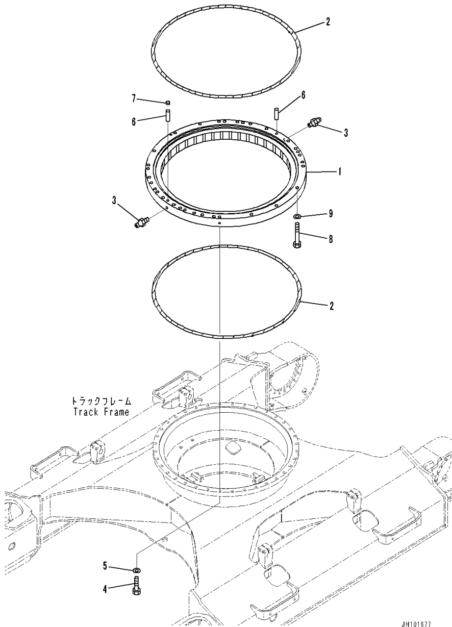
FIG. N1110-001001 Swing Circle (For Asia)
