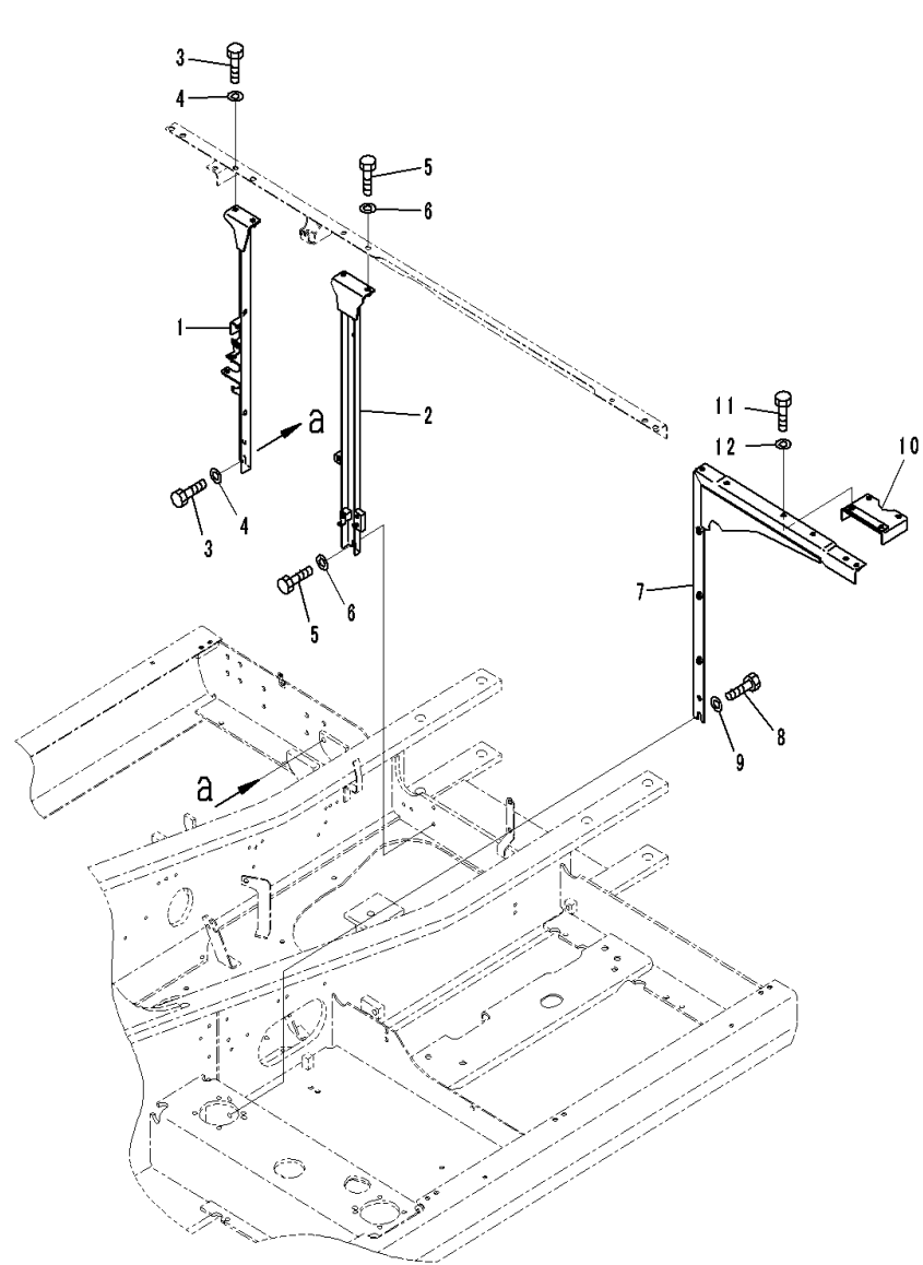
FIG. M1120-002001 Frame (With Pre-cleaner)
