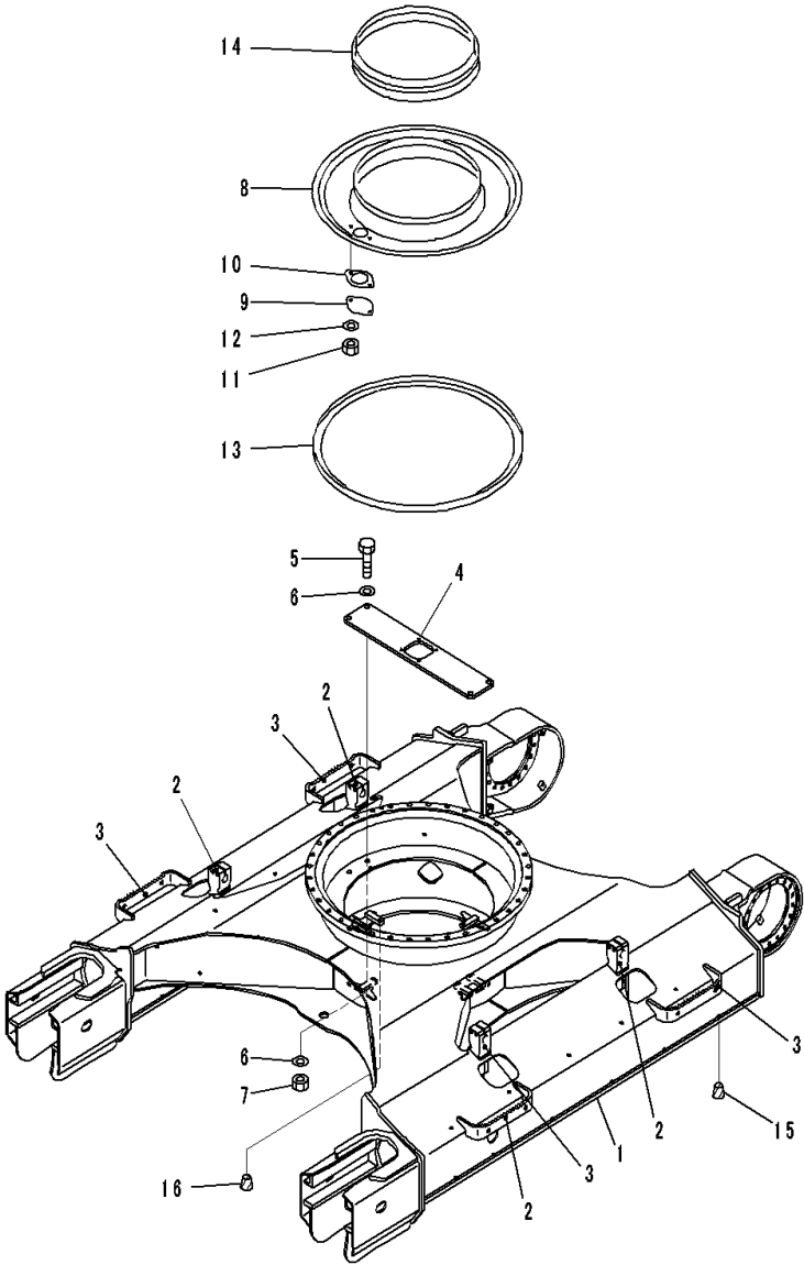
FIG. R1100-002001 Track Frame (Link, 7 Type)
