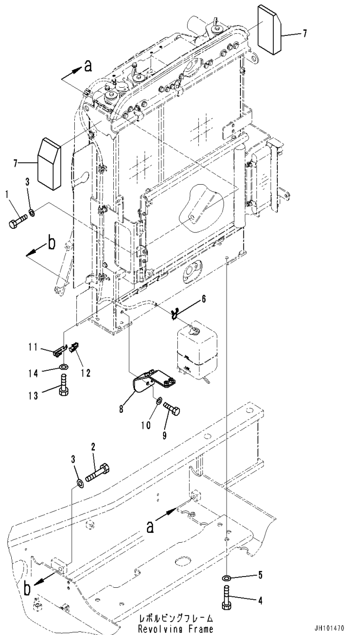
FIG. C0100-001011 Cooling System (Related Parts)
