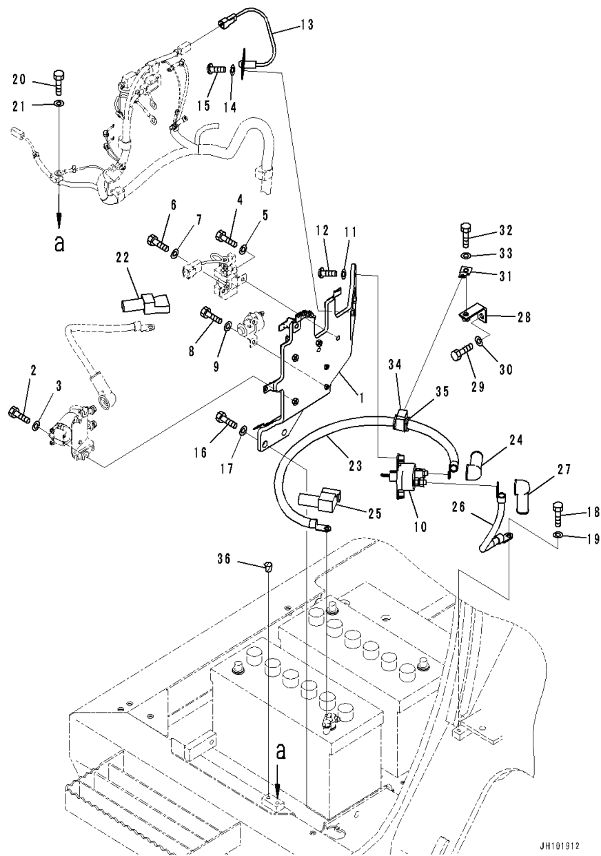
FIG. E0210-001001 Battery Electric Wiring Harness (With Battery Disconnect Switch)
