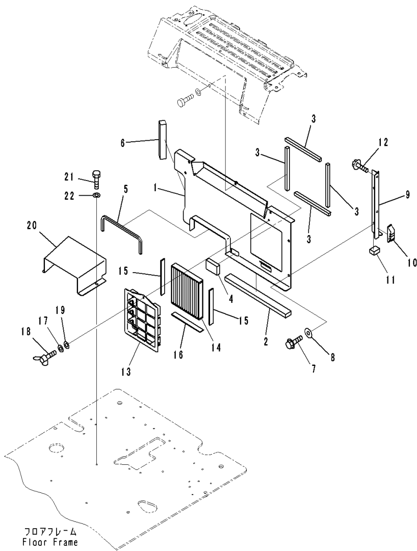
FIG. K1110-001022 Cab (Cab In Parts, Partition and Recirculation Air Filter)
