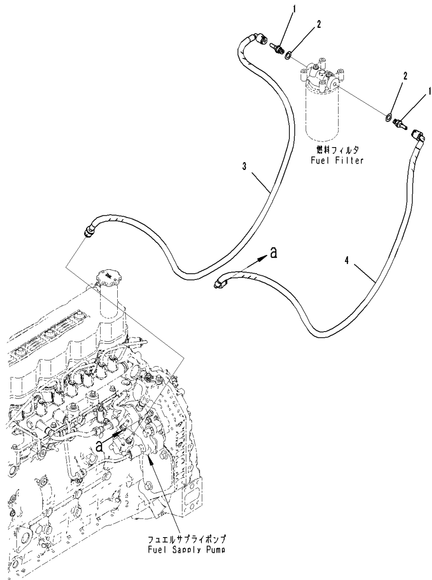
FIG. AFF20-001001 Fuel Filter Piping
