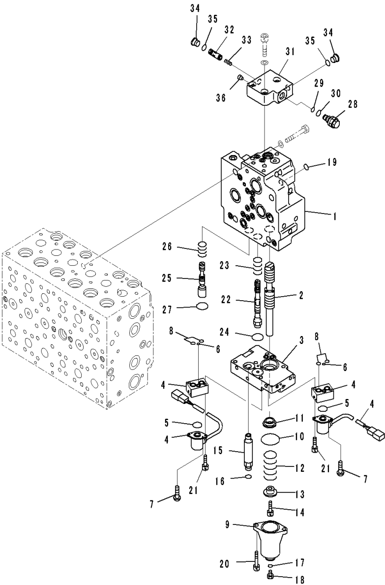
FIG. H0120-002013 Control Valve (7-Spool, 13/21)
