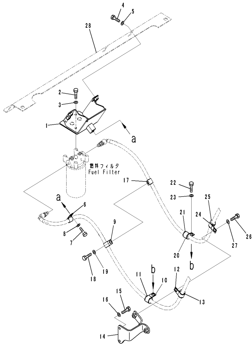
FIG. D0200-002007 Fuel Supply Piping (Fuel Filter Bracket)
