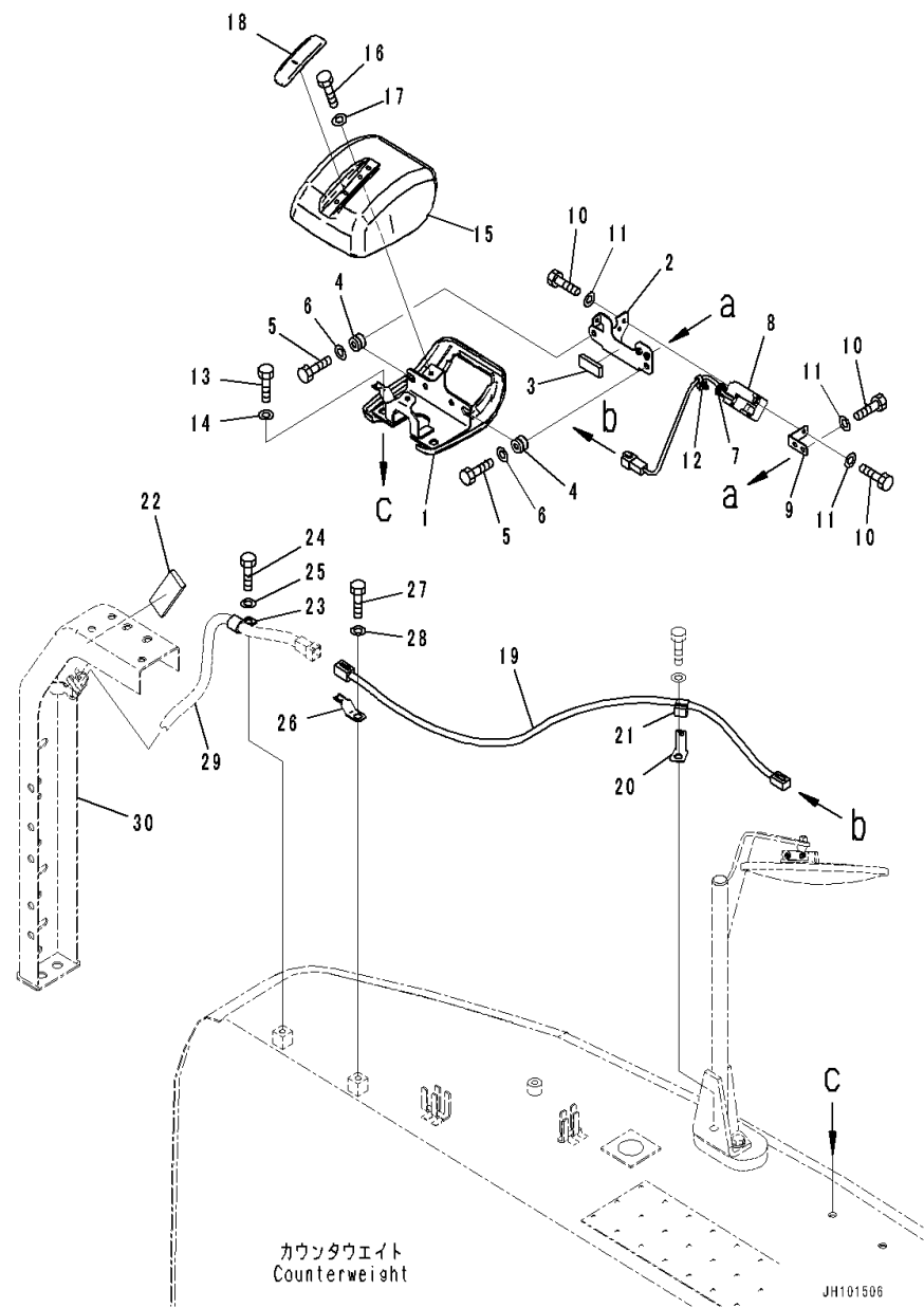
FIG. E0450-001001 Rearview Camera
