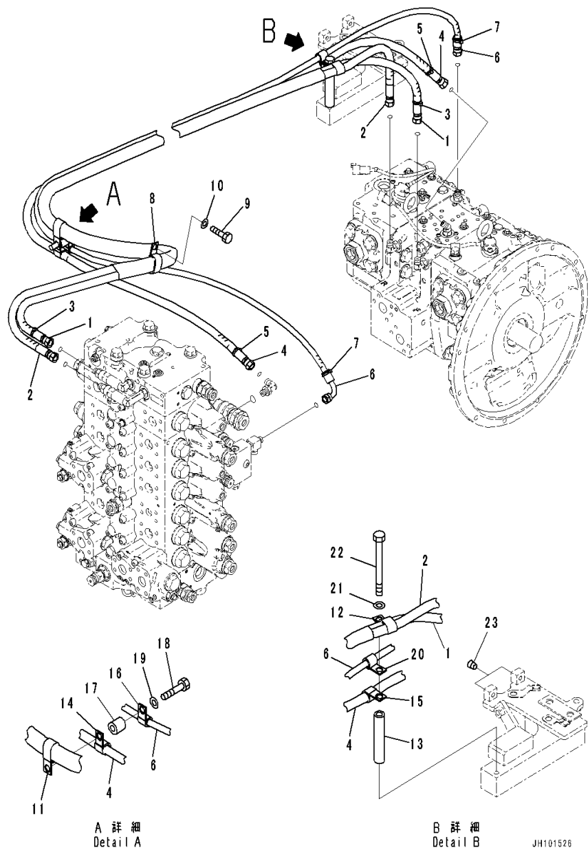
FIG. H1810-001001 LS Piping
