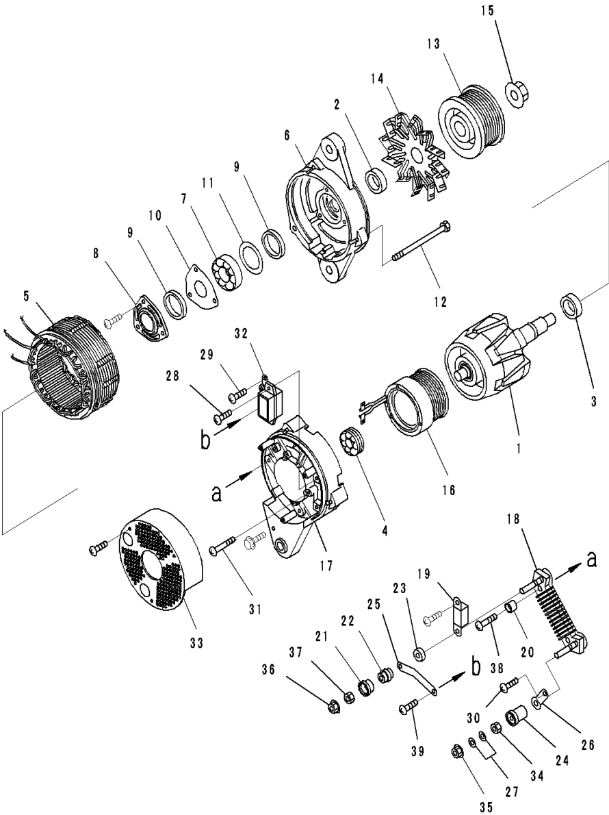
FIG. A6020-001001 Alternator Mounting (For 60Amp.Brushless,China 3rd EX-Gas Regulation) (Inner Parts)
