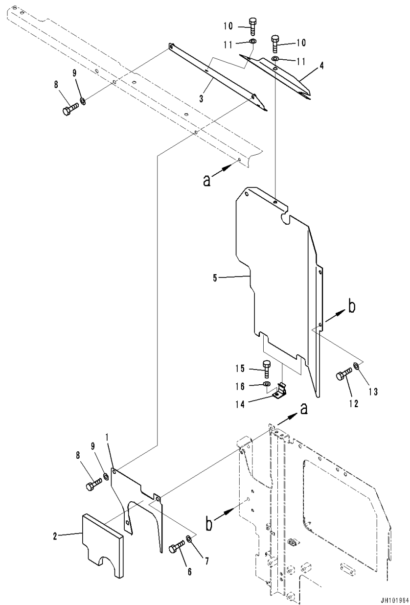
FIG. M1150-002002 Partition (With Pre-cleaner)
