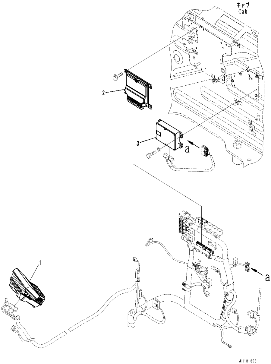
FIG. K1110-002027 Cab (With KOMTRAX) (Controller and Monitor, With KOMTRAX)
