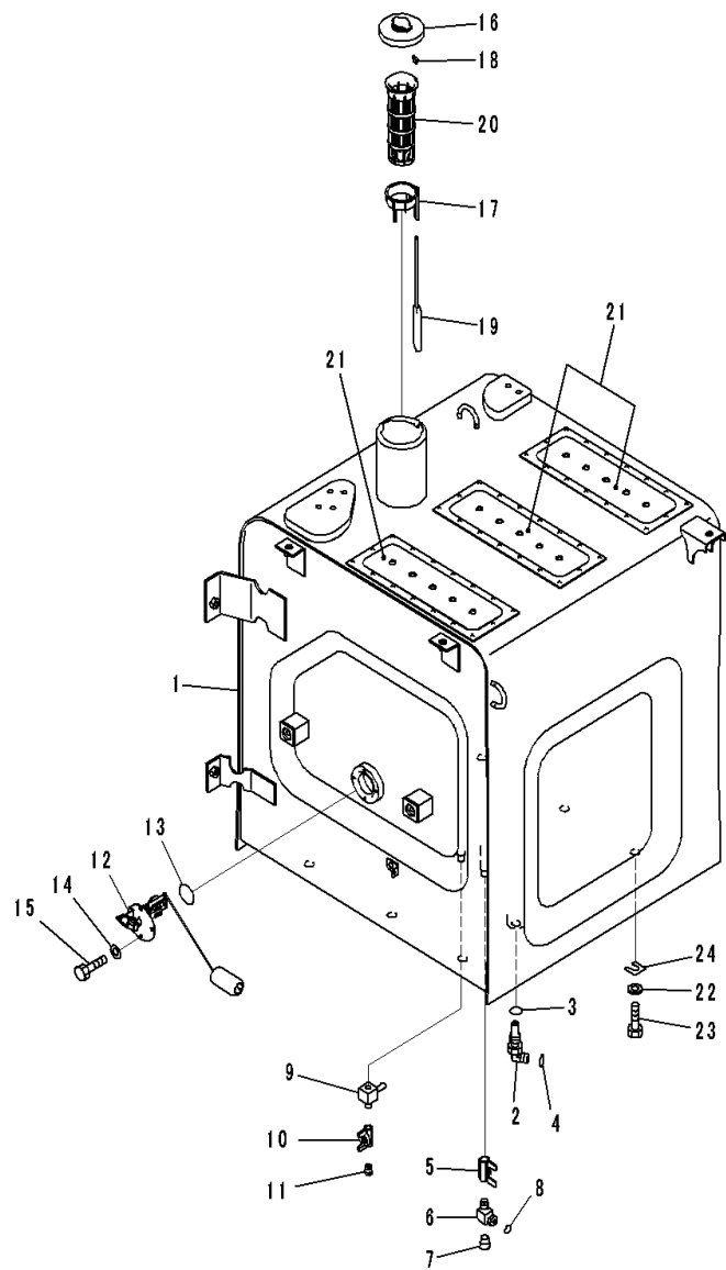
FIG. D0100-001001 Fuel Tank
