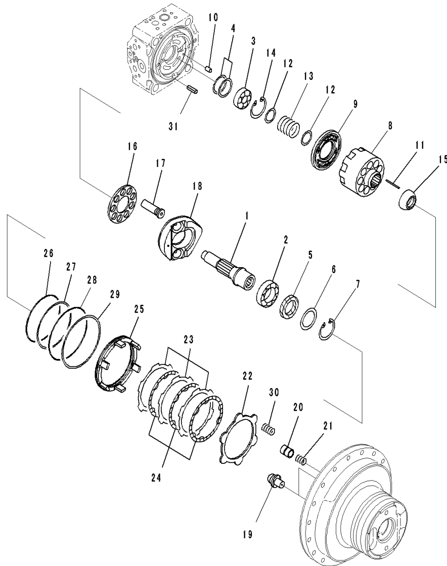
FIG. P1210-001005 Travel Motor and Final Drive (Travel Motor, R.H., 2/2)
