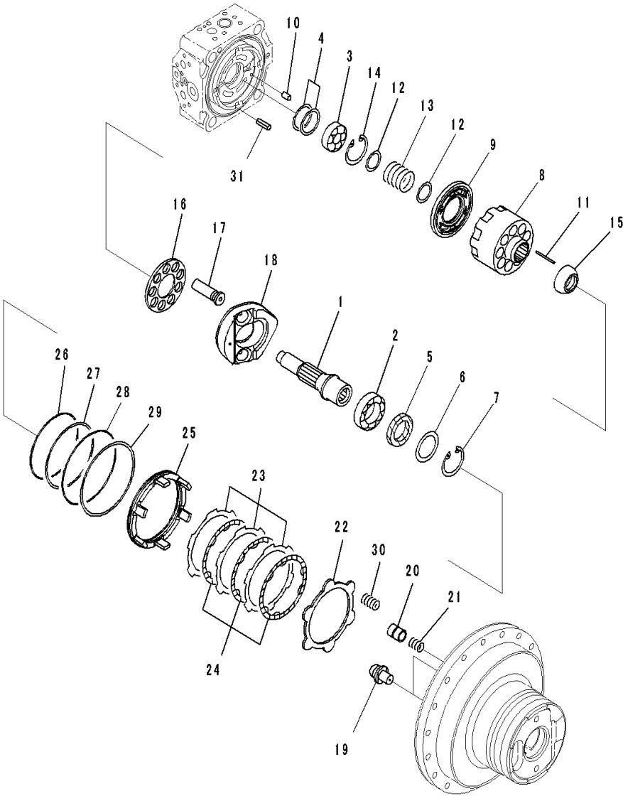
FIG. P1210-001002 Travel Motor and Final Drive (Travel Motor, L.H., 2/2)
