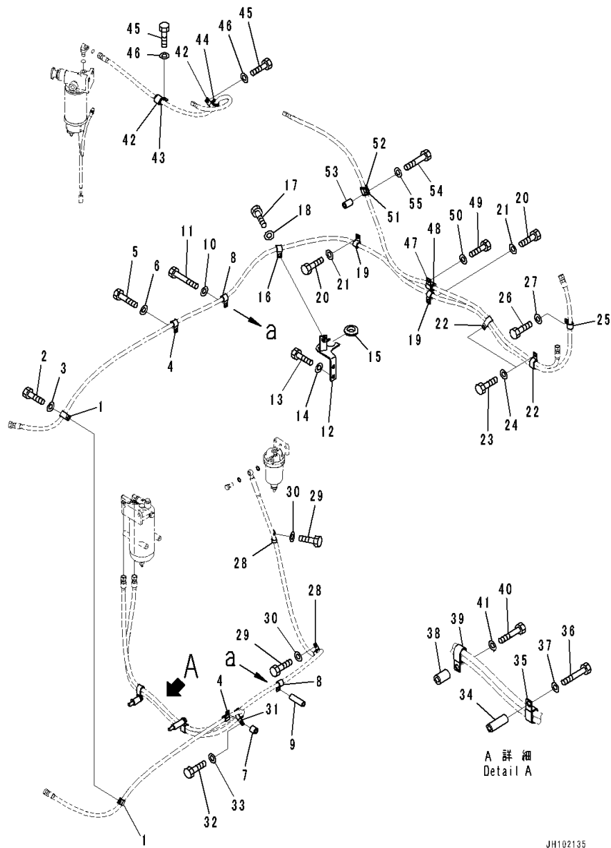
FIG. D0200-002008 Fuel Supply Piping (For Additional Fuel Prefilter) (Clip)
