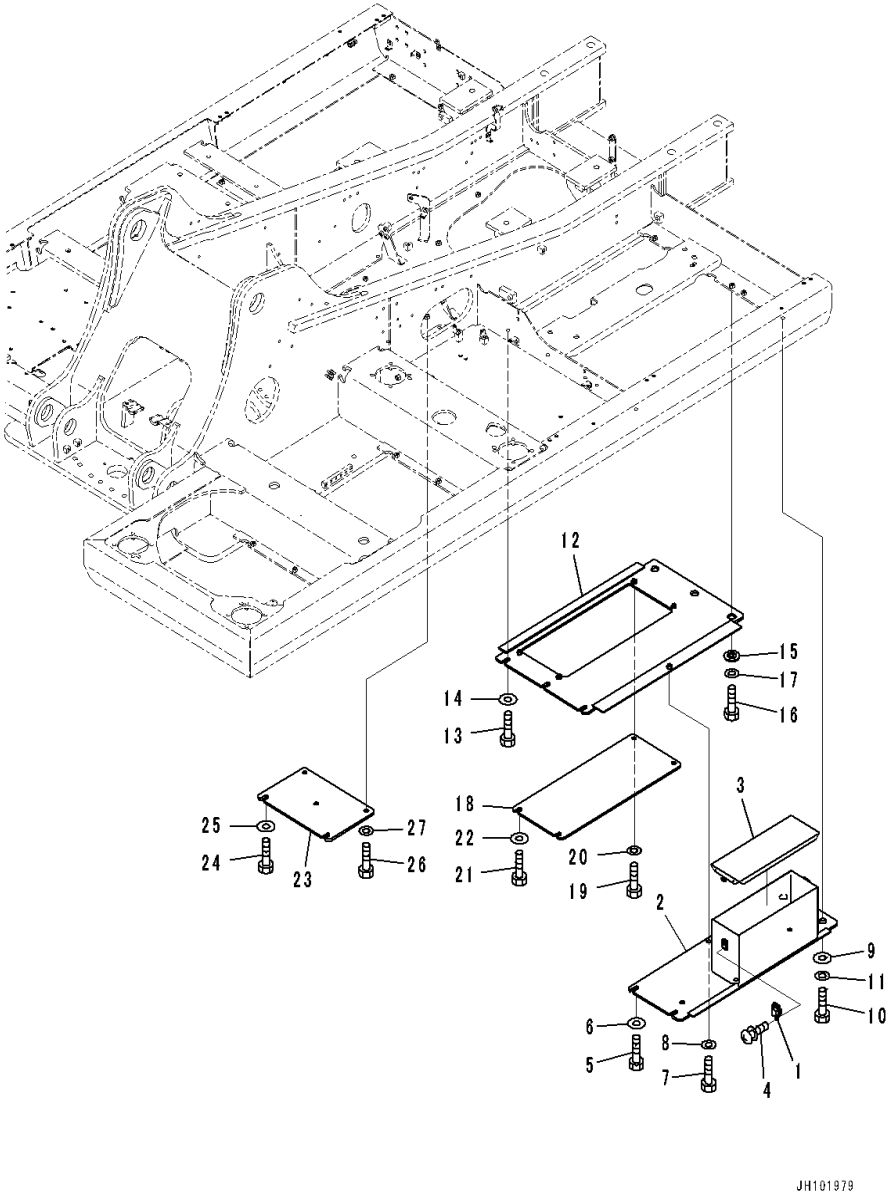
FIG. M1810-002002 Under Cover (Heavy Duty Type) (2/2)
