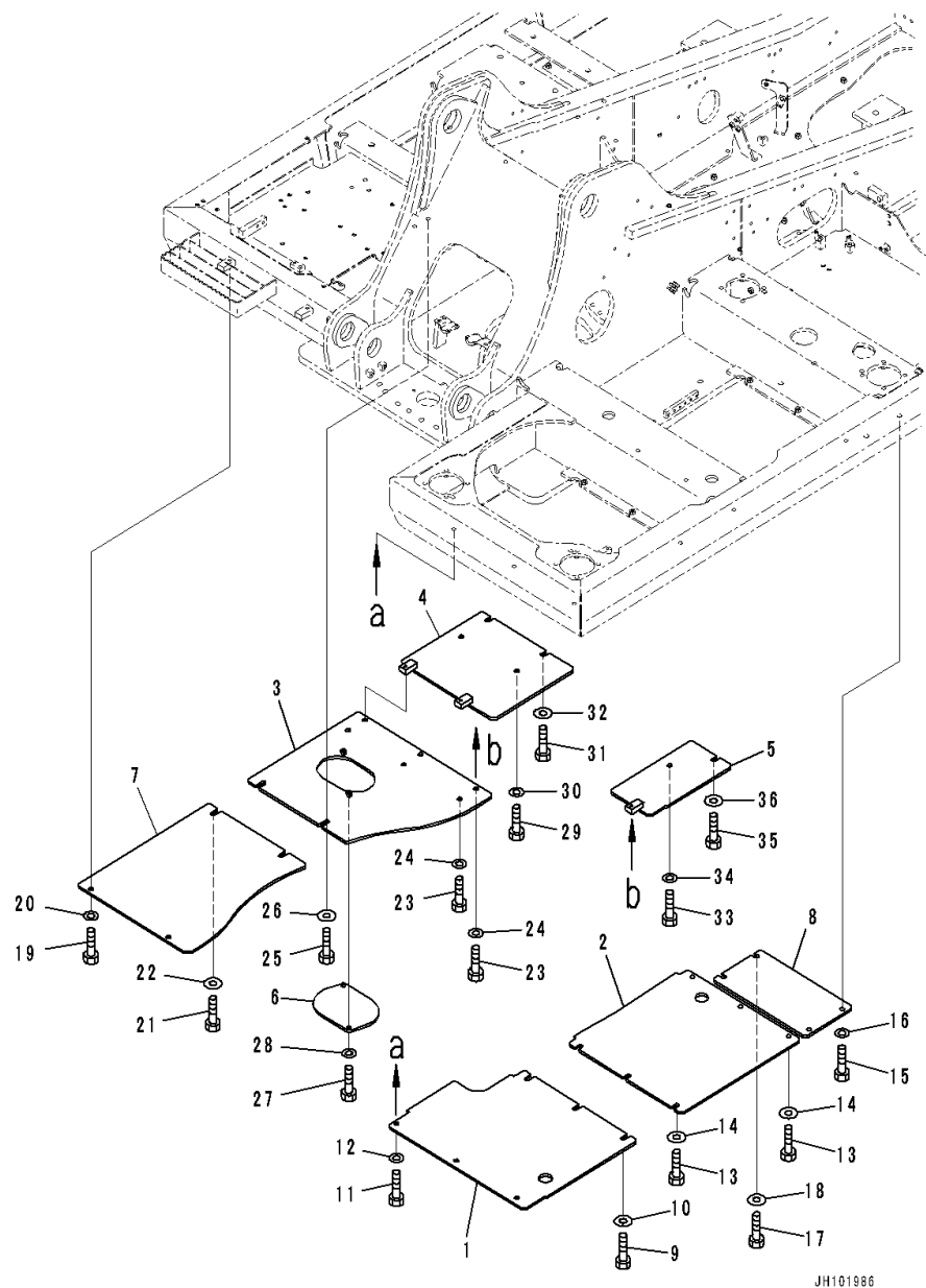
FIG. M1810-002001 Under Cover (Heavy Duty Type) (1/2)
