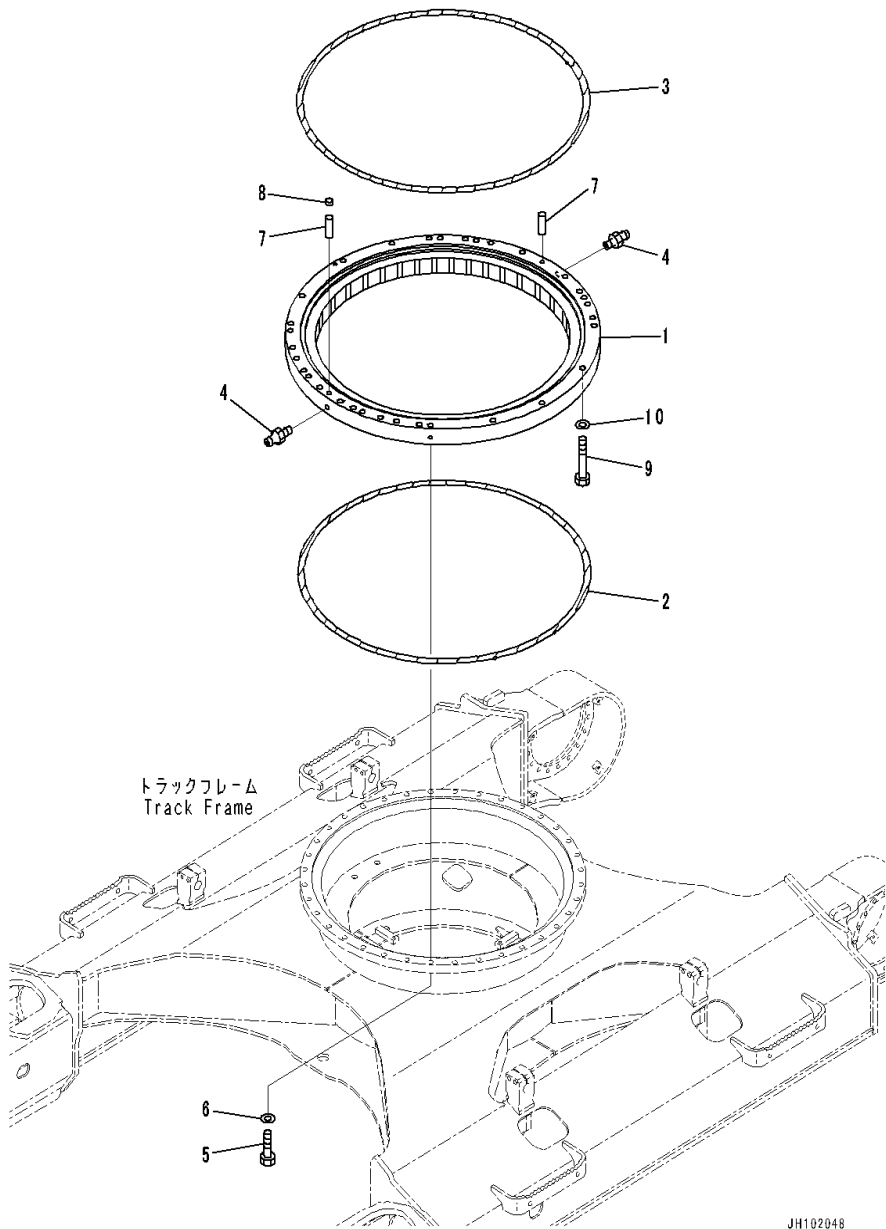
FIG. N1110-002001 Swing Circle (Oil Resistance, For Asia)
