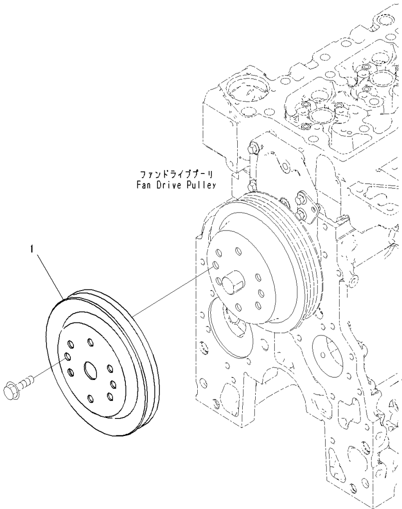
FIG. APA00-001001 Accessory Drive Pulley
