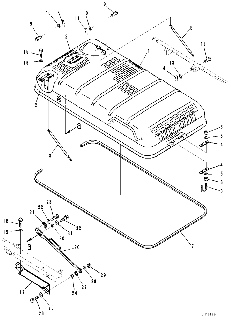
FIG. M1110-002001 Engine Hood (With Pre-cleaner)
