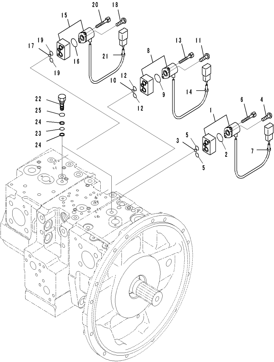
FIG. A9999-001013 Hydraulic Pump (Piston Pump, 11/12)
