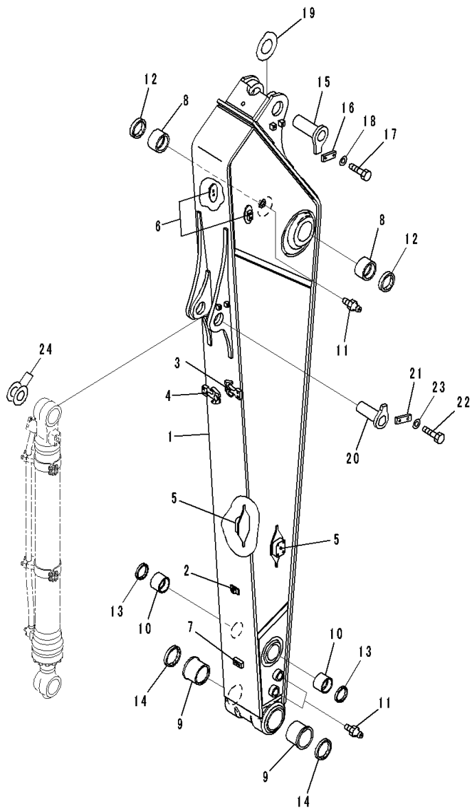
FIG. T1200-001001 Arm (2900mm, Heavy Duty Type,100 Hours Lubrication Interval) (Arm and Pin)
