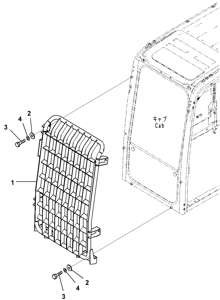
FIG. K0230-002001 Front Guard, Full Guard LV2
