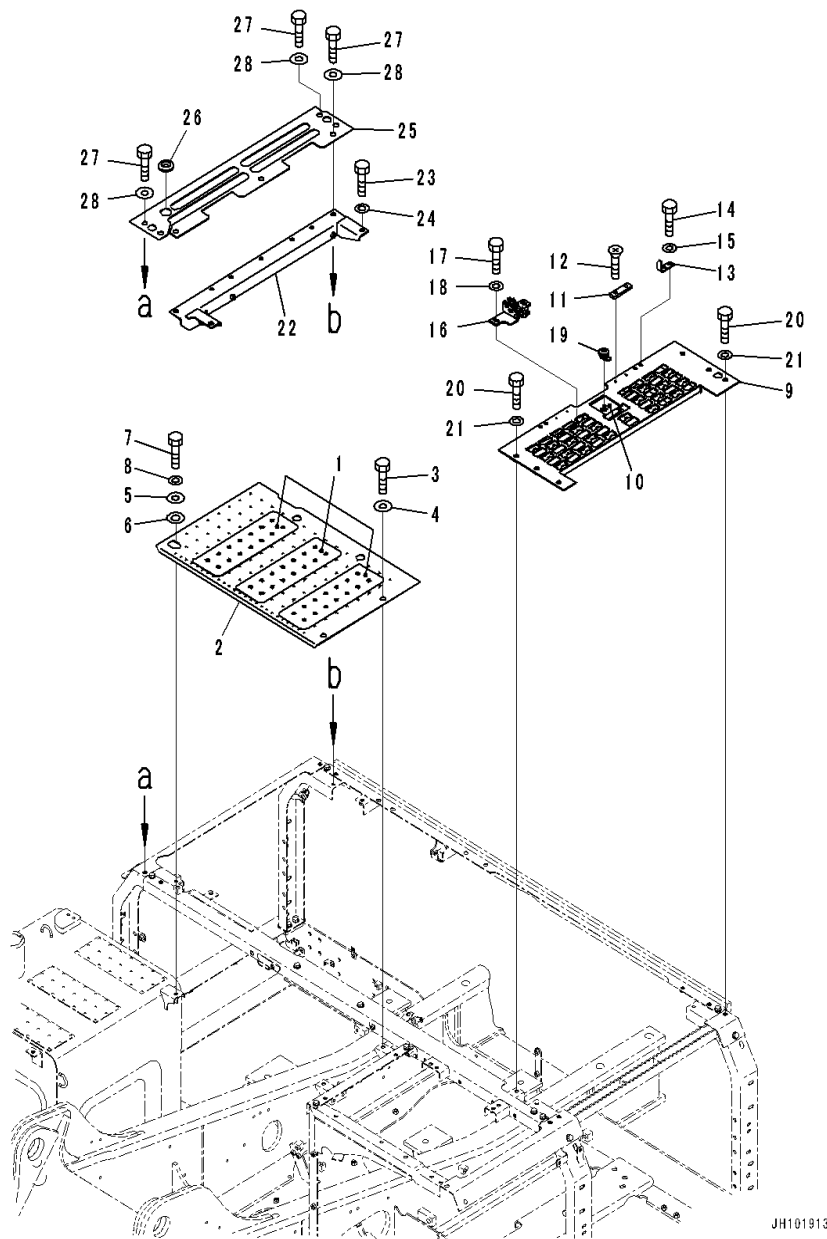
FIG. M1210-001001 Upper Cover
