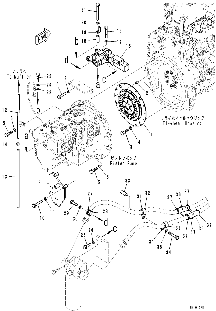
FIG. A9999-001001 Damper (Damper, 1/2)
