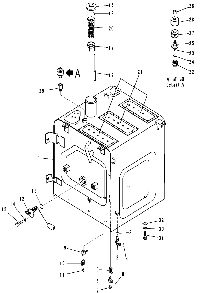
FIG. D0100-003001 Fuel Tank (Refueling Pump, With Breather)
