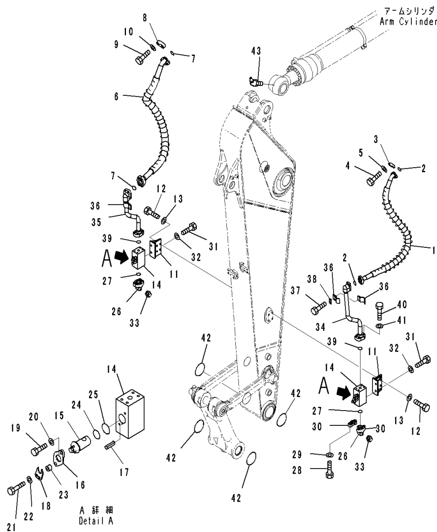
FIG. T1200-003005 Arm (2400mm, Heavy Duty Type, 1-Attachment) (Additional Piping)
