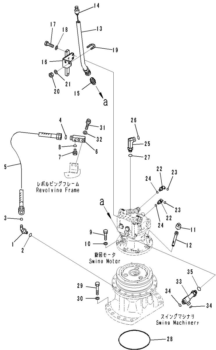
FIG. N1210-001005 Swing Machinery and Motor (Drain Piping)
