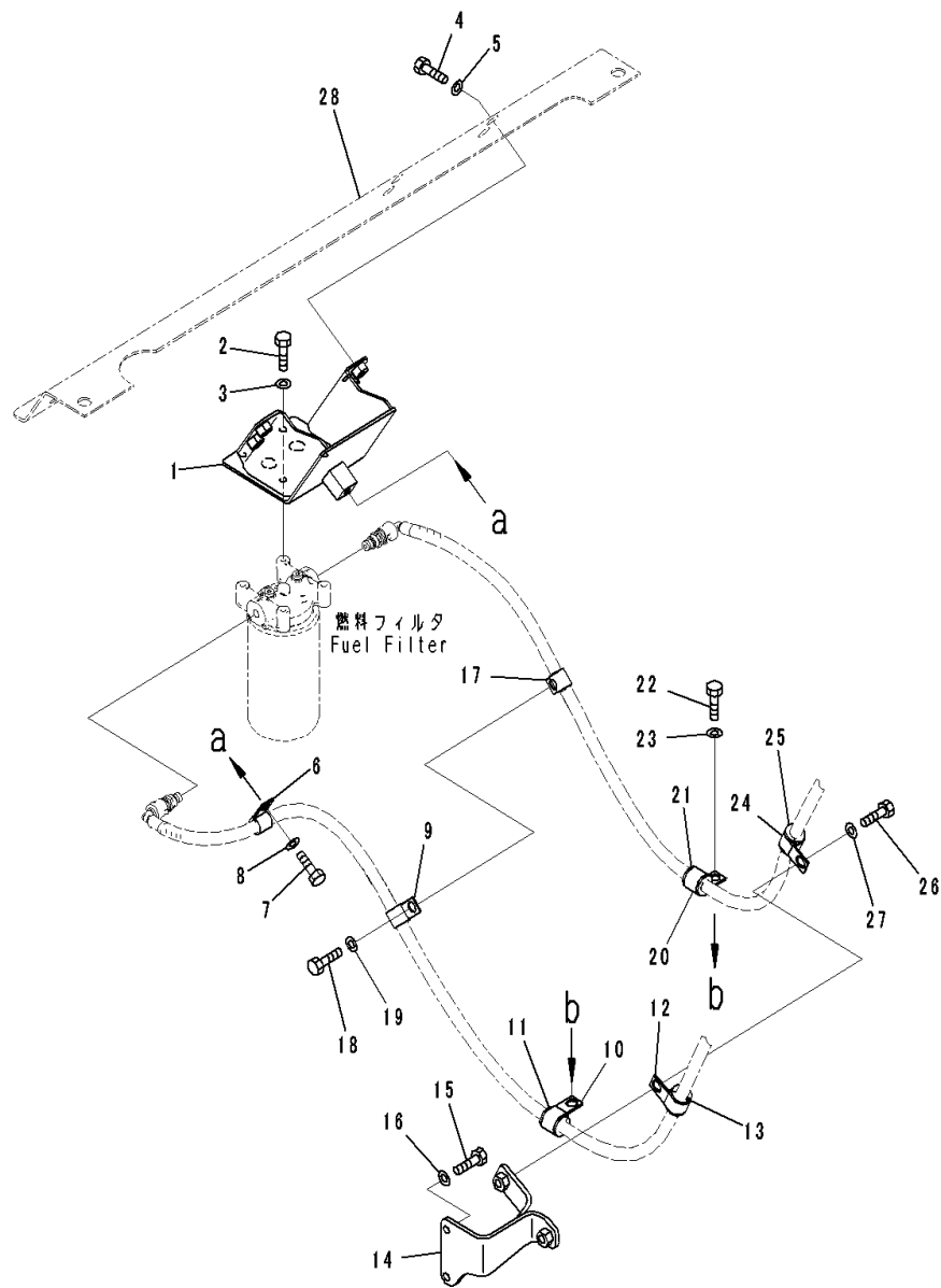
FIG. D0200-001007 Fuel Supply Piping (Fuel Filter Bracket)
