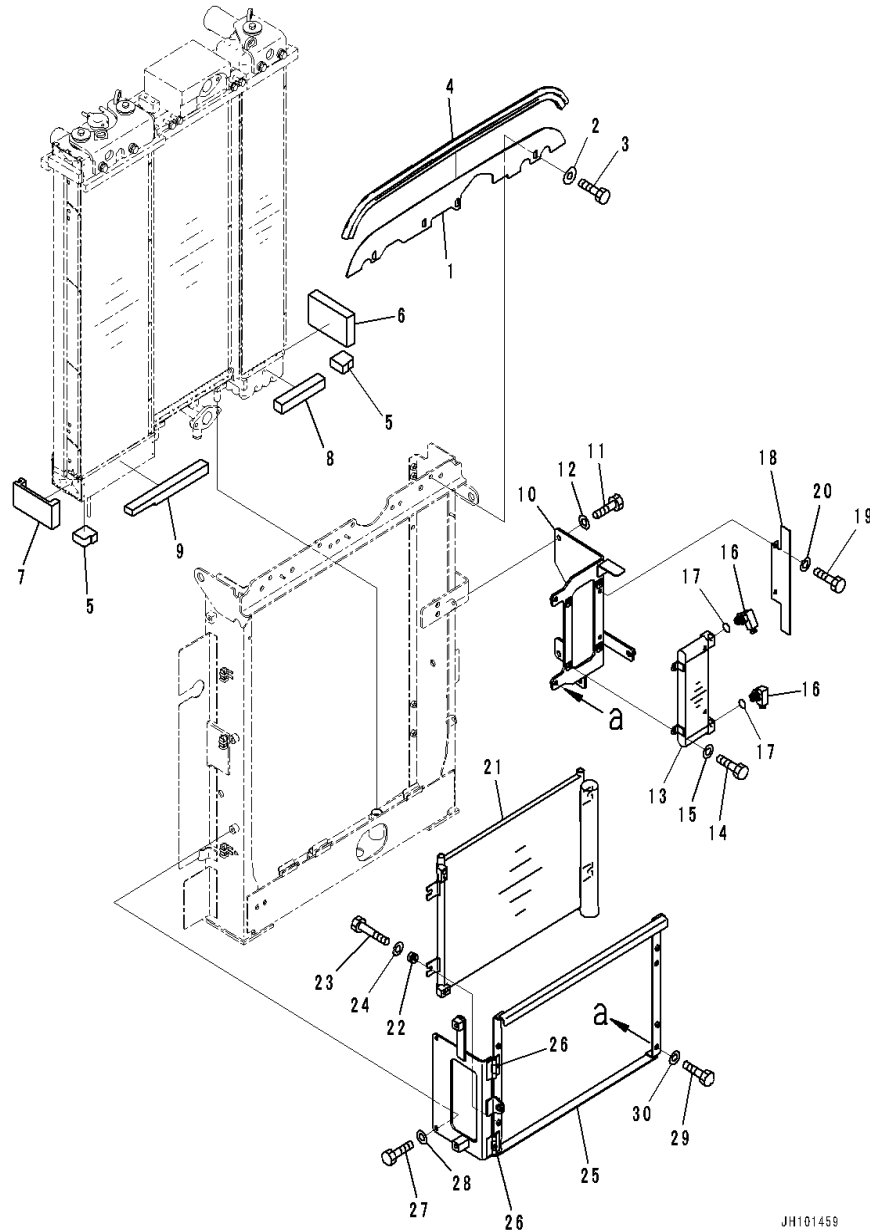
FIG. C0100-001005 Cooling System (Fuel Cooler and Condenser)
