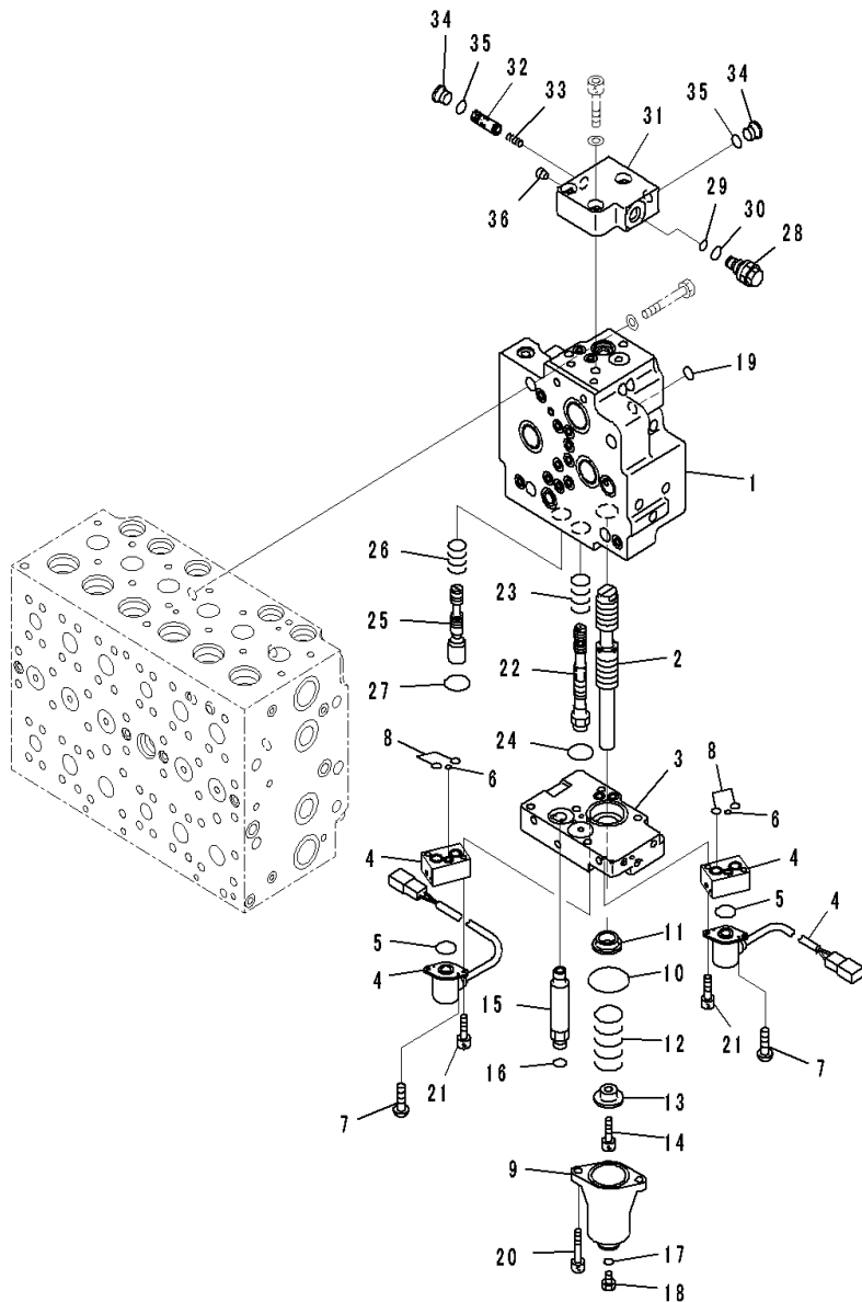
FIG. H0120-001013 Control Valve (6-Spool, 13/18)
