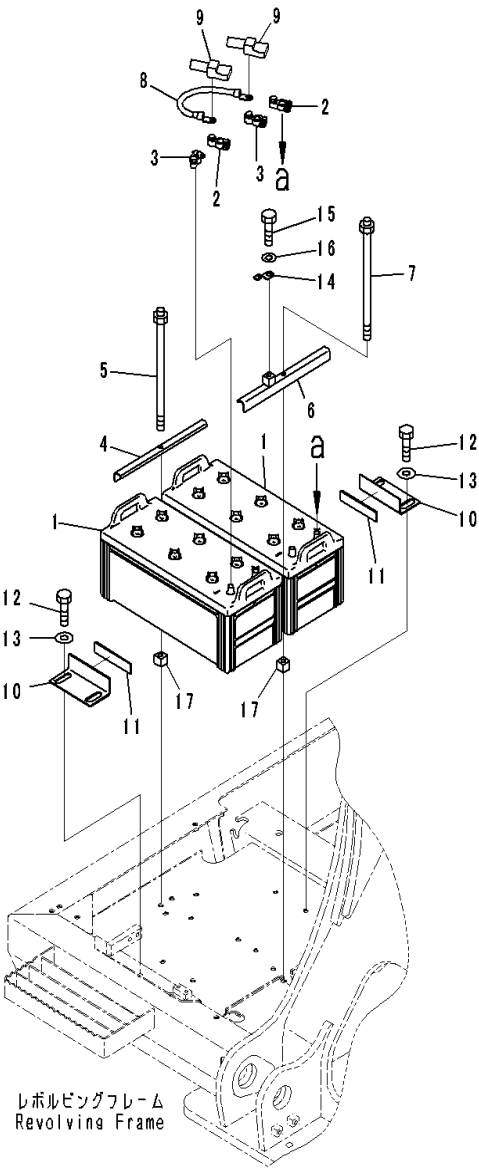
FIG. E0100-002001 Battery (Large Capacity)
