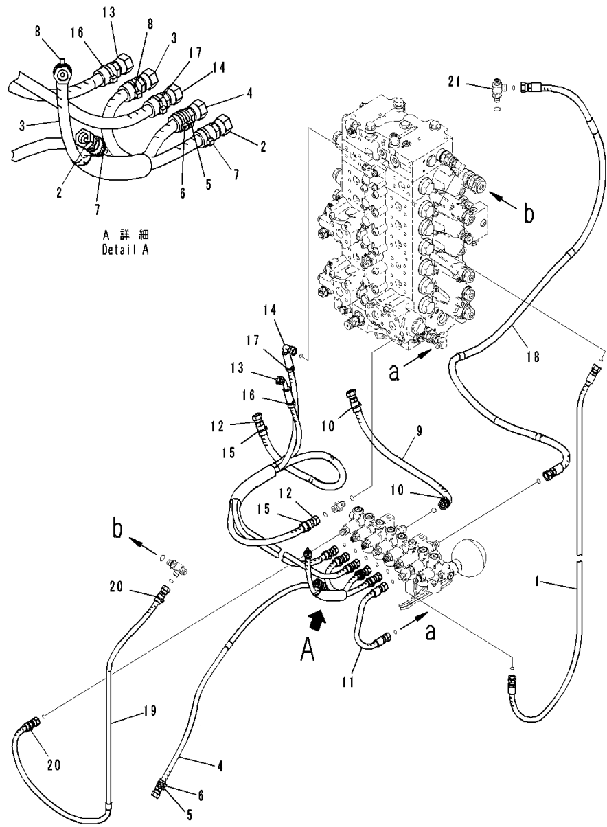
FIG. H1831-002003 Solenoid Valve (1-Additional Actuator Piping, Accumulator) (Solenoid Valve Piping)
