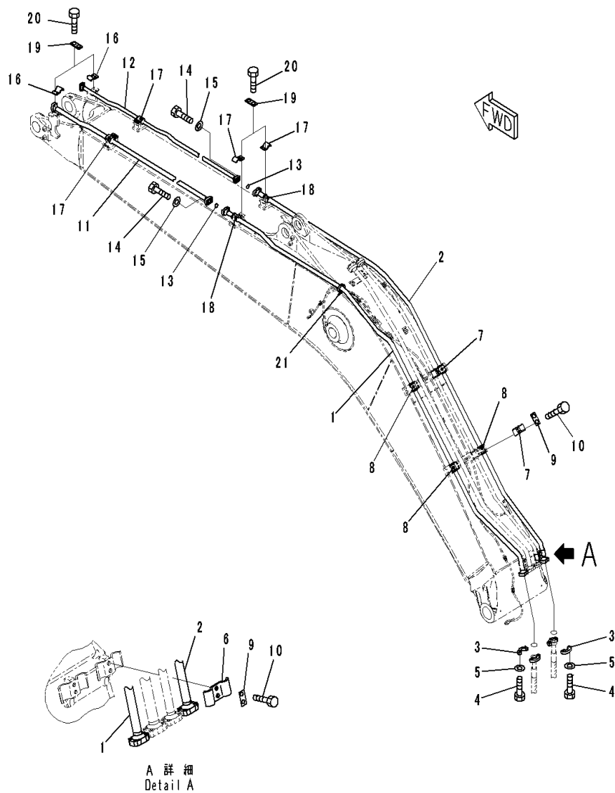
FIG. T1110-001004 Boom (Bucket Cylinder Piping)
