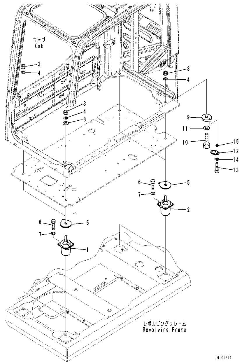
FIG. K1120-001001 Floor Mounting
