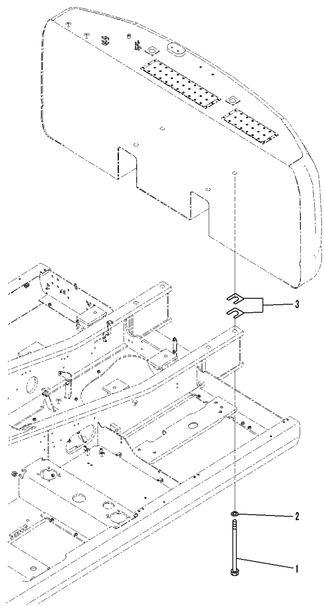
FIG. M1520-001001 Counterweight Mounting
