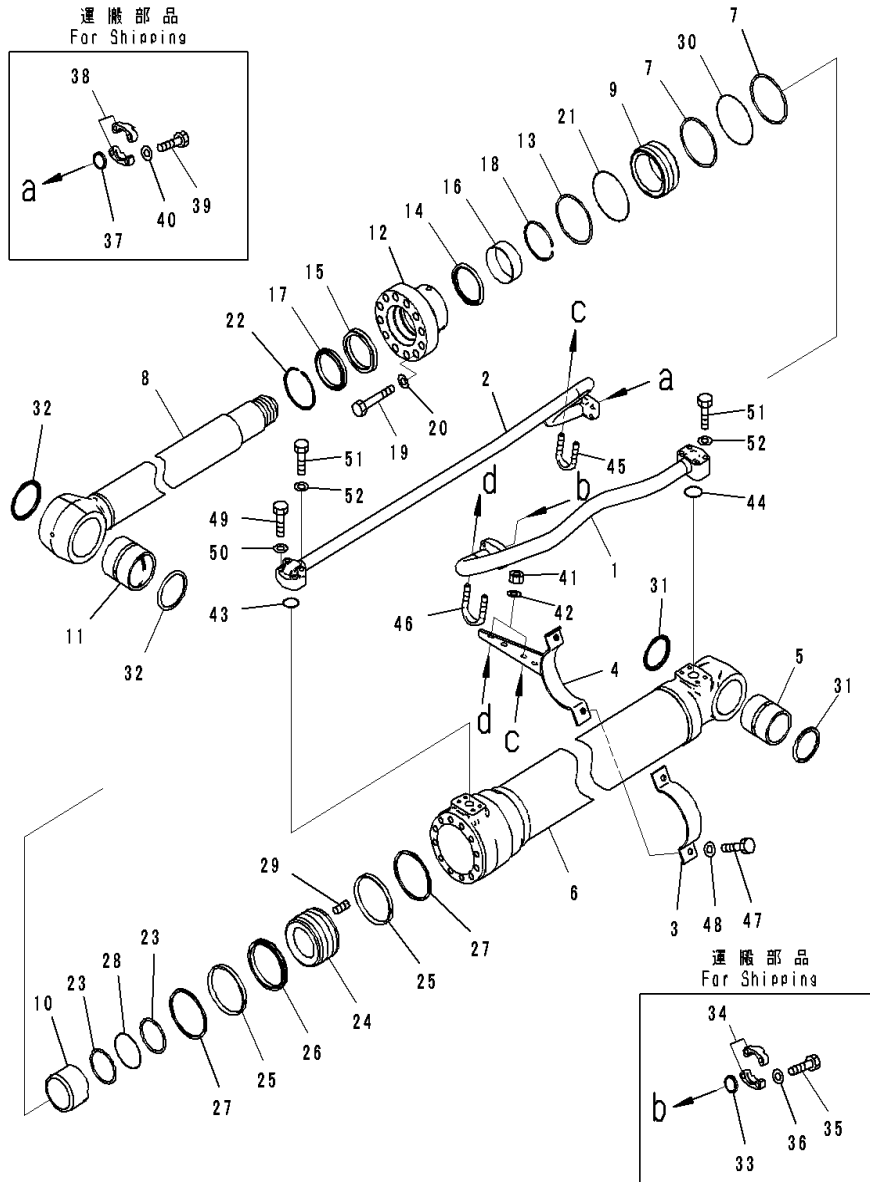
FIG. T1120-001001 Boom Cylinder (100 Hours Lubrication Interval) (Inner Parts, Boom Cylinder, L.H.)
