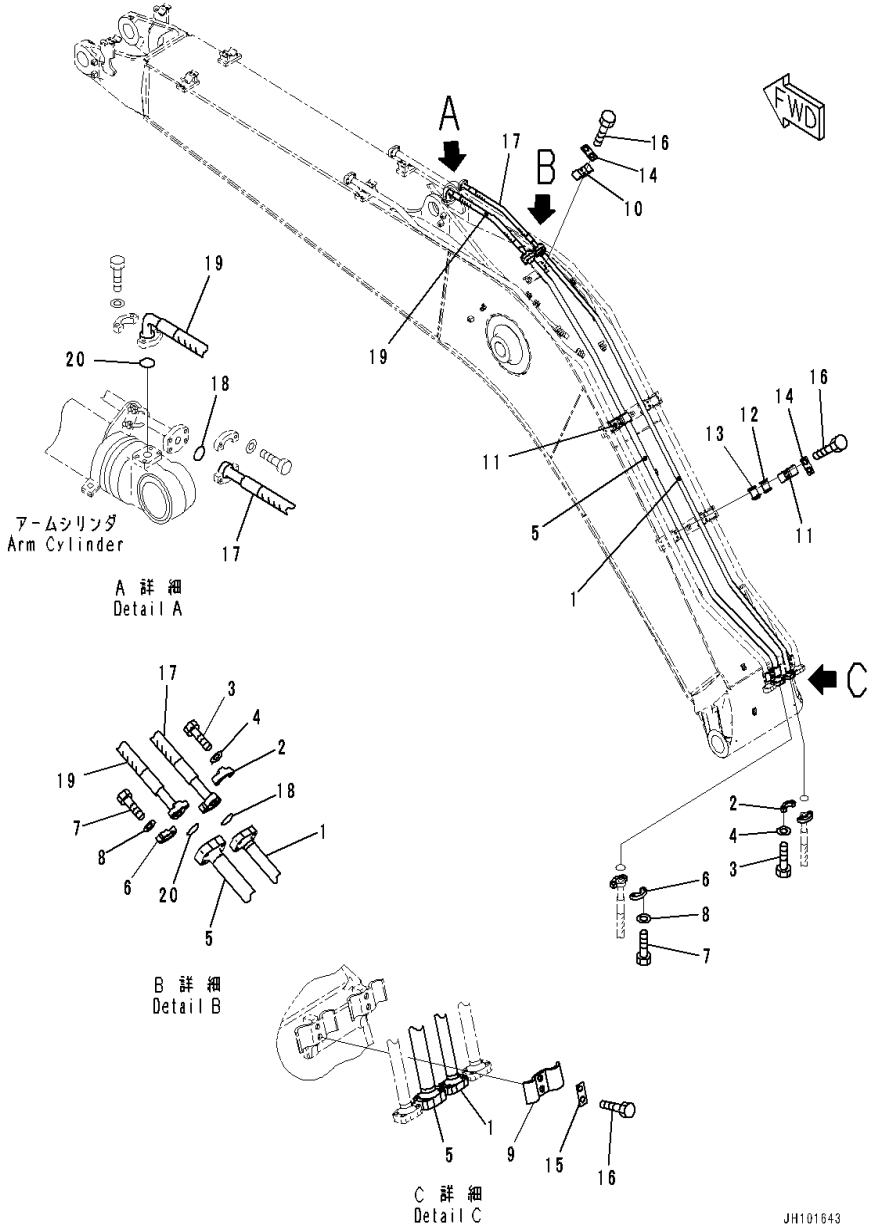
FIG. T1110-001003 Boom (Arm Cylinder Piping)
