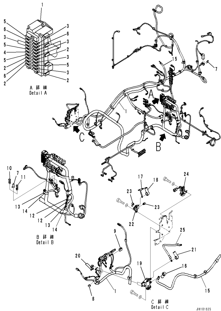
FIG. K1110-001034 Cab (Floor, Wiring Harness)
