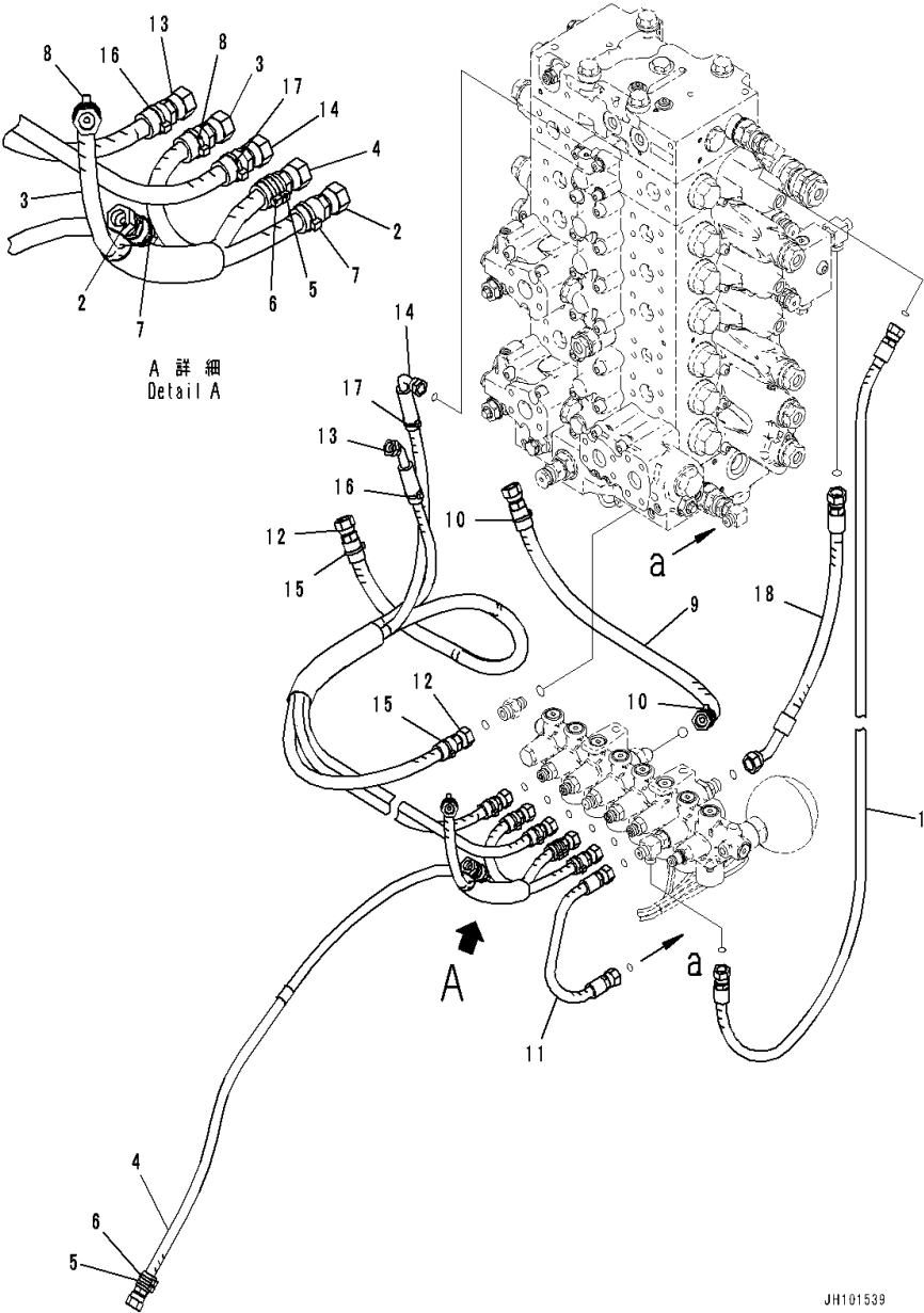
FIG. H1831-001003 Solenoid Valve (Solenoid Valve Piping)
