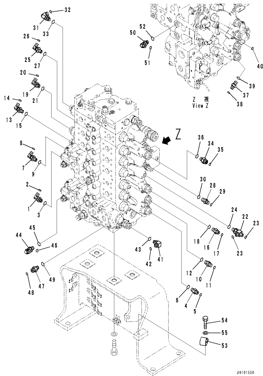
FIG. H0120-002023 Control Valve (Connecting Parts, 1/5)
