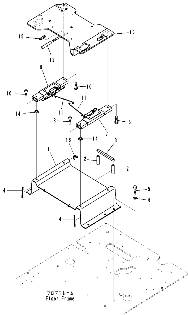
FIG. K1110-001033 Cab (Floor, Base)
