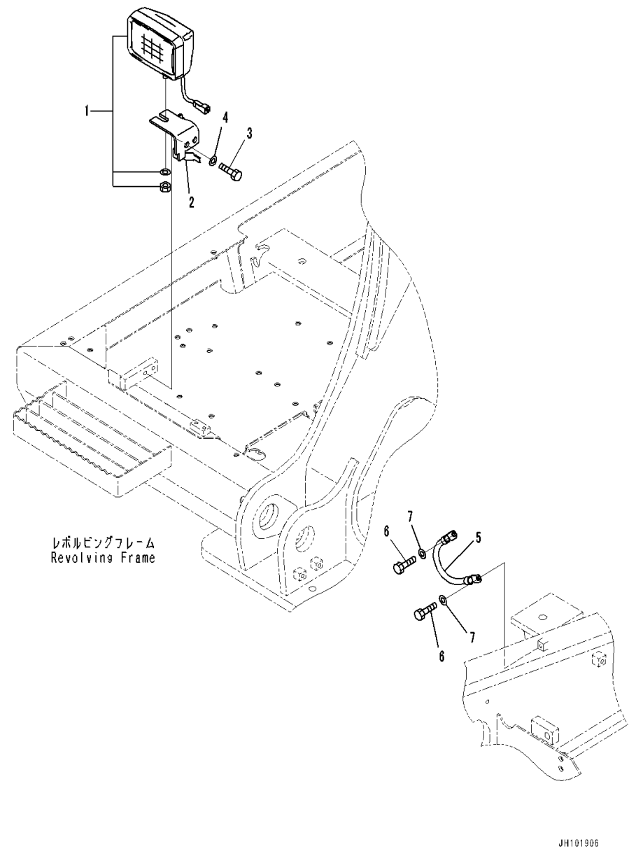
FIG. E0200-001003 Front Working Lamp (Working Lamp, Front)
