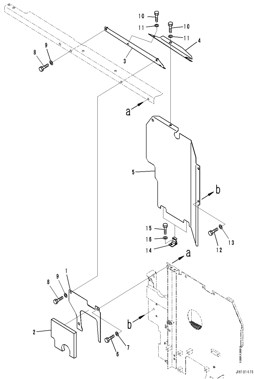
FIG. M1150-001002 Partition (2/4)
