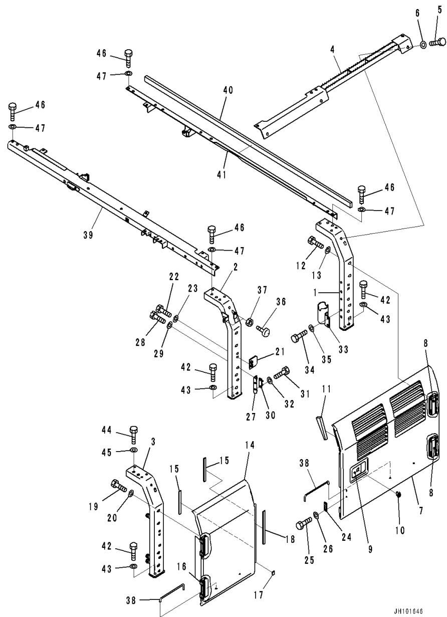
FIG. M1130-002001 Door L.H. (With Pre-cleaner)
