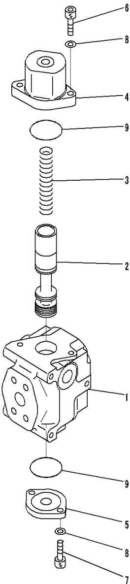
FIG. H1270-001002 Attachment Piping (EPC Valve)
