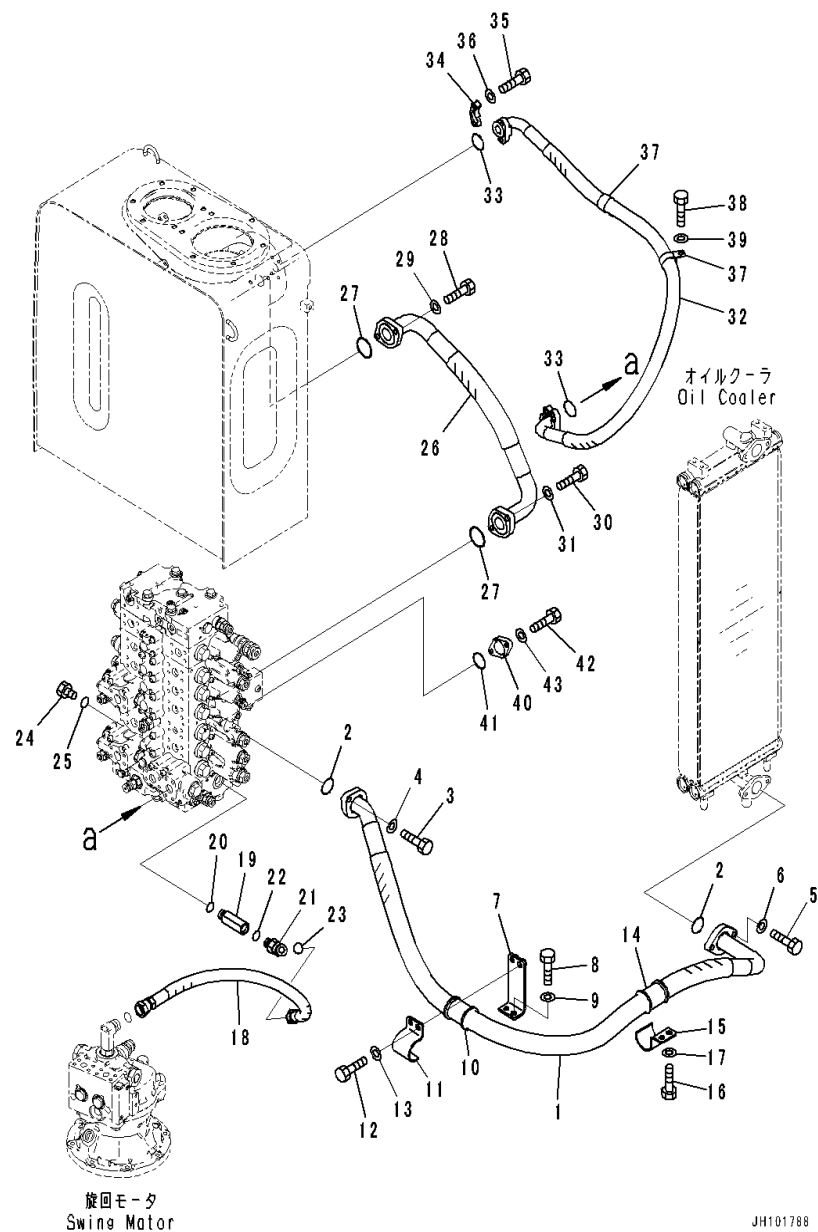
FIG. H0330-001001 Return Piping
