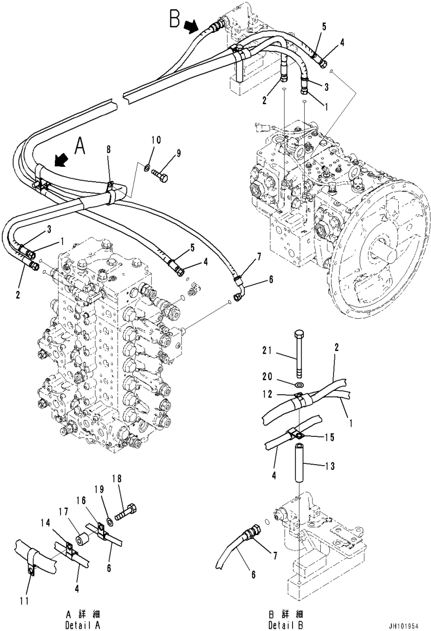
FIG. H1810-002001 LS Piping (1-Additional Actuator Piping, Accumulator)
