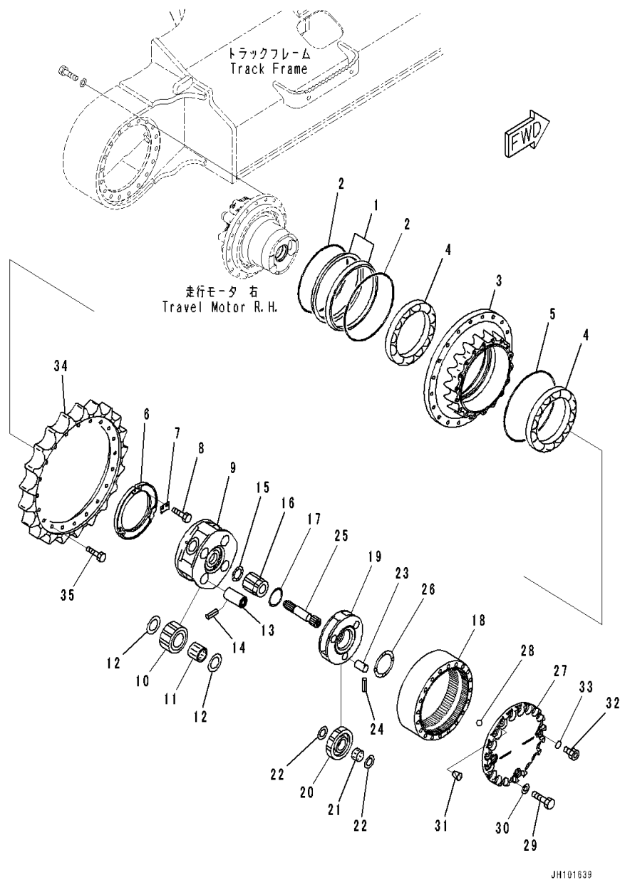
FIG. P1210-001006 Travel Motor and Final Drive (Final Drive R.H.)
