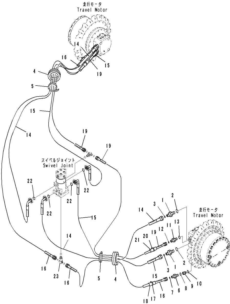
FIG. P1120-001001 Travel Piping
