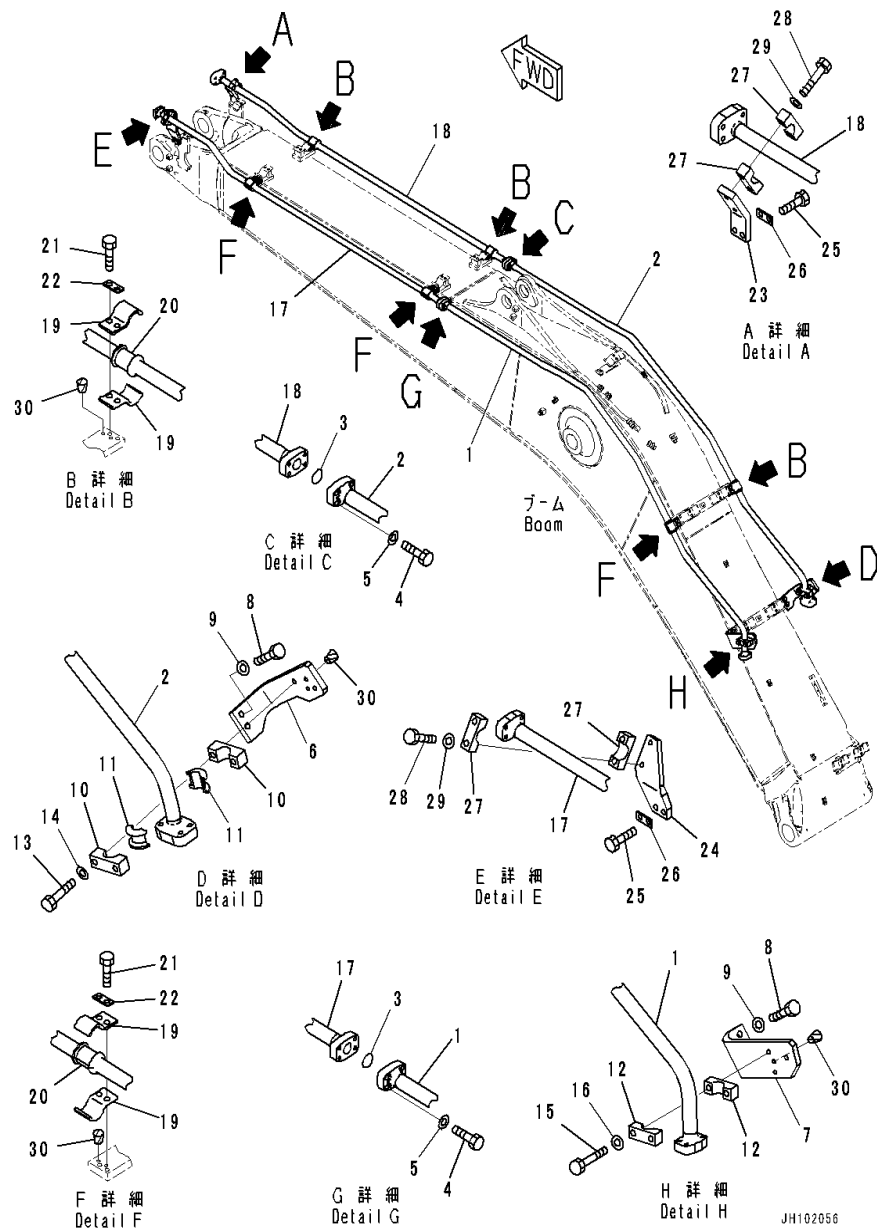
FIG. T1110-002006 Boom (Additional Piping)
