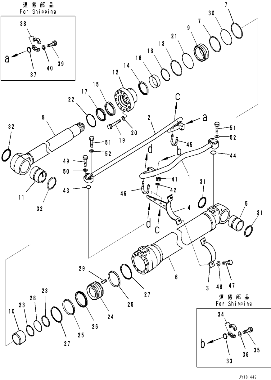
FIG. T1120-001001 Boom Cylinder (100 Hours Lubrication Interval) (Inner Parts, Boom Cylinder, L.H.)
