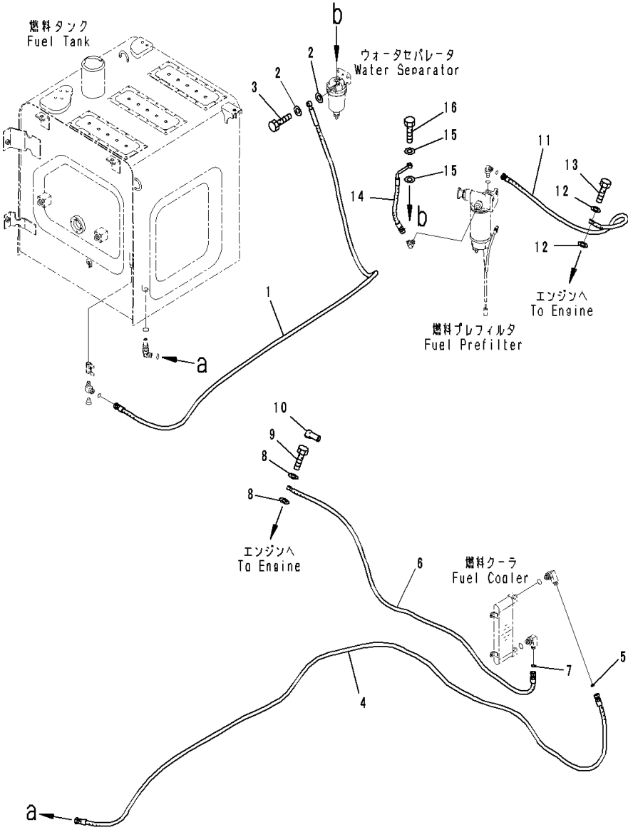
FIG. D0200-001001 Fuel Supply Piping (Fuel Piping)
