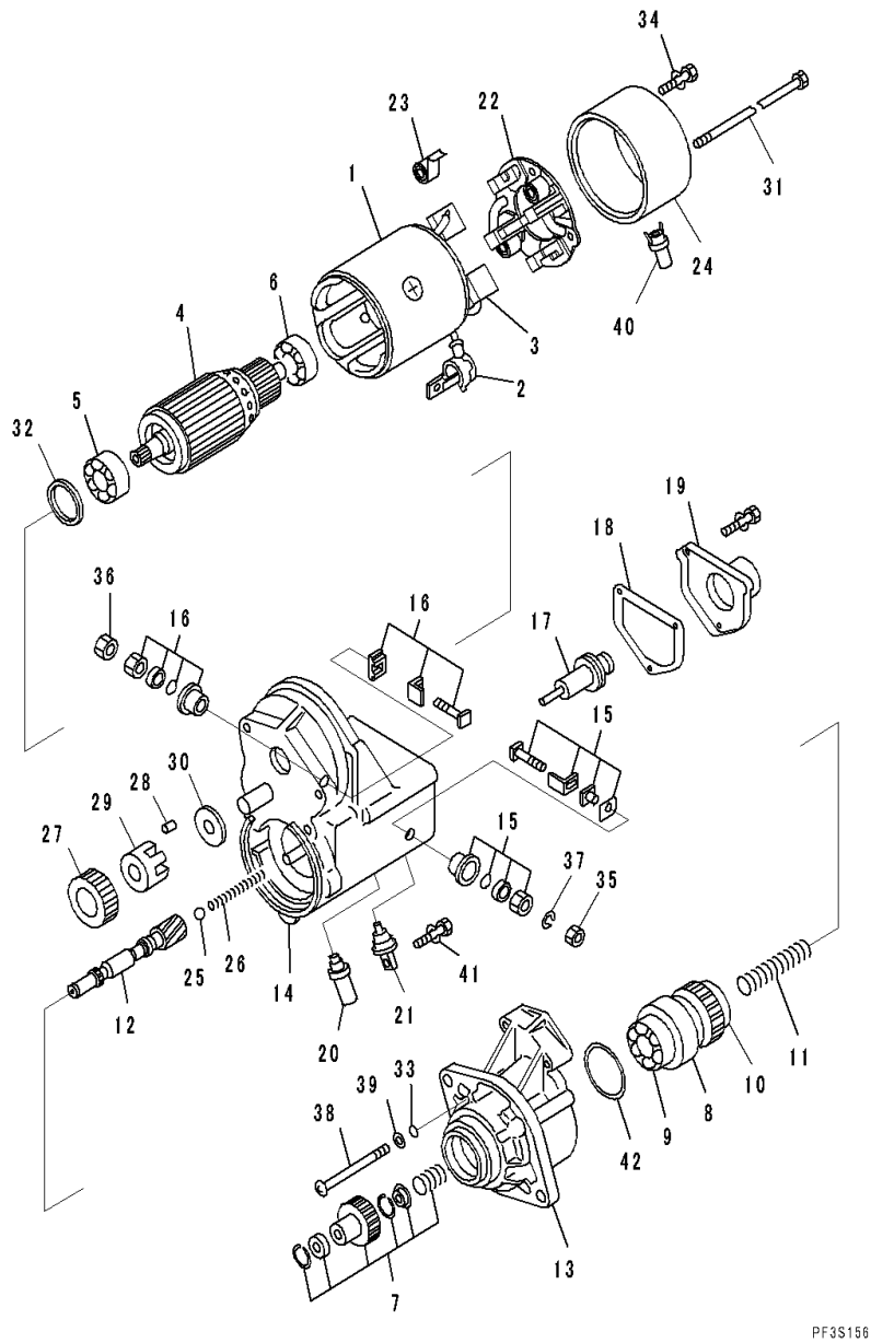
FIG. AST00-001001 Starting Motor (4.5KW)
