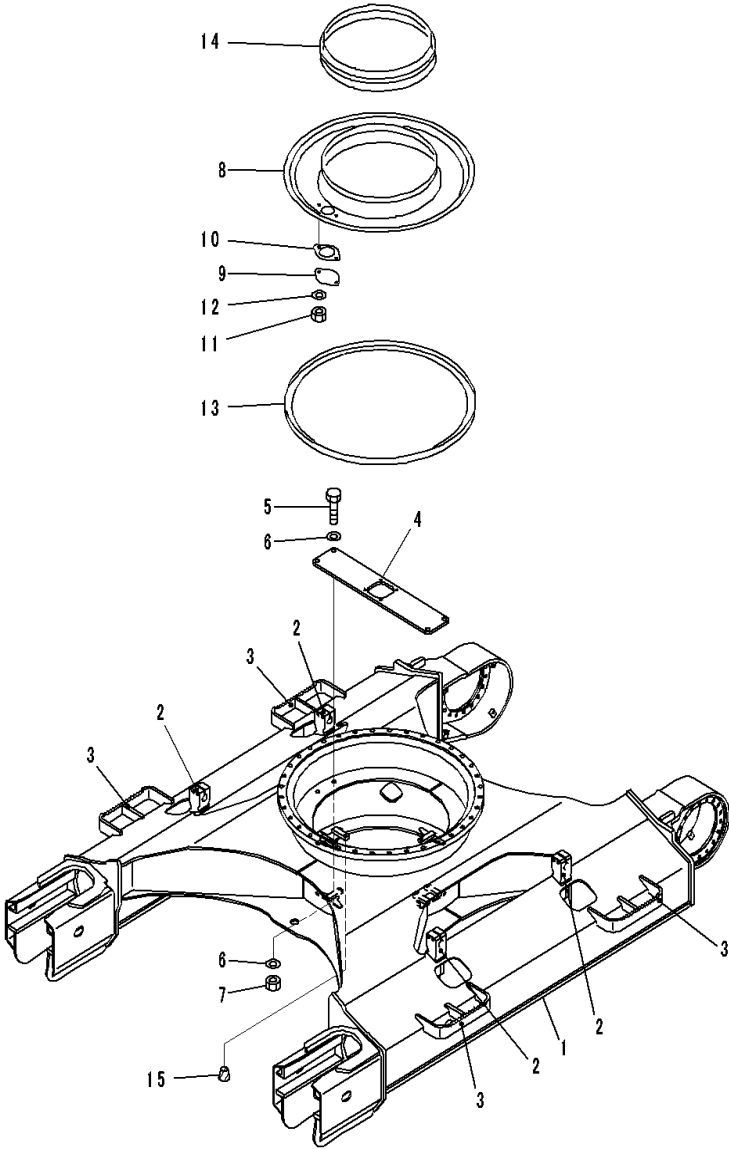
FIG. R1100-001001 Track Frame (Link, 6 Type)
