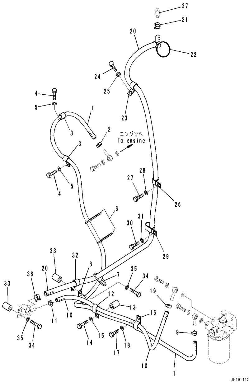
FIG. B0930-001003 Coolant Filter (Hose)
