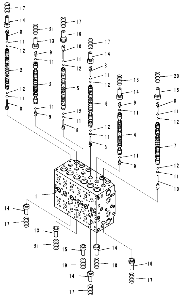
FIG. H0120-001001 Control Valve (6-Spool, 1/18)
