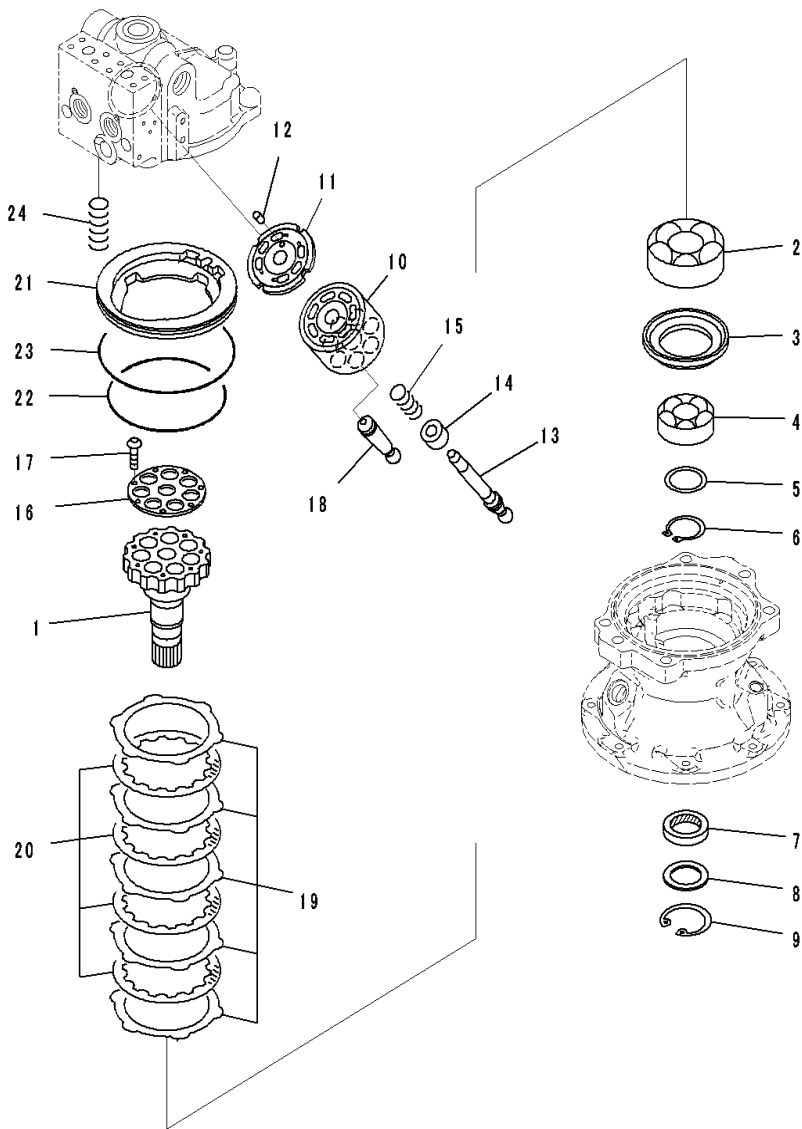
FIG. N1210-001002 Swing Machinery and Motor (Swing Motor, 2/3)
