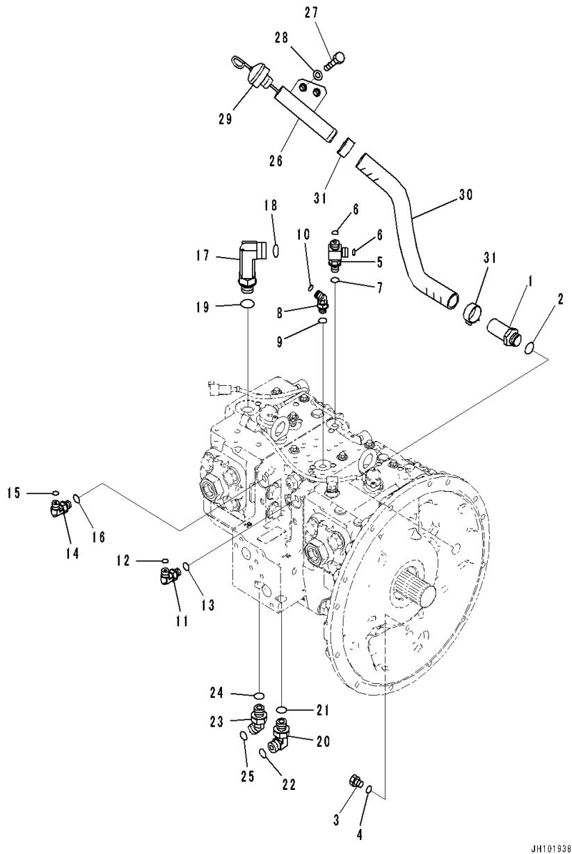
FIG. H0210-002001 Hydraulic Pump (1-Additional Actuator Piping, Accumulator) (Related Parts)
