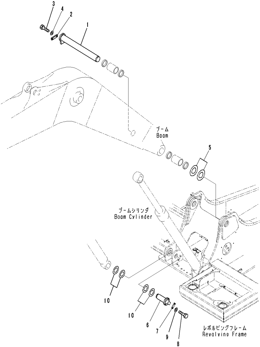
FIG. J1310-001001 Boom Foot Pin (100 Hours Lubrication Interval)
