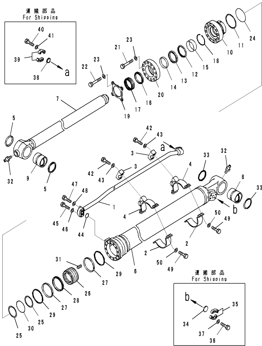
FIG. T1200-001003 Arm (100 Hours Lubrication Interval, Multi Dust Cylinder) (Inner Parts, Bucket Cylinder)
