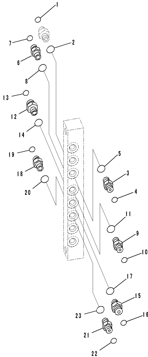
FIG. H1833-001003 Pressure Switch Block (Related Parts, 1/2)
