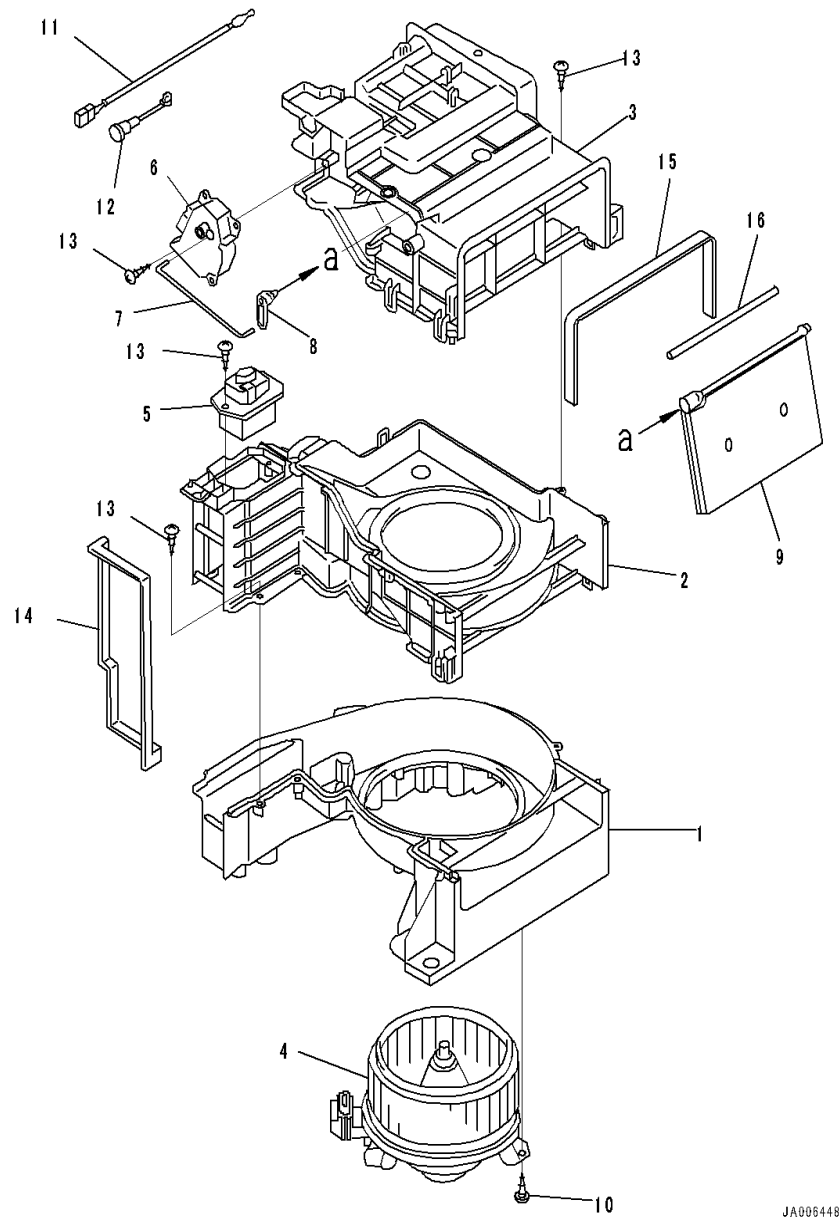
FIG. K1110-001049 CAB (Inner Parts, Air Conditioner Unit, 2/3)
