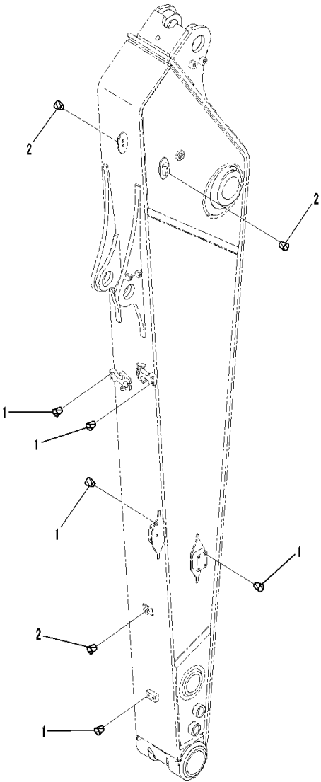
FIG. T1200-001002 Arm (2900mm, Heavy Duty Type) (Plug)
