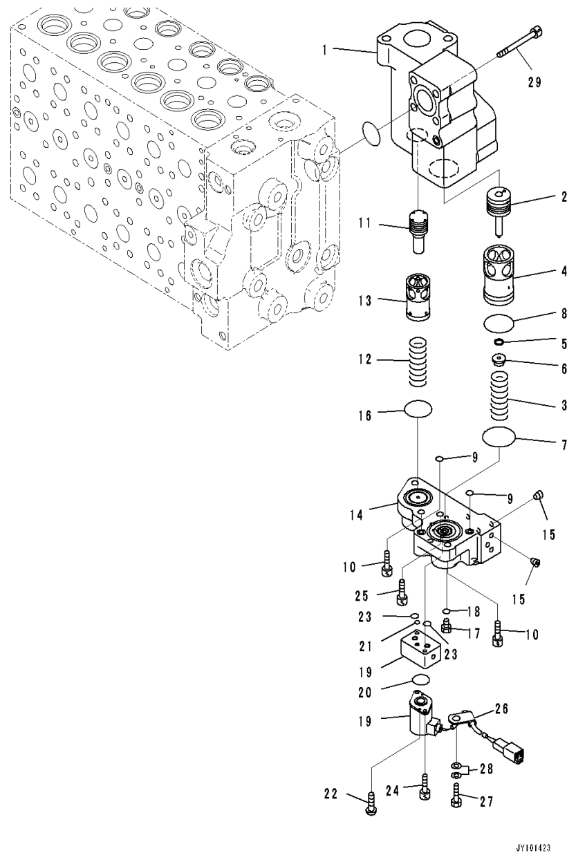
FIG. H0120-001015 Control Valve (6-Spool, 15/18)
