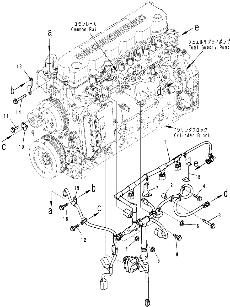
FIG. AWR00-001001 Wiring Harness (5.5KW)
