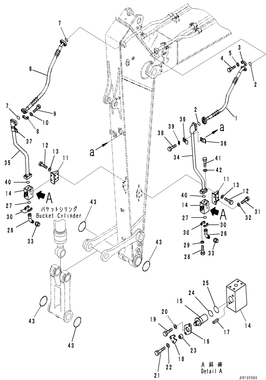
FIG. T1200-002006 Arm (2900mm, Heavy Duty Type, 1-Attachment) (Additional Piping)
