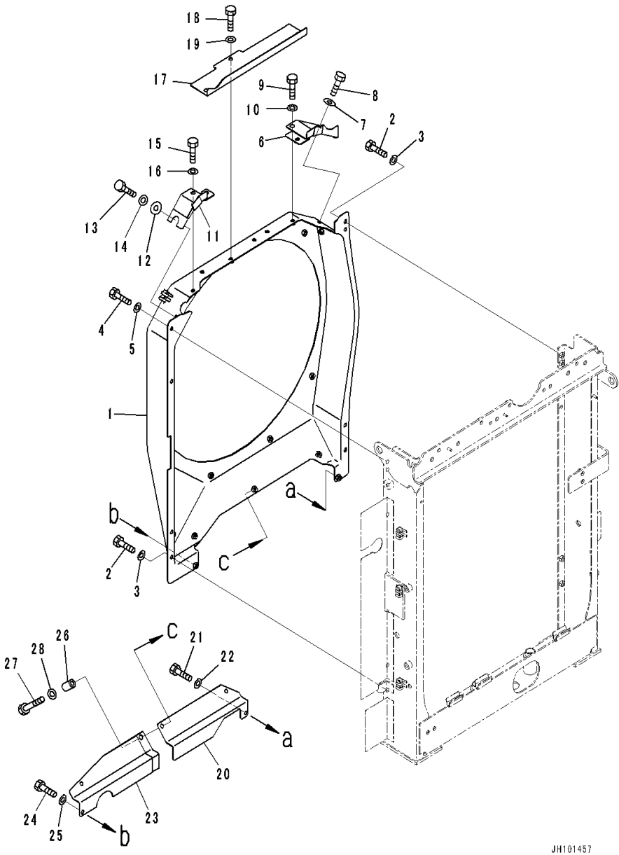
FIG. C0100-001003 Cooling System (Shroud)
