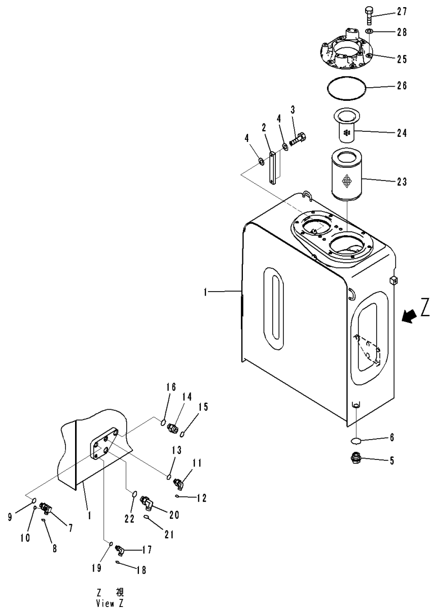
FIG. H0110-002001 Hydraulic Tank (1-Additional Actuator Piping, Accumulator) (Tank)
