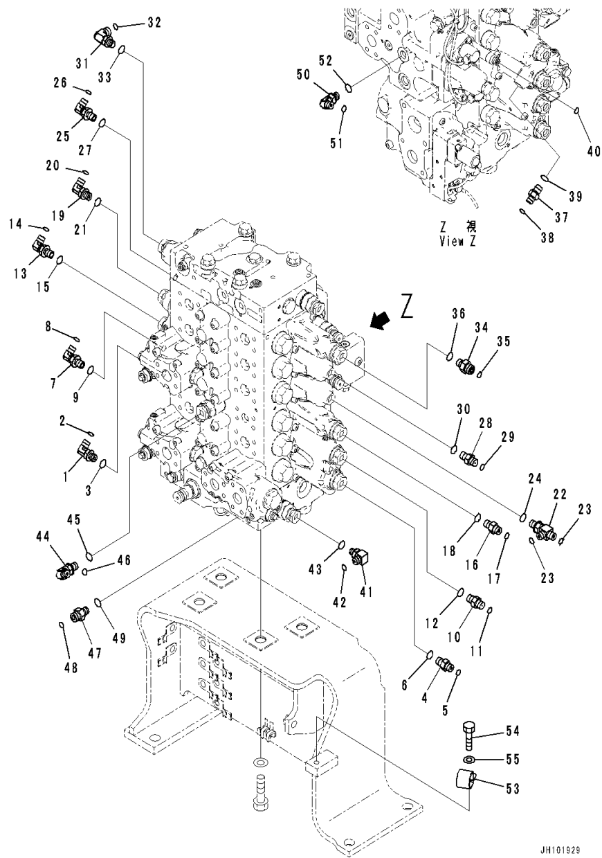
FIG. H0120-001020 Control Valve (Connecting Parts, 1/5)
