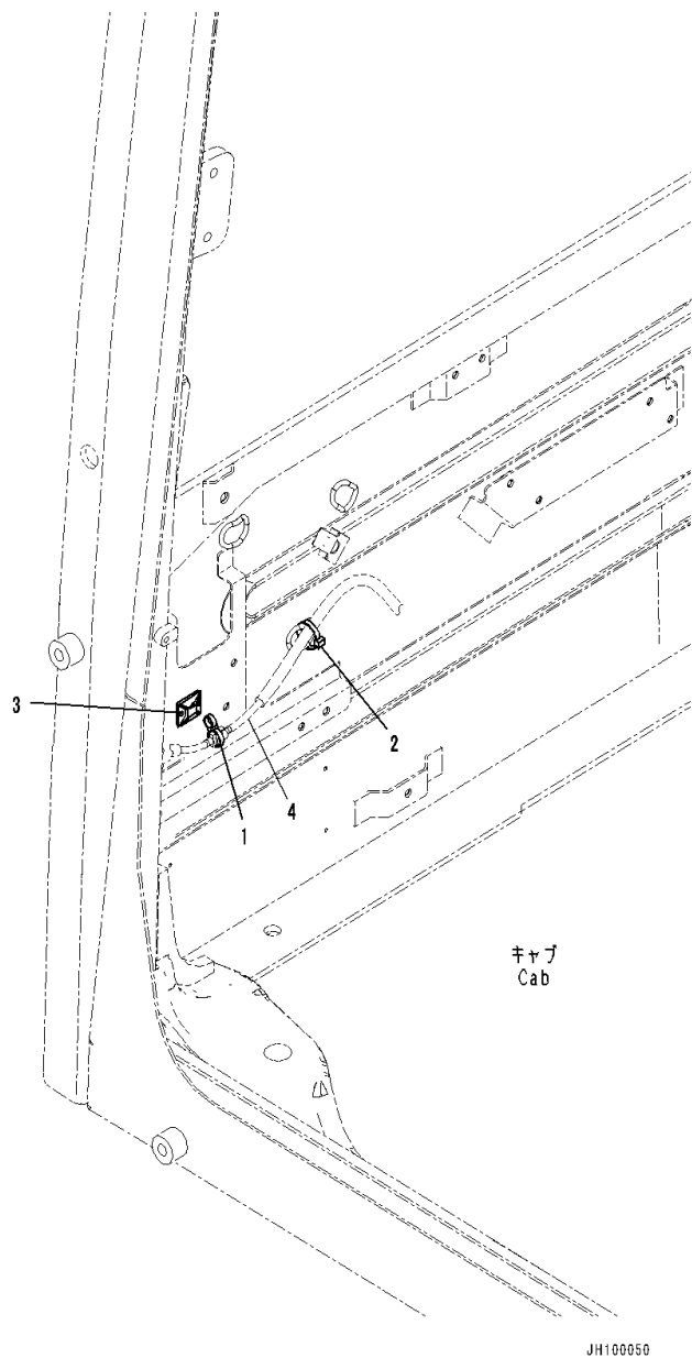
FIG. K1110-001018 Cab (Cab In Parts, Washer Hose Mounting)
