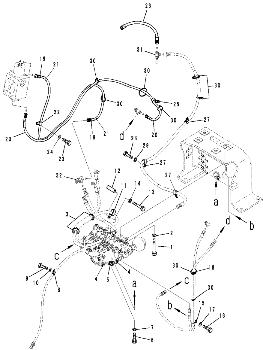
FIG. H1831-002004 Solenoid Valve (1-Additional Actuator Piping, Accumulator) (Mounting)
