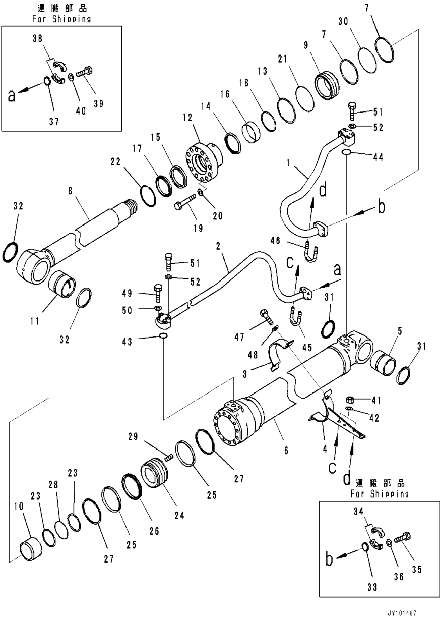
FIG. T1120-001002 Boom Cylinder (100 Hours Lubrication Interval) (Inner Parts, Boom Cylinder, R.H.)
