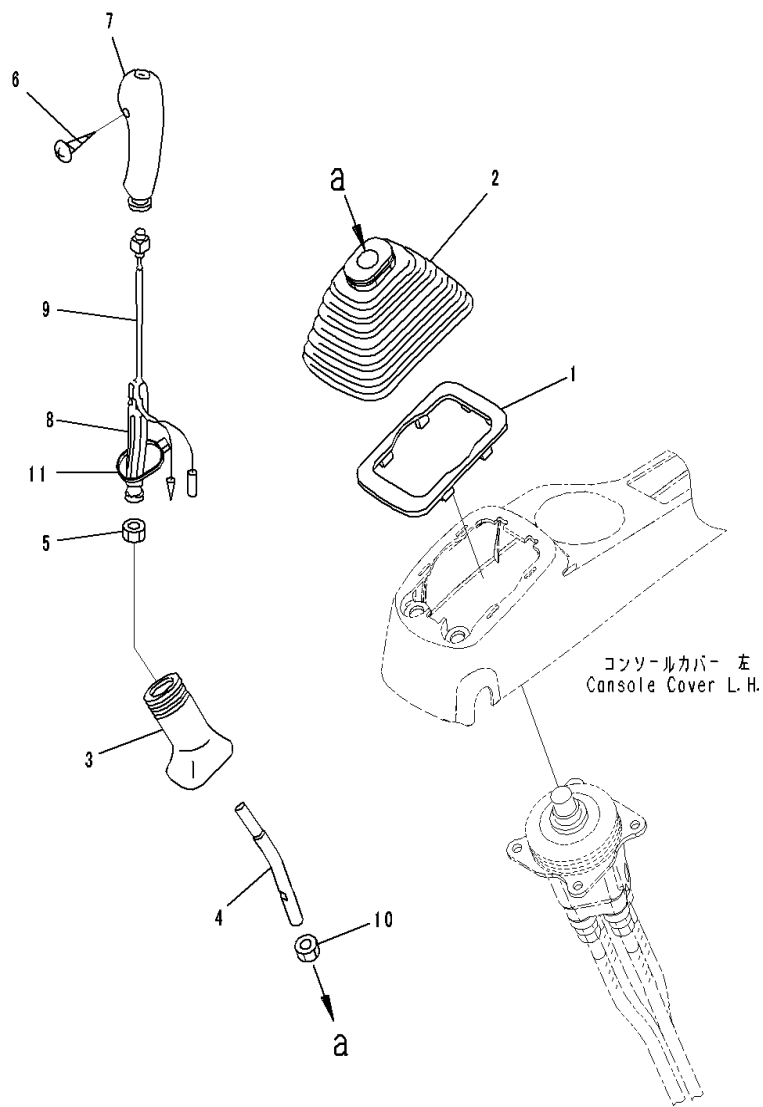
FIG. K1110-001037 Cab (Floor, Work Equipment Control Lever, L.H.)
