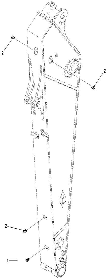
FIG. T1200-002002 Arm (2900mm, Heavy Duty Type, 1-Attachment) (Plug)
