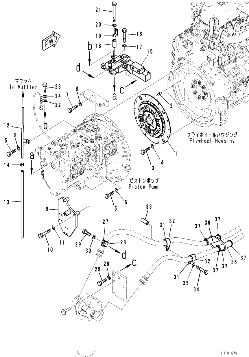
FIG. A9999-001001 Damper (1/1)
