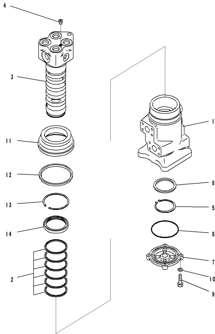
FIG. N1310-001001 Swivel Joint (Inner Parts, Swivel Joint)
