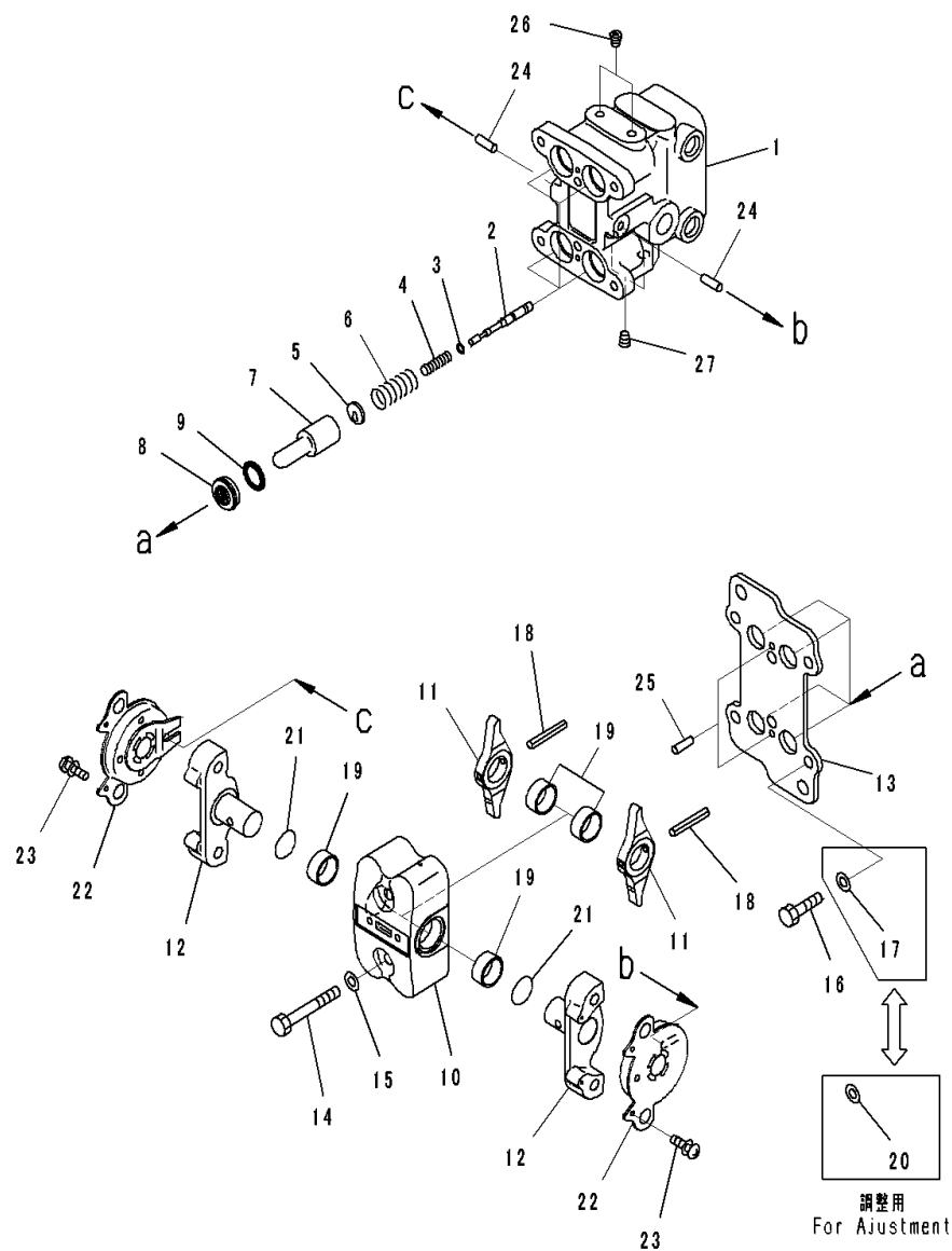
FIG. K1110-001029 Cab (PPC Valve, 1/3, For Travel)
