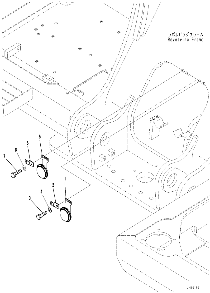
FIG. E0410-001001 Horn
