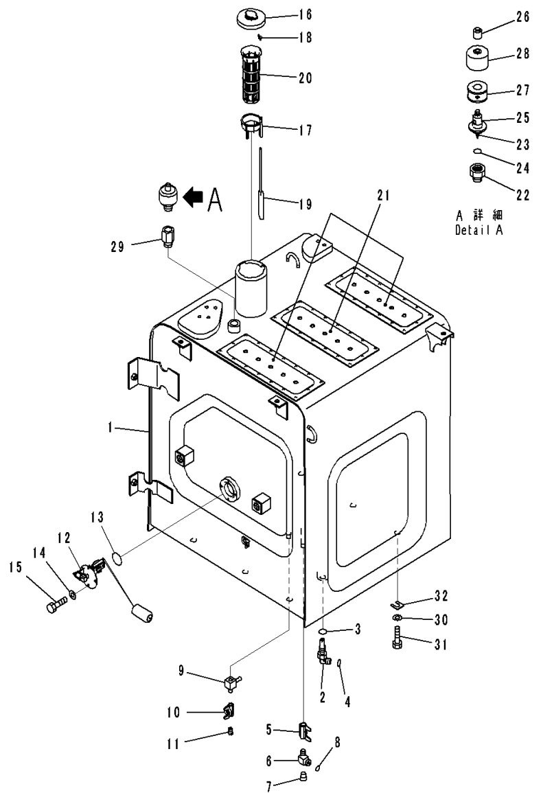
FIG. D0100-002001 Fuel Tank (With Breather)
