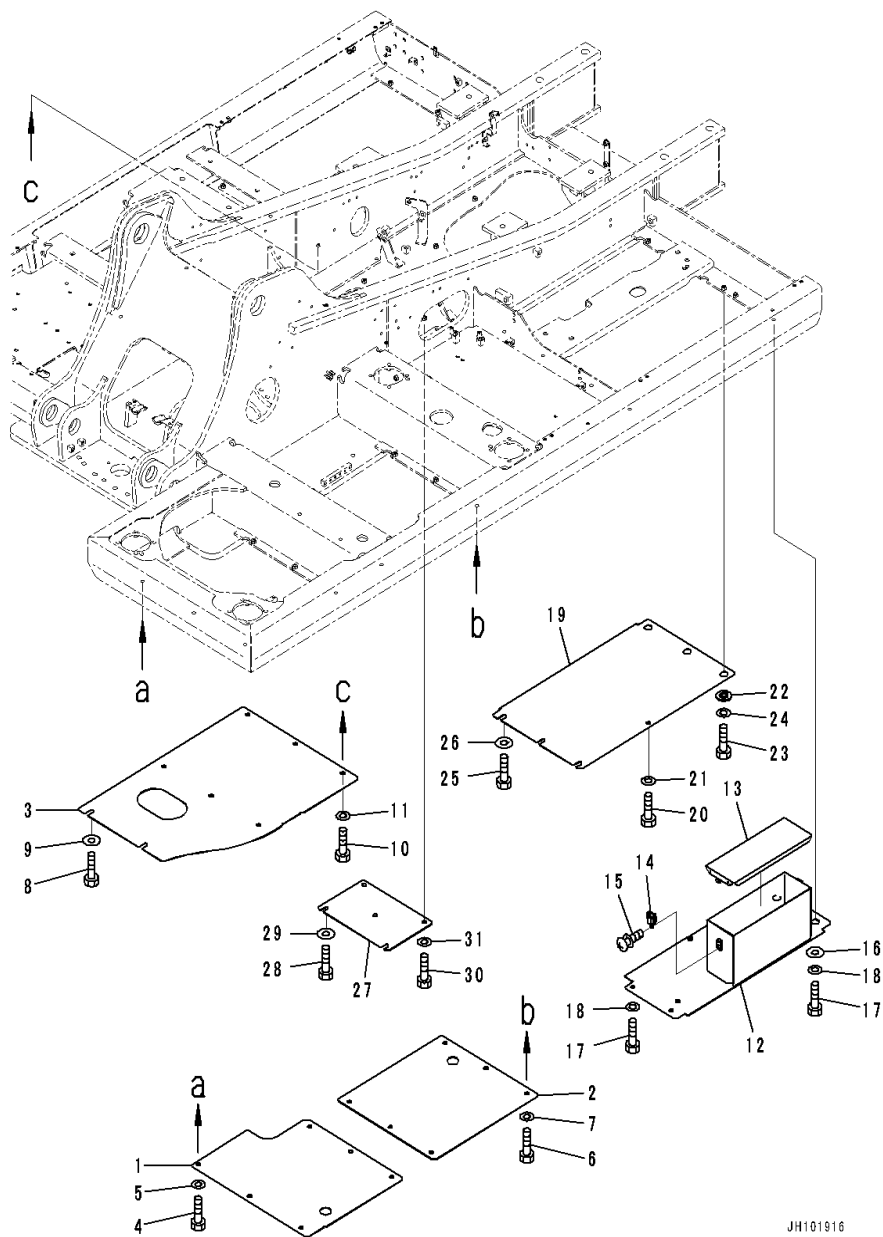
FIG. M1810-001001 Under Cover
