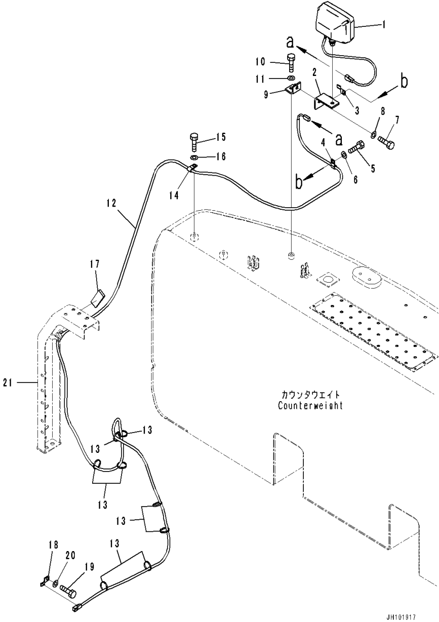
FIG. E0320-001001 Additional Rear Working Lamp
