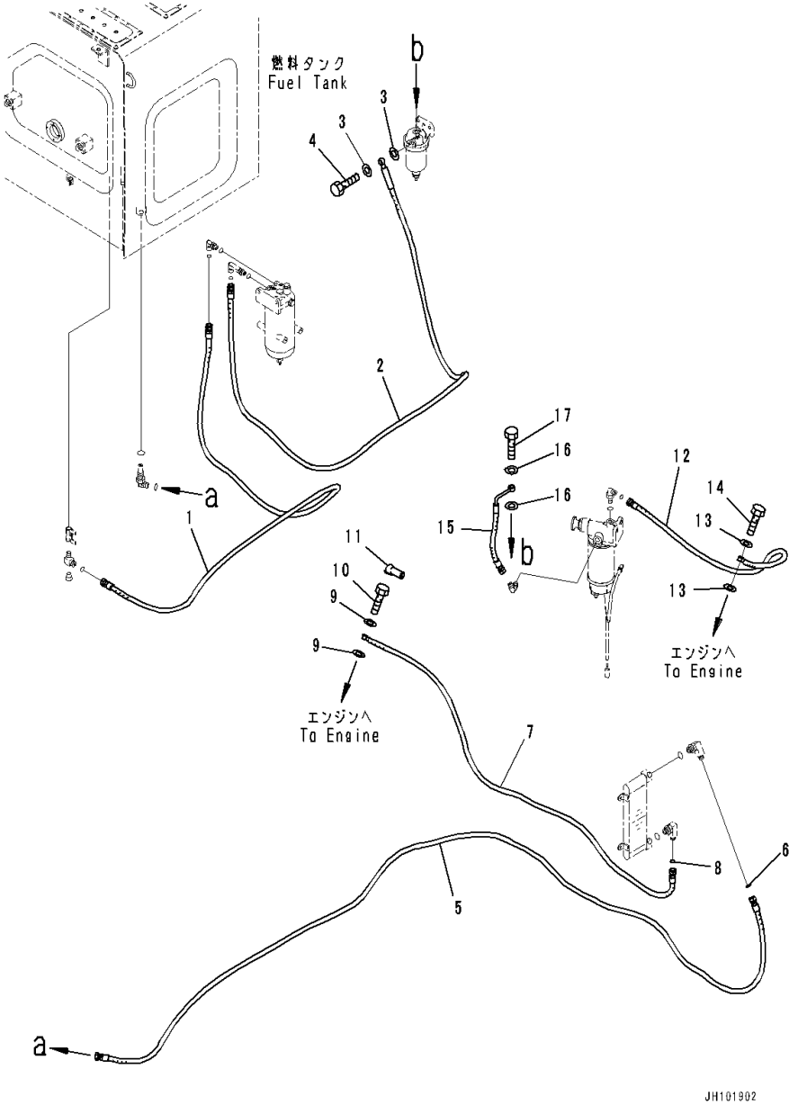
FIG. D0200-002001 Fuel Supply Piping (For Additional Fuel Prefilter) (Fuel Piping)
