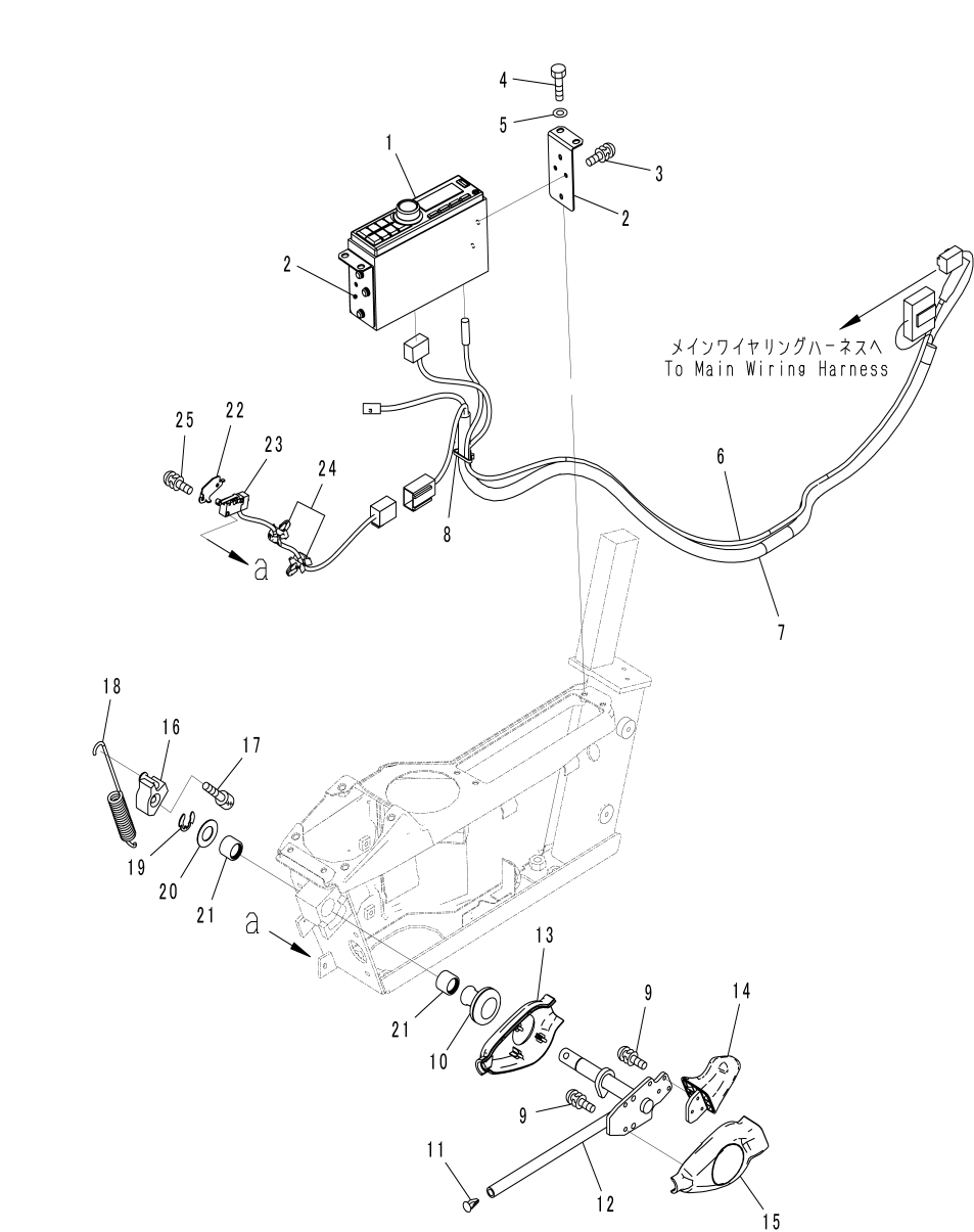
FIG. K1110-001041 Cab (Radio USB MP3) (Floor, Radio and Work Equipment Lock Lever, Radio USB MP3)
