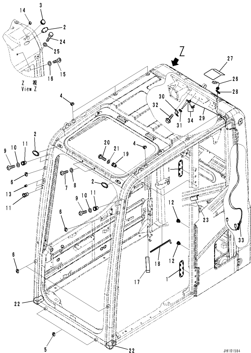
FIG. K1110-001013 Cab (With GPRS 3G) (KOMTRAX Antenna, With GPRS 3G)
