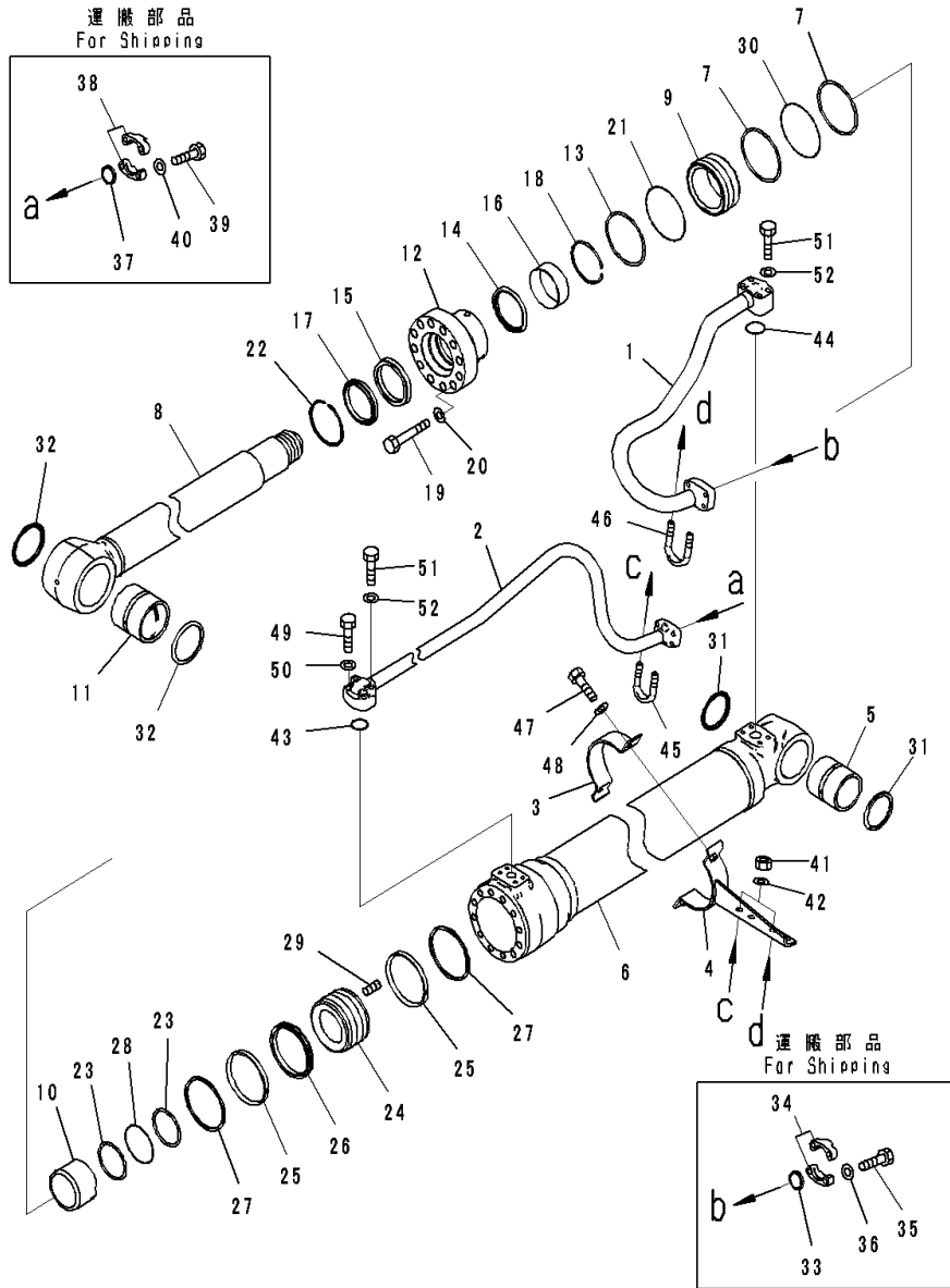
FIG. T1120-001002 Boom Cylinder (100 Hours Lubrication Interval) (Inner Parts, Boom Cylinder, R.H.)
