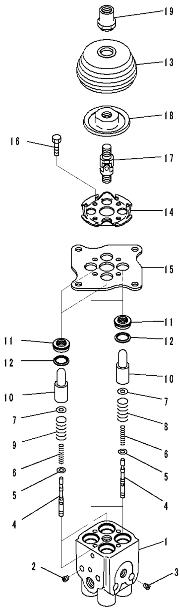
FIG. K1110-001044 Cab (PPC Valve, 3/3, R.H.)
