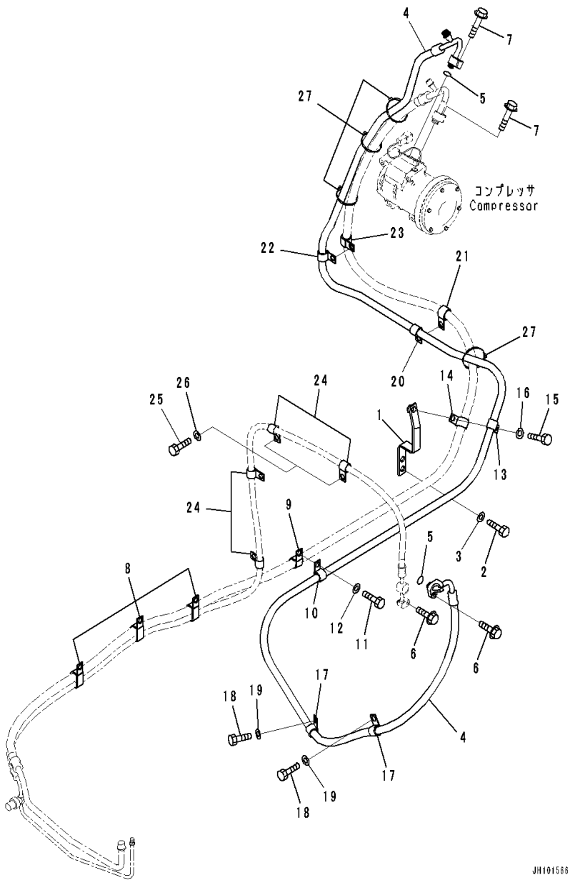
FIG. K0700-001004 Air Conditioner (Cooler Piping)
