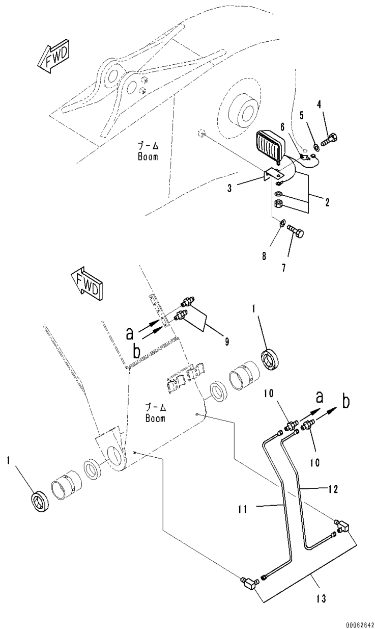
FIG. T1110-001007 Boom (Working Lamp)
