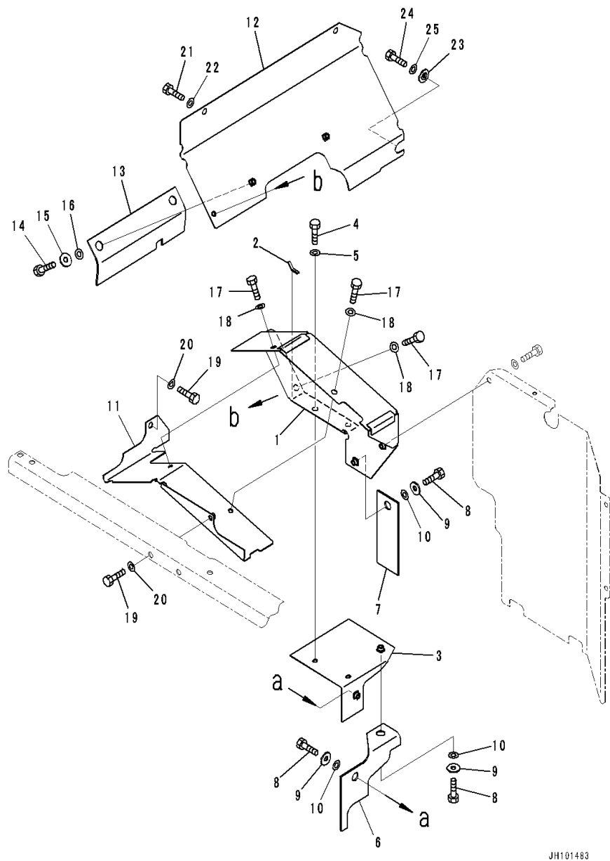
FIG. M1150-002003 Partition
