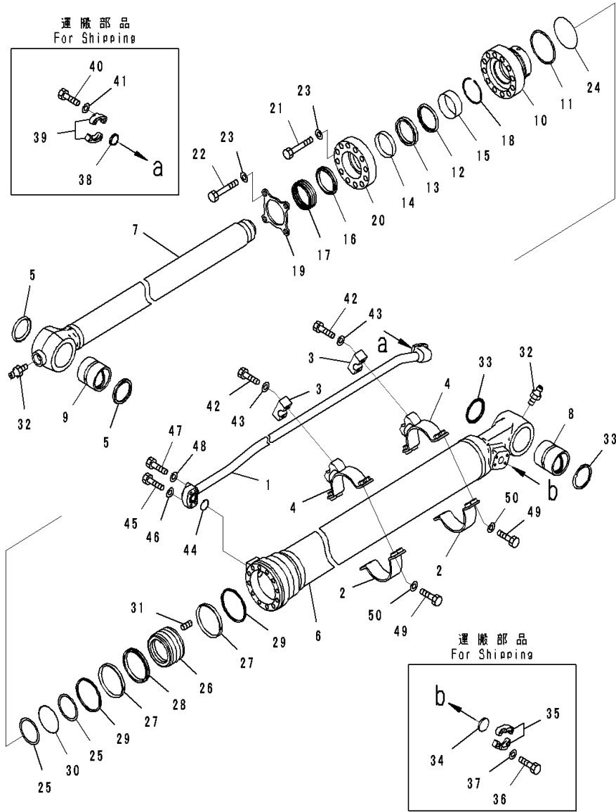
FIG. T1200-003002 Arm (100 Hours Lubrication Interval, Multi Dust Cylinder) (Inner Parts, Bucket Cylinder)
