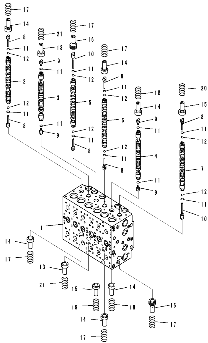
FIG. H0120-002001 Control Valve (7-Spool, 1/21)
