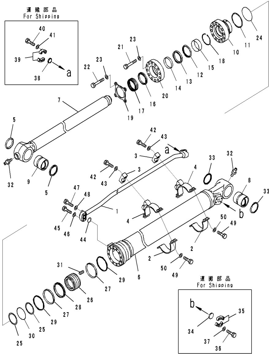
FIG. T1200-002003 Arm (100 Hours Lubrication Interval, Multi Dust Cylinder) (Inner Parts, Bucket Cylinder)
