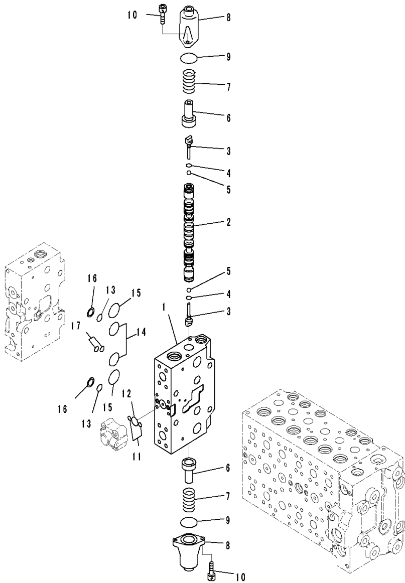
FIG. H0120-002018 Control Valve (7-Spool, 18/21)
