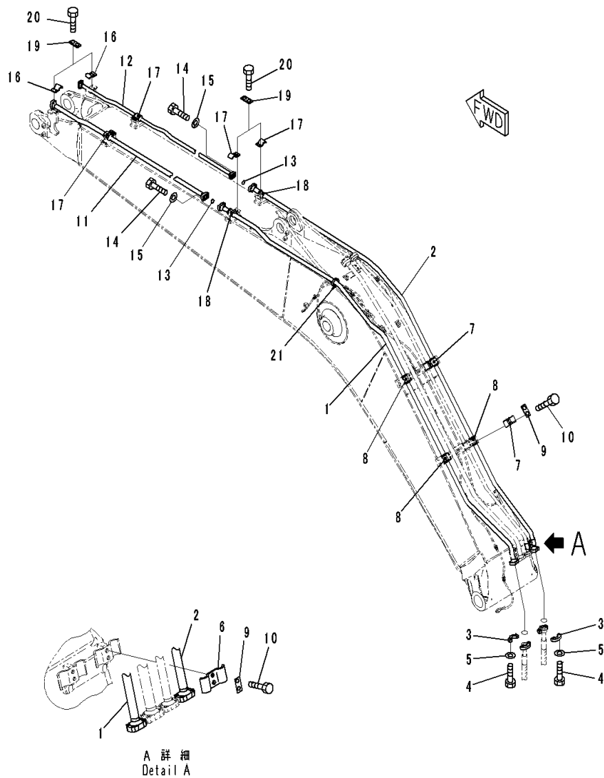
FIG. T1110-002004 Boom (Bucket Cylinder Piping)
