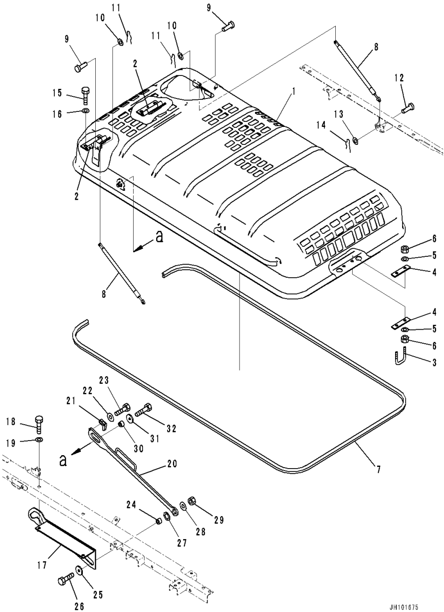
FIG. M1110-001001 Engine Hood
