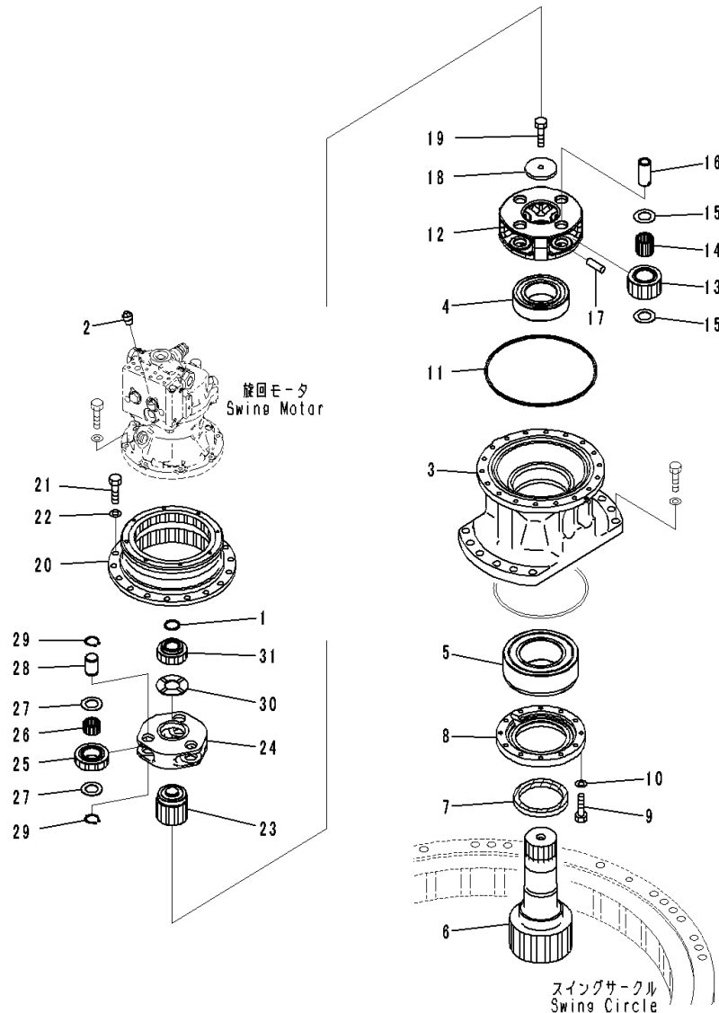
FIG. N1210-001004 Swing Machinery and Motor (Oil Resistance) (Mounting)
