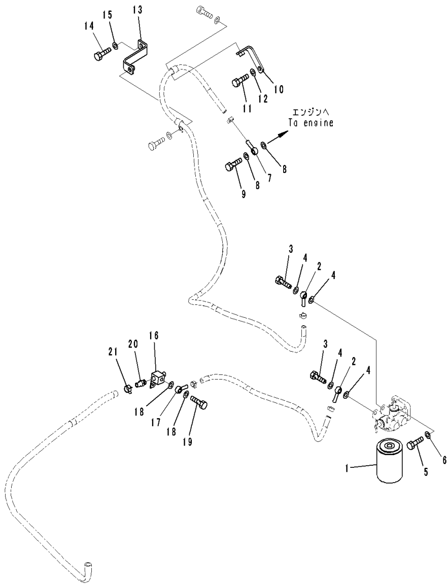
FIG. B0930-001002 Coolant Filter (Bracket)
