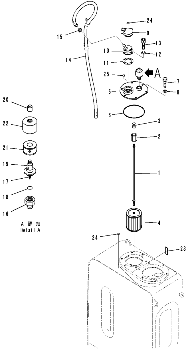
FIG. H0110-002002 Hydraulic Tank (Breather)
