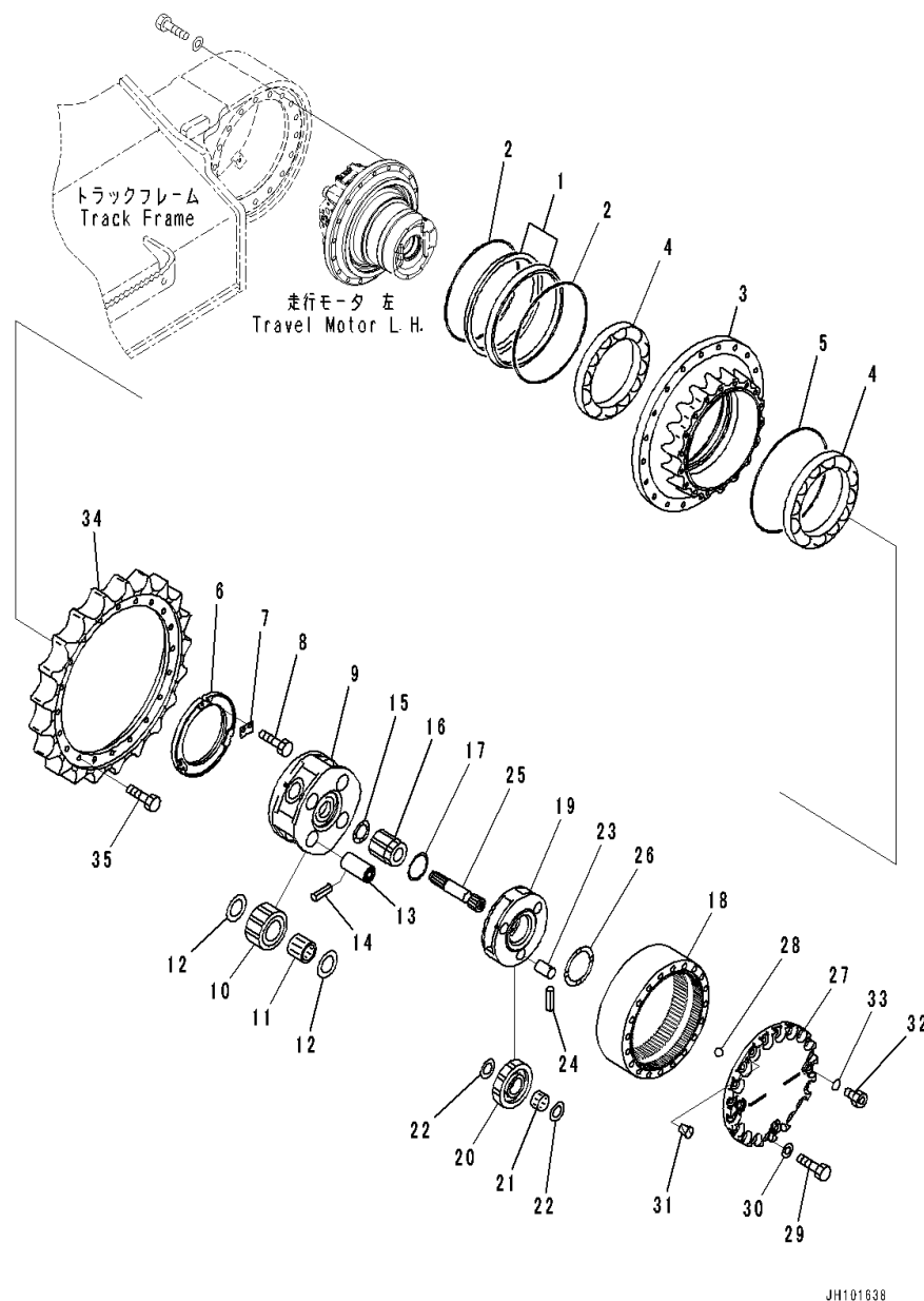
FIG. P1210-001003 Travel Motor and Final Drive (Final Drive L.H.)
