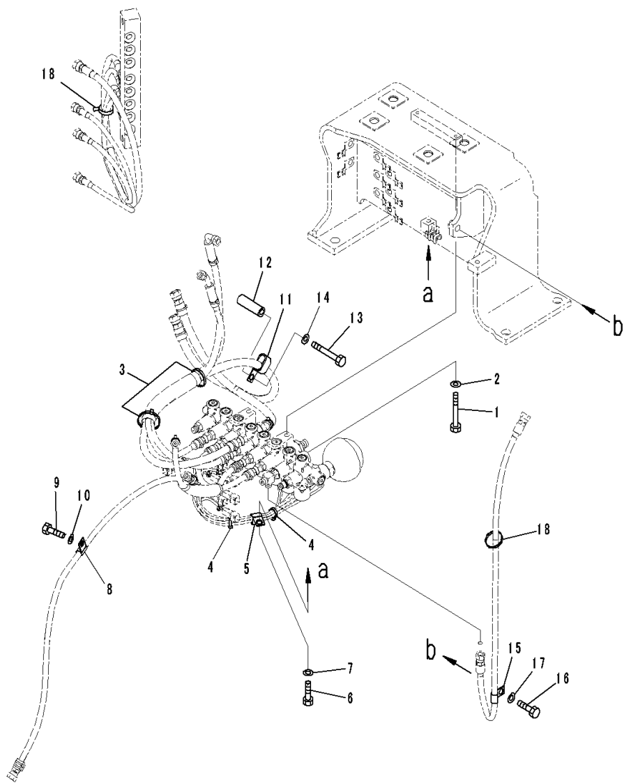
FIG. H1831-001004 Solenoid Valve (Mounting)
