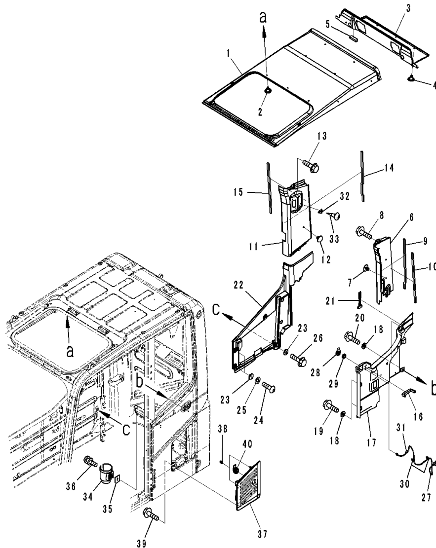
FIG. K1110-001011 Cab (Roof Cover, Hanger, Drink Holder and Air Intake)
