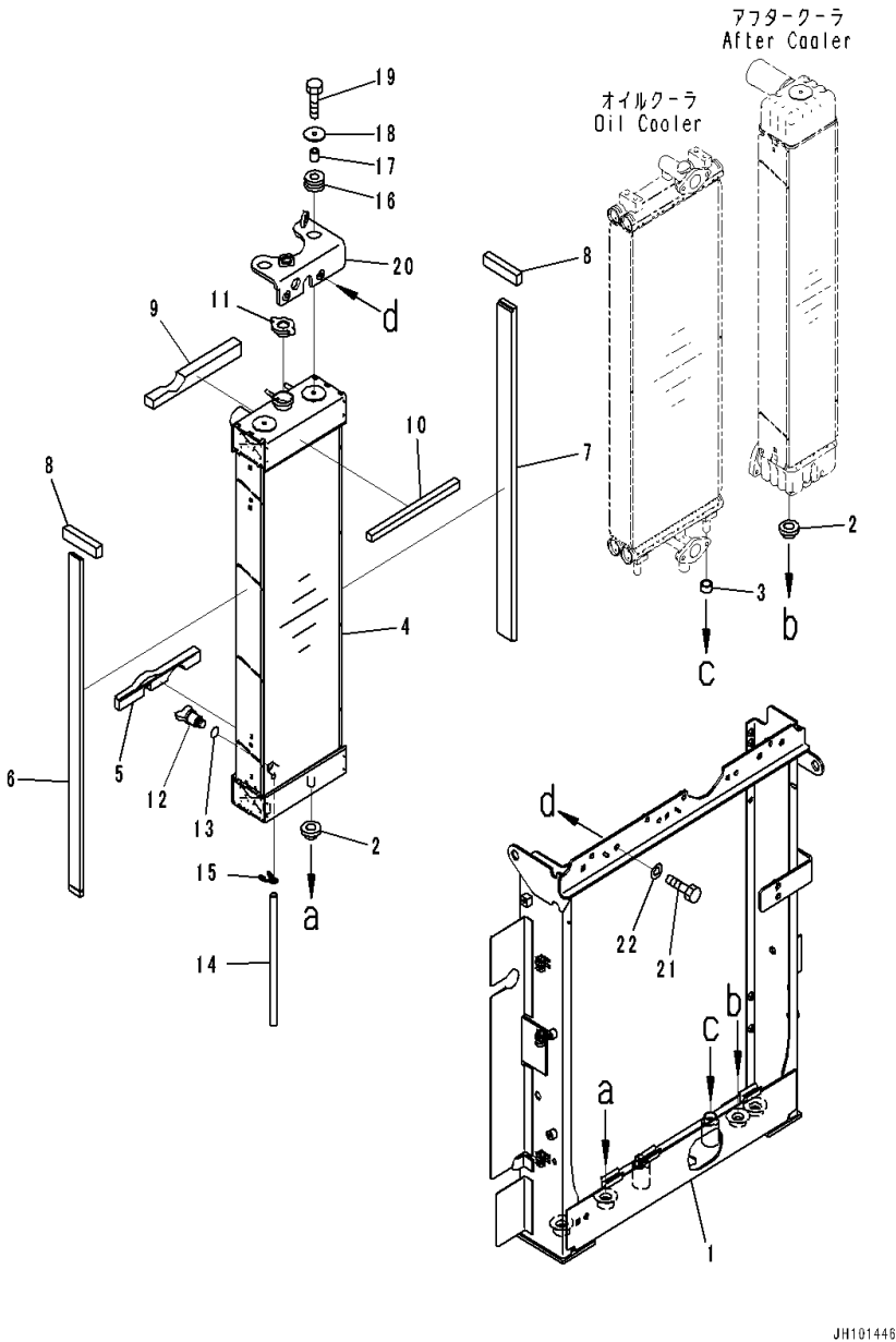
FIG. C0100-001001 Cooling System (Radiator)
