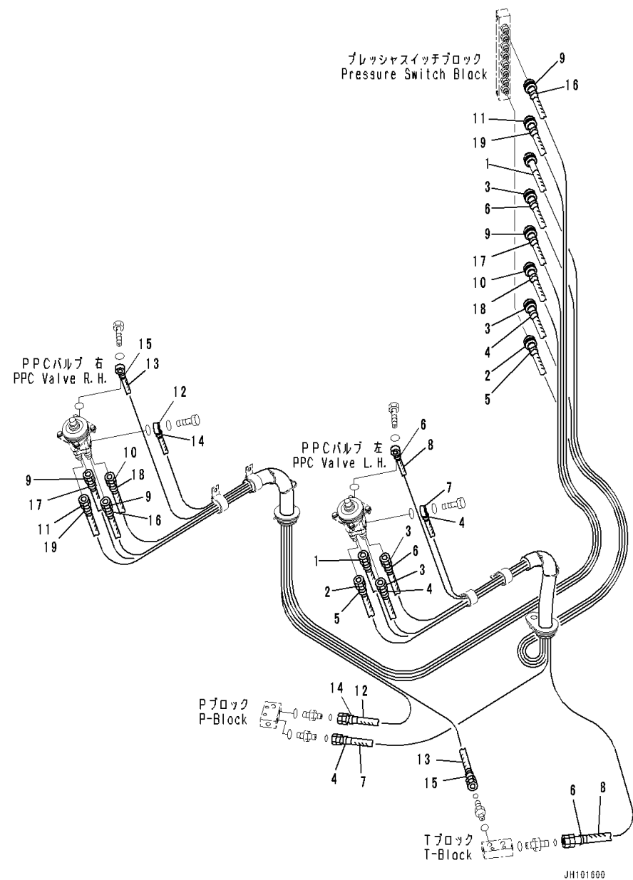
FIG. K1110-001054 Cab (Floor, PPC Valve Piping for Work Equipment)
