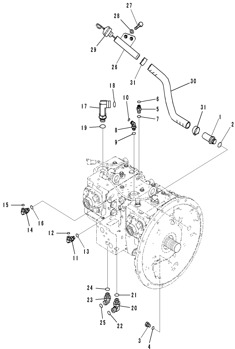
FIG. H0210-001001 Hydraulic Pump (Related Parts)
