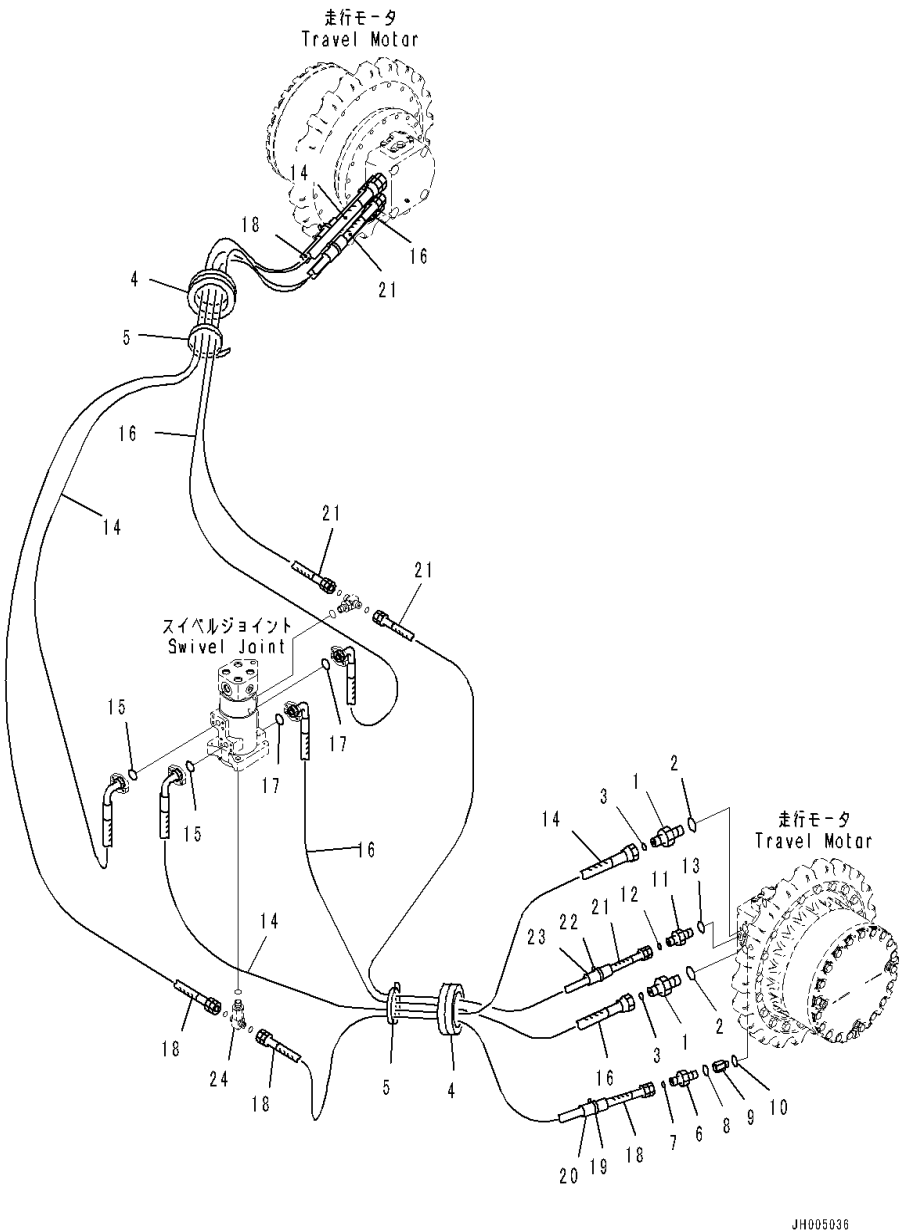
FIG. P1120-002001 Travel Piping, Long Track Frame
