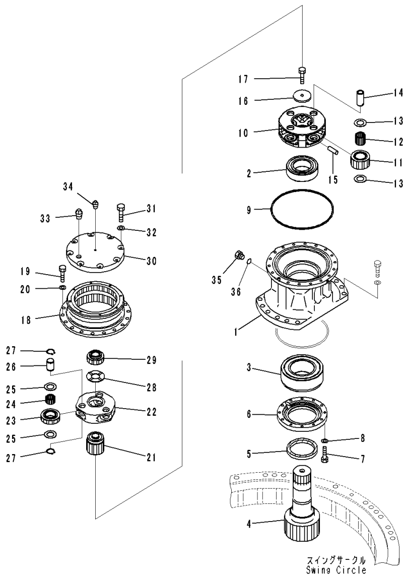
FIG. N1210-002001 Swing Machinery and Motor (Supply Only, Oil Resistance)
