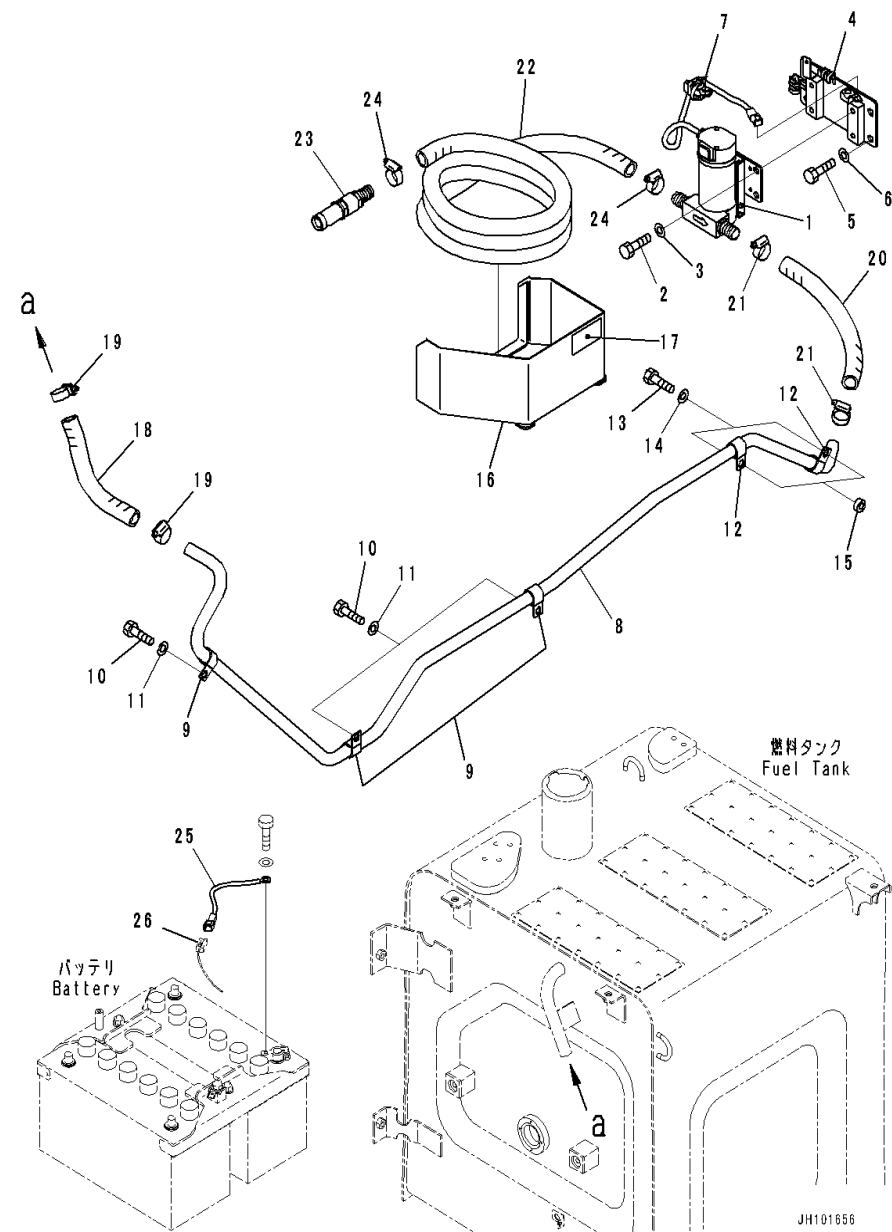
FIG. W1113-001001 Refueling Pump
