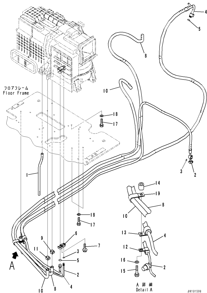
FIG. K1110-001052 Cab (Floor, Air Conditioner Piping)
