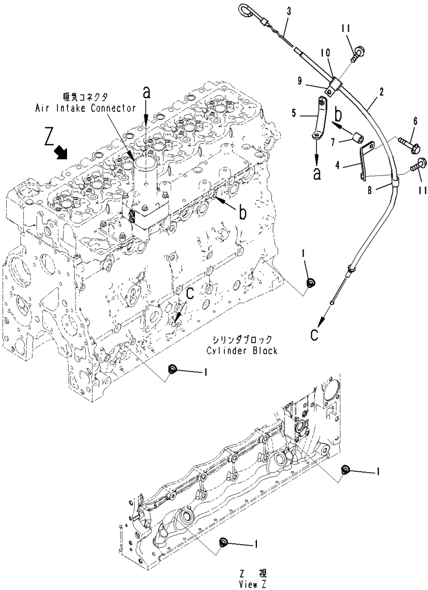
FIG. ALG00-001001 Oil Level Gauge
