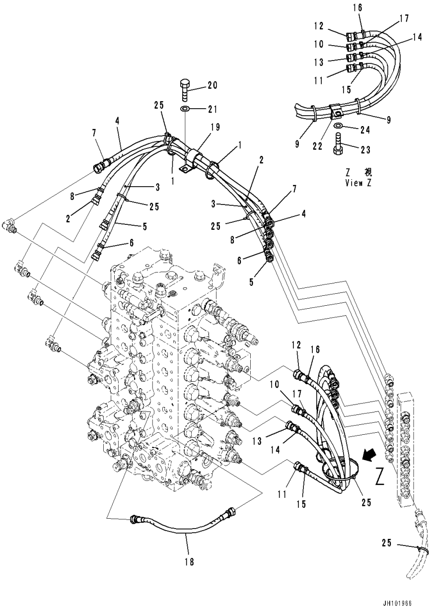
FIG. H1840-001001 Proportional Pressure Control (PPC) Main Piping
