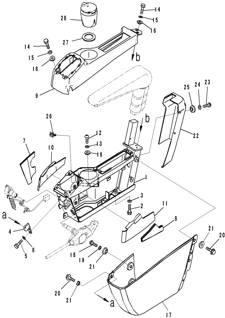
FIG. K1110-001040 Cab (Floor, PPC Valve Mounting for Work Equipment, L.H., 2/2)
