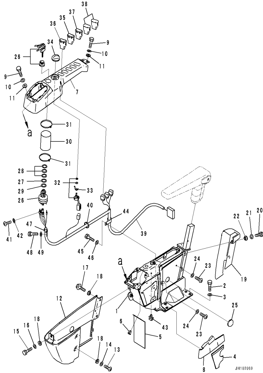
FIG. K1110-003047 Cab (With Amber Color Warning Beacon) (Floor, Console, R.H., With Beacon Lamp)
