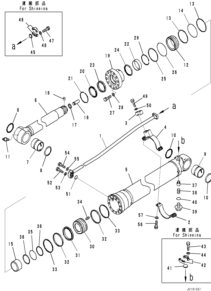
FIG. T1140-001001 Arm Cylinder (Inner Parts, Arm Cylinder) (100 Hours Lubrication Interval)
