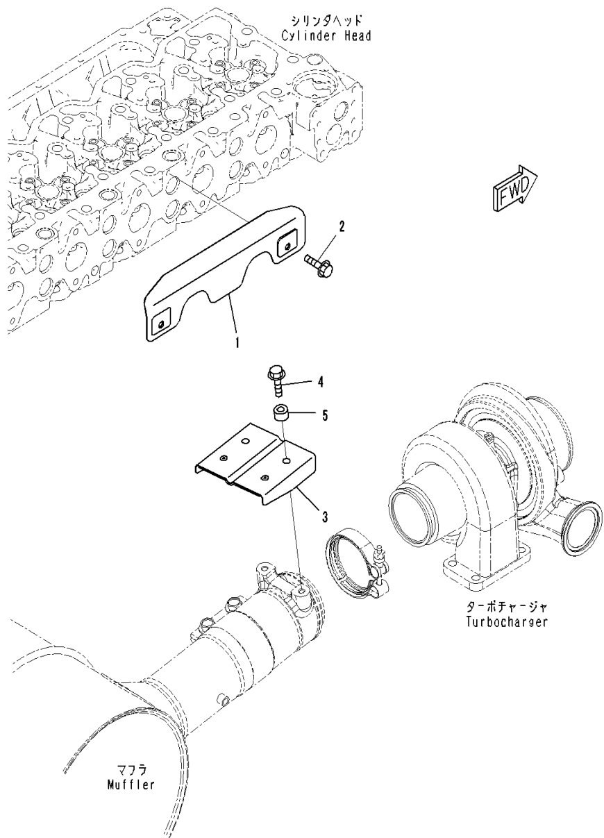
FIG. A1570-001001 Heat Shield
