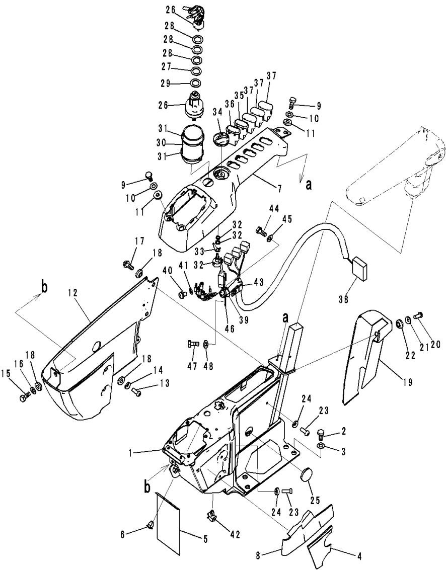
FIG. K1110-001046 Cab (Floor, Console, R.H.)
