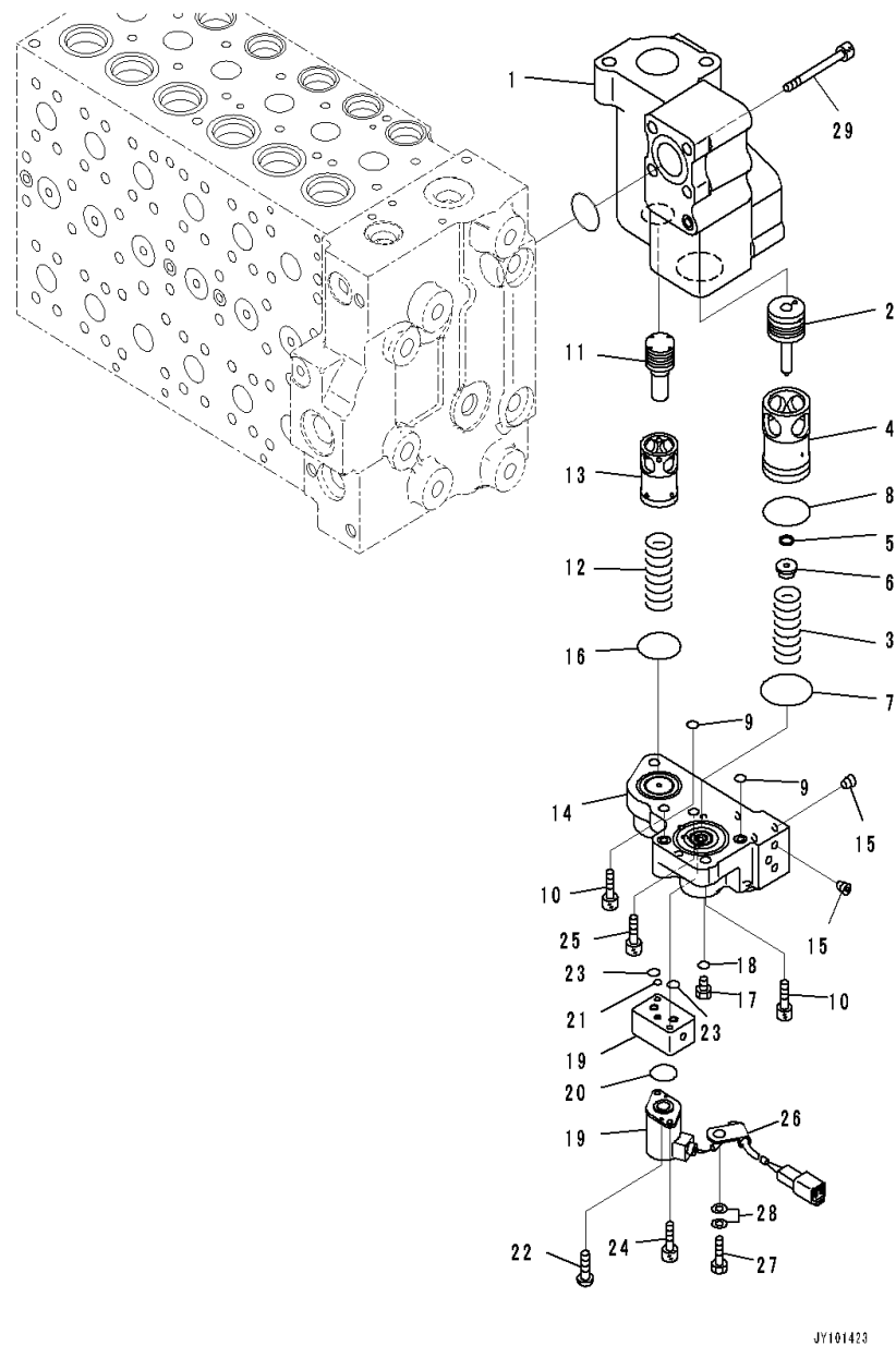
FIG. H0120-002015 Control Valve (7-Spool, 15/21)
