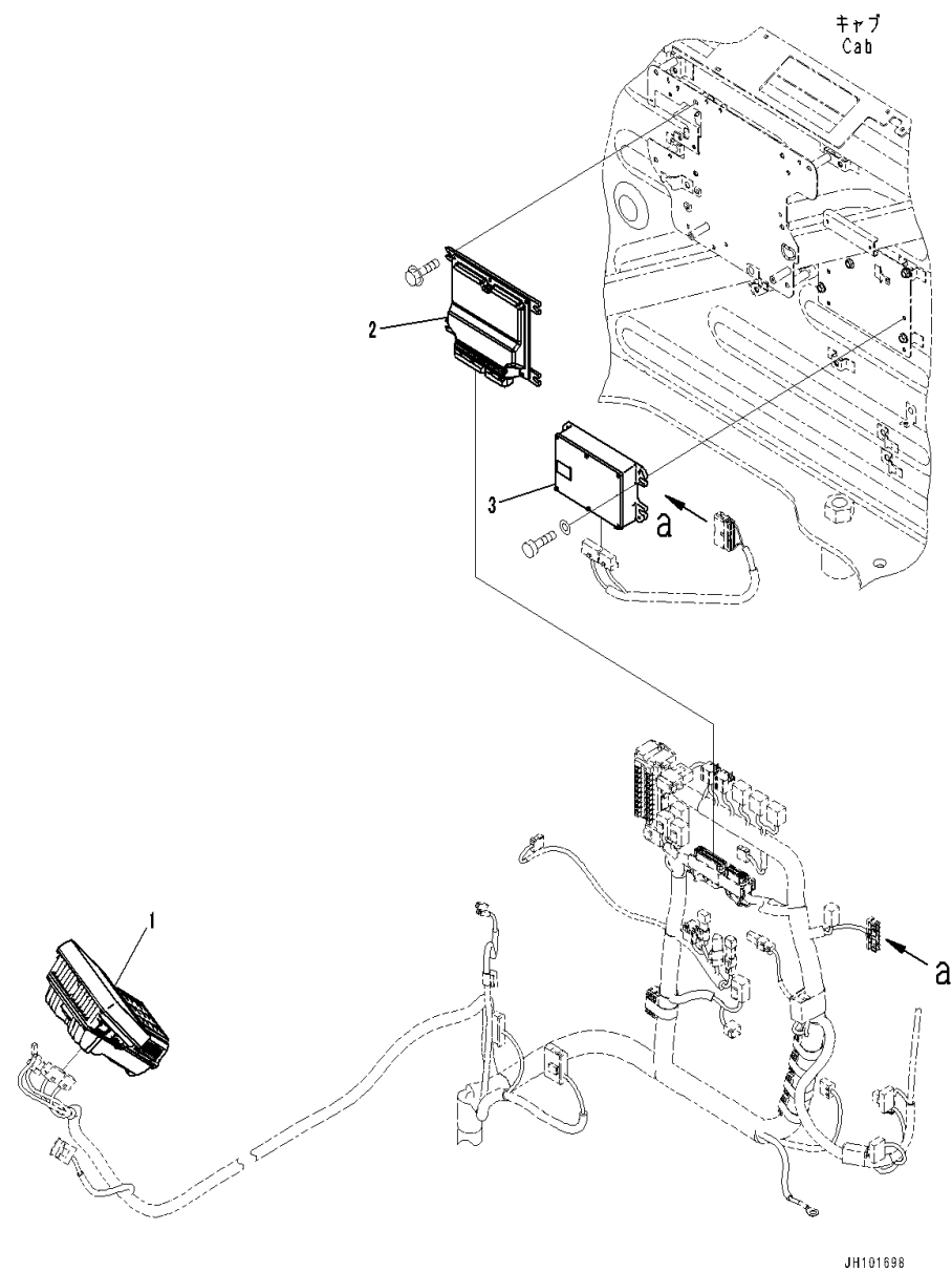
FIG. K1110-001027 Cab (Controller and Monitor)
