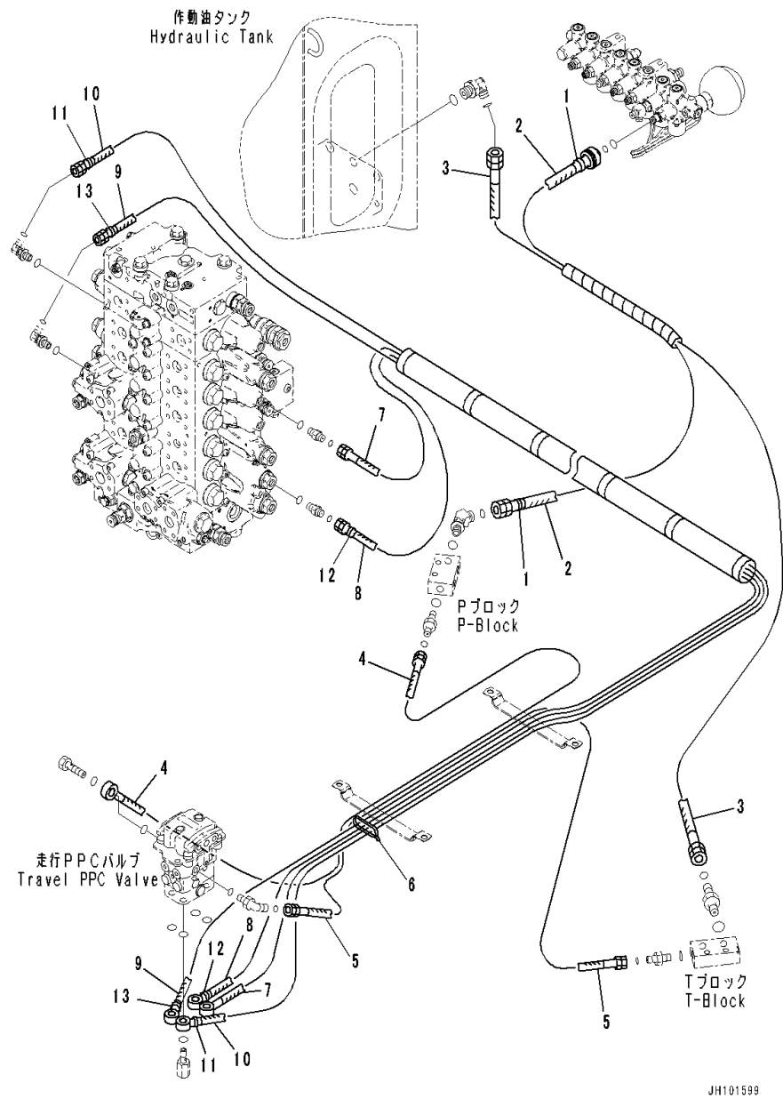
FIG. K1110-001053 CAB (Floor, PPC Valve Piping for Travel)
