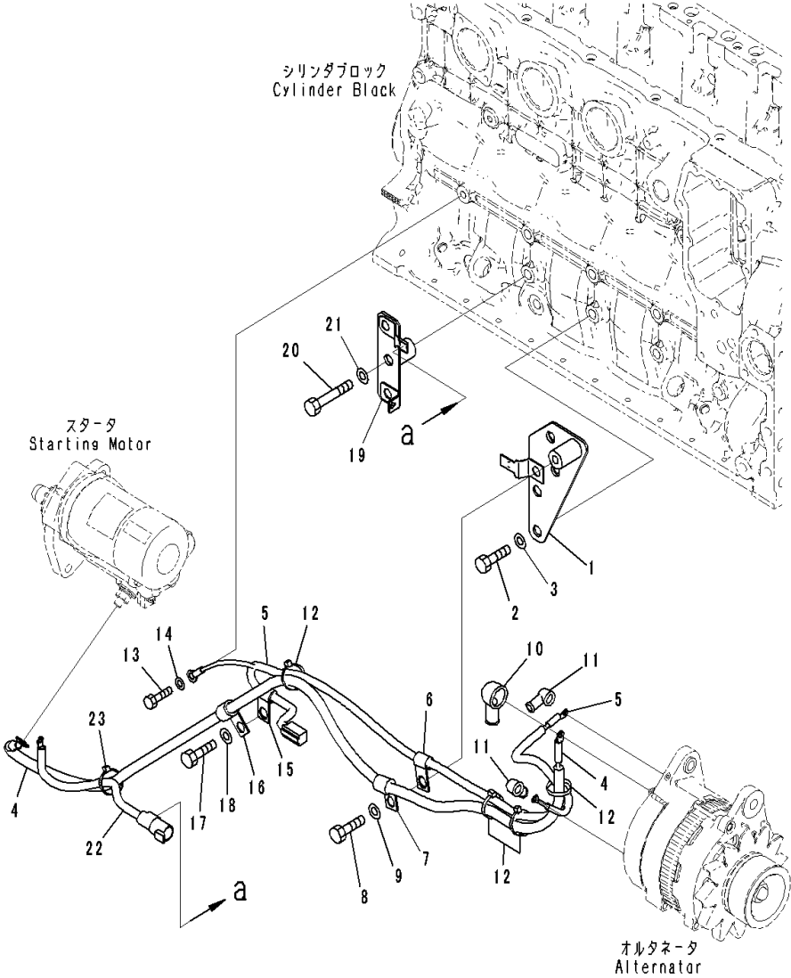
FIG. E0250-001001 Engine Wiring Harness
