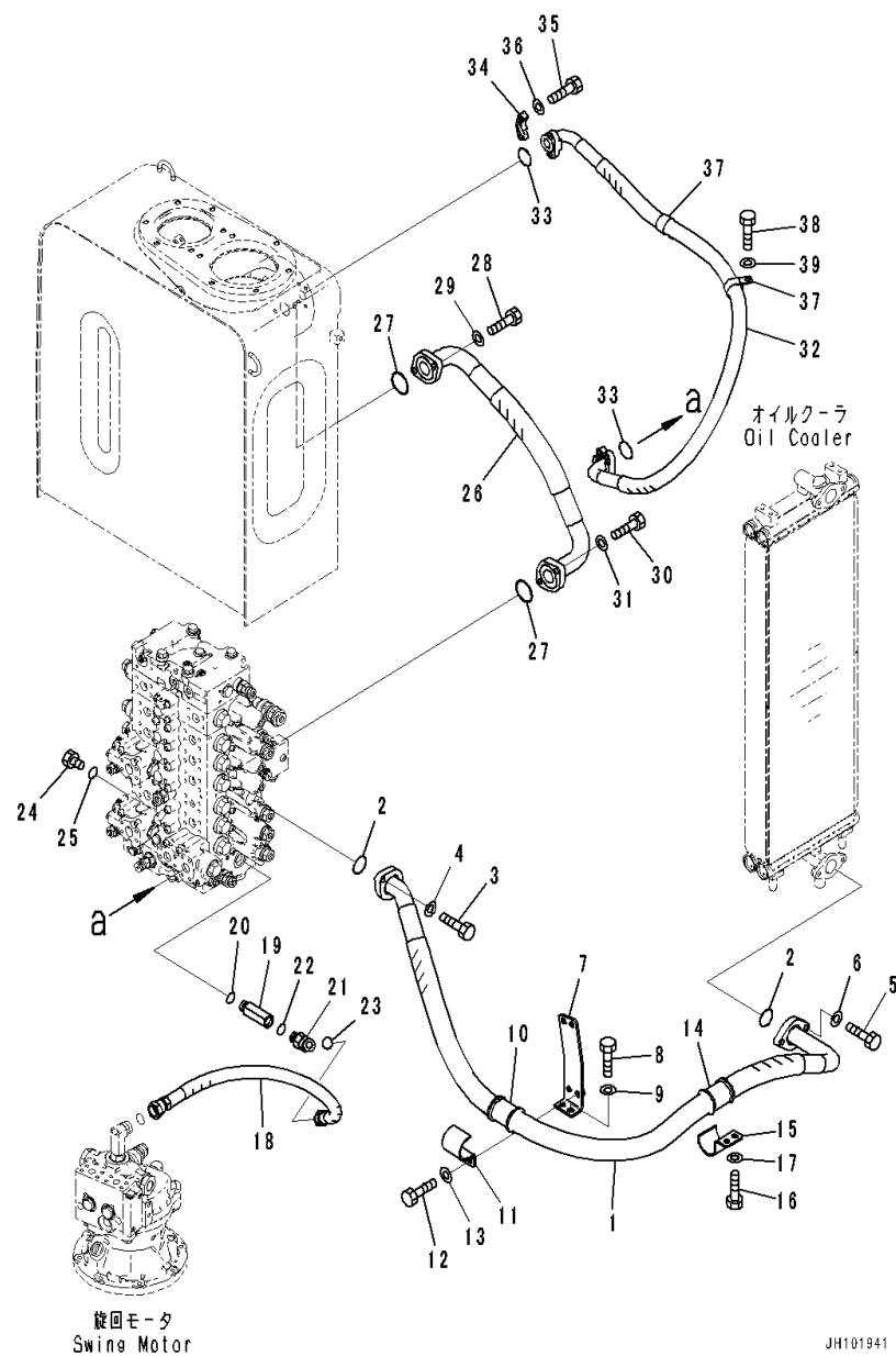
FIG. H0330-002001 Return Piping (1-Additional Actuator Piping, Accumulator)
