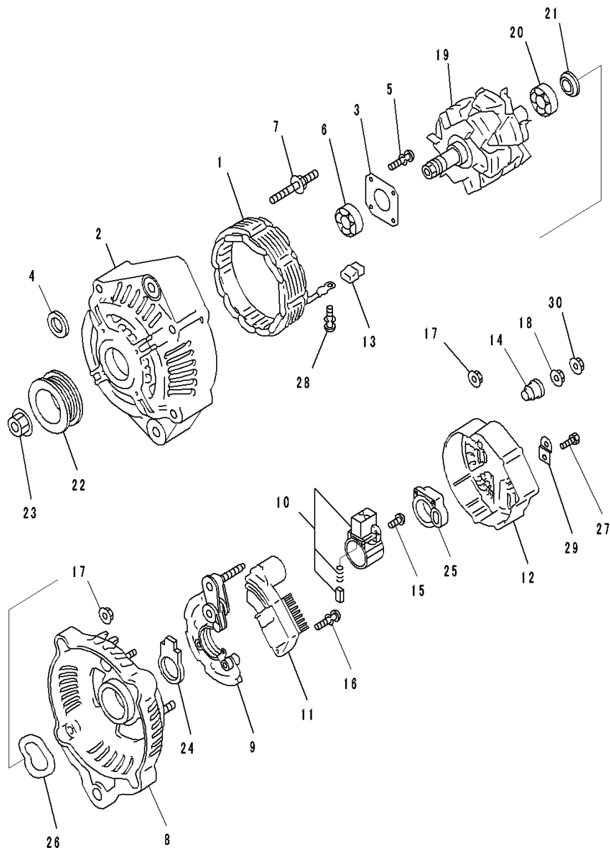
FIG. A6020-002001 Alternator Mounting (35Amp.) (Inner Parts)
