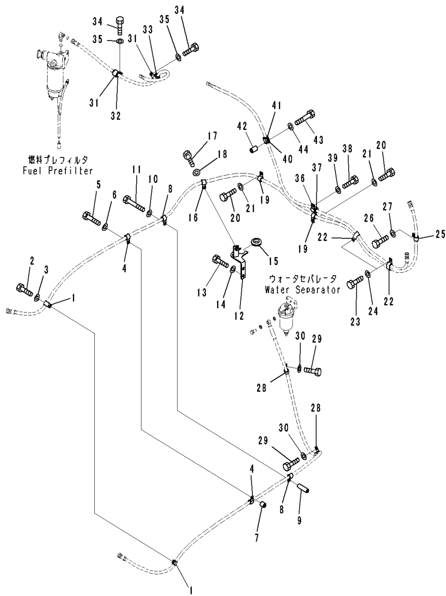
FIG. D0200-001008 Fuel Supply Piping (Clip)
