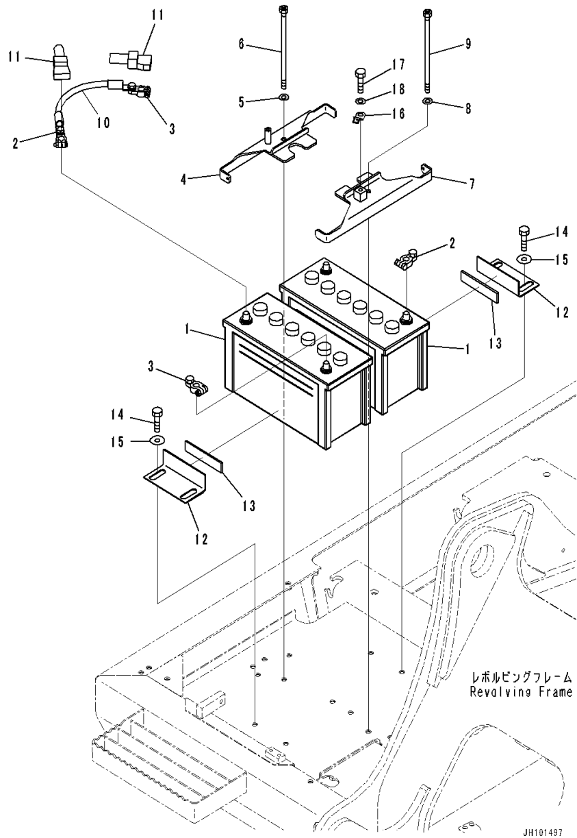
FIG. E0100-001001 Battery
