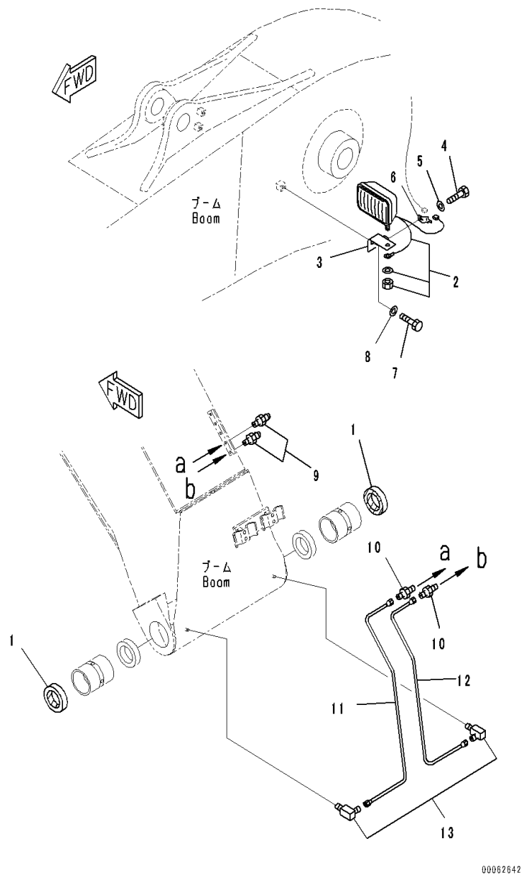
FIG. T1110-002007 Boom (Working Lamp)
