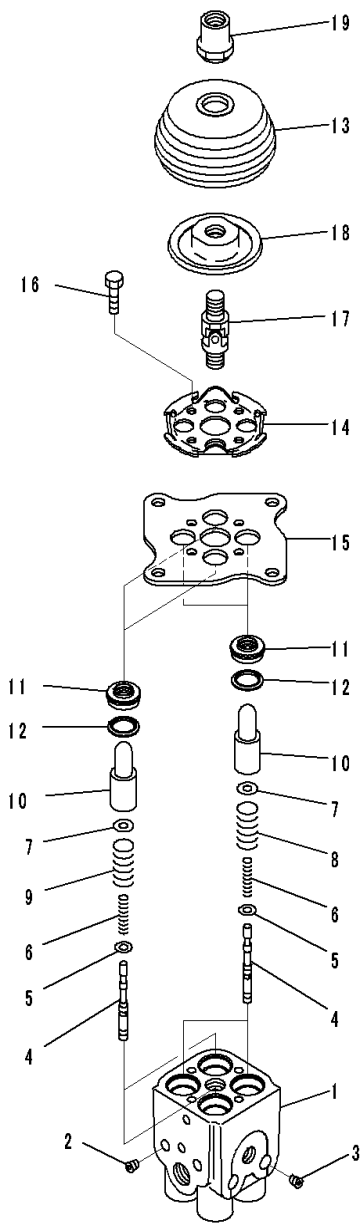
FIG. K1110-001038 Cab (PPC Valve, 2/3, L.H.)
