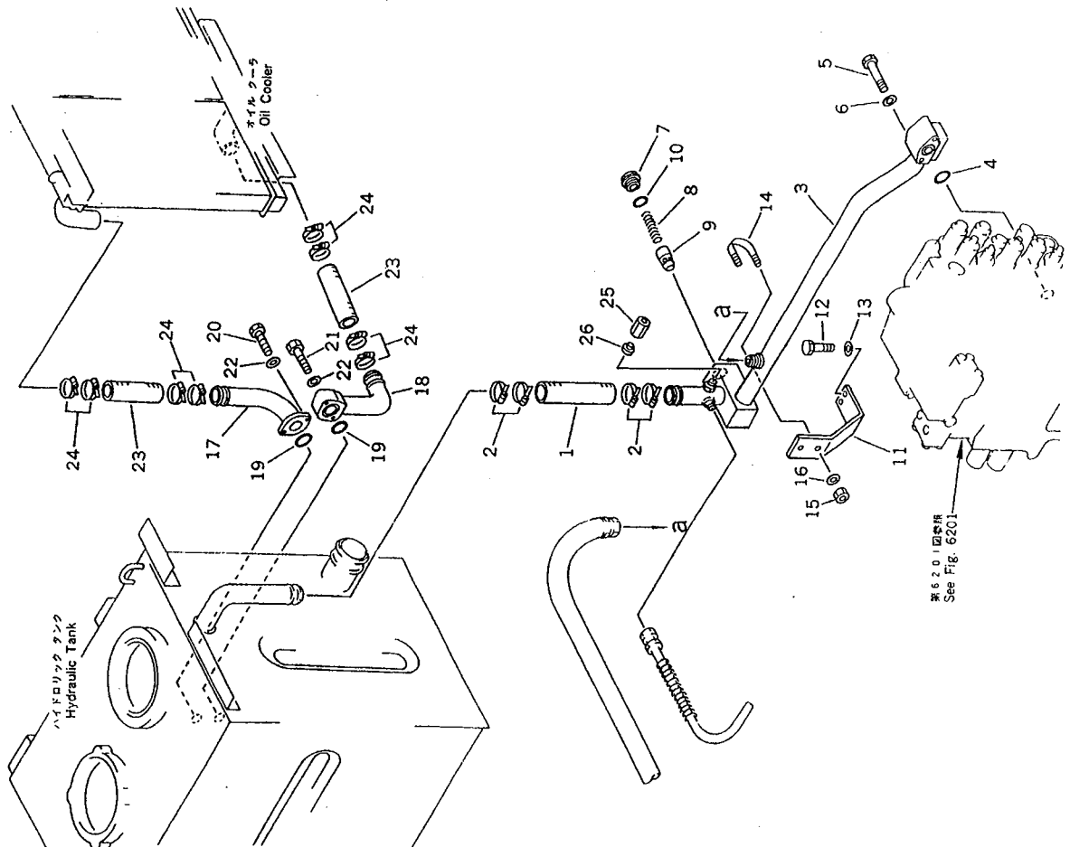
FIG. 6524 HYDRAULIC PIPING (RETURN AND OIL COOLER) (WITHOUT AUTO DECELERATION) (WITHOUT SWING MECHANICAL BRAKE) (PC240)
