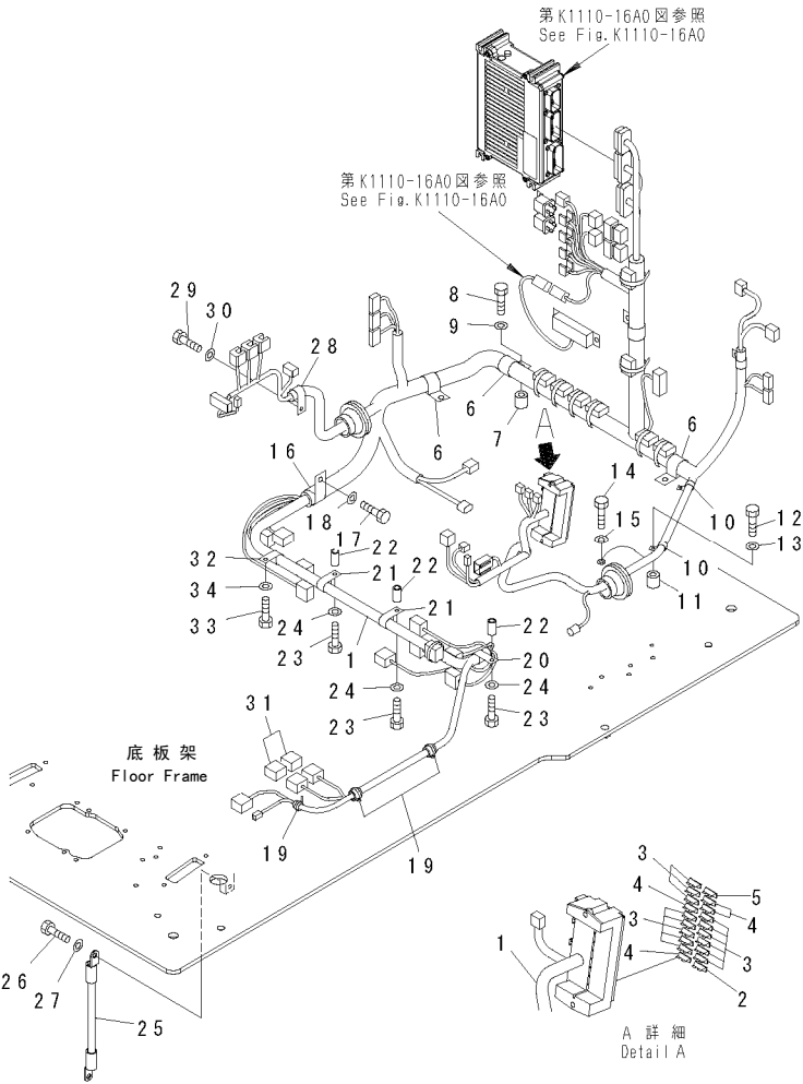
FIG.K1110-23A0 FLOOR FRAME (OPERATOR'S CAB) (WINDOW WASHER) 地板架（驾驶室）（洗窗器）
