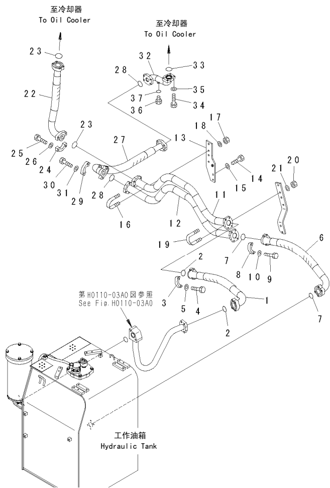
FIG. H0320-01A0 OIL COOLER LINES 油冷却回路
