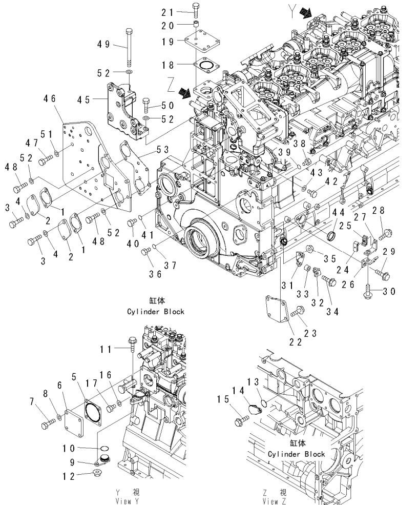
FIG. A1550-A4B1 COVER FOR EGR LESS 无EGR用盖板
