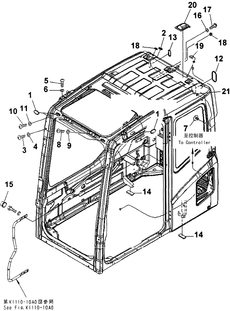
FIG.K1110-11A0 FLOOR FRAME (OPERATOR'S CAB) (PLUG BOLT AND ANTENNA) 底板架（驾驶室）（螺塞和天线）
