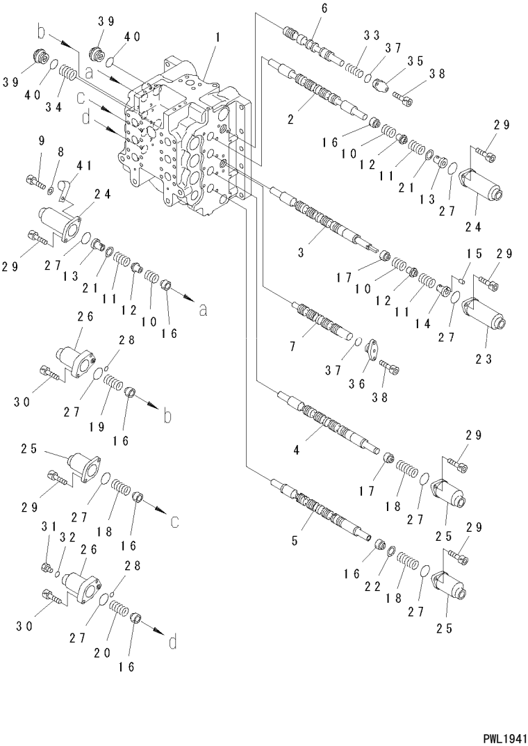
FIG. Y1660-05A0 MAIN VALVE (5/8) 主阀 (5/8)
