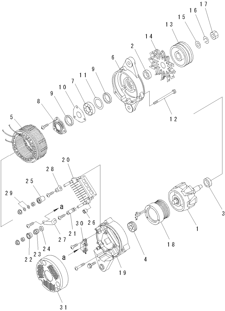
FIG. A6010-B4N2 ALTERNATOR (60A) (SANDY AND DUSTY SPEC.) (INNER PARTS) 发电机 (60A) (沙尘地仕样) (内部品)
