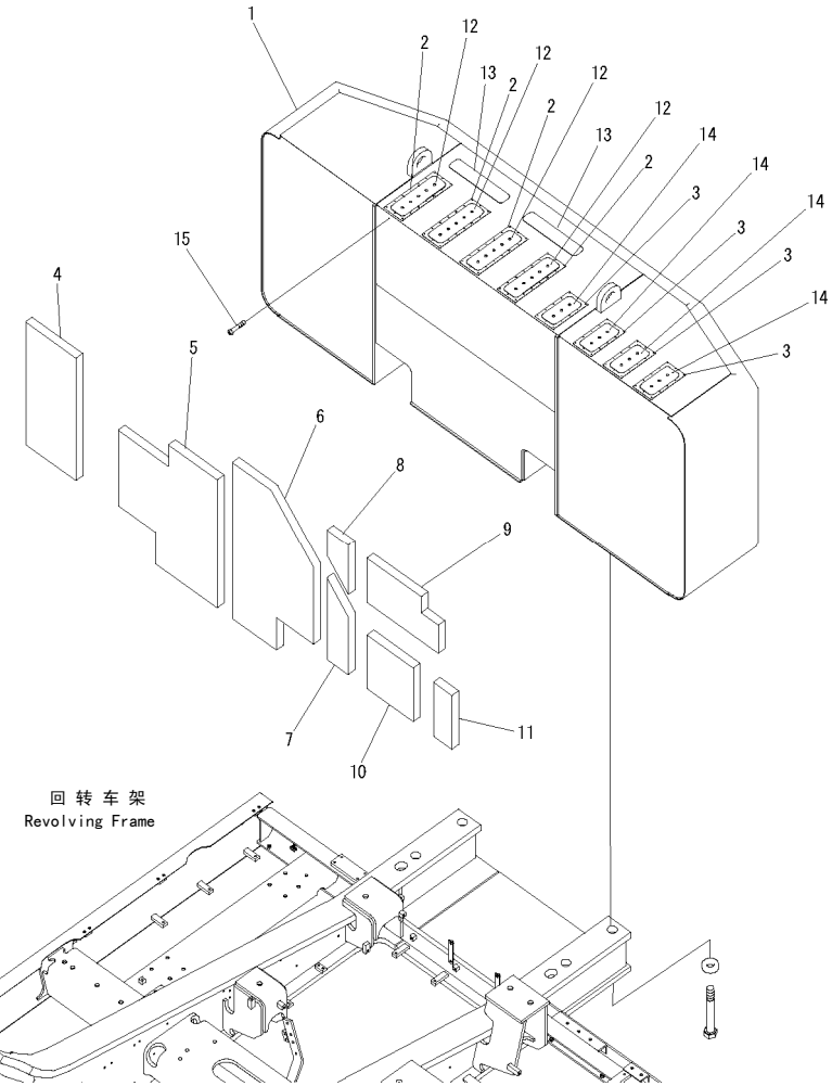
FIG. M1510-01A0 COUNTER WEIGHT (10750KG) 配重(10750KG)
