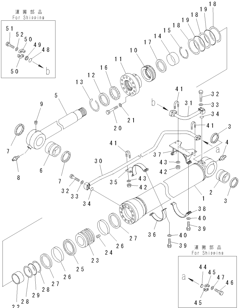
FIG. Y1620-41A0 BUCKET CYLINDER 铲斗油缸
