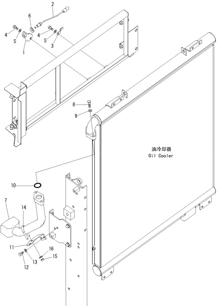
FIG. C0100-11A0 COOLING (SENSOR AND OIL COOLER TUBE) 冷却 (传感器和油冷却器管)
