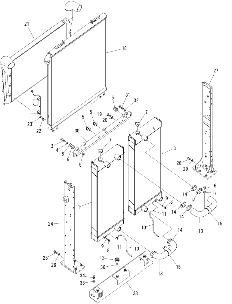
FIG. C0100-01A0 COOLING (RADIATOR ,OIL COOLER AND AFTER COOLER) 冷却(散热器、油冷却器和后冷器)
