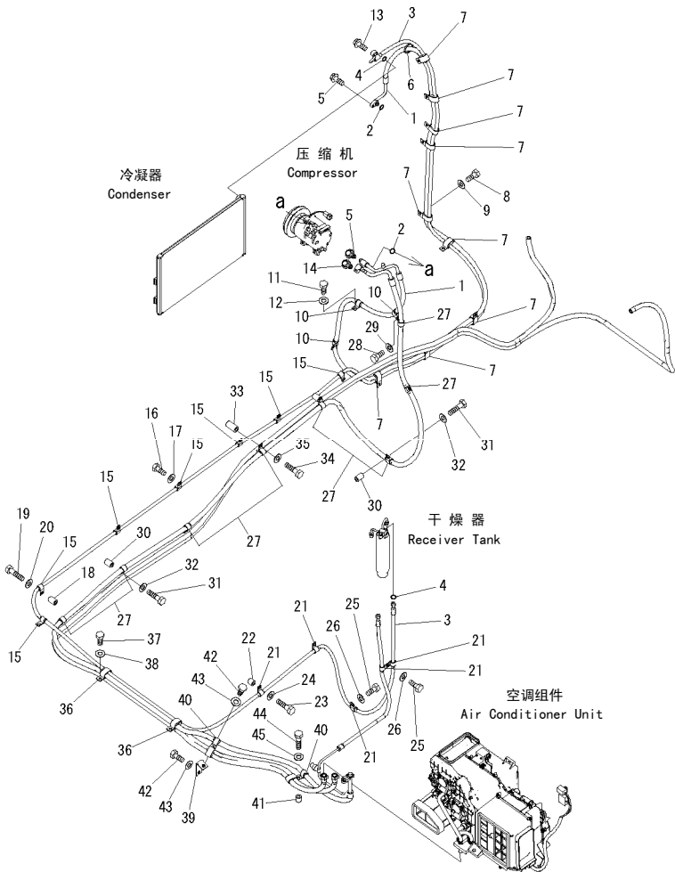
FIG. K0700-02A0 AIR CONDITIONER (HEATER HOSE AND CLAMP) 空调（加热器软管和卡箍）
