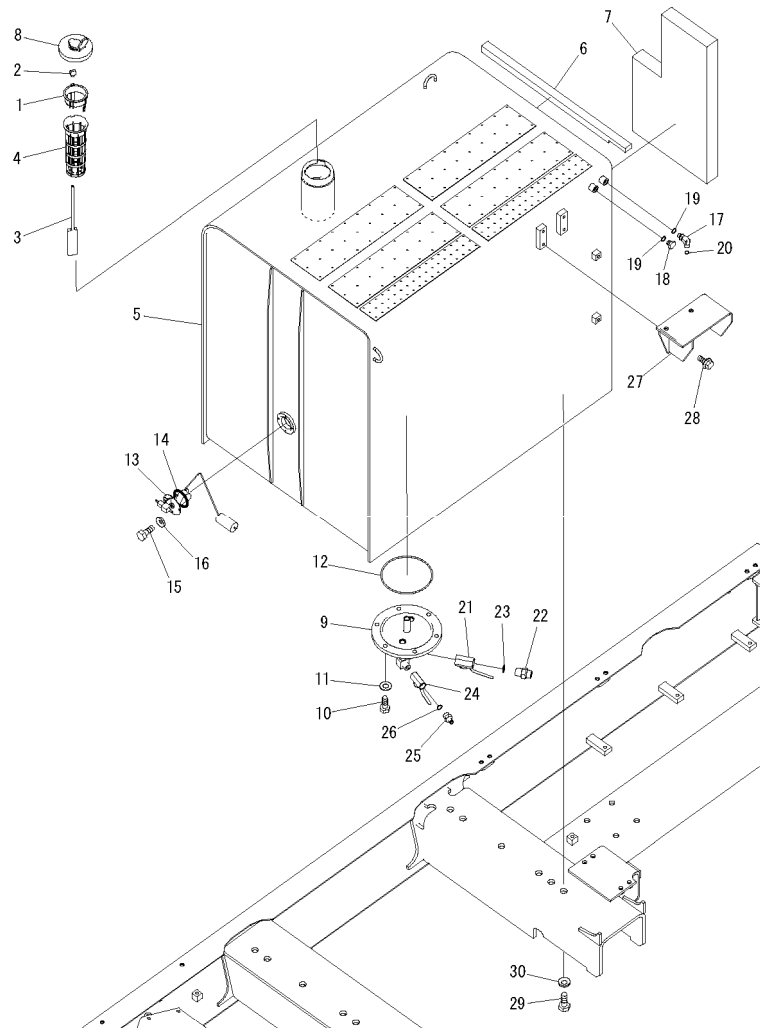
FIG. D0100-01A0 FUEL TANK 燃油箱
