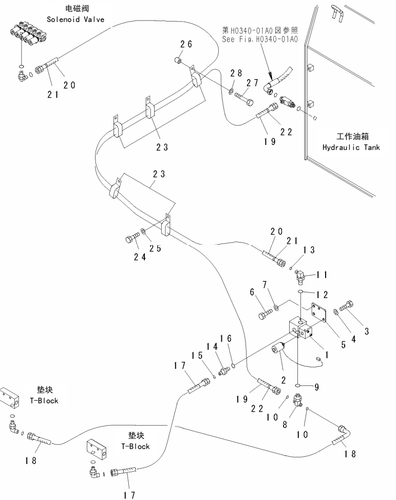
FIG. H1840-02A0 PPC MAIN LINE (PPC LOCK SOLENOID VALVE) PPC主油路 (PPC锁定电磁阀)
