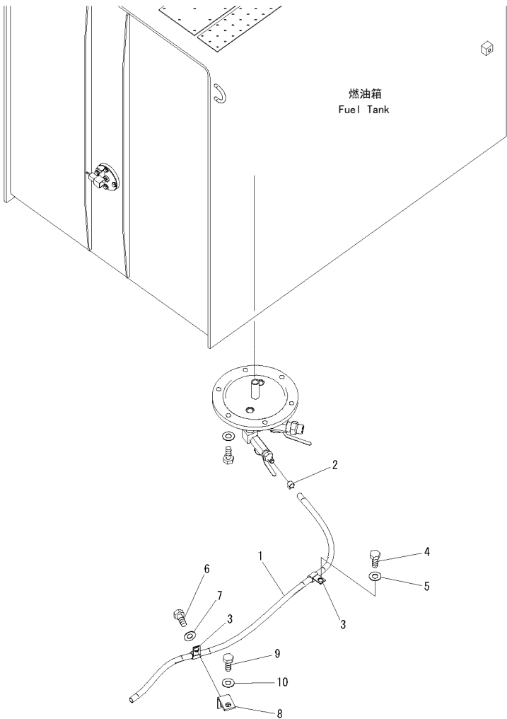
FIG.D0200-04A0 FUEL LINE (DRAIN PIPING) 燃油回路(放油管路)
