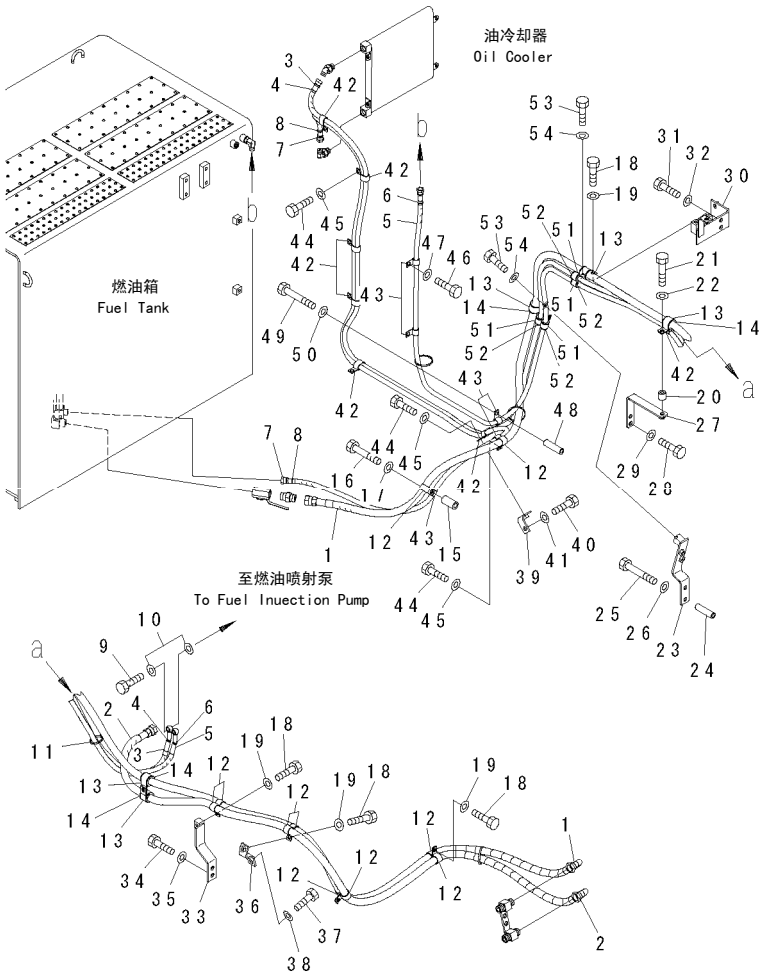
FIG.D0200-01A0 FUEL LINE (FUEL HOSE) 燃油管路(燃油管)
