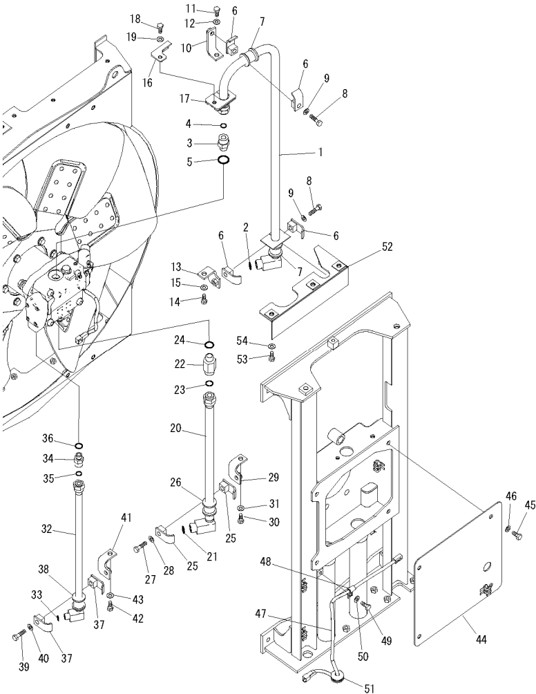
FIG. C0100-06A0 COOLING (FAN MOUNT) (FAN MOTOR PIPING) 冷却 (风扇安装) (风扇马达管路)
