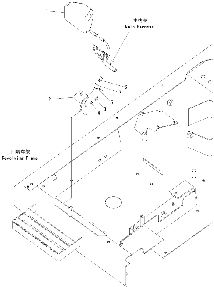
FIG. E0200-06A0 WIRING (WORKING LAMP ,FRONT) 线束(前工作灯)
