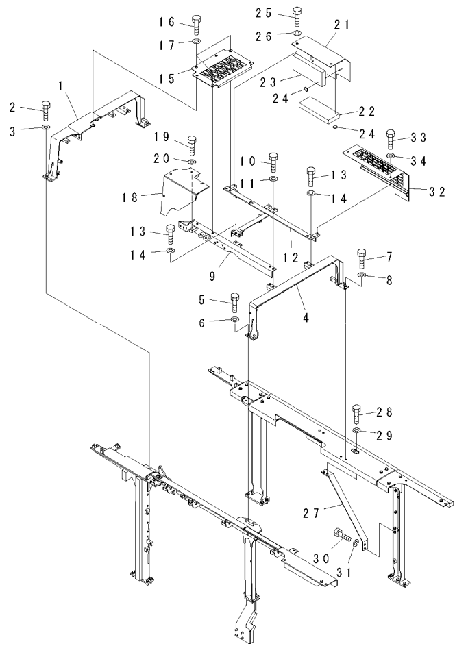
FIG. M1120-02A0 FRAME (MACHINE CAB) (ADDITIONAL FILTER SPEC.) (STEP AND COVER) 支架 (机罩) (附加滤清器仕样) (踏板和盖)
