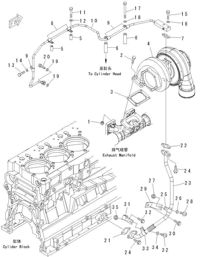
FIG. A1530-A4L8 TURBOCHARGER MOUNTING AND LUBRICATOR 涡轮增压器安装和润滑
