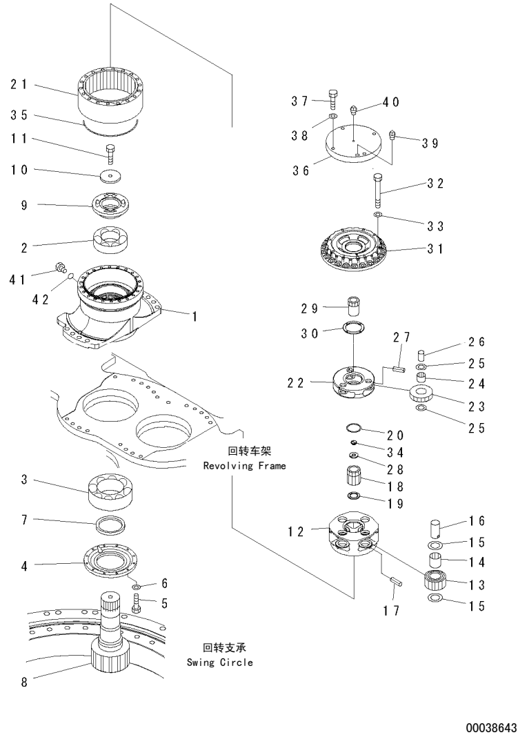
FIG. Y0260-01A0 SWING MACHINERY ASS'Y (SUPPLY PARTS) 回转减速机 (配件)
