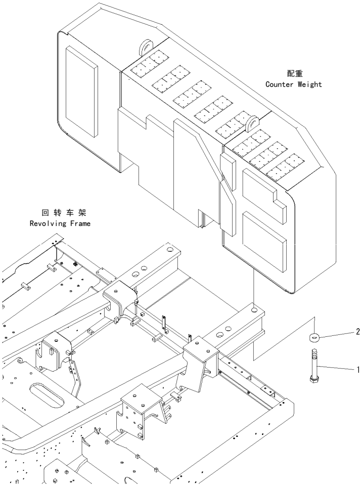
FIG. M1520-01A0 COUNTER WEIGHT MOUNTING 配重安装
