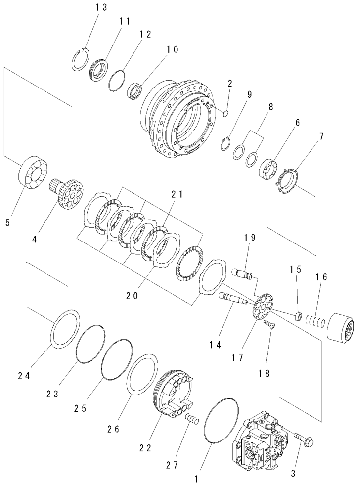
FIG. Y1641-02A0 TRAVEL MOTOR (2/3) 行走马达 (2/3)
