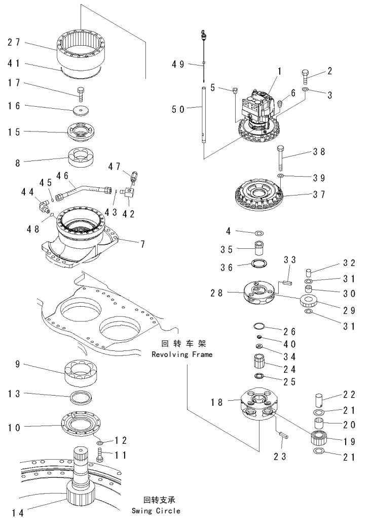
FIG. N1210-03A0 SWING MACHINERY (L. H.) 回转减速器(左)
