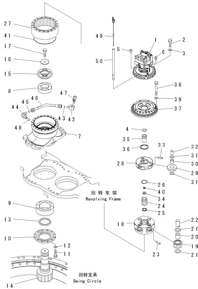
FIG. N1210-01A0 SWING MACHINERY (R. H.) 回转减速器(右)
