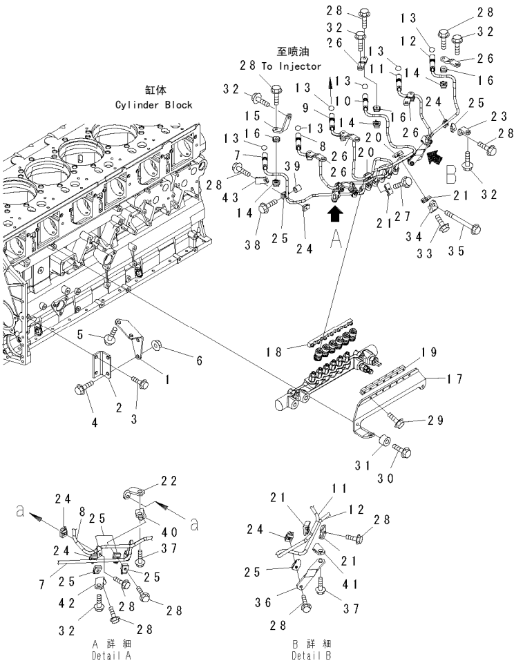
FIG. A4030-A4C1 FUEL SUPPLY PUMP BRACKET AND PIPING 燃油泵支架和油管
