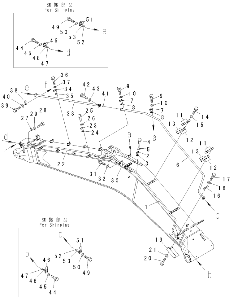
FIG. T1110-04A5 BOOM (7.3M) (BUCKET CYLINDER LINE) 大臂(7.3M)(铲斗油缸回路)
