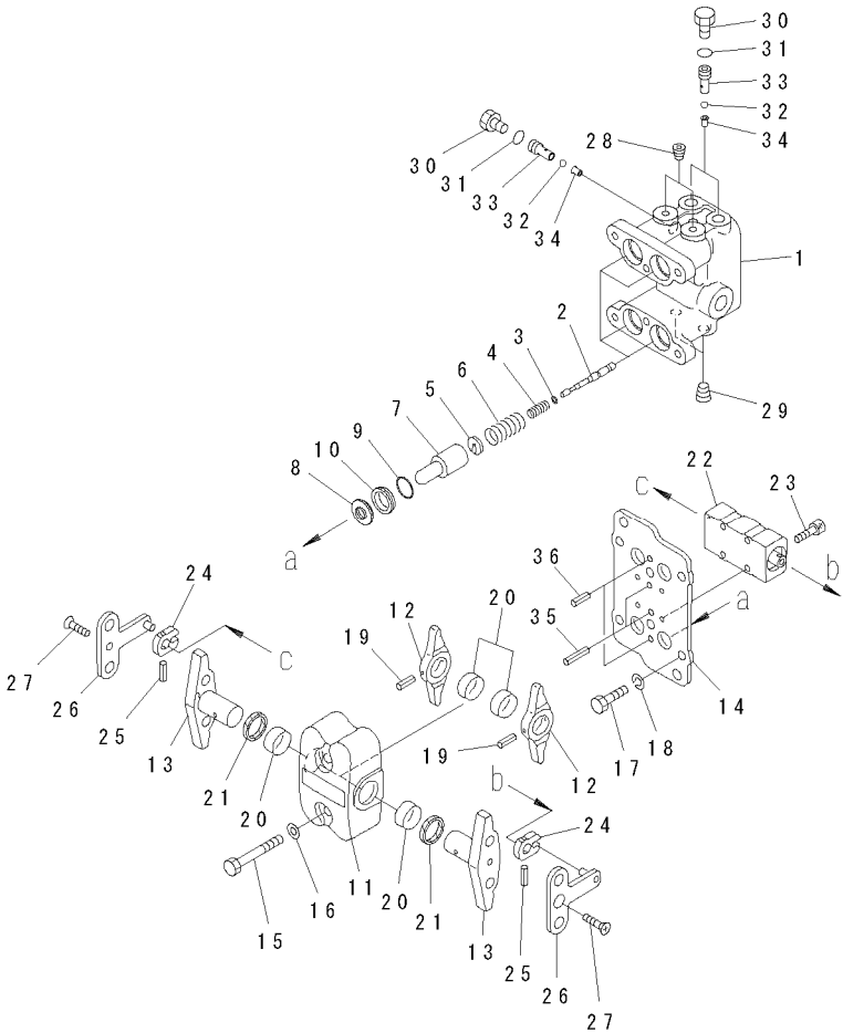
FIG. Y1670-01A0 PPC VALVE (FOR TRAVEL) PPC阀(行走用)
