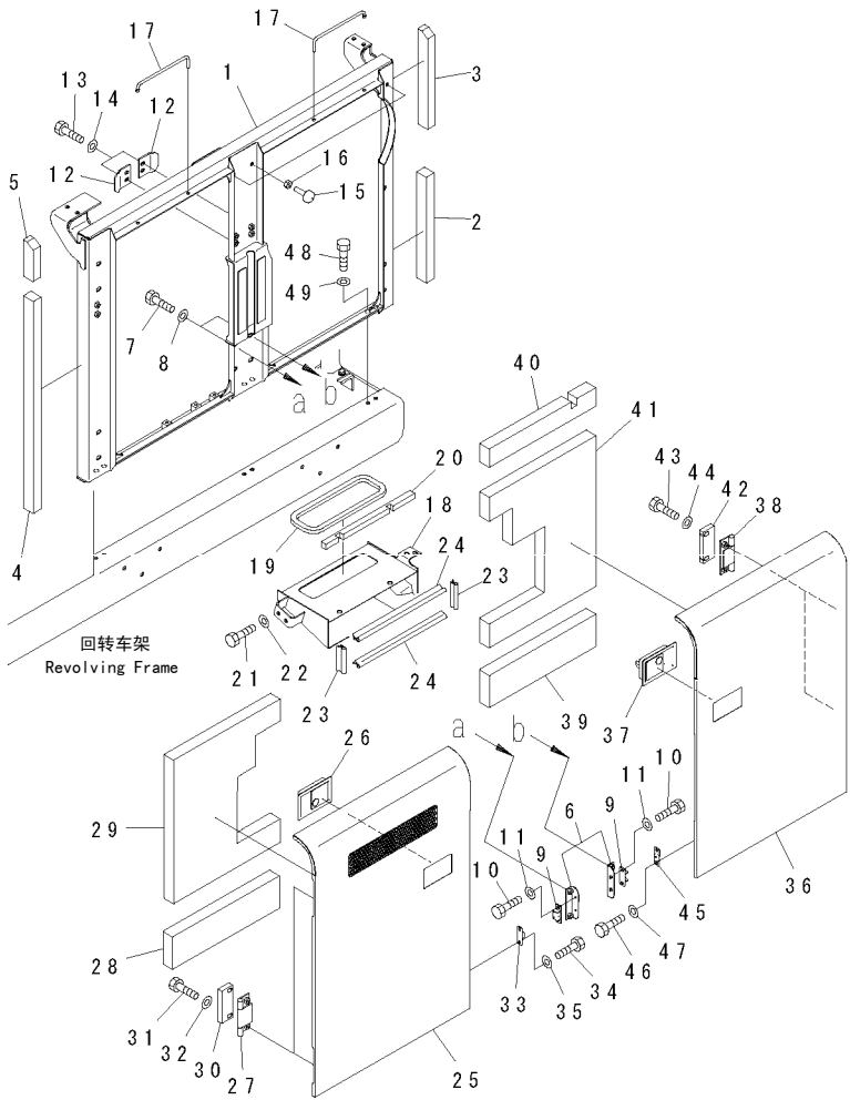
FIG.M1130-01A0 LEFT SIDE COVER (MACHINE CAB) 左盖(机罩)
