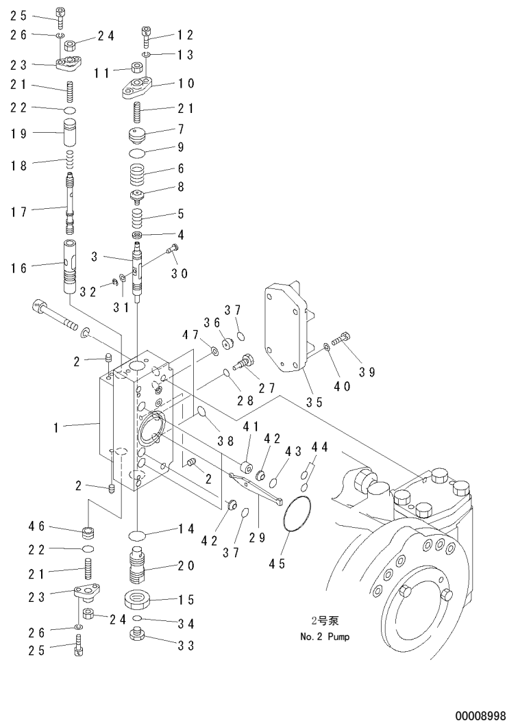
FIG. Y1600-28A0 MAIN PUMP (8/9) (NO. 2 PUMP) 主泵 (8/9) (2号泵)
