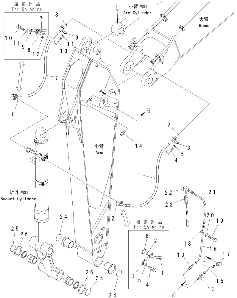
FIG. T1200-03A1 ARM (3.5M) (BUCKET CYLINDER HOSE AND SPACER) 小臂 (3.5M) (铲斗油缸软管和垫)
