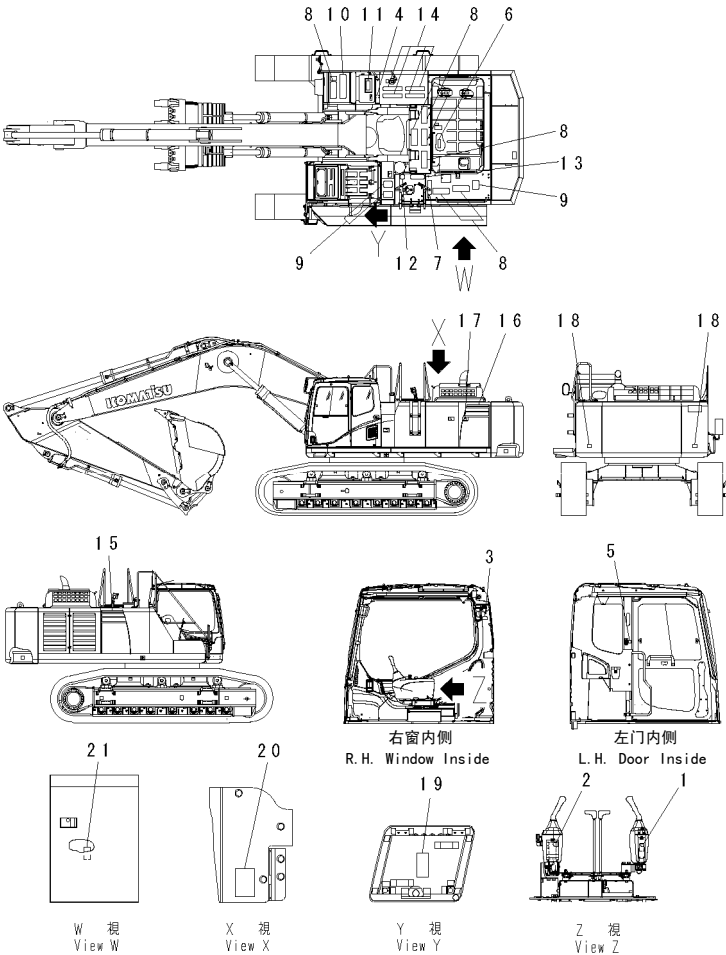
FIG.U0100-03A3 DECAL AND PLATE (SEAT AND SYMBOL MARK) (CHINESE) 警示标牌（座和符号标记）（中文）
