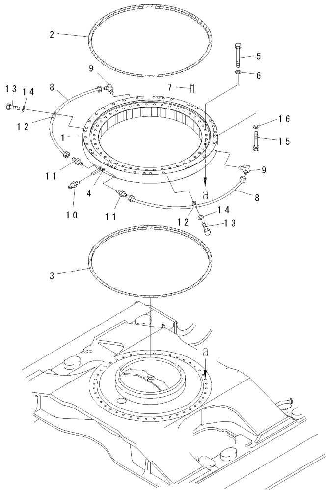
FIG.N1110-01A0 SWING CIRCLE 回转支承
