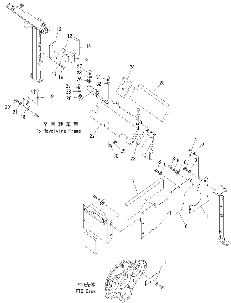
FIG.M1150-01A0 PARTITION (1/2) 隔离箱 (1/2)
