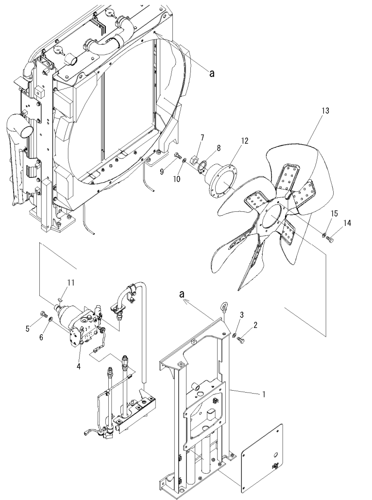
FIG. C0100-05A0 COOLING (FAN MOUNT) (FAN AND MOTOR) 冷却 (风扇安装) (风扇和马达)
