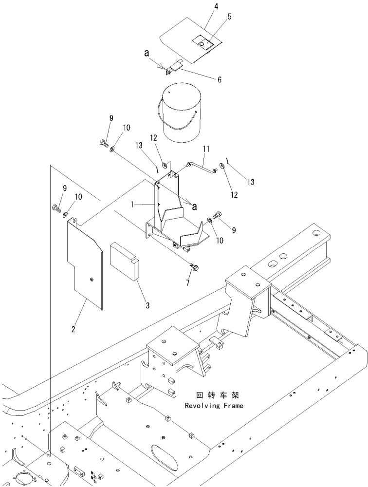
FIG.M1160-01A0 PARTITION (CAB REAR) 隔离箱(驾驶室后)
