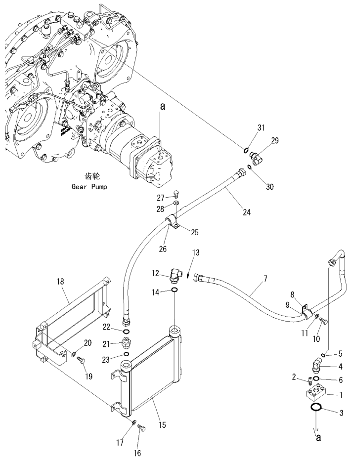
FIG. B0600-06A0 POWER TAKE OFF (P. T. O. PIPING) (DELIVERY LINES) 动力切断 (PTO管路) (输油管路)
