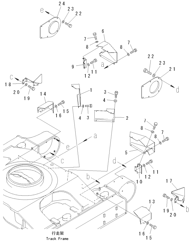
FIG.R1150-01A0 TRAVEL PIPING GUARD 行走管路护板
