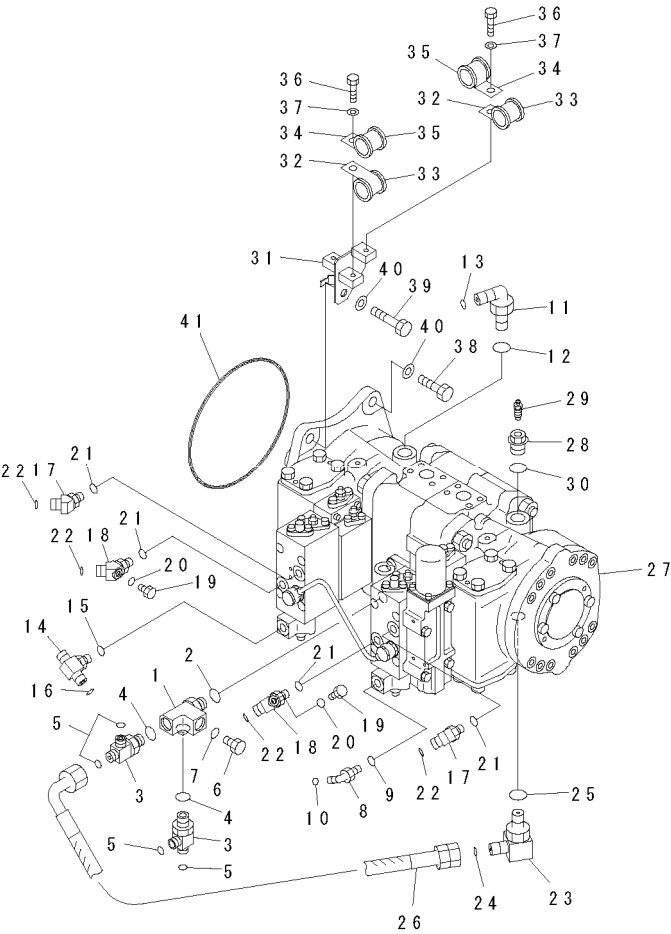
FIG. H0210-01A0 NO. 1 PUMP 1号泵
