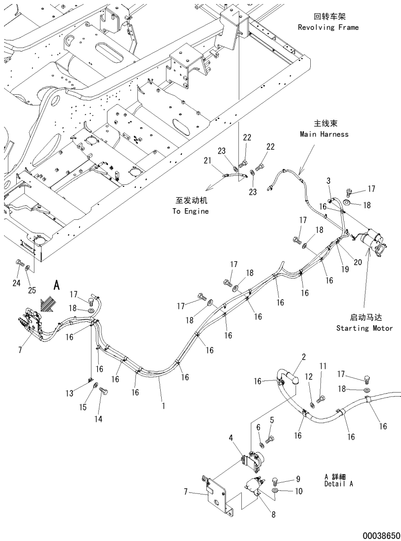
FIG. E0200-01A0 WIRING (STARTING HARNESS) 配线(启动线束)
