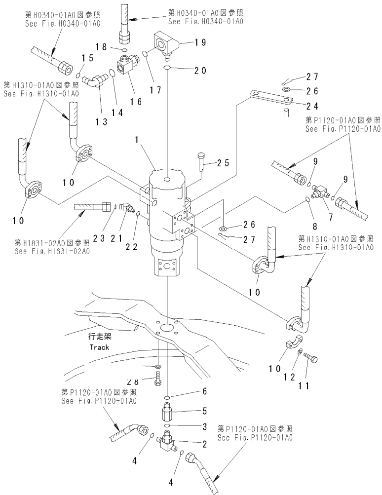
FIG. N1310-01A0 SWIVEL JOINT 回转接头
