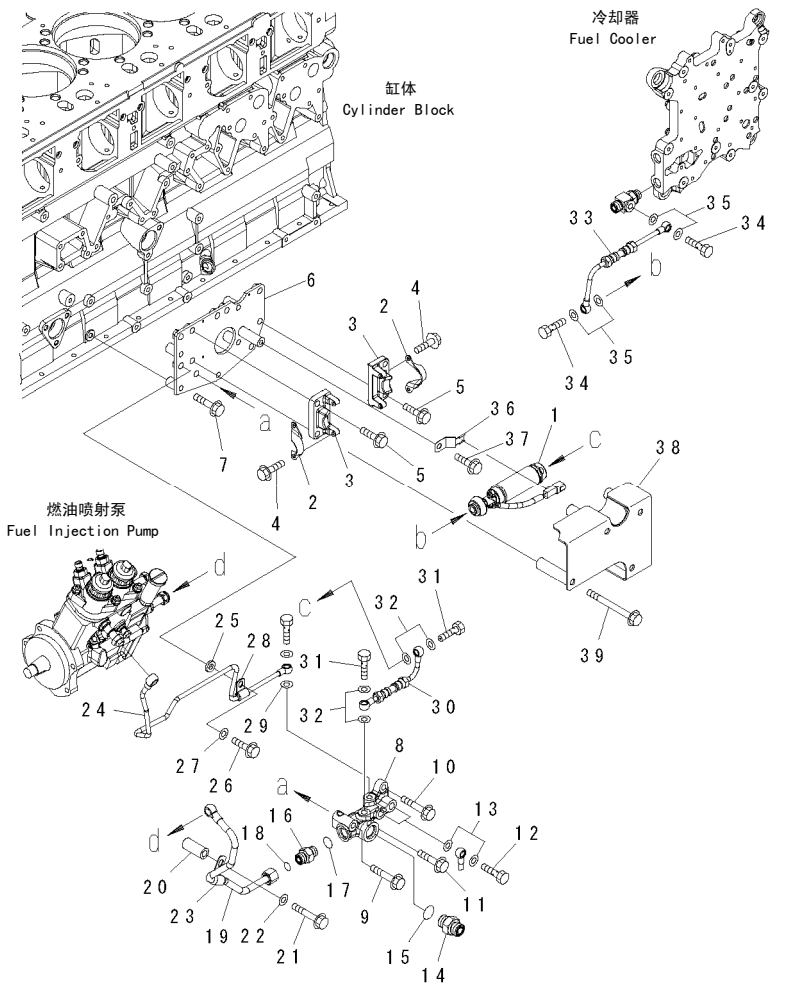
FIG. A4110-B4N2 FUEL PRIMING PUMP 燃油引液泵
