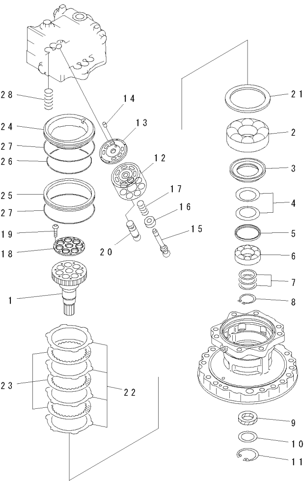
FIG. Y1640-02A0 SWING MOTOR (2/3) 回转马达 (2/3)
