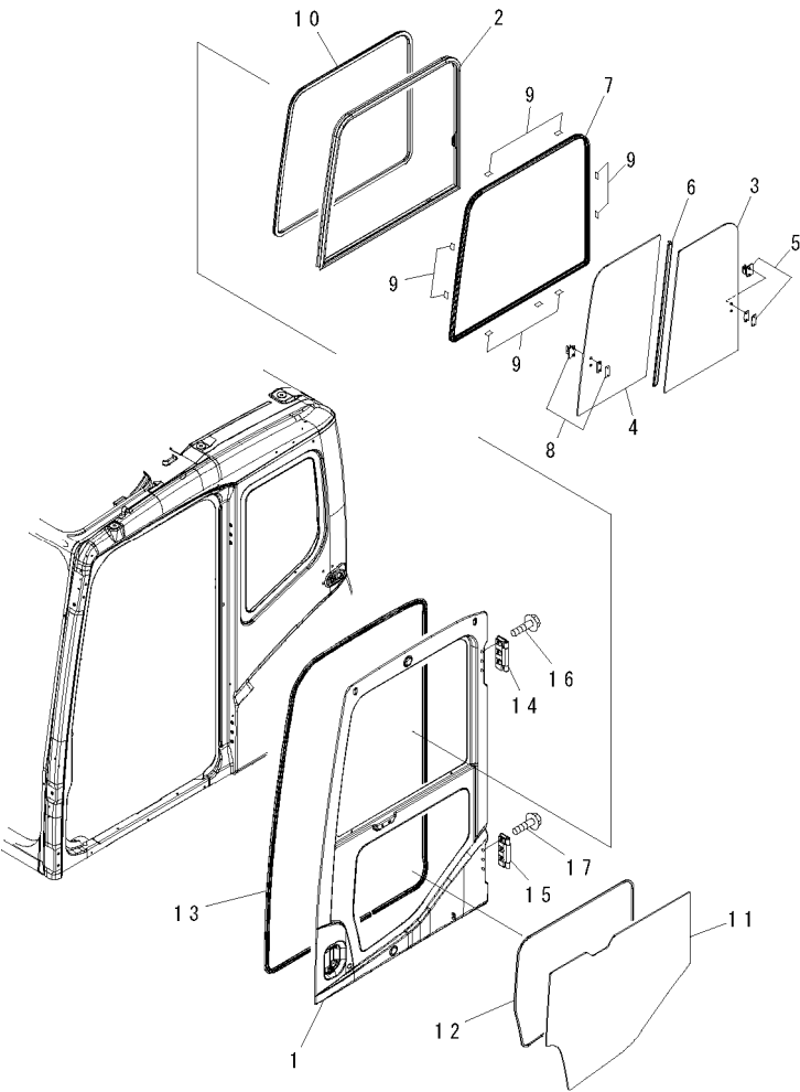
FIG.K1110-05A0 FLOOR FRAME (OPERATOR'S CAB) (DOOR) 底板架（驾驶室）（门）
