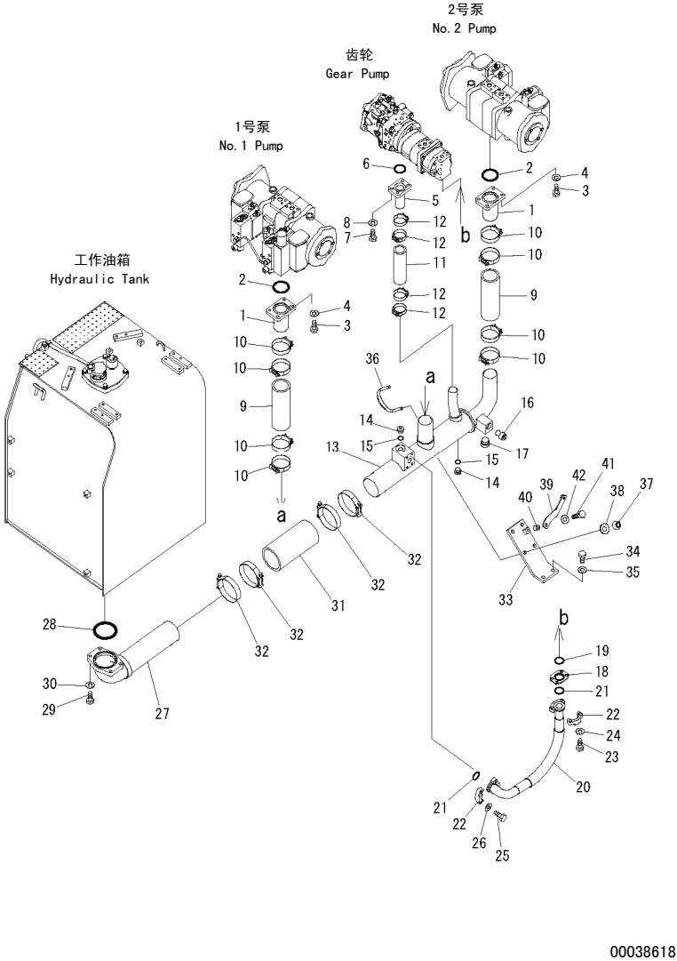
FIG. H0311-01A0 SUCTION LINES 吸油管路
