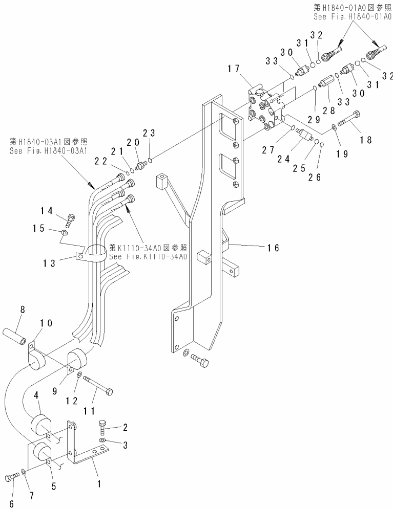
FIG. H1833-01A0 SHUTTLE VALVE (BRACKET AND VALVE) 梭阀 (支架和阀)
