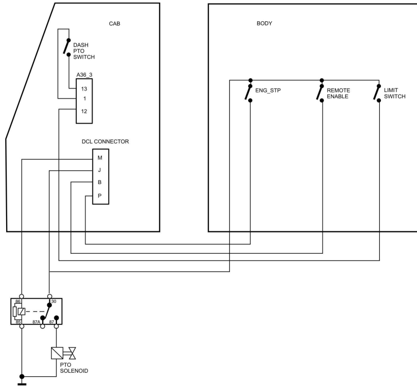
Fig. 33 Example TE / MRU showing Body Builder supplied wiring for Controls
