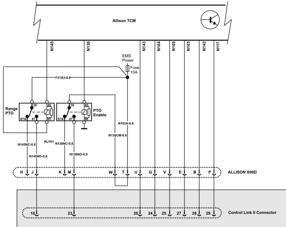
Fig. 24 Allison Connections — TE / MRU, LR Control Link II
