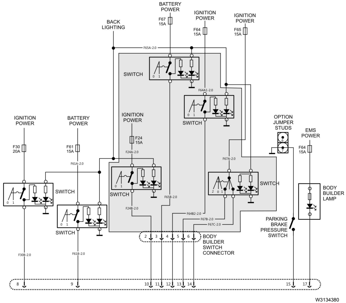
Fig. 15 Conventional Auxiliary Switches
