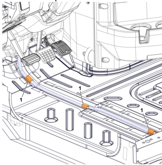
Fig. 9 Granite BodyLink III Routing Beneath Driver Seat
