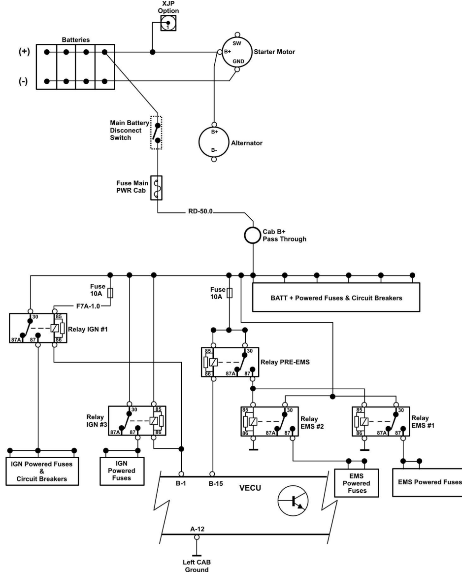
Fig. 2 Battery & Ignition - Switched Supplies - Conventional Trucks
