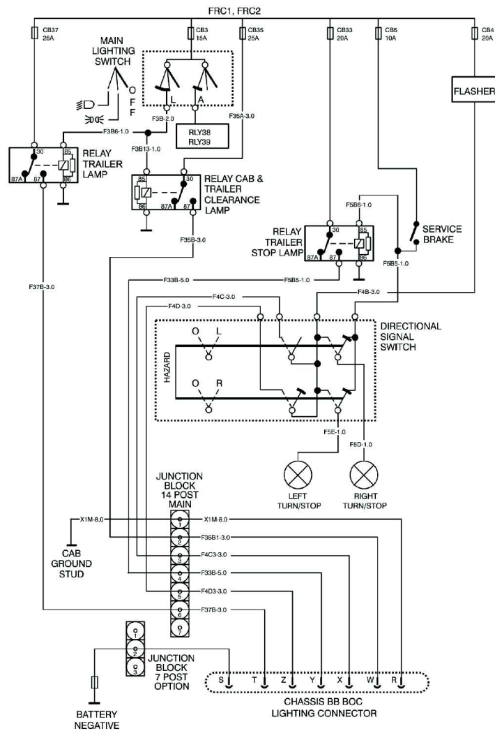
Fig. 27 TE / MRU / LR Lighting Connections
