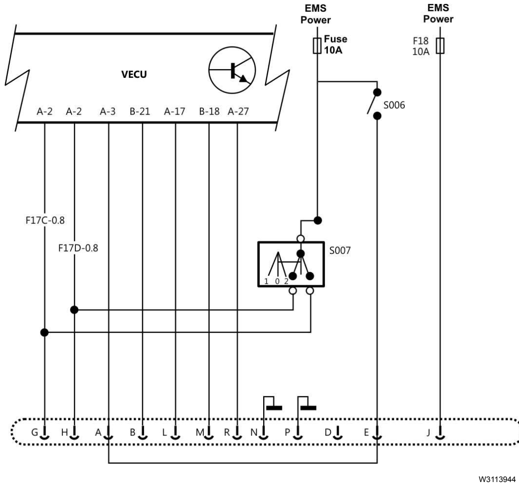
Fig. 25 PTO & Engine Speed Control Connections
