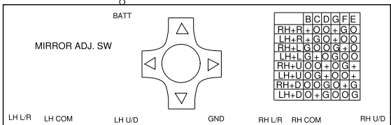
S030 SWITCH, MIRROR CONTROL
