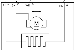
M110LHM MIRROR, LH, HEATED, MOTORIZED
