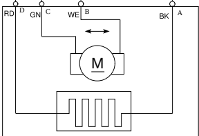
M110RHM MIRROR, RH, HEATED, MOTORIZED
