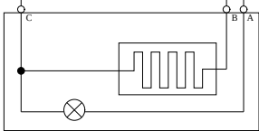
M110RHL_MATE MIRROR, RH, HEATED, LIGHTED
