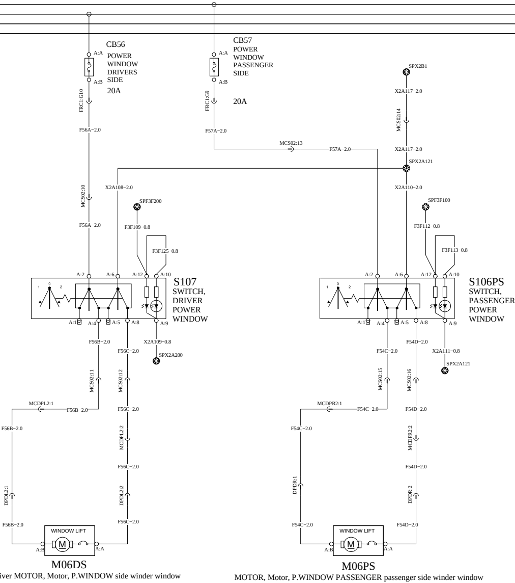
DRIVER driver MOTOR, Motor, P.WINDOW side winder window
