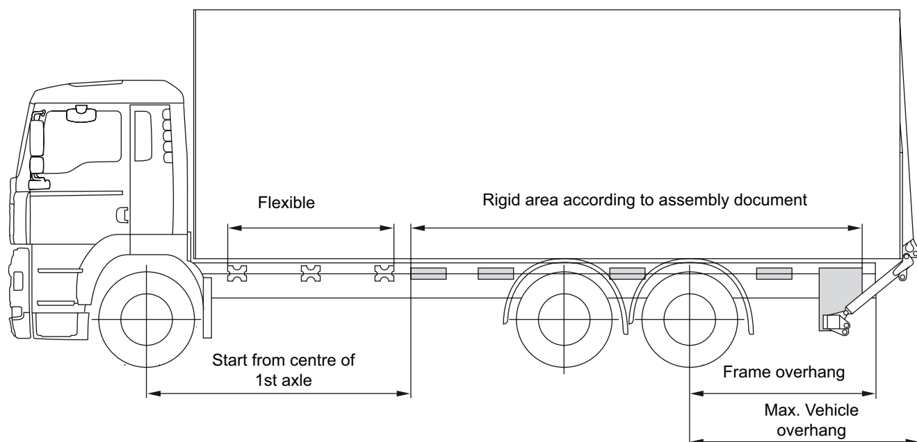
Fig. 93: Tail-lift overhang dimension, dimensions with partially rigid connection ESC-633
