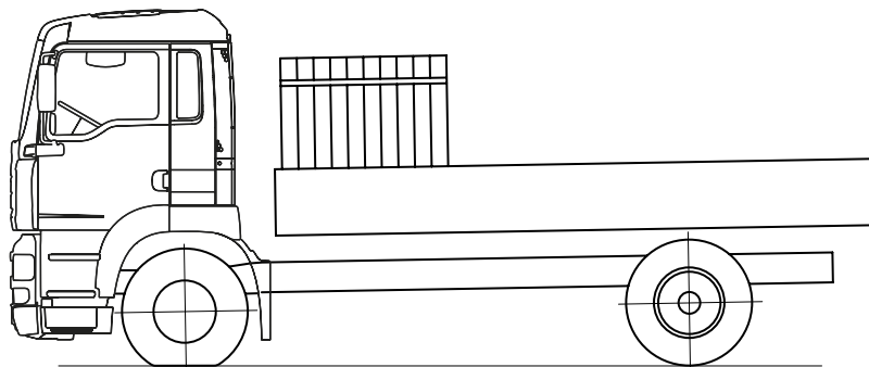
Fig. 1: Overloading the front axle ESC-052
