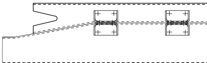
Fig. 54: Subframe – adapting it by expanding it ESC-098
