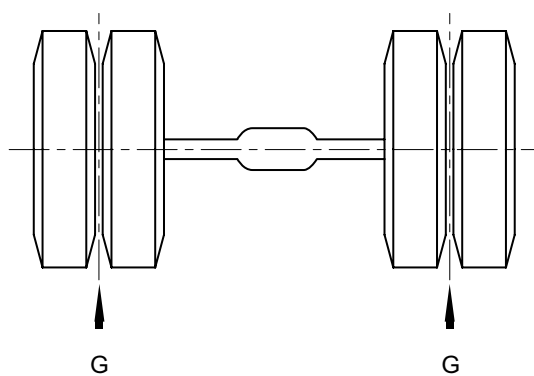
Fig. 3: Difference in wheel load ESC-126
