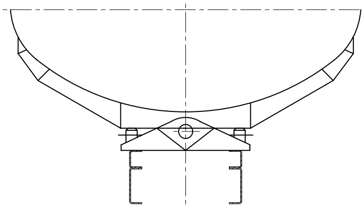
Fig. 73: Front mounting as a pendulum mounting ESC-103
