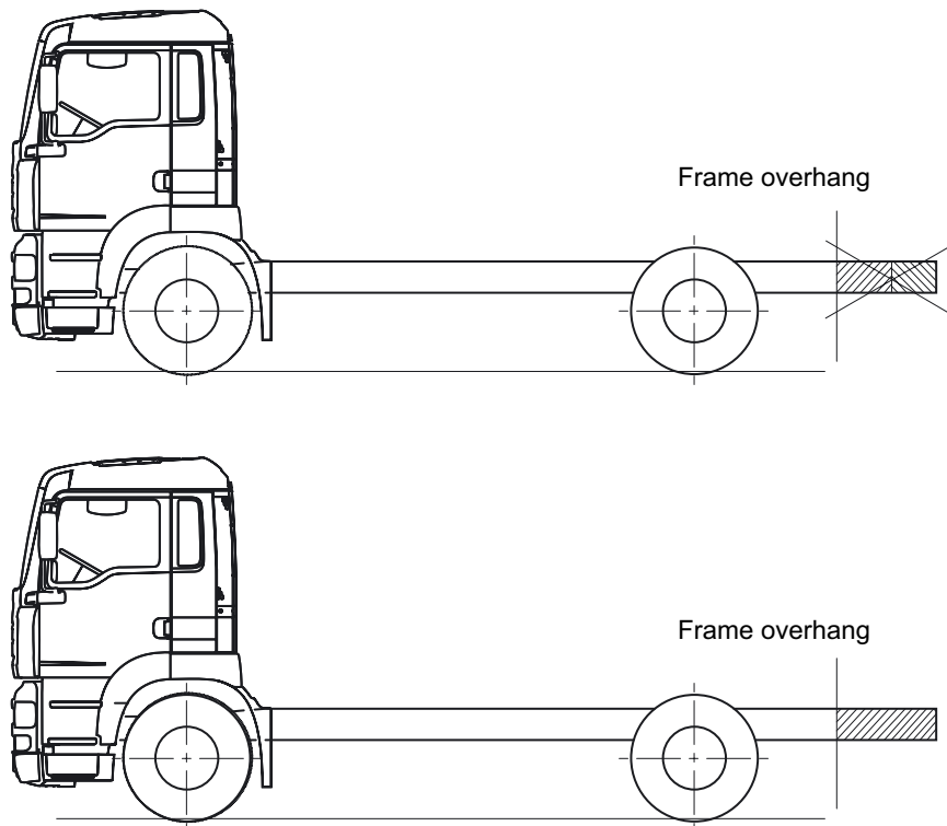
Fig. 22: Extending the frame overhang ESC-093
