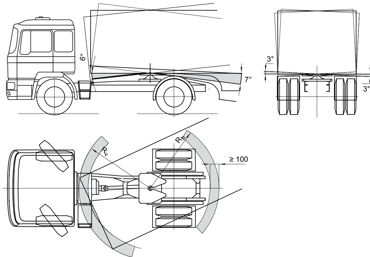
Fig. 47: Dimensions for semitrailer tractor units ESC-002
