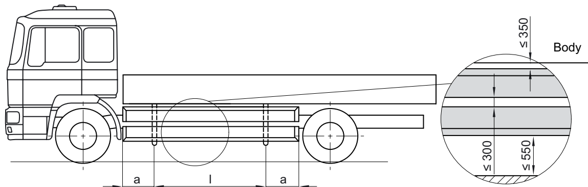
Fig. 39: Sideguards on M2000 and F2000 vehicles ESC 200
