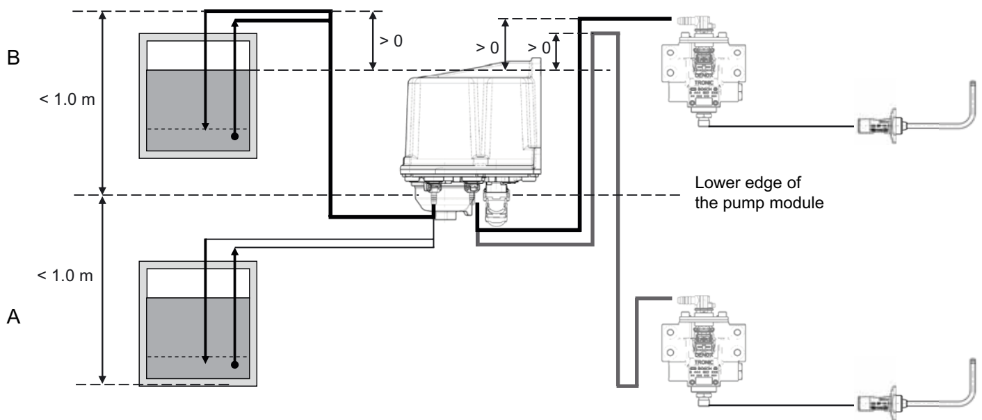
Fig. 48: Installation overview ESC-422
