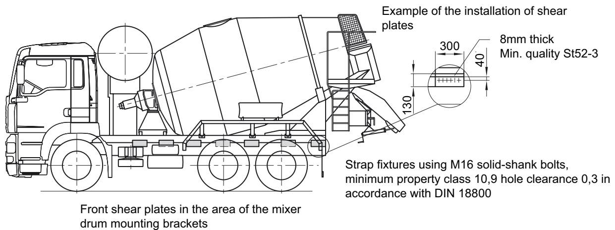
Fig. 95: Transport mixer body ESC-016
