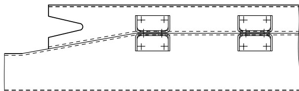
Fig. 62: Subframe - adapting by widening ESC-098
