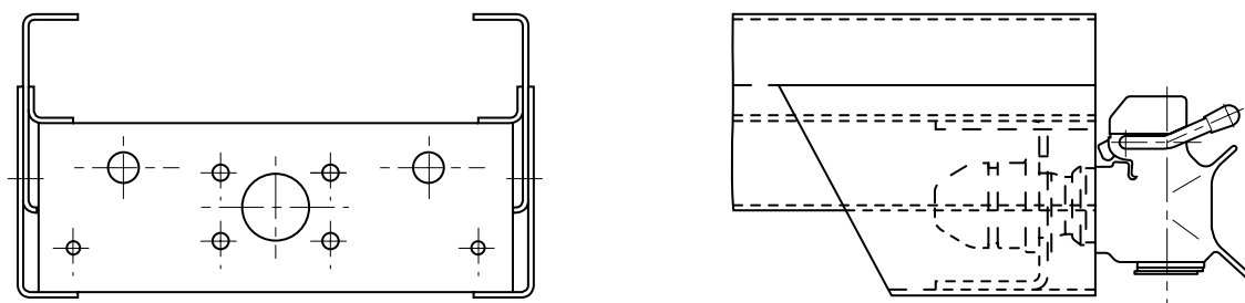
Fig. 35: Lowered trailer coupling ex.ESC-015 ESC-515
