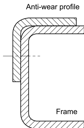
Fig. 78: Anti-wear profile for interchangeable container ESC-121
