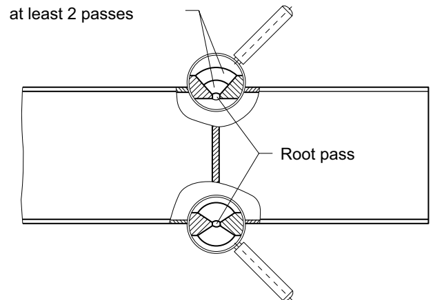
Fig. 15: Welding at X and Y seam ESC-003
