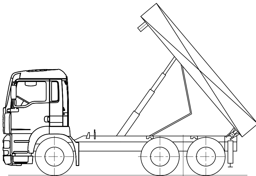
Fig. 86: Rear tipper with scissors-action support and rear support ESC-106
