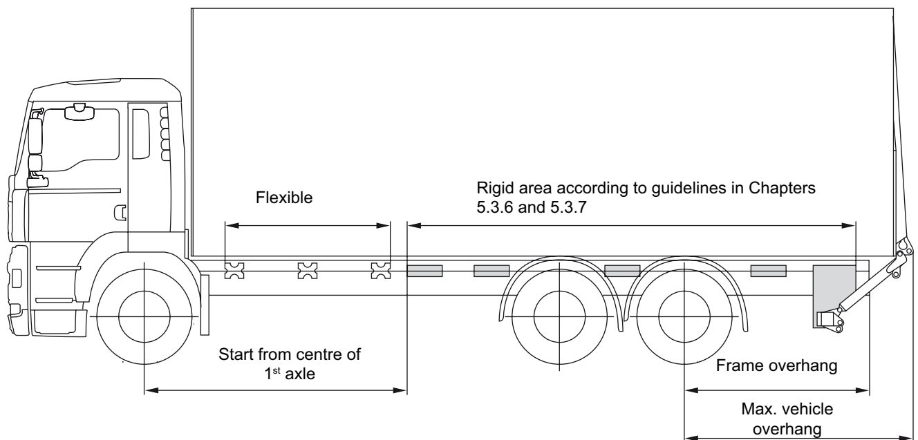
Fig. 71: Tail-lift installation: overhang dimension, dimensions with partially rigid connection ESC-633
