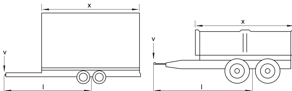
Fig. 105: Length of the trailer body and theoretical drawbar length (see also booklet „Coupling devices“) ESC-510
