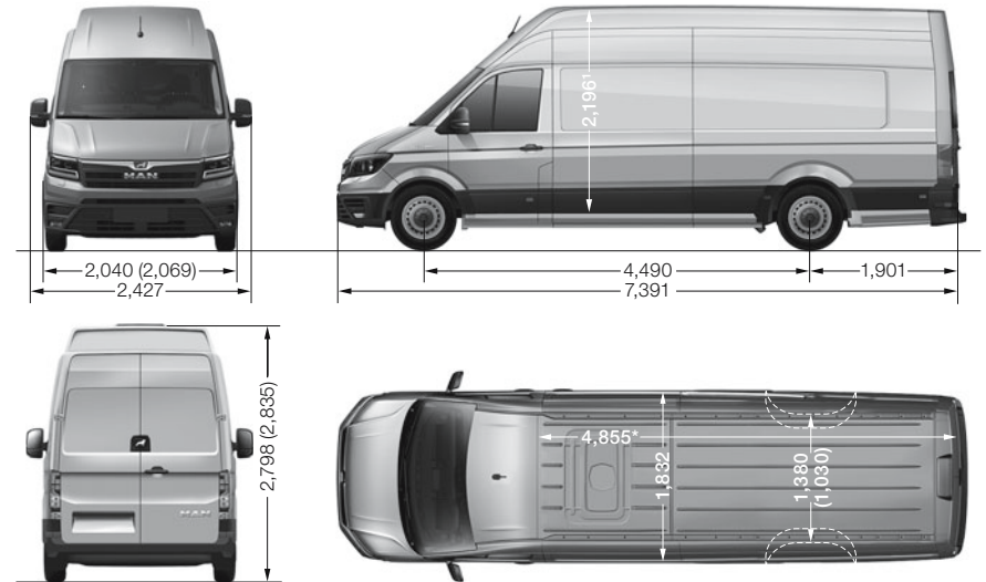
MAN TGE Panel van Extra-long with Super-high roof
