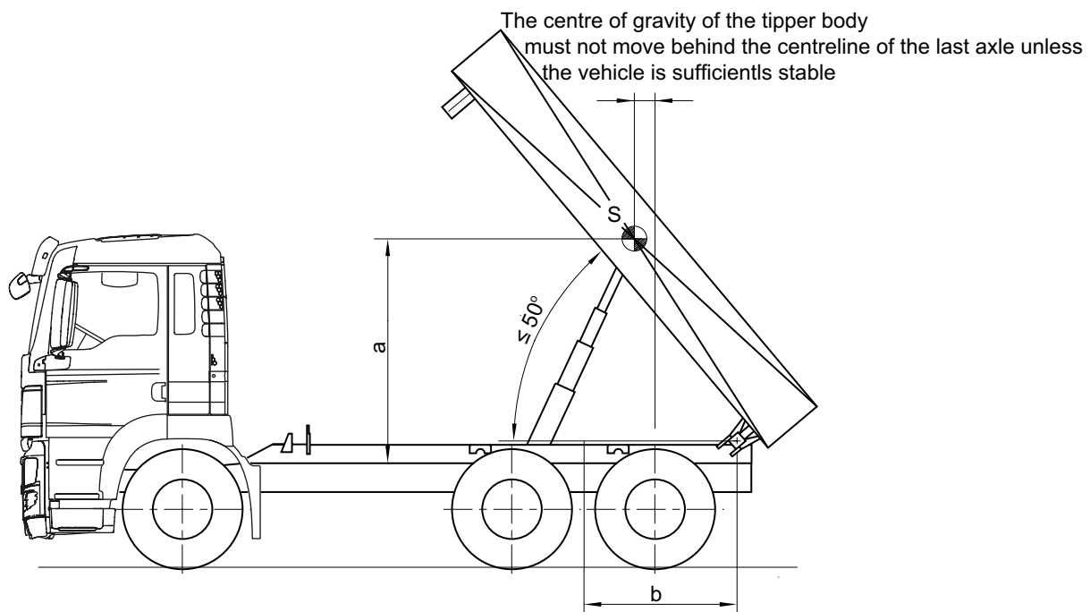
Fig. 100: Tippers: Maximum values for centre of gravity height and tipper mounting spacing ESC-405
