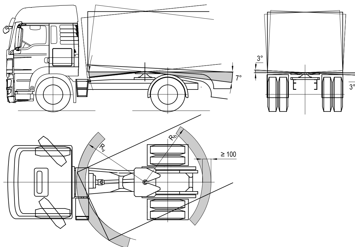
Fig. 37: Dimensions for semitrailer tractor units ESC-402
