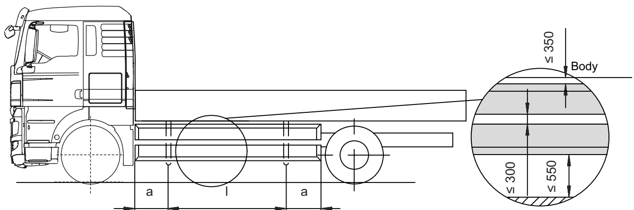
Fig. 43: TGA sideguards ESC-460
