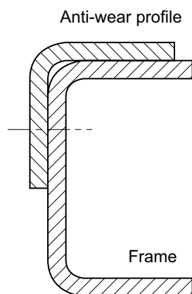
Fig. 93: Anti-wear profile for interchangeable container ESC-121
