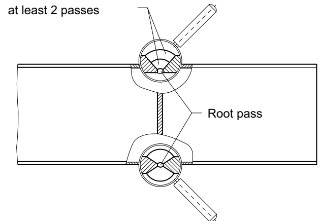
Fig. 16: Welding at X and Y seam ESC-003
