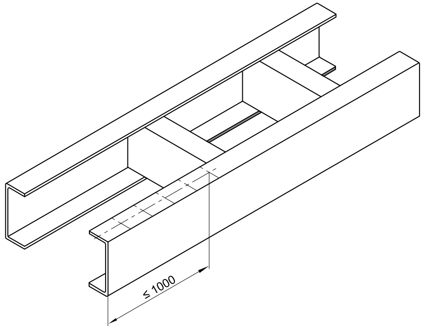
Fig. 11: Drill holes at frame end ESC-032
