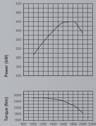
600 hp
