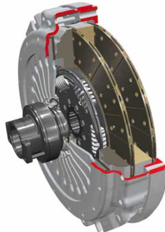
Double-plate clutch
