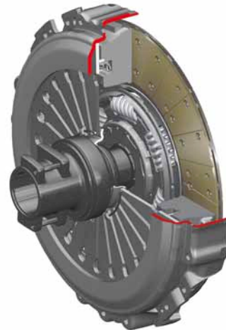
Single-plate clutch
