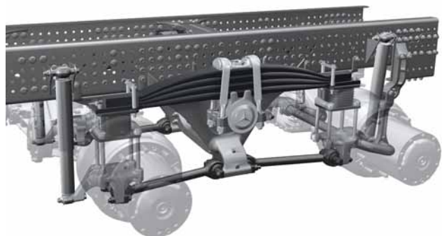
Steel suspension with 2 driven rear axles
