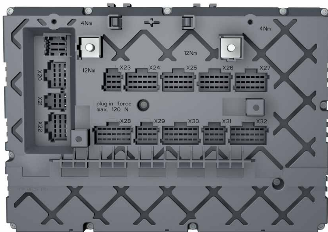
Single SAM, rear view
