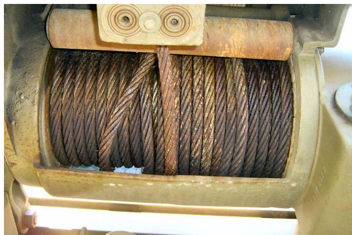
Figure 9-21: Unimog's Winch Assembly Underside
