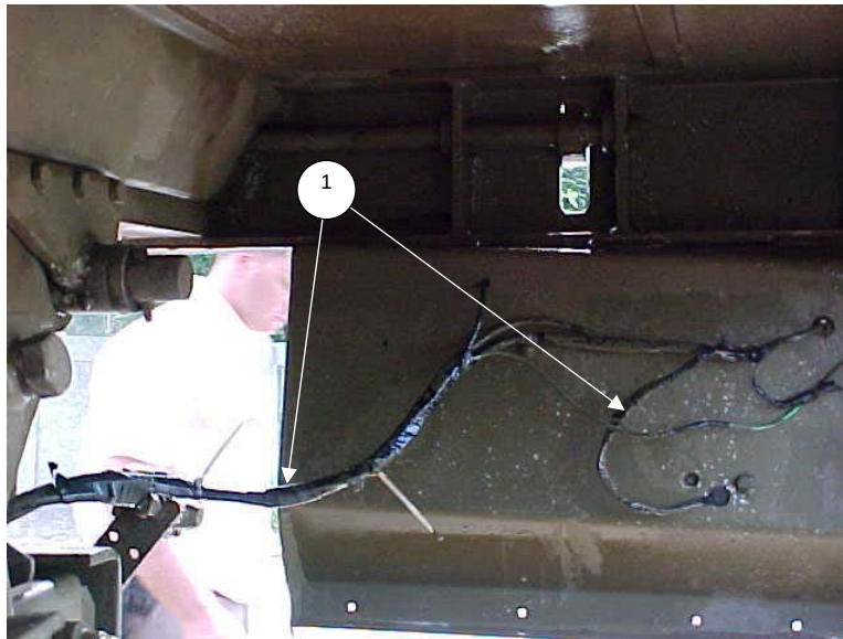
Figure 9A-3: Unimog Dump's Rear Electrical Cables
