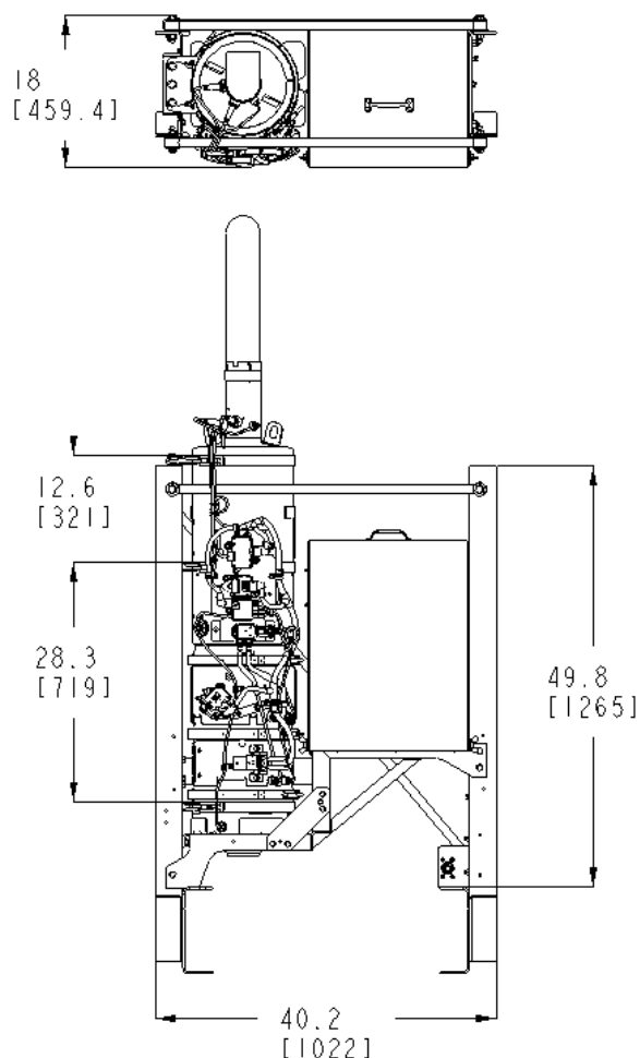
Figure 3-10.2 Model 220 Vertical Exhaust Measurement inches (mm)
