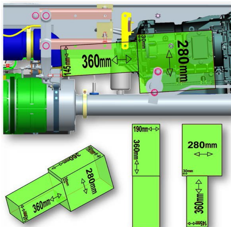
Figure 3-12.3 Model 220 PTO Clearances 2 of 2
