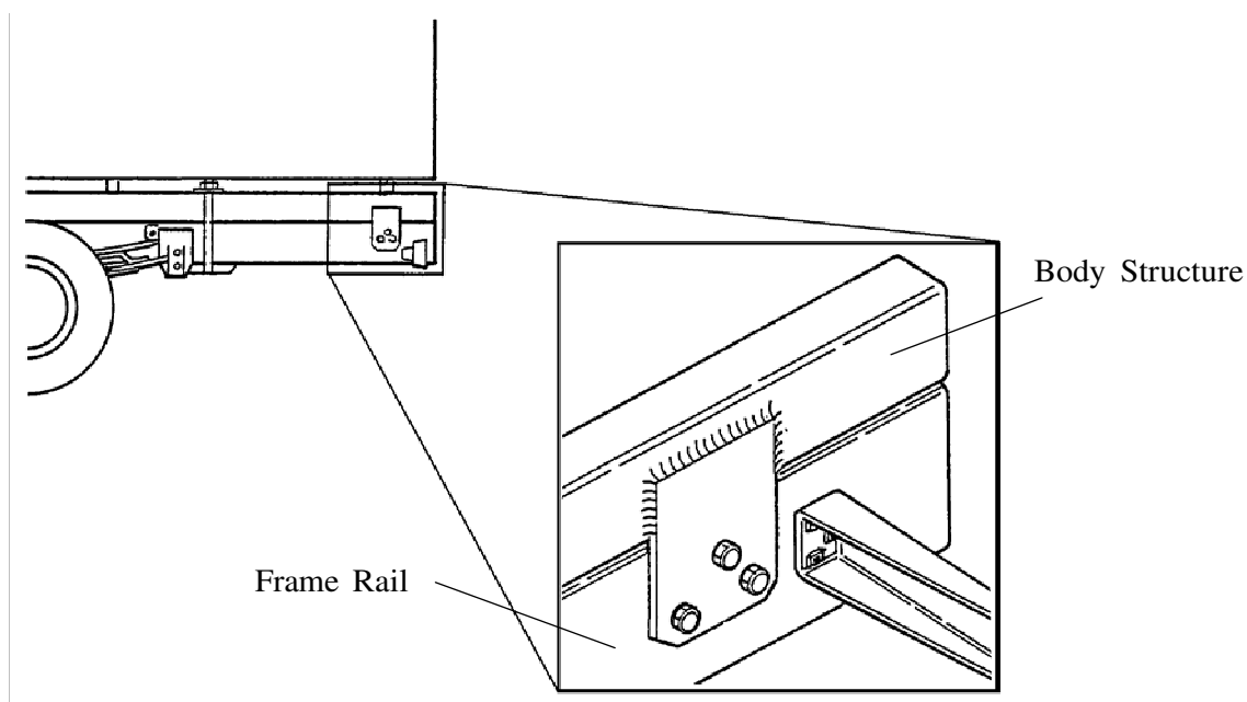
Figure 5-11 Example of Fishplate Bracket at Rear End of Body, used with U-Bolts
