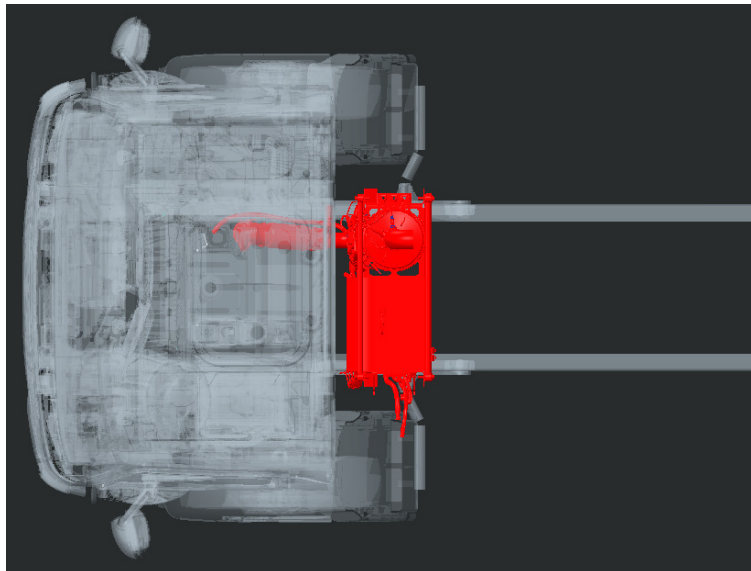
Figure 4-7.2 Top view of Vertical Exhaust Canister with Vertical Tailpipe
