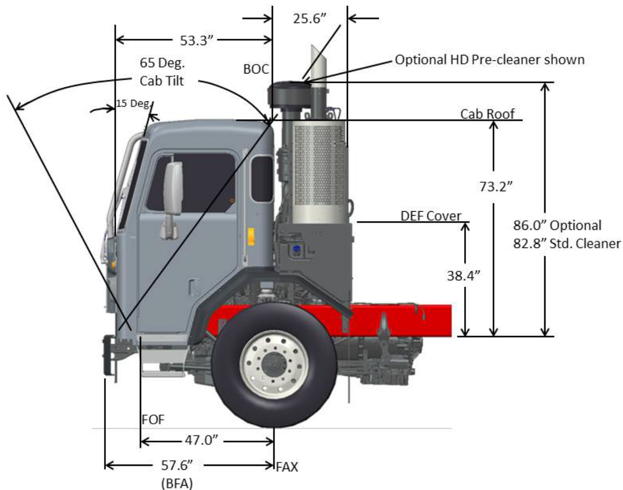
FIGURE 3-2. 520 Cab Dimensions
