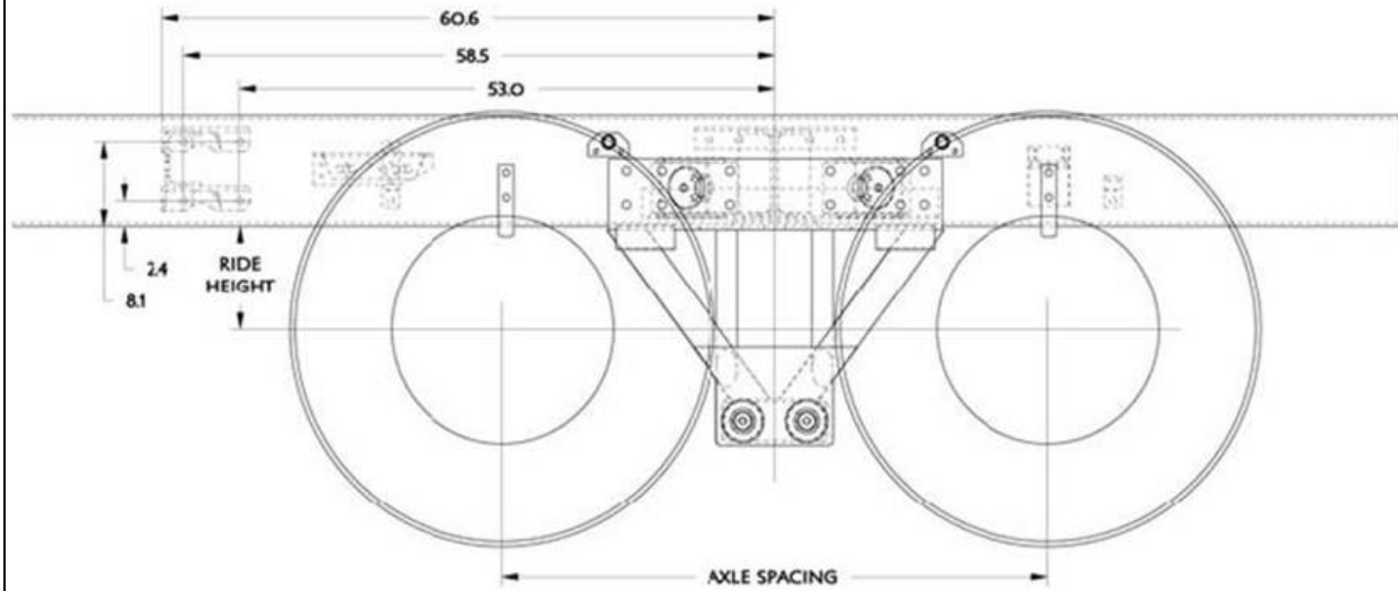
FIGURE 3-14. Chalmers 854 Tandem Frame Drilling
