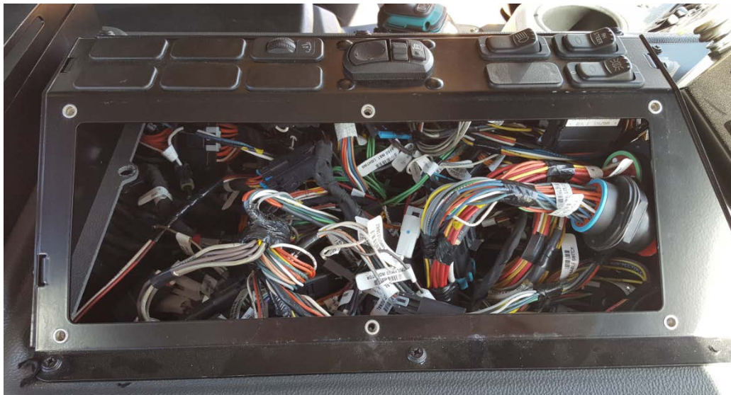
FIGURE 6-5. Body Builder Connections in Cab
