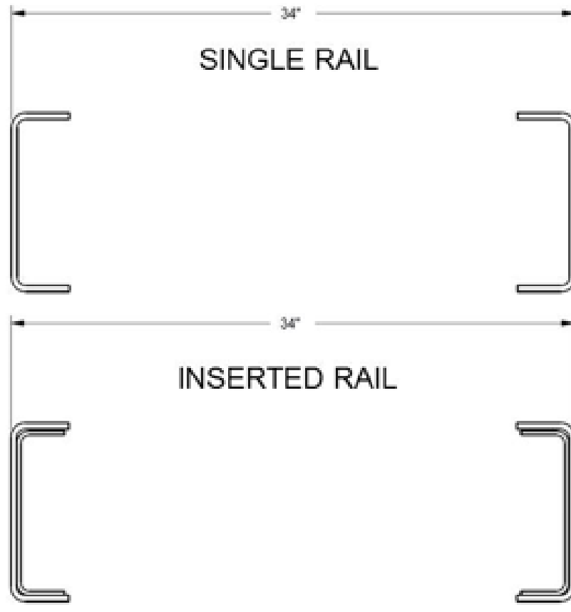
FIGURE 3-12. Frame Rail Configurations
