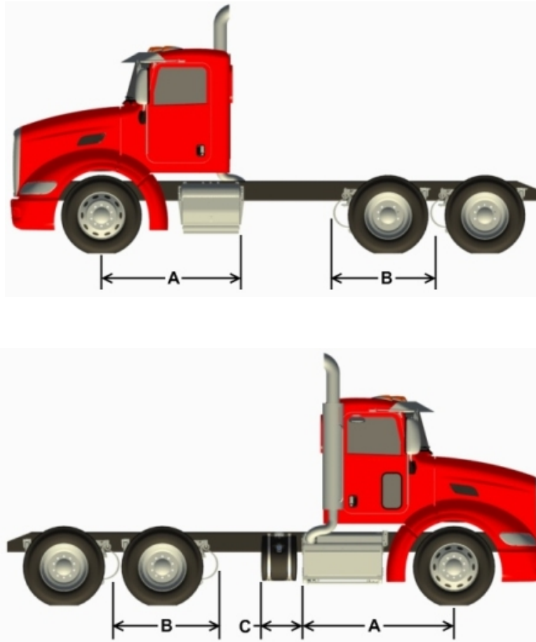
FIGURE 3-14. Frame Space
