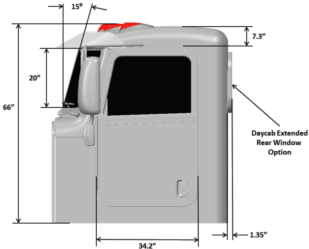
FIGURE 3-5. Cab Dimensions 1.9m Medium Duty Cab Family
