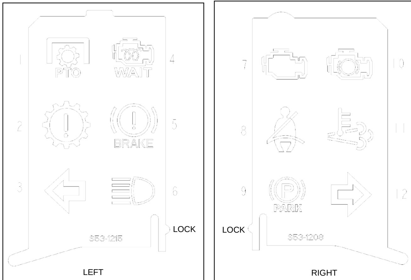
FIGURE 6-12. Telltale Symbol Standard Card
