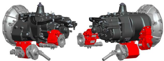
FIGURE 7-4. HD Manual Transmission – RT Vocational
