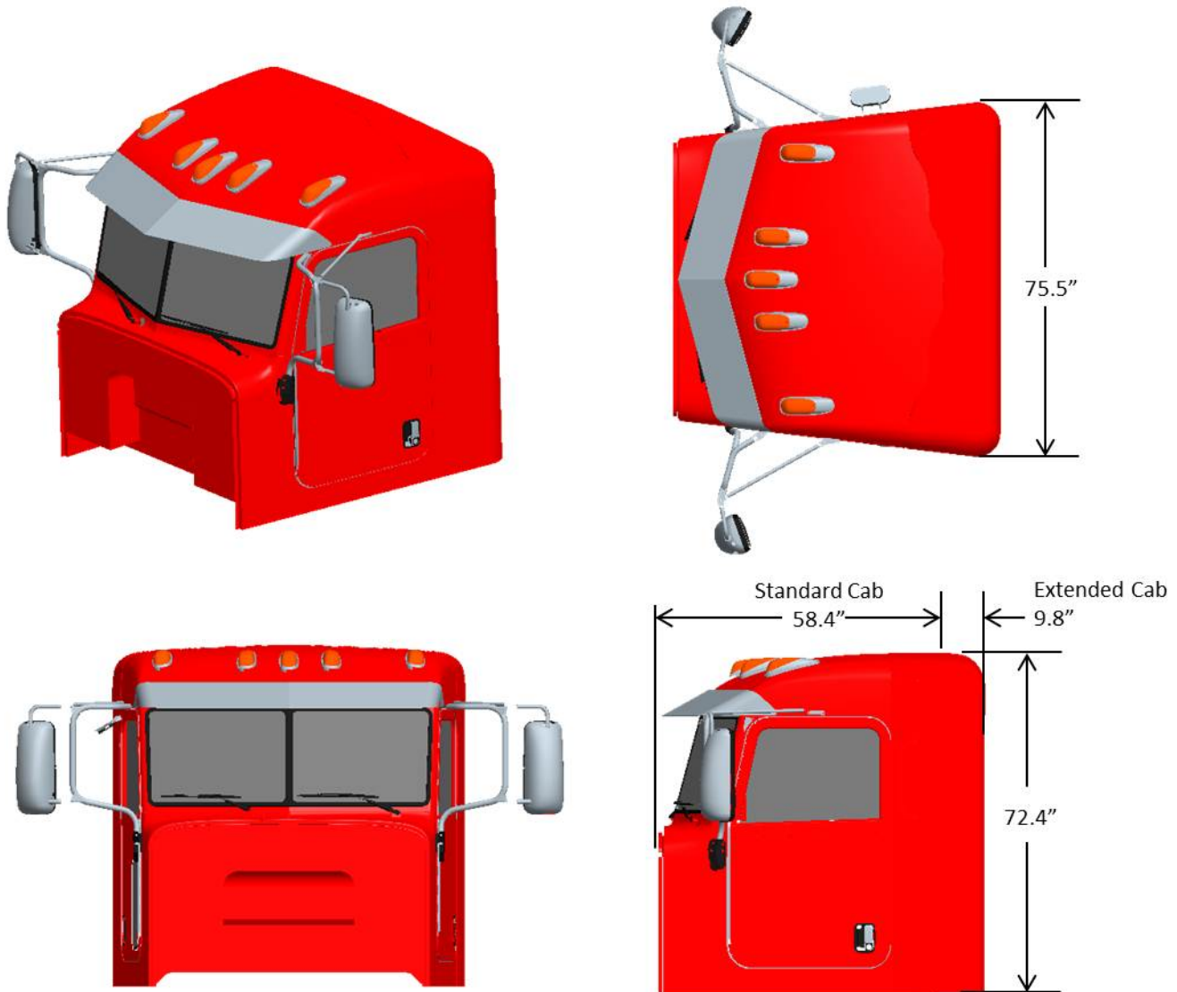
FIGURE 3-11. Extended Cab
