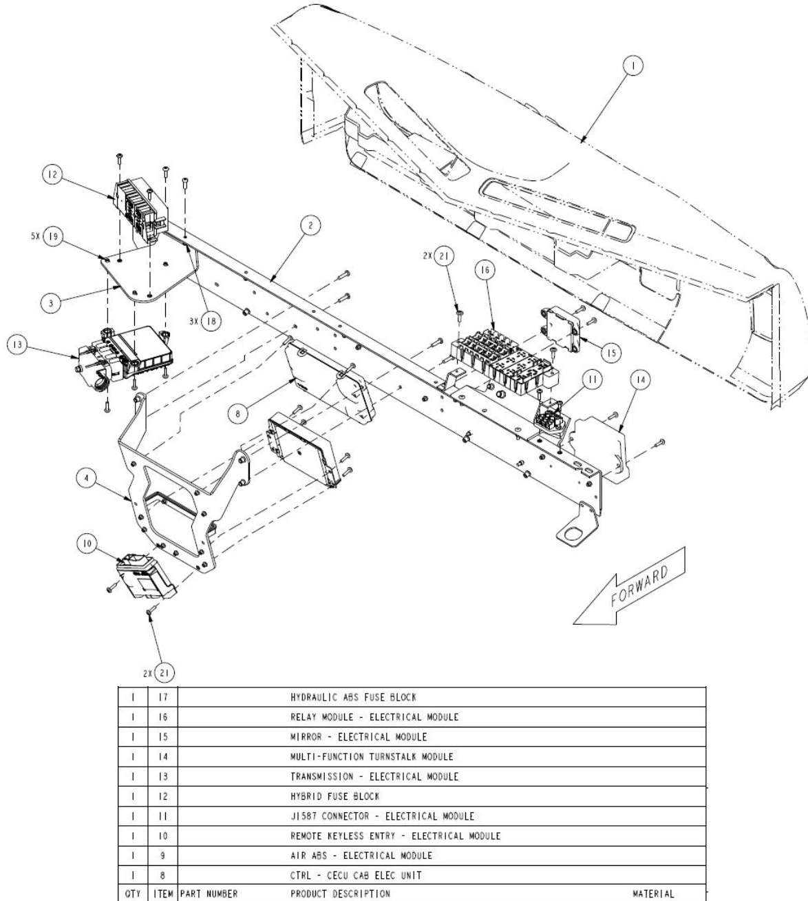
FIGURE 6-5. CECU Location and Other Electrical Modules
