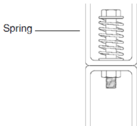
FIGURE 4-4. Mounting Brackets
