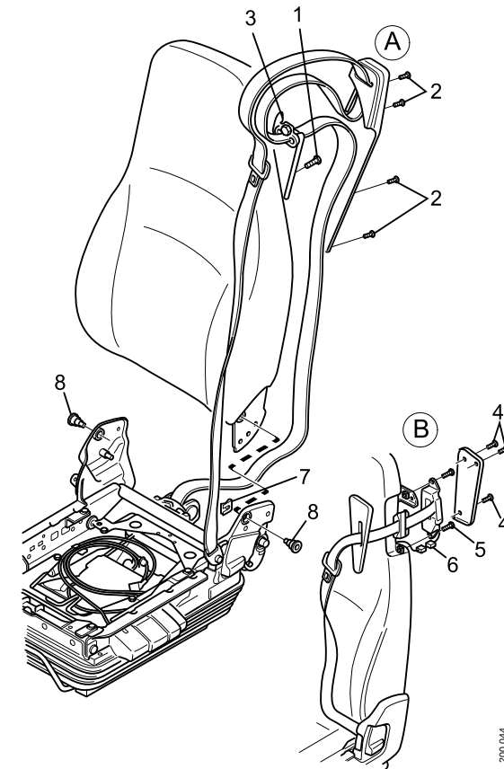
Basic and Medium seats (A), Luxury seat (B)
