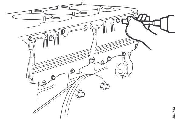
Camshaft covers
