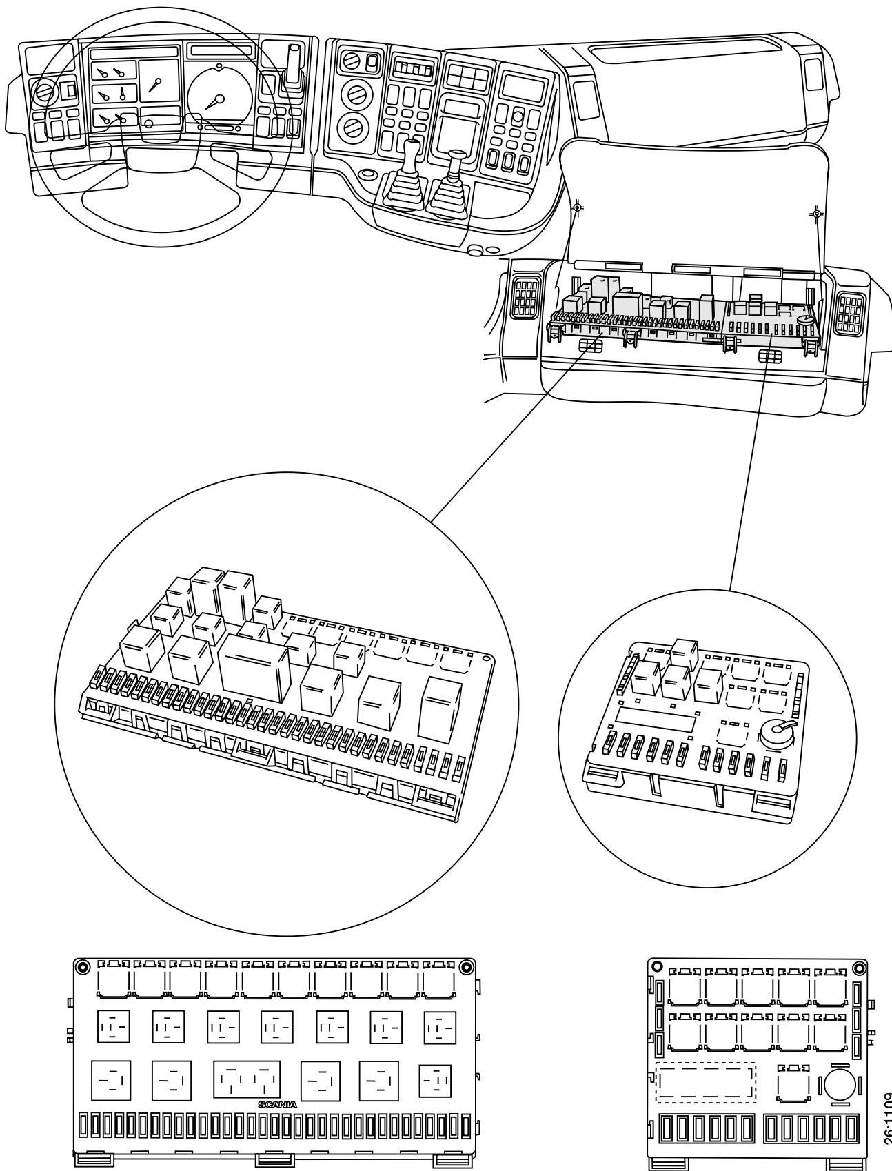
Central electric unit
