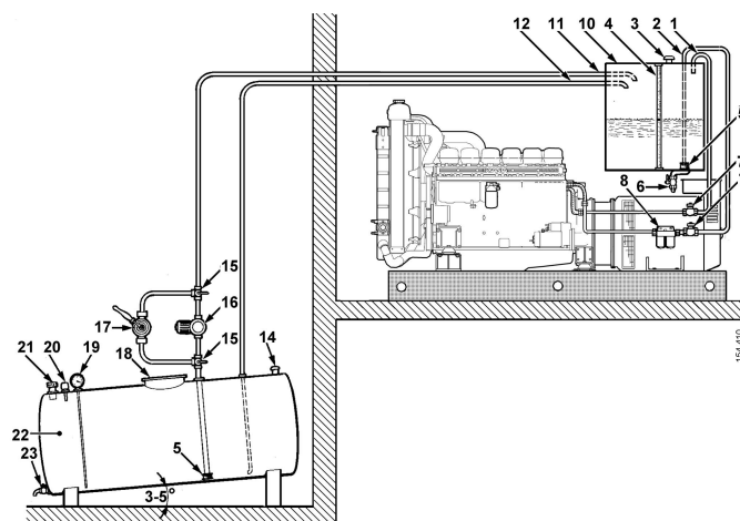
Example of a fuel system for a stationary industrial engine
