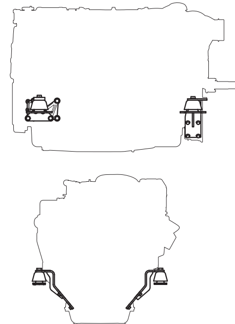
Examples of flexible engine suspension
