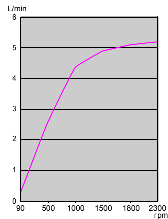
Feed pump flows for DI16 XPI.
