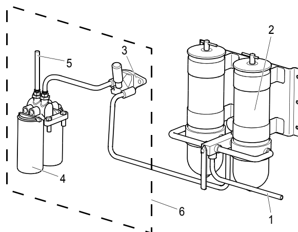
Fuel filter installation on PDE engines.
