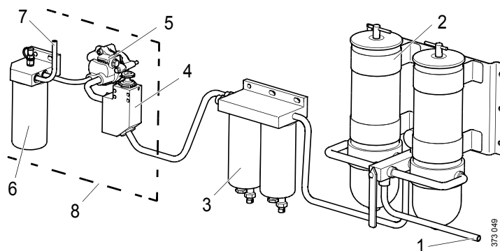
Fuel filter installation on XPI engines.
