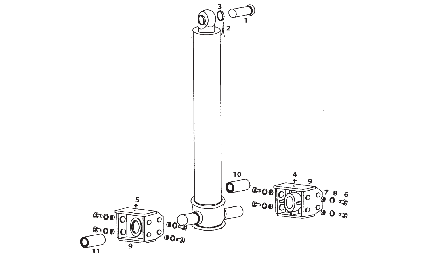
CYLINDER MOUNTING (FE CYLINDER)
