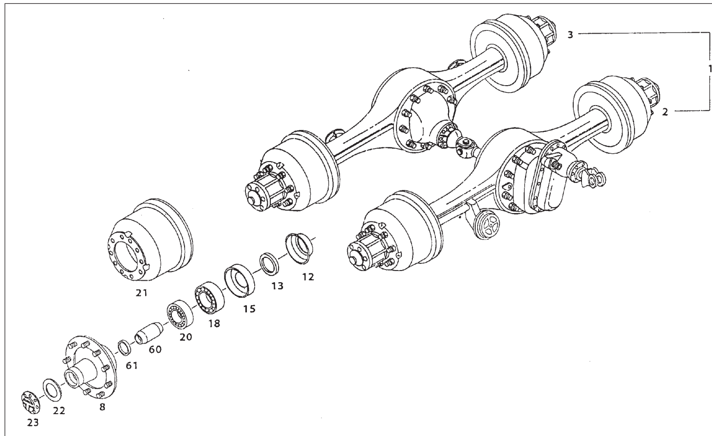
REAR AXLE (TANDEM BOGIE AXLE)
