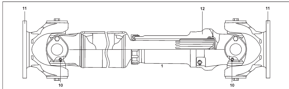
PROPELLER SHAFT FRONT (SPICER)
