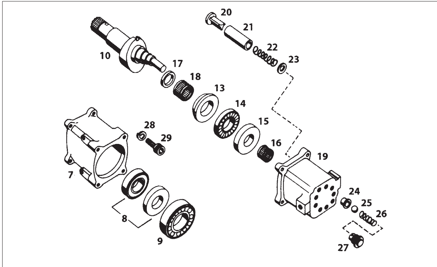
AXIAL PISTON PUMP MK III (G-600 GEAR BOX)
