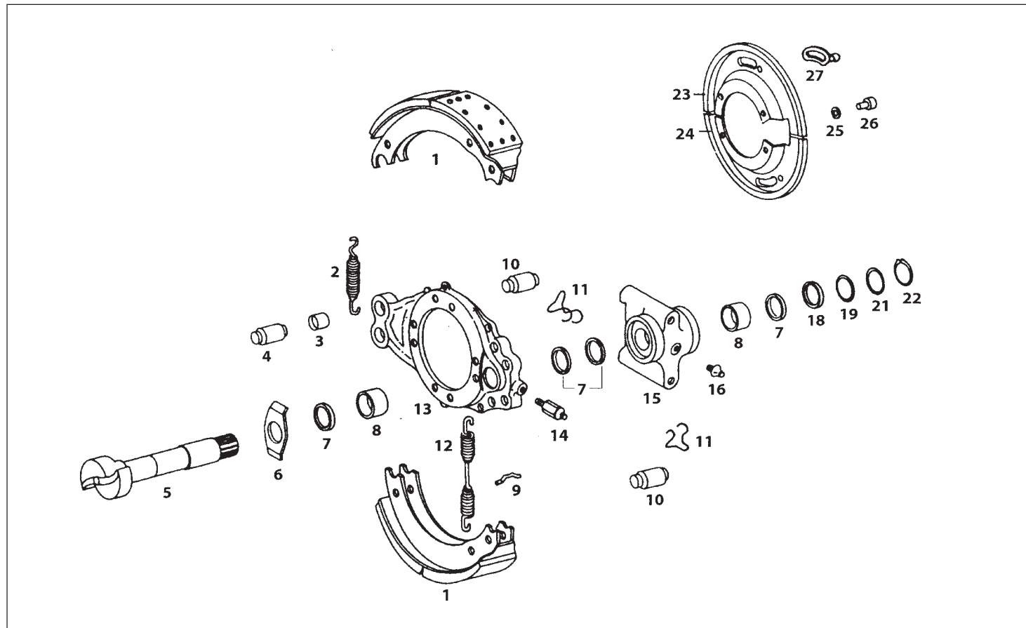
REAR WHEEL BRAKE (M/S AAL)
