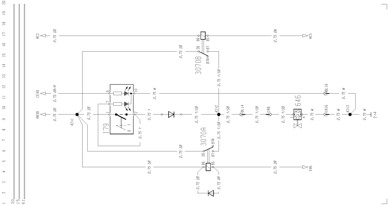
TAG AXLE LOCK, RADT-R6S
