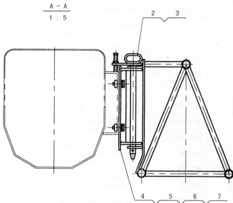
QY25K5.14 副起重臂 Jib
