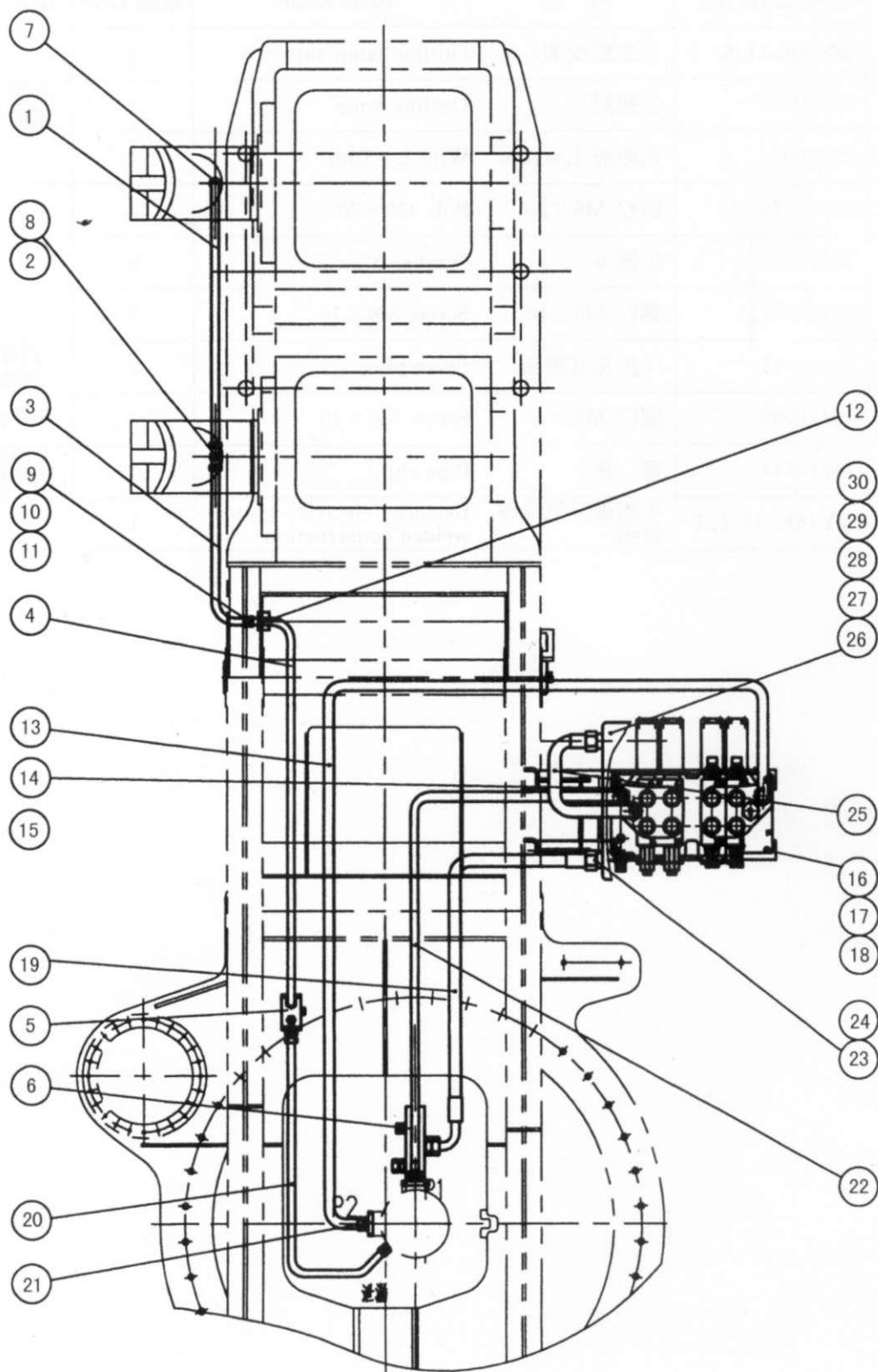
QY25K5. 13.1 进回油泄漏配管 The Input Oil、Oil Returns's Piping Plan
