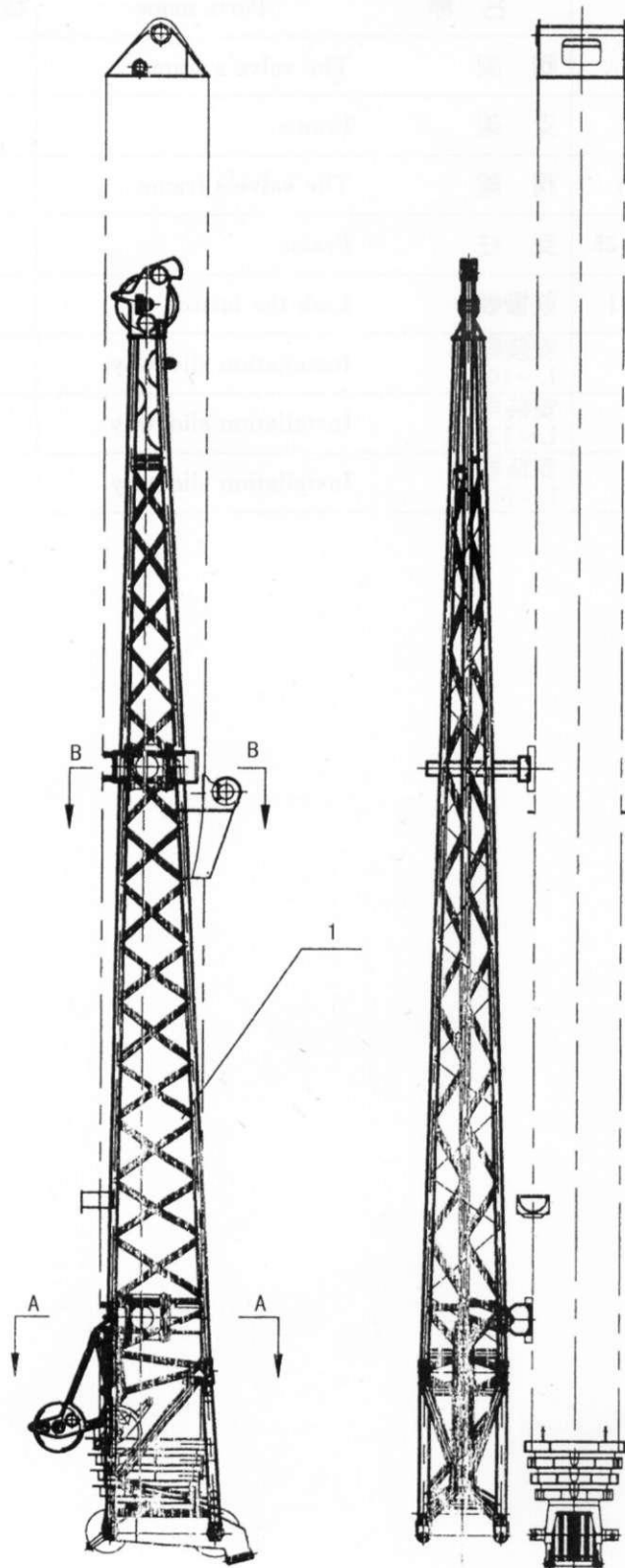
QY25K5.14 副起重臂 Jib
