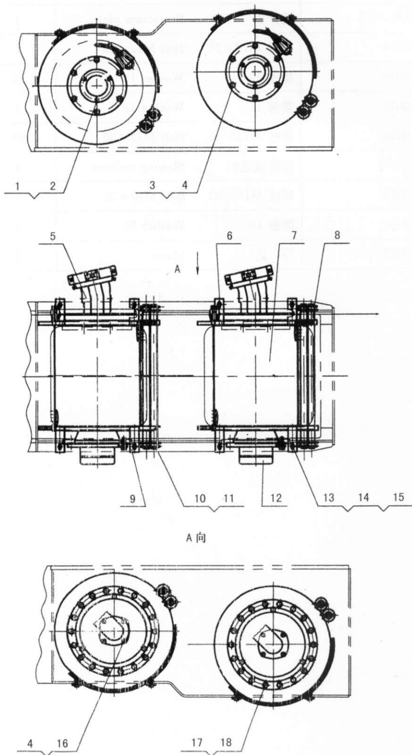
QY25K5.08 起升机构 Lifting Movement
