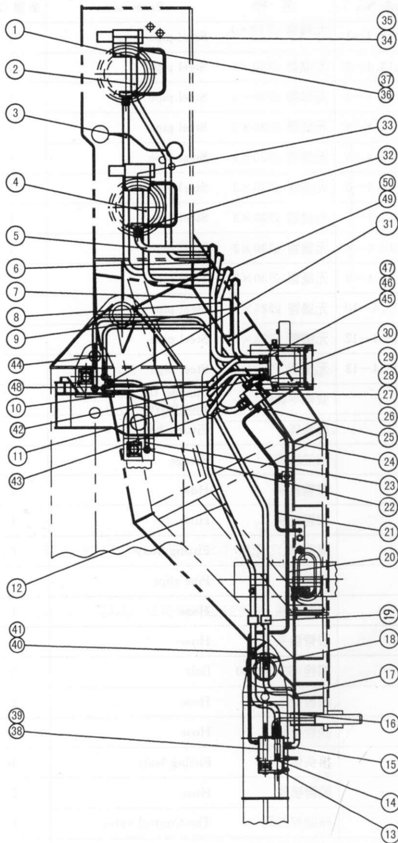
QY25K5. 13.4 起升变幅伸缩配管 The Rise、Change The Range's The Pipe Route Picture
