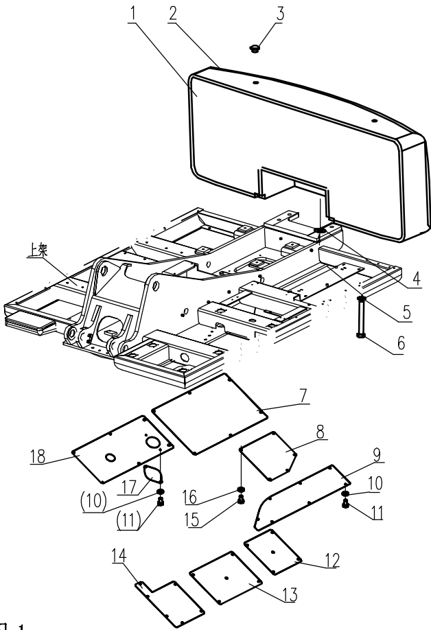
配重 底盖板装配 1 COUNTERWEIGHT AND UNDER COVER MOUNTING 1
