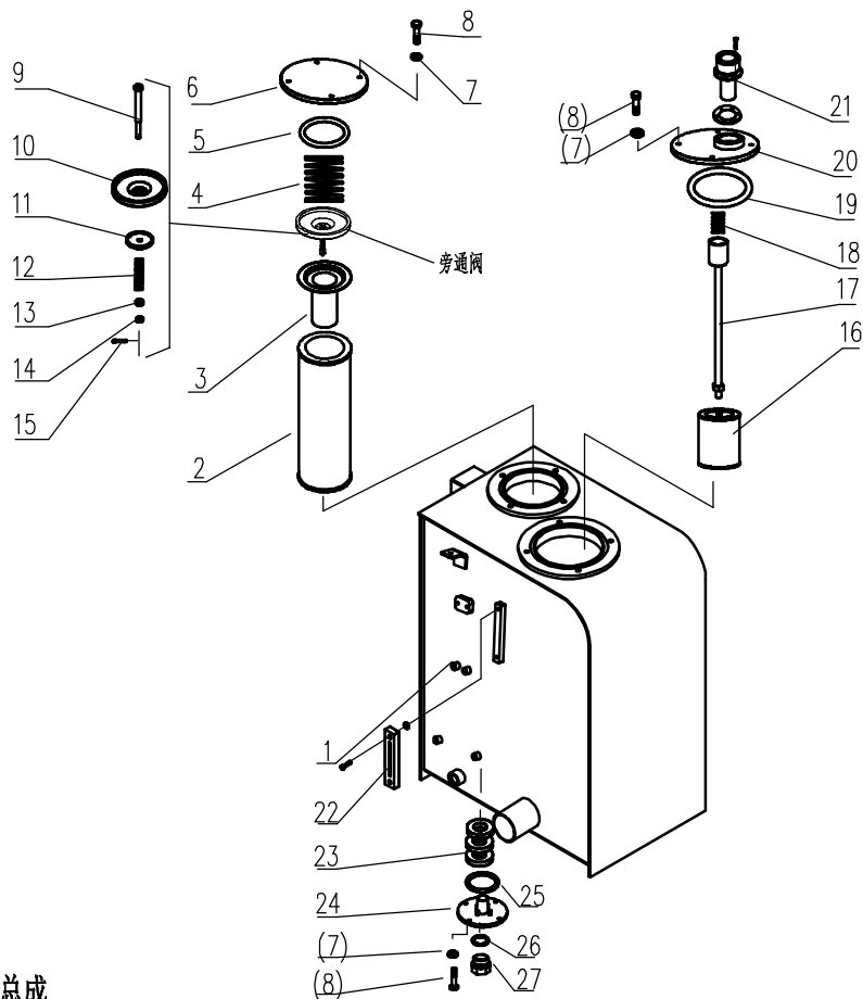
液压油箱总成 HYDRAULIC TANK ASS'Y
