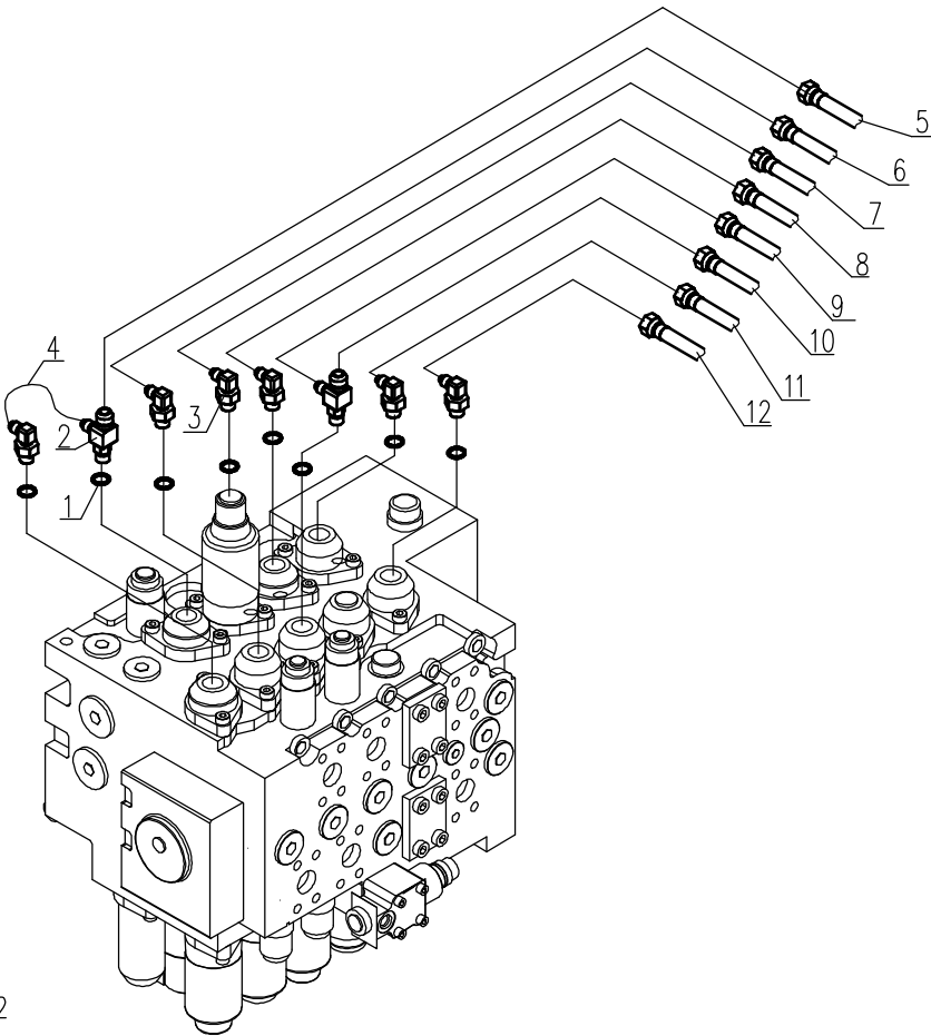
主阀组装 2 MAIN VALVE MOUNTING 2
