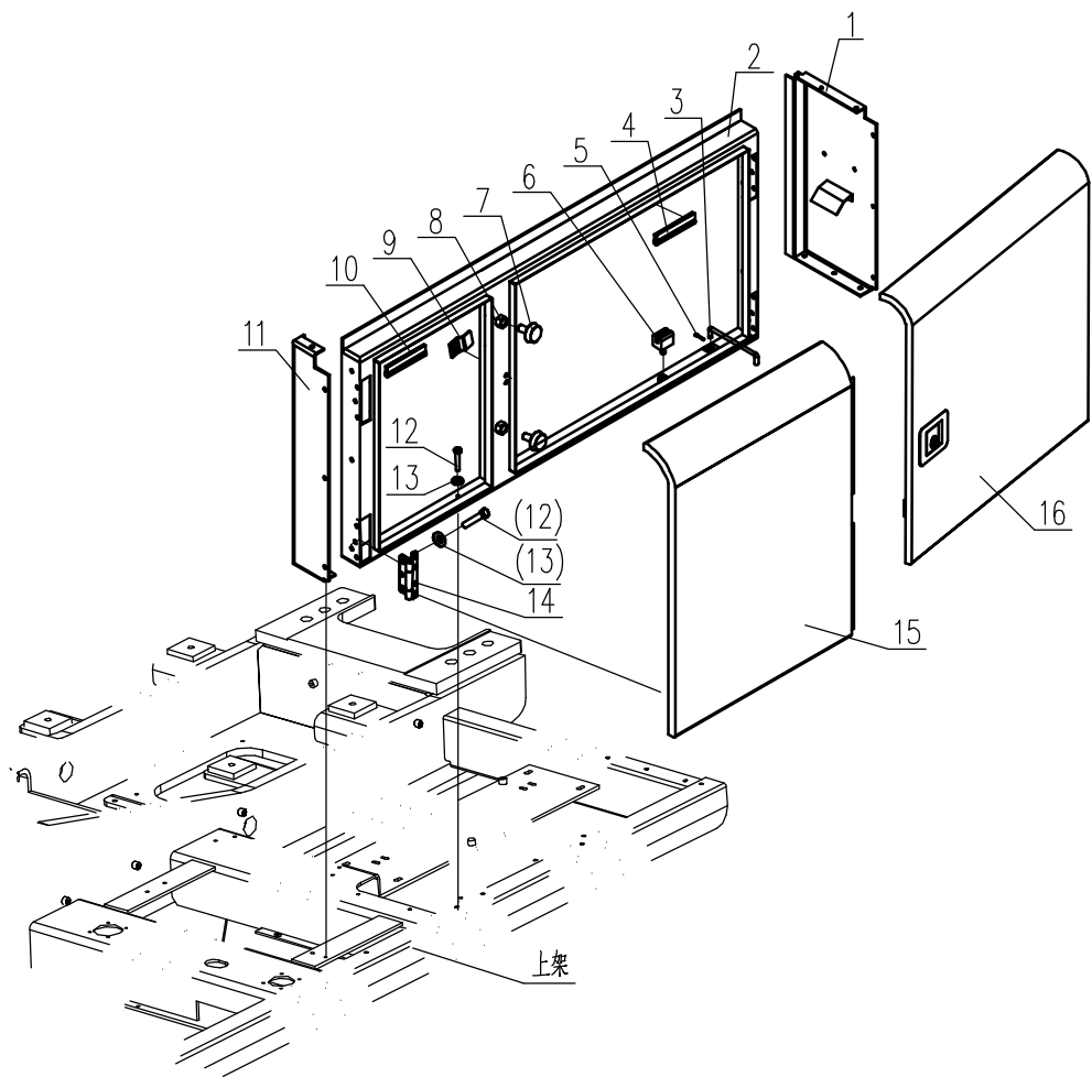
水箱 左侧门安装 3 RADIATOR AND LEFT DOOR MOUNTING 3
