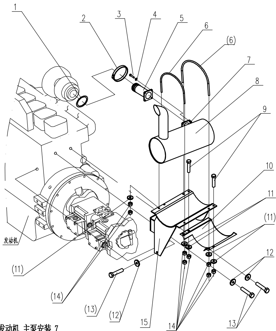
ENGINE AND MAIN PUMP MOUNTING 7
