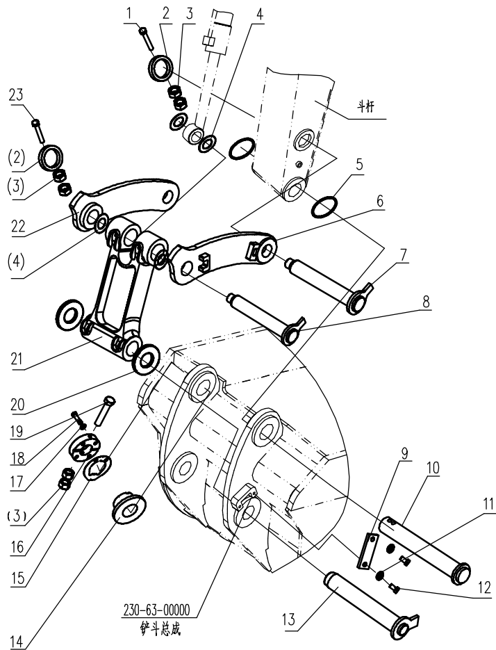
工作装置总装 3 WORKING EQUIPMENT MOUNTING 3
