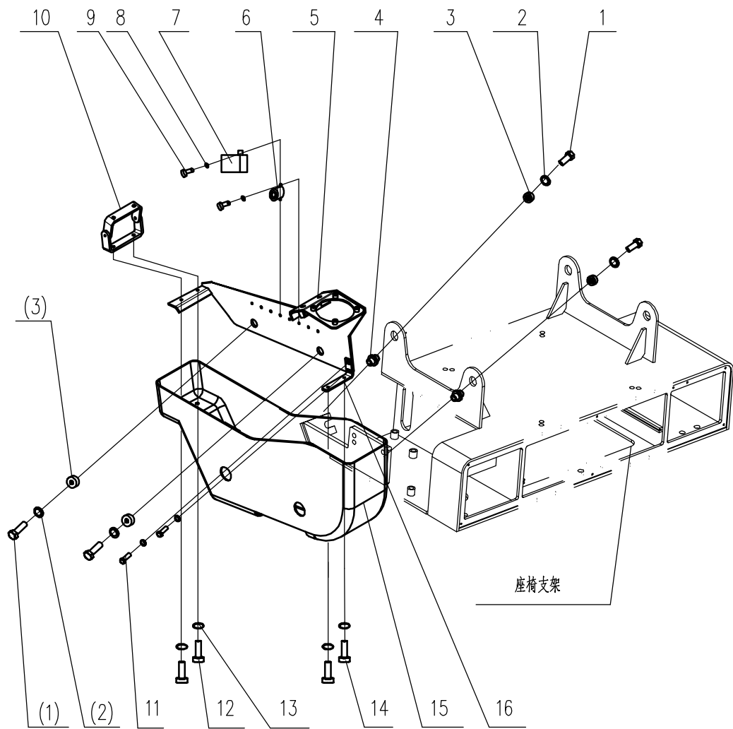
台架组装 8 BENCH MOUNTING 8
