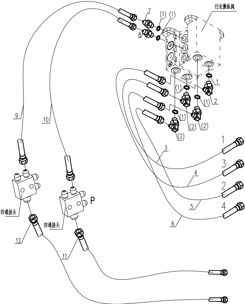
台架组装 3 BENCH MOUNTING 3
