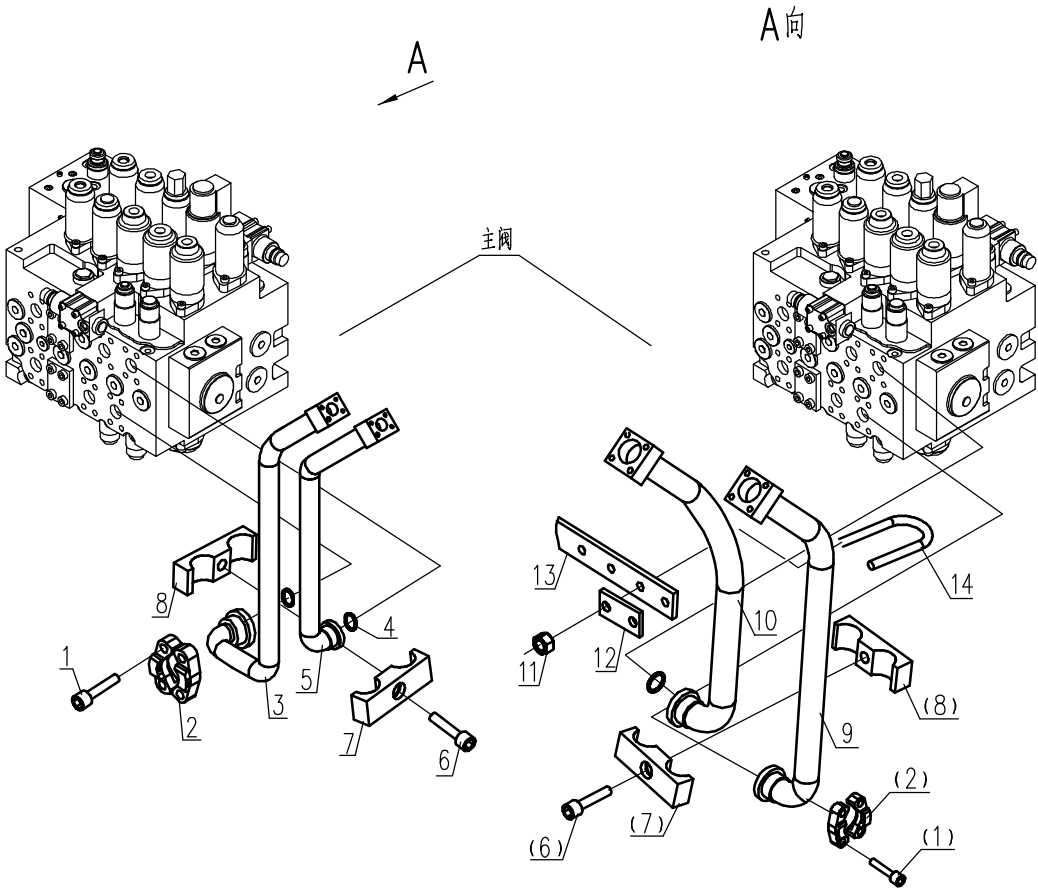
主阀组装 6 MAIN VALVE MOUNTING 6
