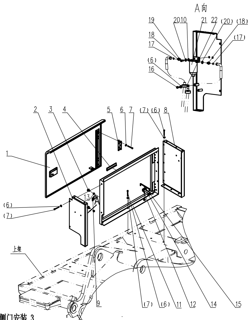
右侧箱体及侧门安装 3 RIGHT BOX AND DOOR MOUNTING 3
