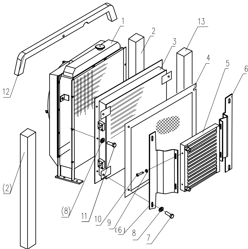
水箱 左侧门安装 1 RADIATOR AND LEFT DOOR MOUNTING 1
