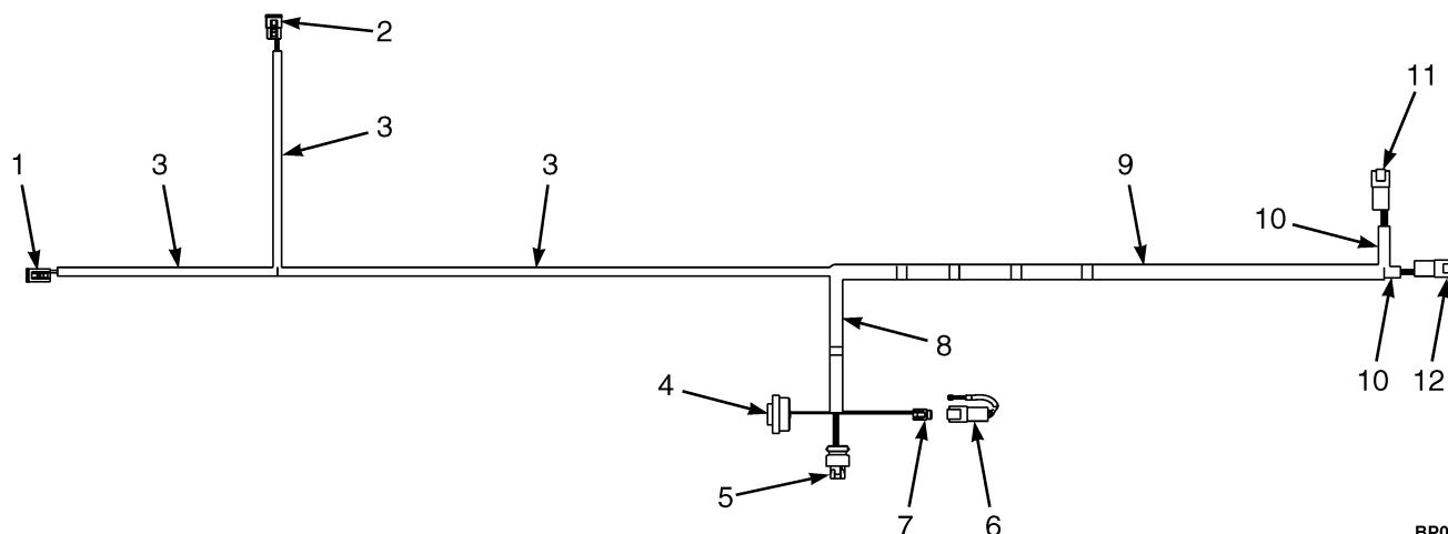
WIRE HARNESS (FIGURE 2-29) RH LIGHT WITH FREEZER DISPLAY — WITH TURN SIGNAL (10/2013 →)
