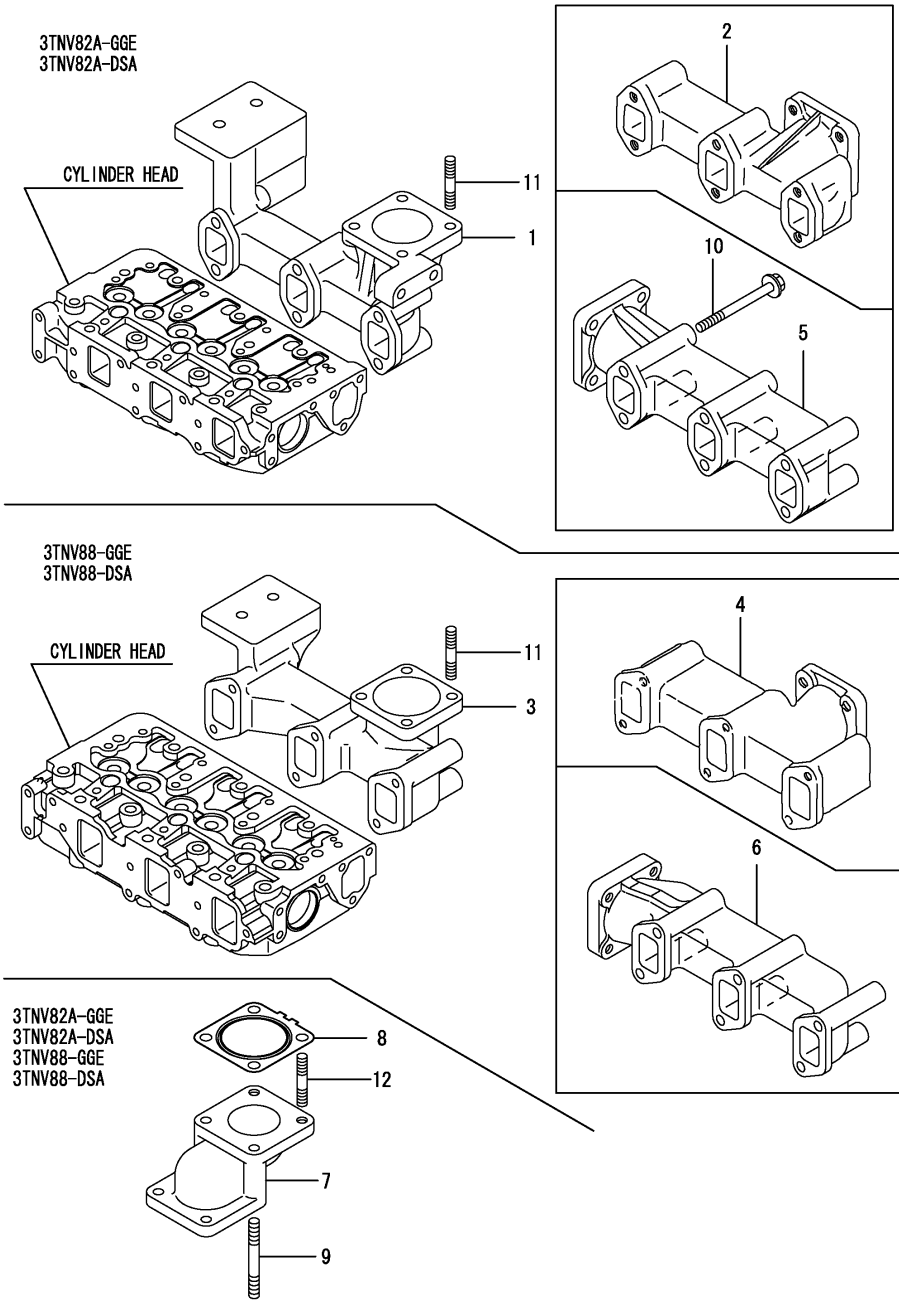
Fig.3. EXHAUST MANIFOLD
