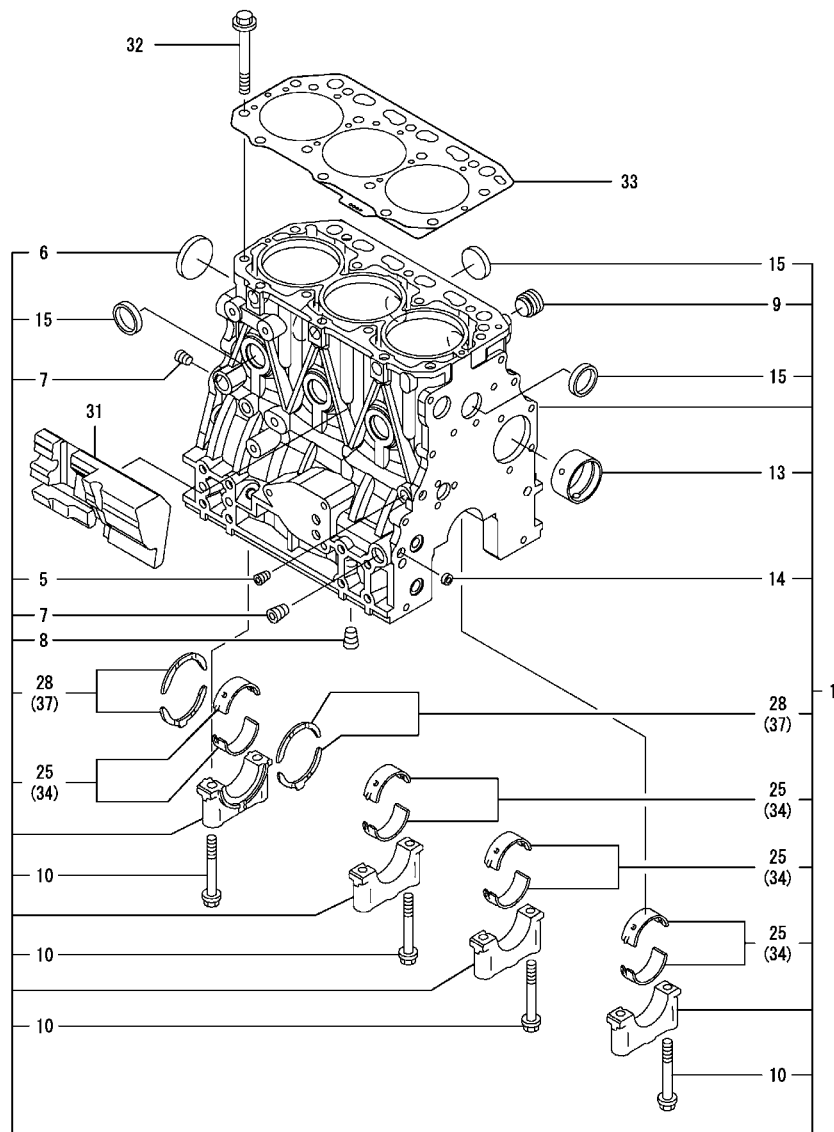
Fig.1. CYLINDER BLOCK
