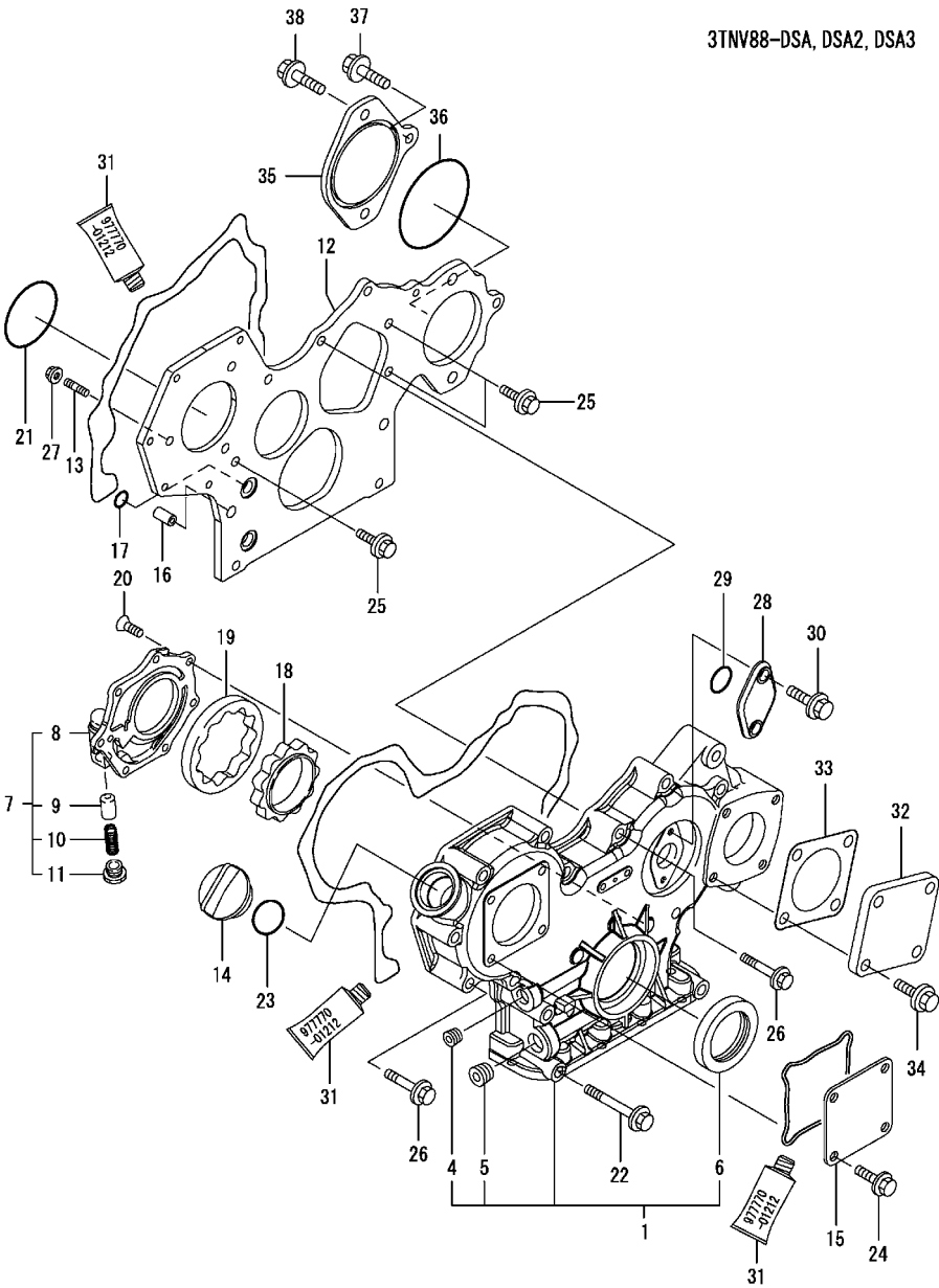
Fig.2. GEAR HOUSING
