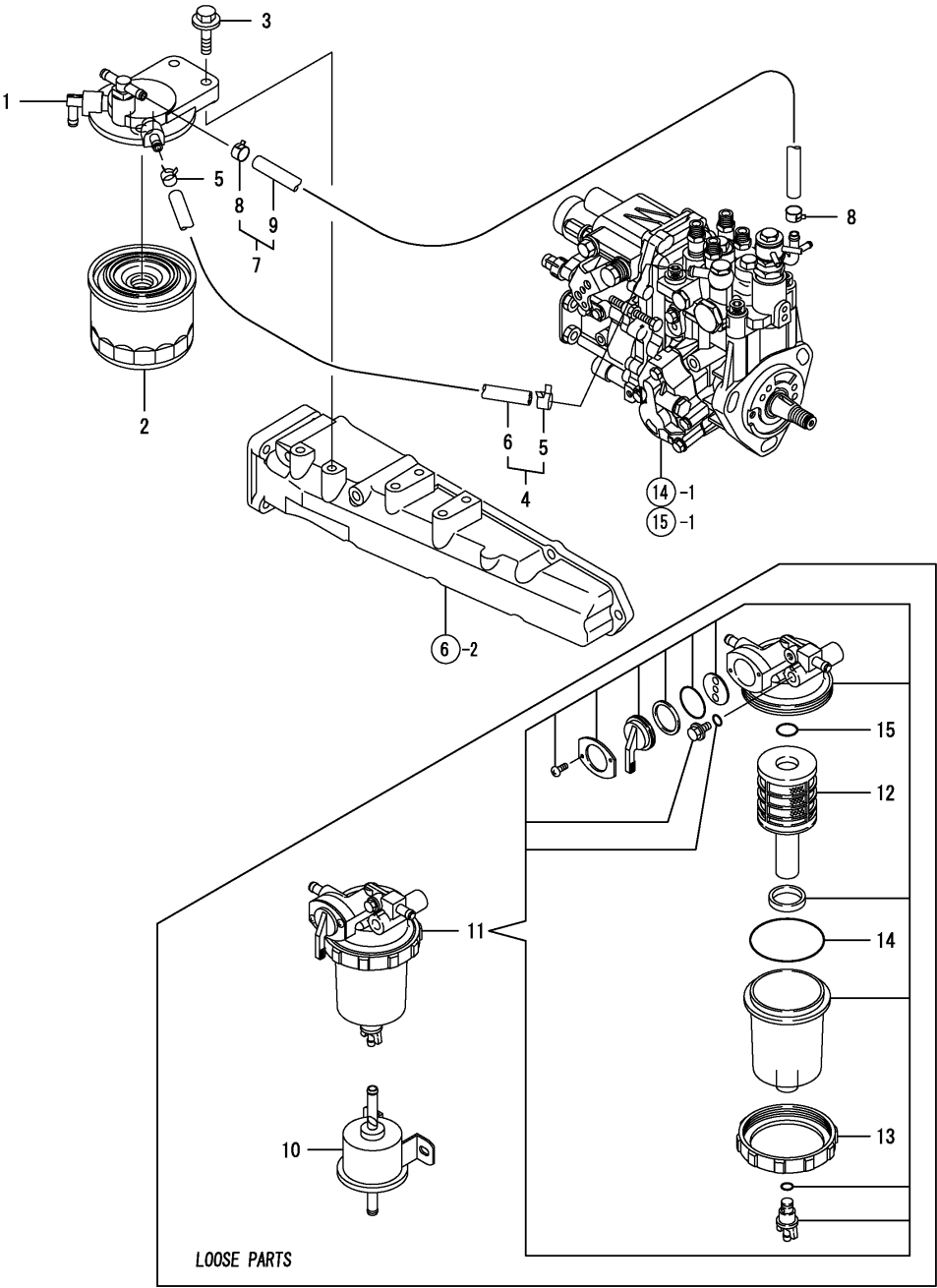
Fig.18. FUEL LINE
