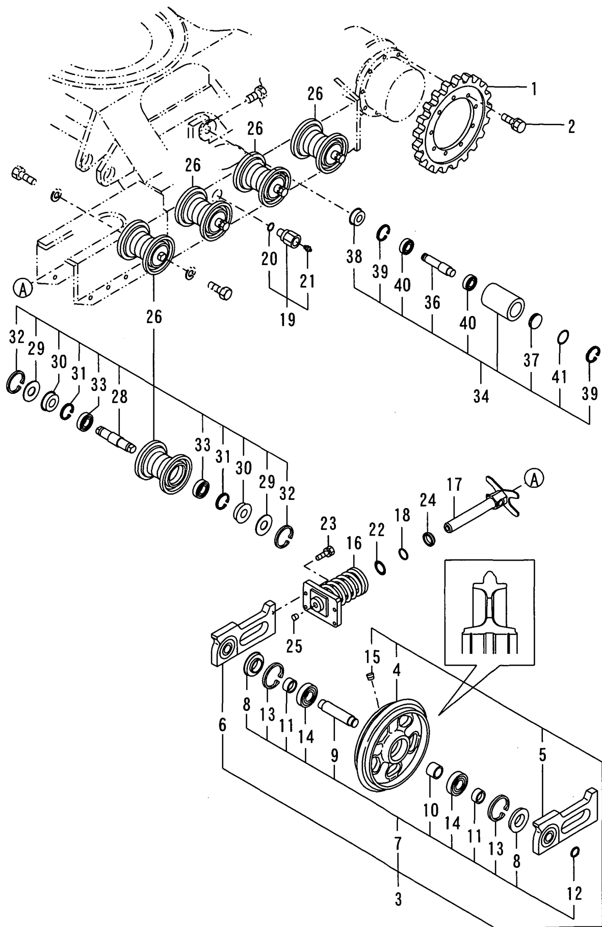
Fig. 1 ROLLER & ADJUST https://truckmanualshub.com/
