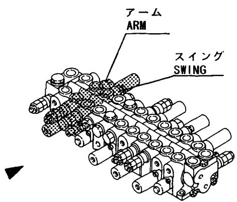
コントロールバルブ ASSY CONTROL VALVE ASSY 172168-74120 Fig. 40 Ref. No. 1 INC Fig. 40 Ref. No. 2~34 Fig. 41 Ref. No. 1~40 Fig. 42 Ref. No. 1~36 Fig. 43 Ref. No. 1~34 Fig. 44 Ref. No. 1~25
