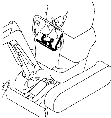
Fig. 16 CONTROL EQUIPMENT (STOPPER LEVER)
