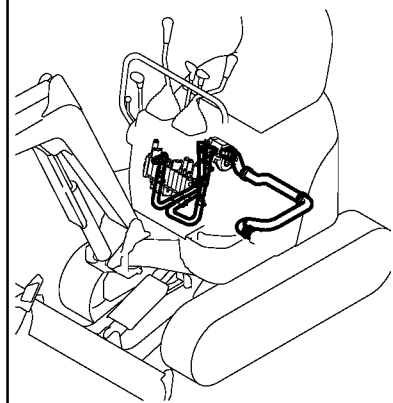
Fig. 48 HYD. OIL PIPING (CONTROL V. ~ TURNING MT SWING CYL.)
