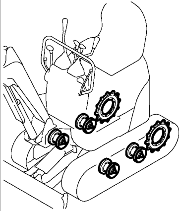
Fig. 14 CRAWLER, IDLER &amp; ADJUST
