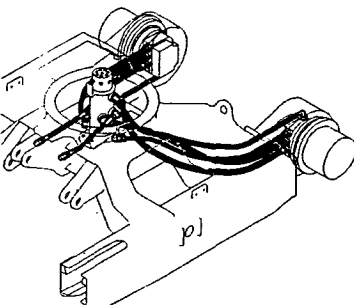
Fig. 54 油圧配管 (走行) (レンコン仕様) HYD. OIL PIPING (TRAVEL) (LOTUS ROOT SPEC.)
