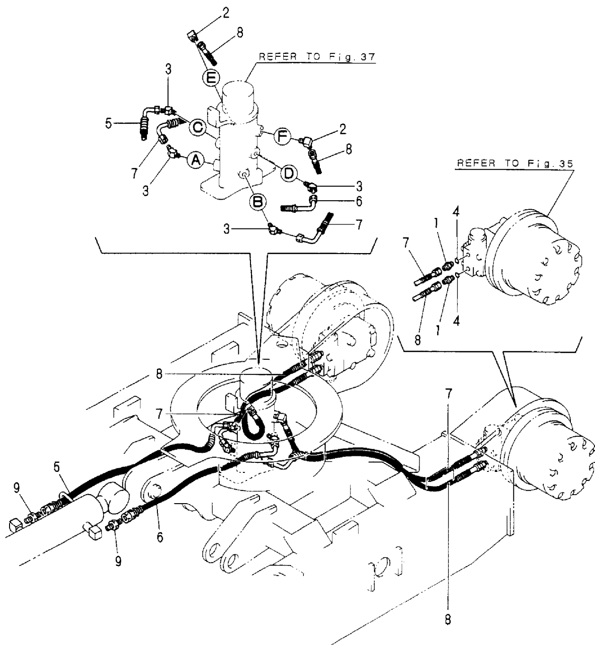
Fig. 53 油压配管 (走行) HYD. OIL PIPING (TRAVEL)
