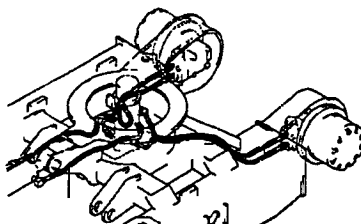
Fig. 53 油圧配管 (走行) HYD. OIL PIPING (TRAVEL)
