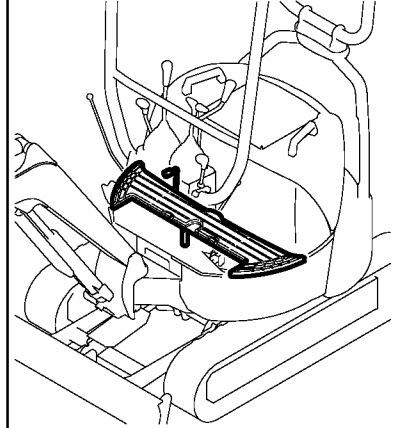
Fig. 23 INSTRUMENT PANEL & SEAT MOUNT
