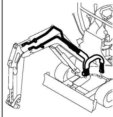
Fig. 47 GREASING
