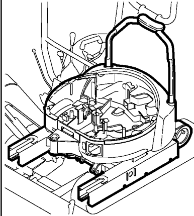
Fig. 20 FRAME &amp; TURNING BEARING
