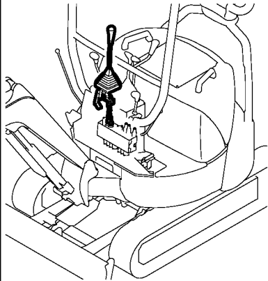
Fig. 16 CONTROL EQUIPMENT (OPERATION: ARM & TURNING)
