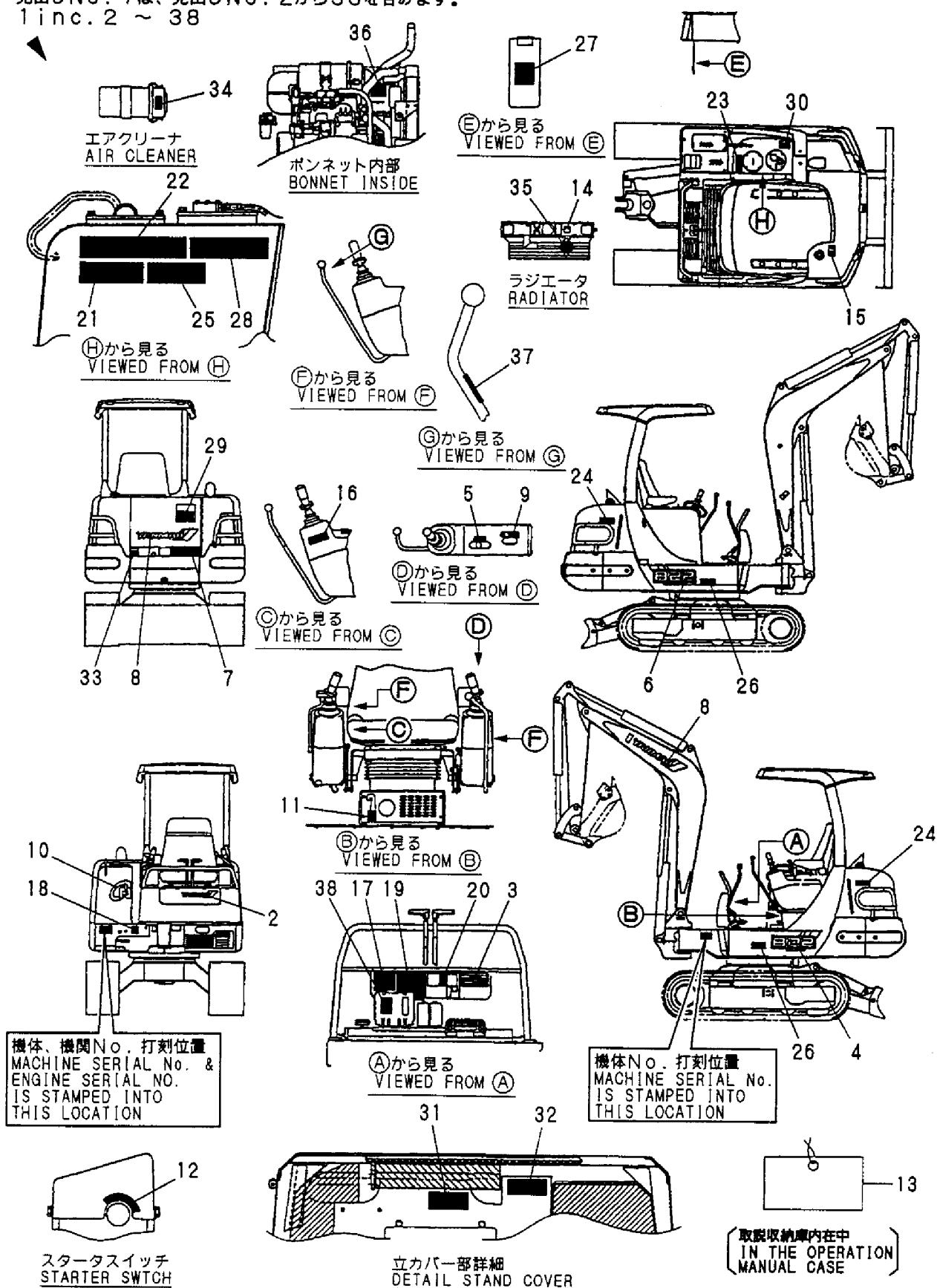
Fig. 6 銘板 (キャノピ) (AS) LABEL (CANOPY) (AS)
