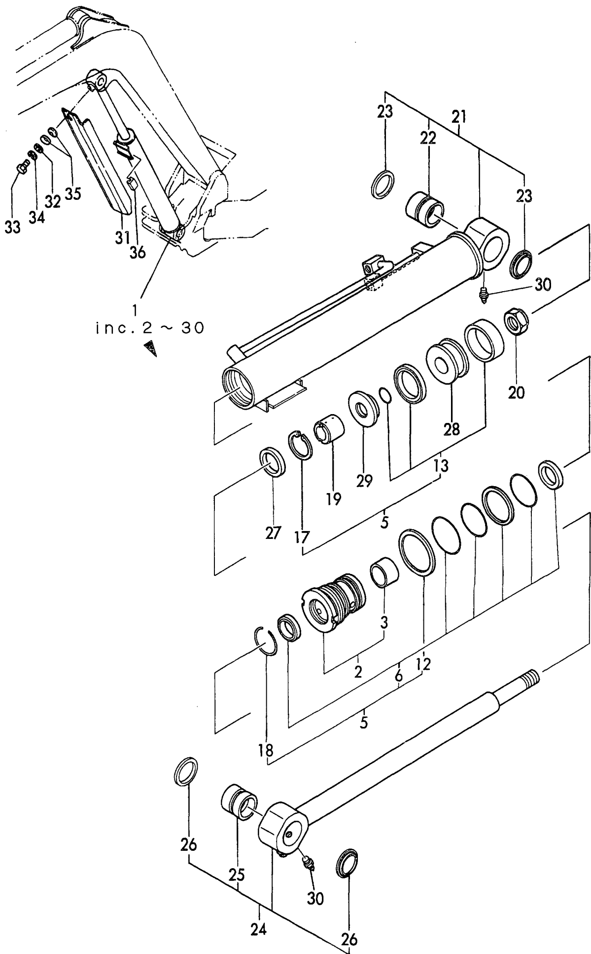
Fig. 30 BOOM CYLINDER https://truckmanualshub.com/
