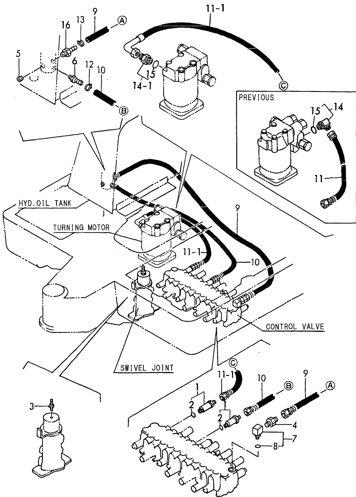
Fig. 53 HYD.OIL PIPING (RETURN) https://ruclmanuals.club.com/
