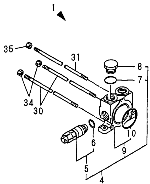
PUMP 1
