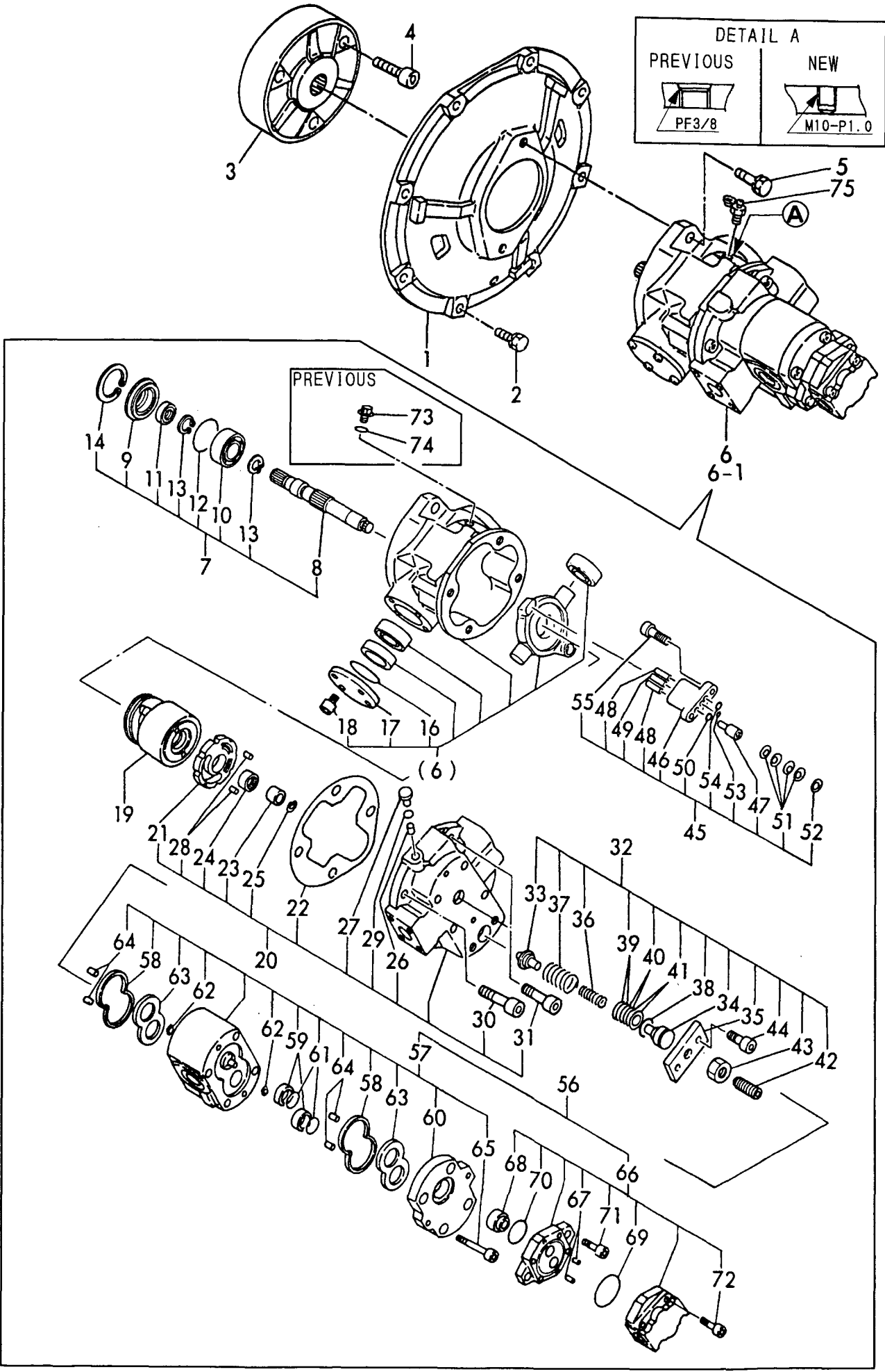
Fig. 29 HYD. OIL PUMP & JOINT https://truckmanualshub.com/
