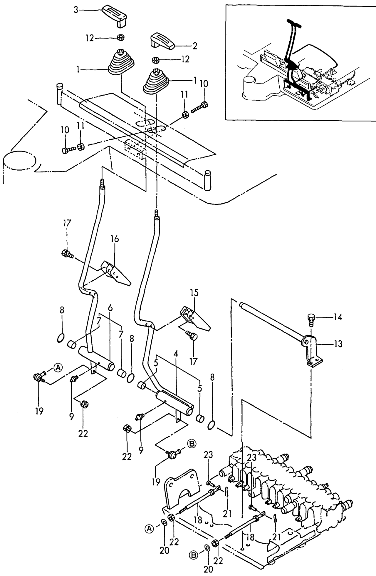
Fig. 16 CONTROL EQUIPMENT (TRAVEL)
