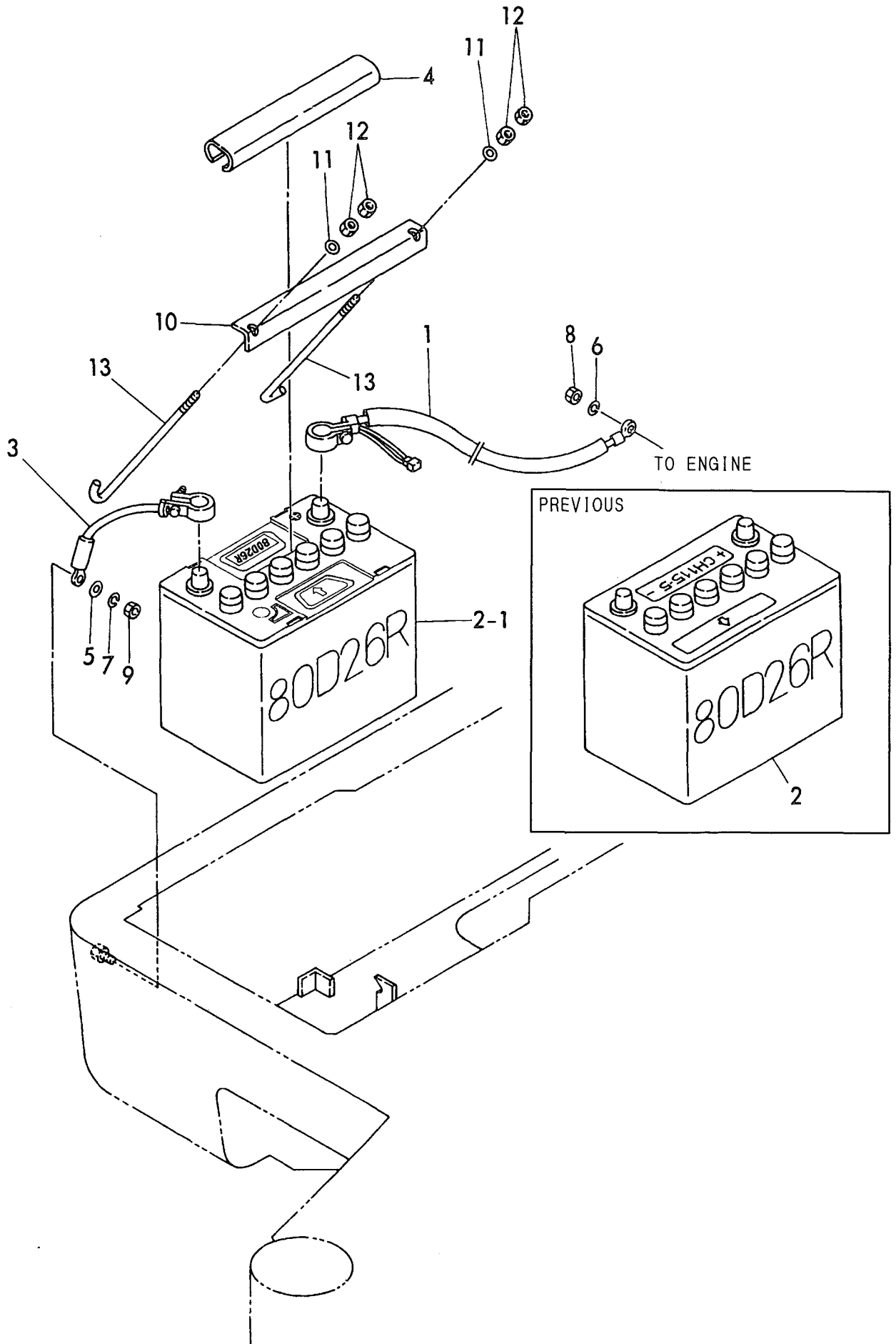
Fig. 8 BATTERY
