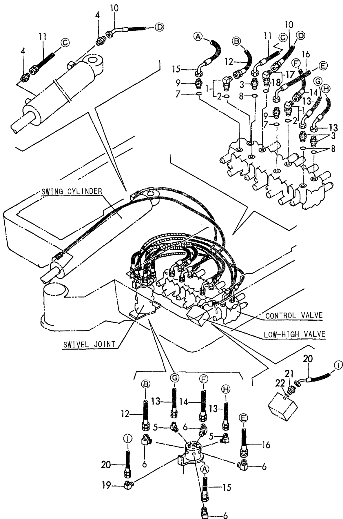
Fig. 52 HYD. OIL PIPING (VALVE SWIVEL, SWING)
