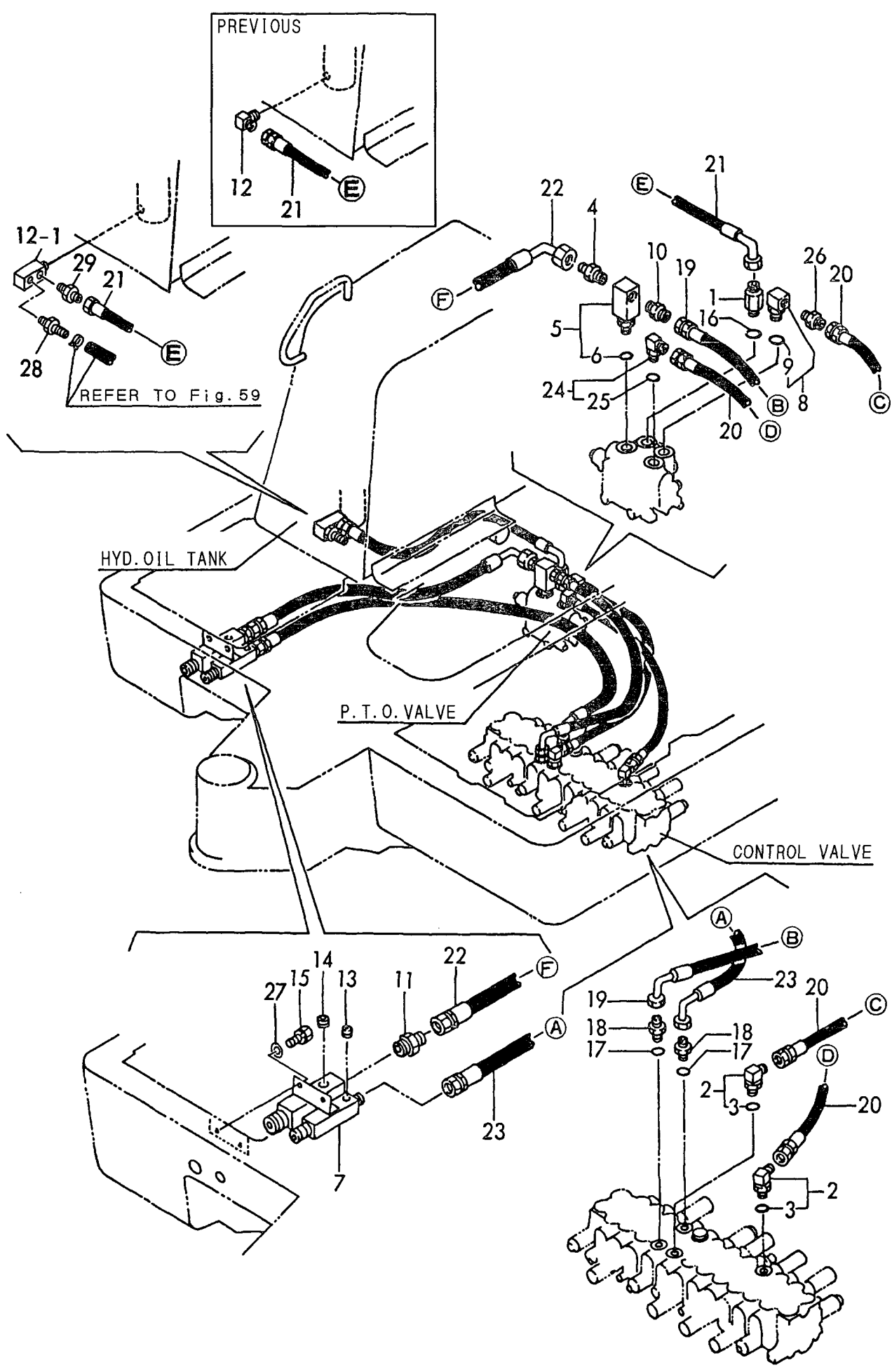
Fig. 54 HYD. OIL PIPING (P. T. O. VALVE, FRAME)
