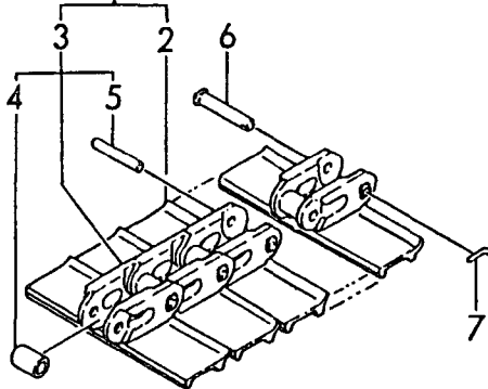
CRAWLER (270)
