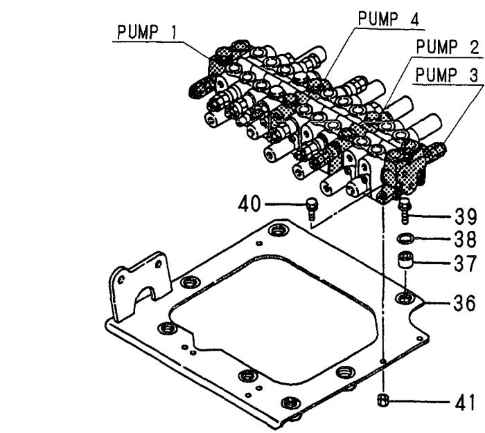
PUMP 4
