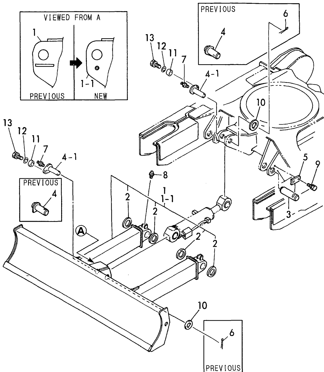
Fig. 63 BLADE (850) https://truckmanualshub.com/
