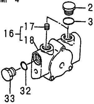
PUMP 4
