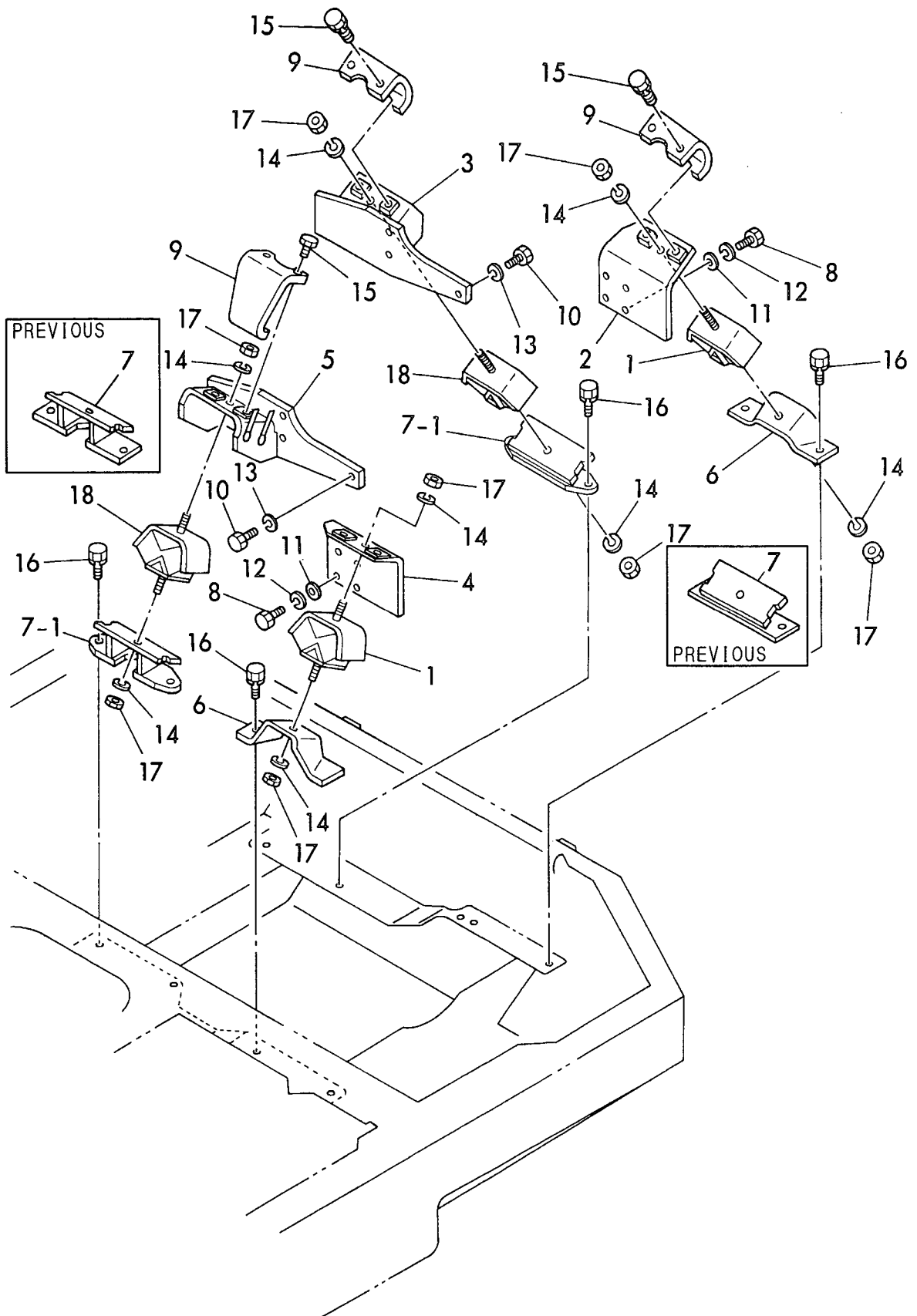
Fig. 5 ENGINE MOUNT https://truckmanualshub.com/
