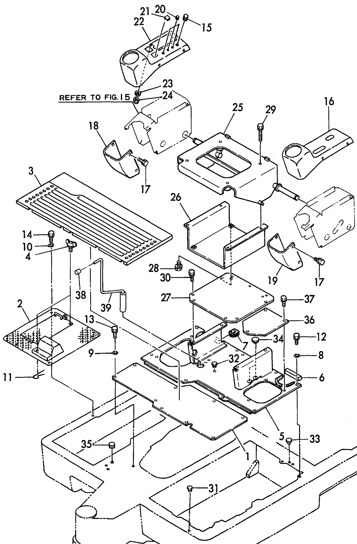
Fig. 24 SEAT MOUNT & STEP https://trucks.mmmalshub.com/
