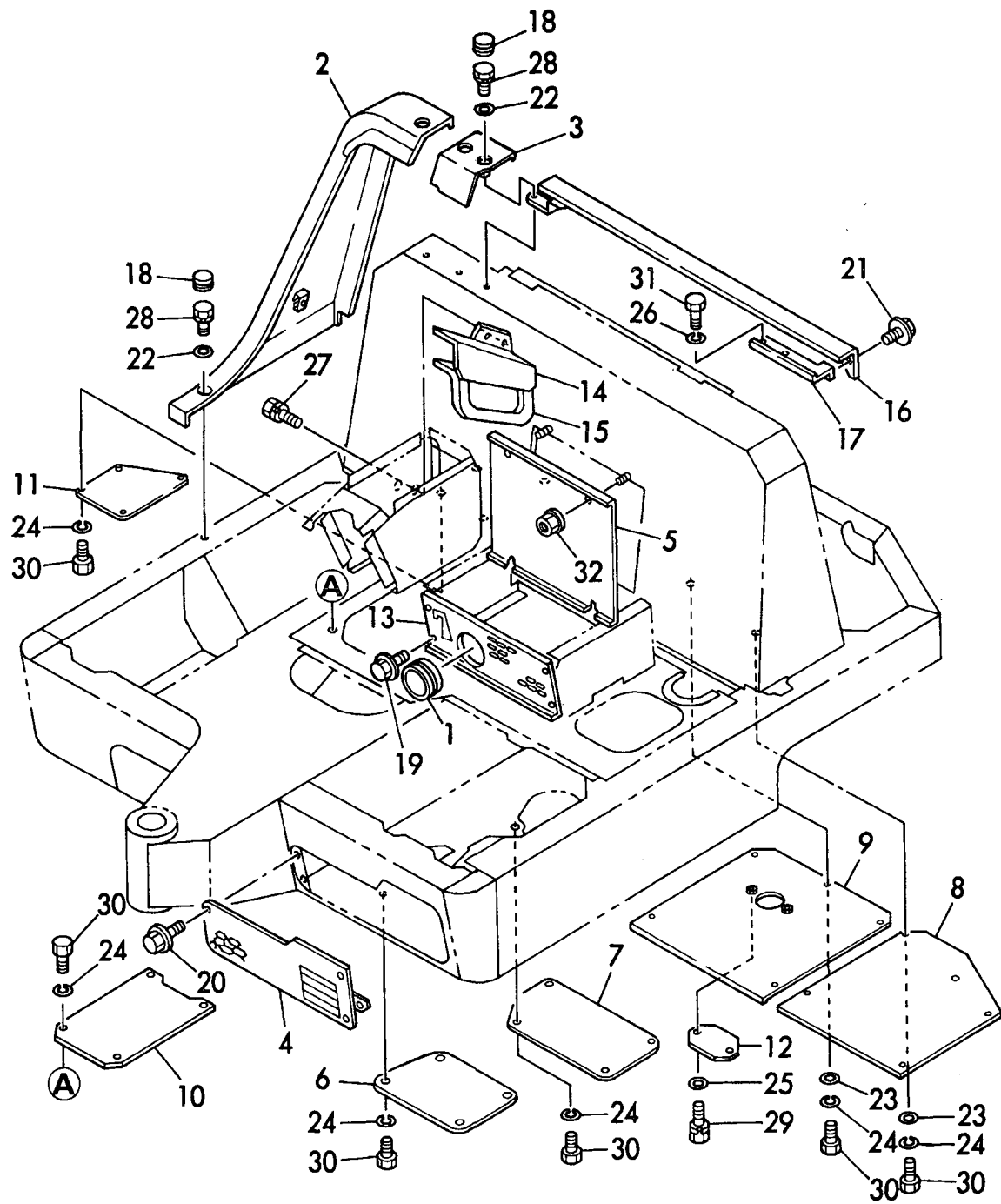
Fig. 22 FRAME COVER (CABIN) https://rukkmanualshub.com/
