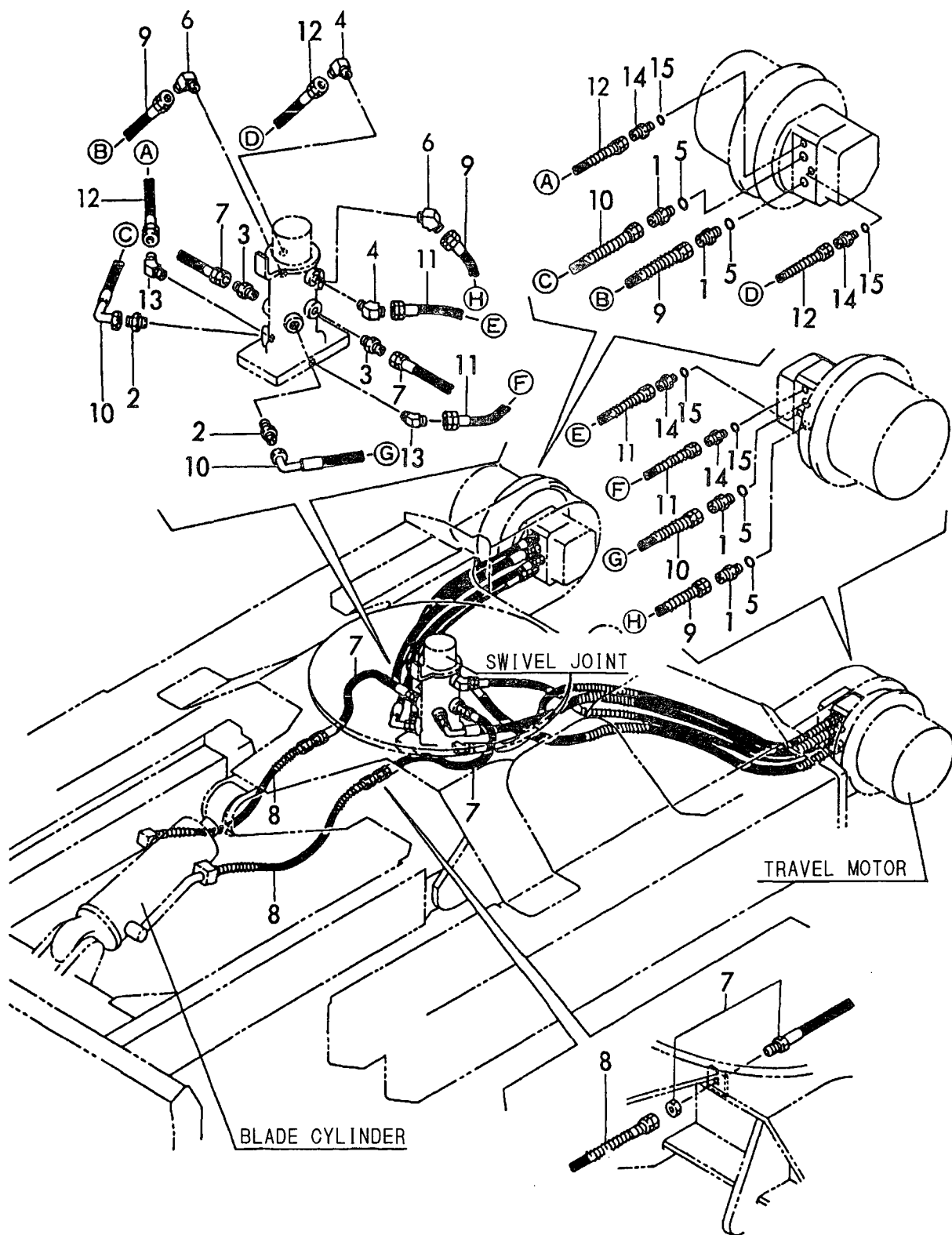
Fig. 56 HYD.OIL PIPING (TRAVEL) (DOUBLE SPEED) (NEW)
