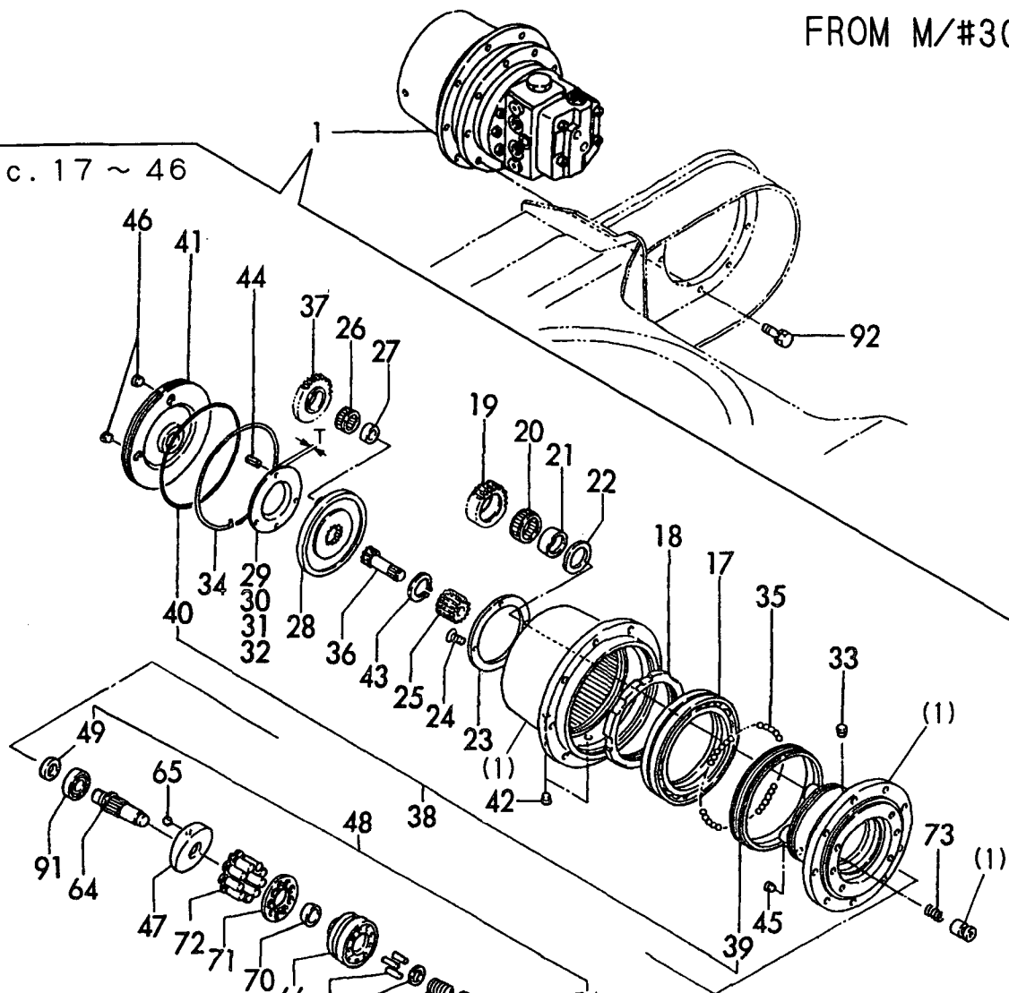
Fig. 36 TRAVEL MOTOR (DOUBLE SPEED) (NEW)
