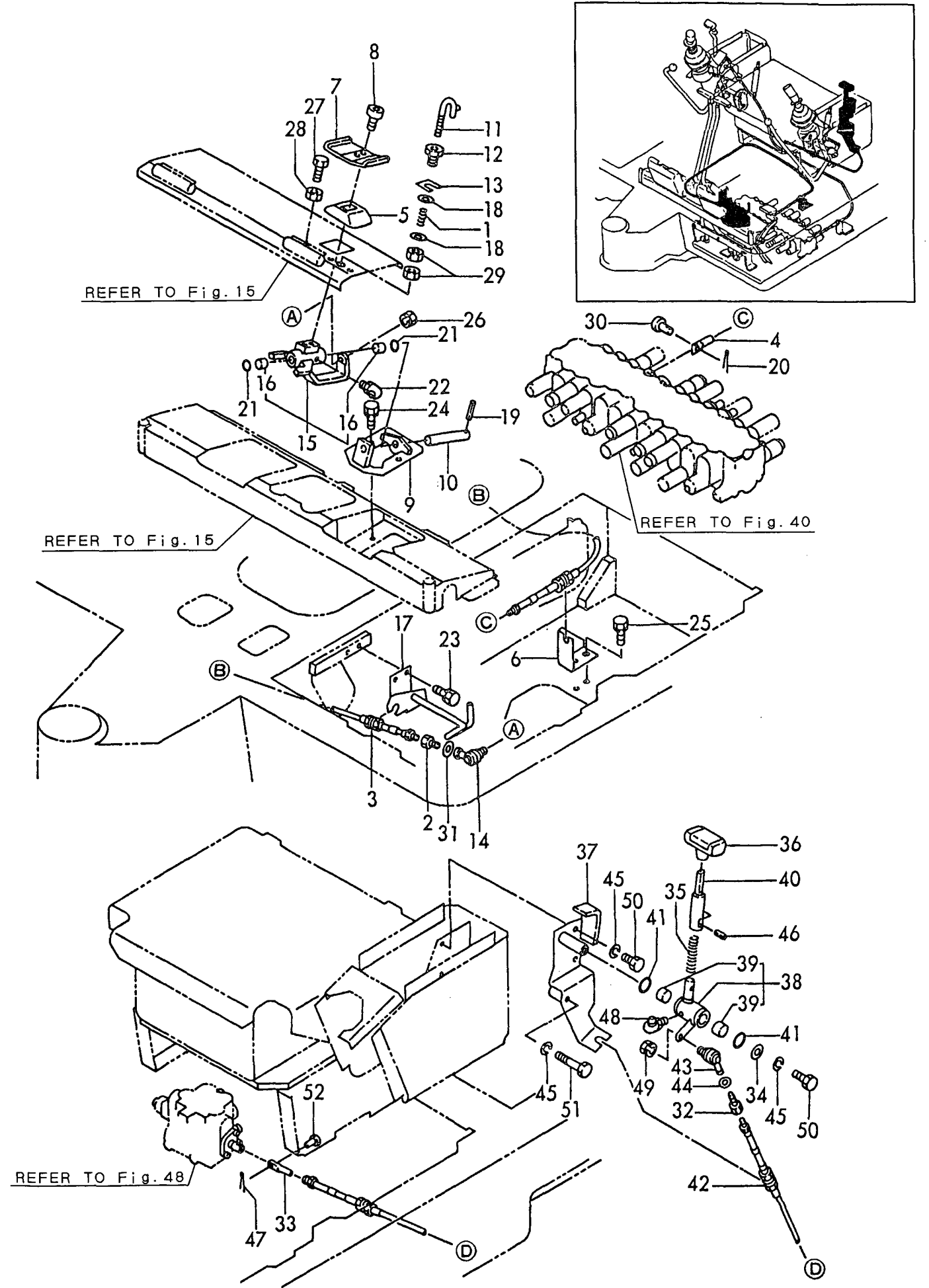
Fig. 20 CONTROL EQUIPMENT (P. T. O. CONTROL)
