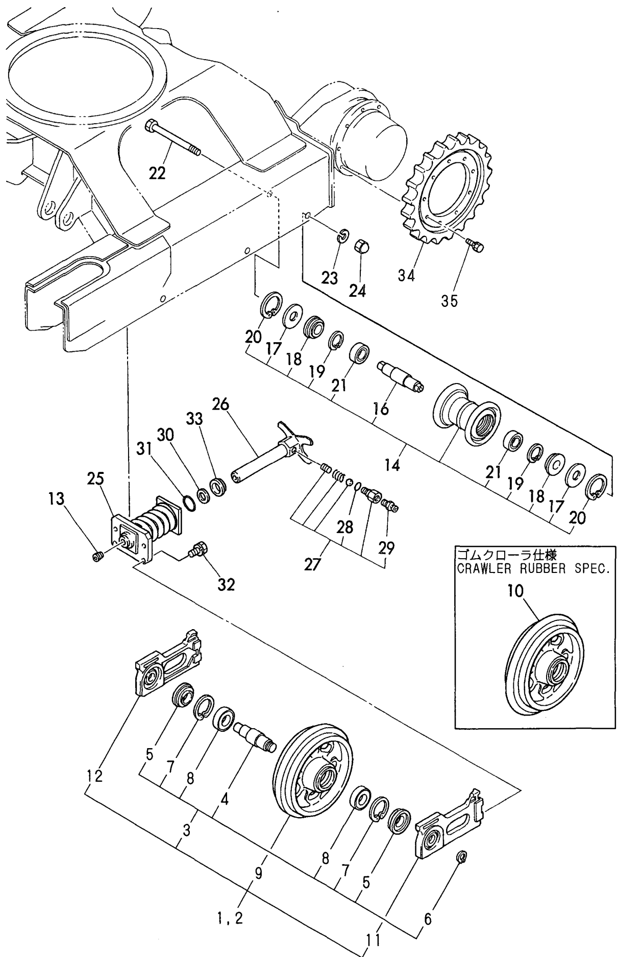
Fig. 13 ROLLER & ADJUST http://stickmanualshub.com/
