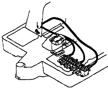
Fig.54 HYD.OIL PIPING (P.T.O. VALVE, FRAME)
