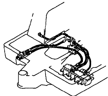
Fig.55 HYD.OIL PIPING (TRAVEL) (SINGLE SPEED) (PREVIOUS)
