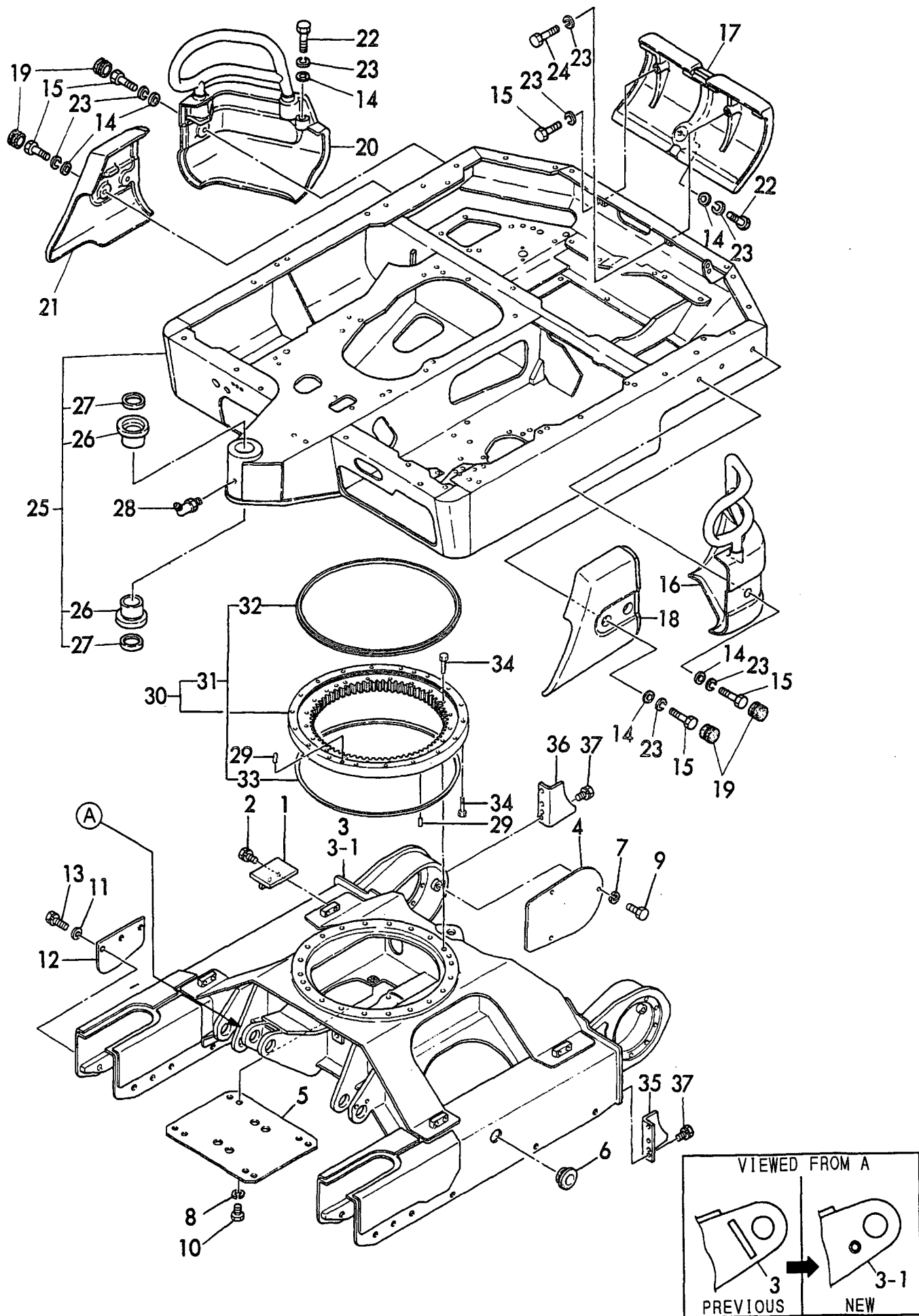
Fig. 21 FRAME & TURNING BEARING https://truckmanualshub.com/
