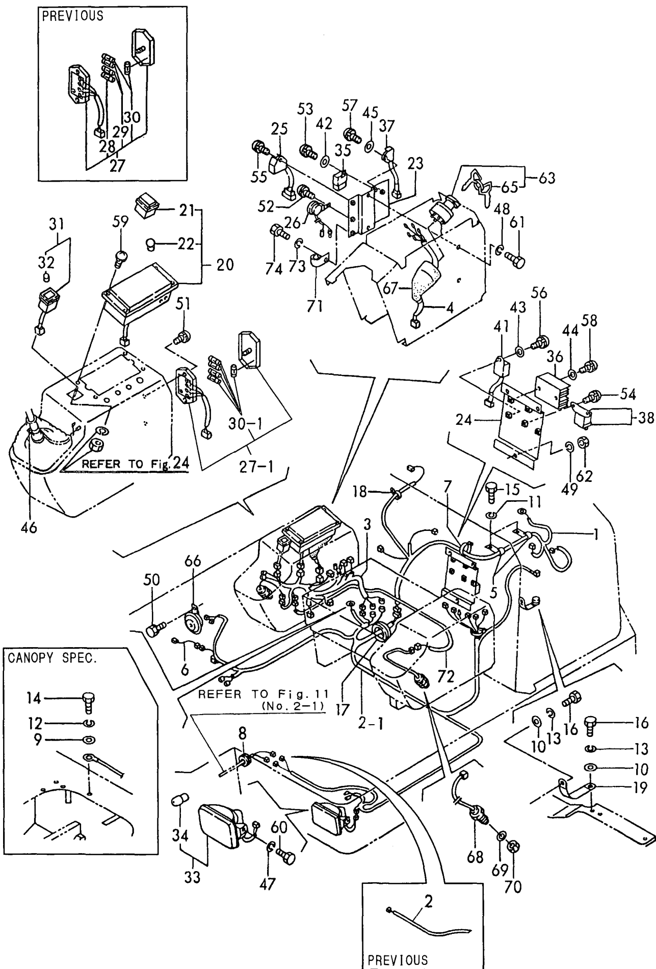
Fig. 9 ELECTRIC PART (CABIN, CANOPY) https://truckmanparts.com/
